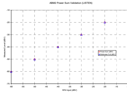
Figure 4-10 ABM2 Power Sum Validation
