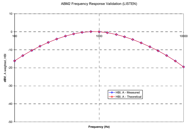
Figure 4-8 ABM2 Frequency Response Validation
