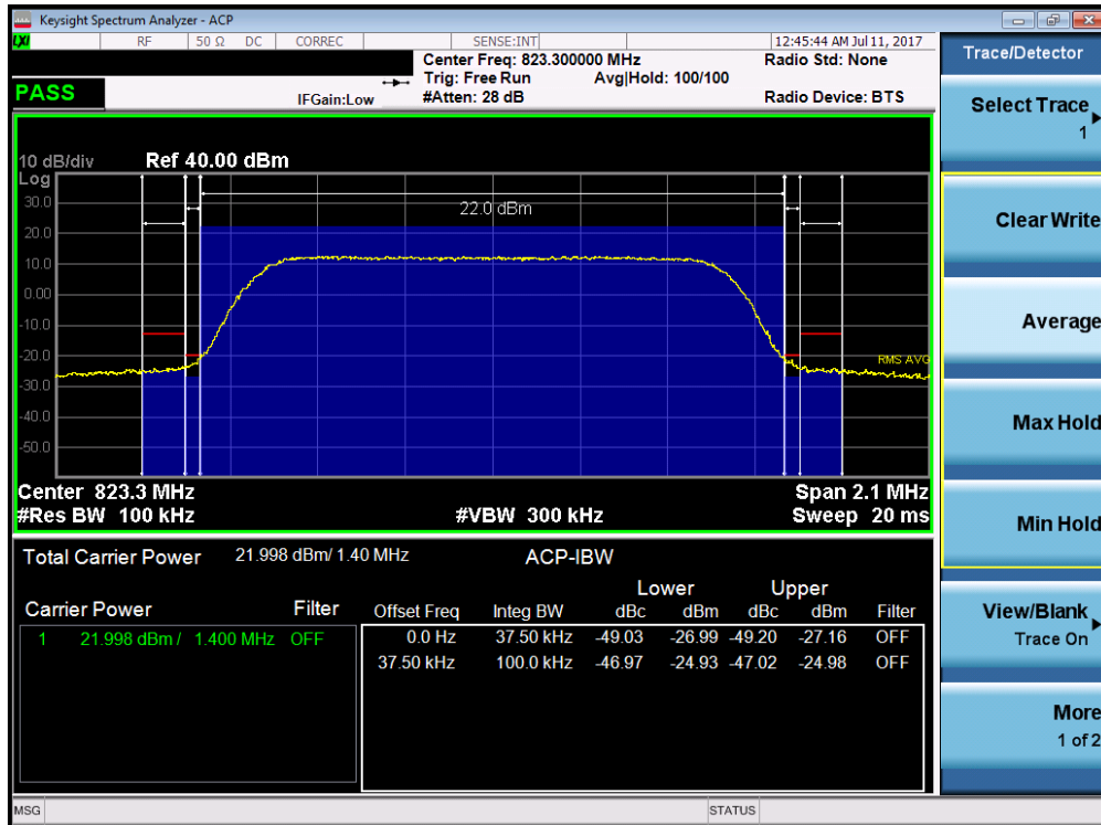
Plot 7-24. Channel Edge Plot (1.4MHz QPSK – RB Size 6 – High Channel)
