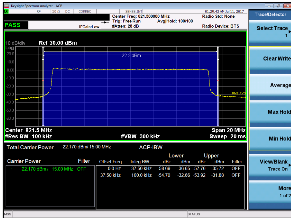
Plot 7-30. Channel Edge Plot (15MHz QPSK – RB Size 75)
