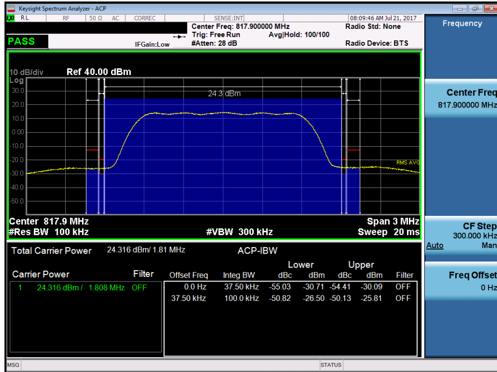
Plot 7-21. Channel Edge Plot (Ch. 476)
