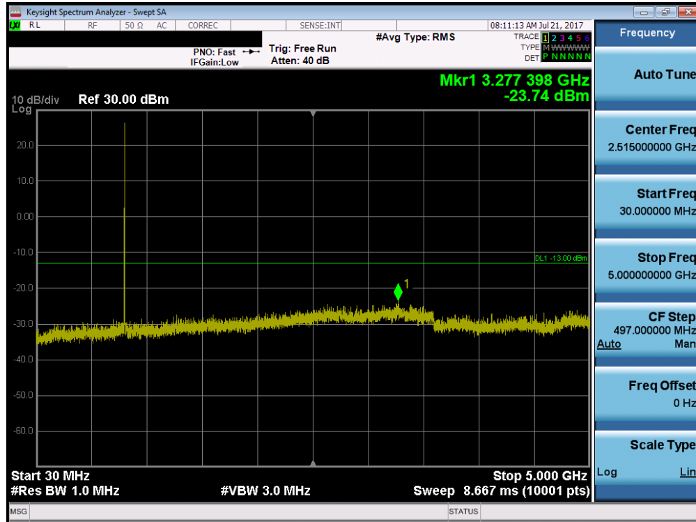
Plot 7-15. Conducted Spurious Plot (Ch. 684)
