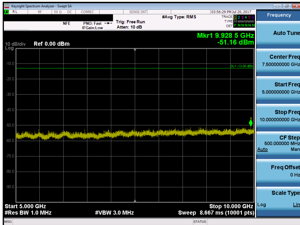
Plot 7-20. Conducted Spurious Plot ( 1.4MHz QPSK – RB Size 1, RB Offset 0 – High Channel)
