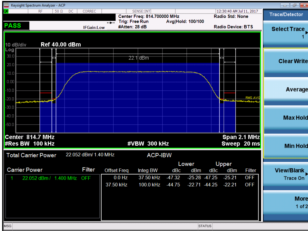
Plot 7-23. Channel Edge Plot (1.4MHz QPSK – RB Size 6 – Low Channel)
