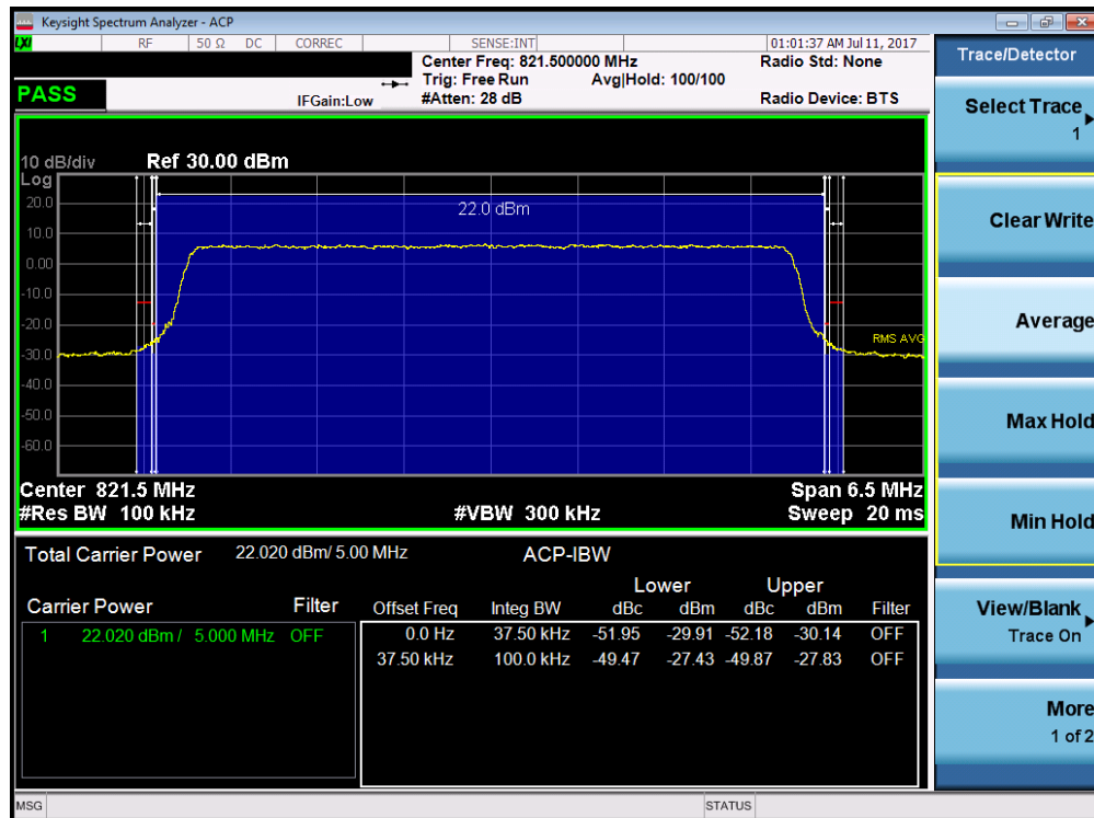
Plot 7-28. Channel Edge Plot (5MHz QPSK – RB Size 25 – High Channel)
