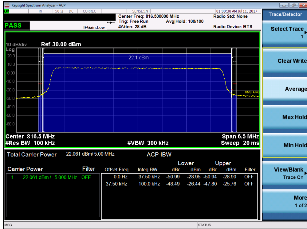
Plot 7-27. Channel Edge Plot (5MHz QPSK – RB Size 25– Low Channel)
