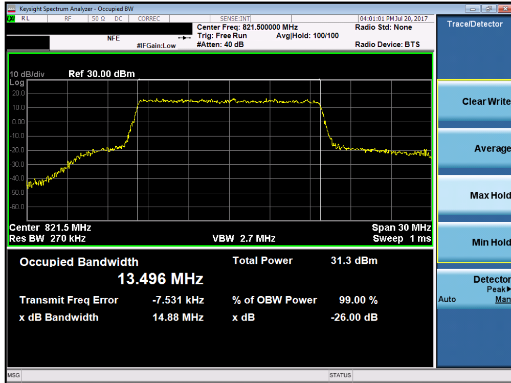
Plot 7-11. Occupied Bandwidth Plot (15MHz QPSK – RB Size 75)
