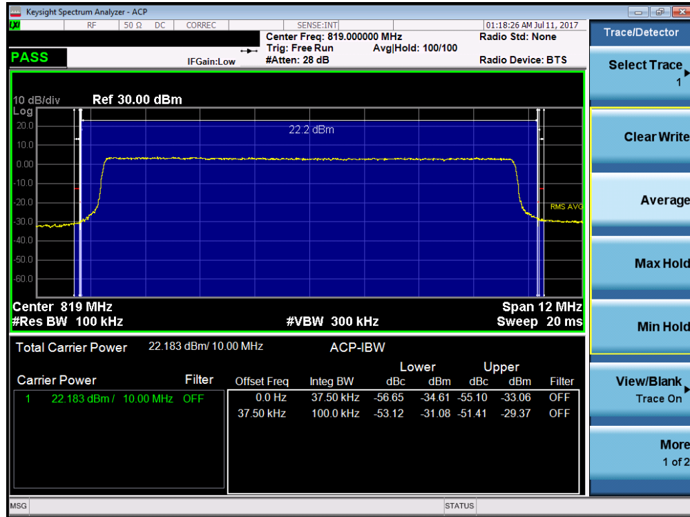
Plot 7-29. Channel Edge Plot (10MHz QPSK – RB Size 50)
