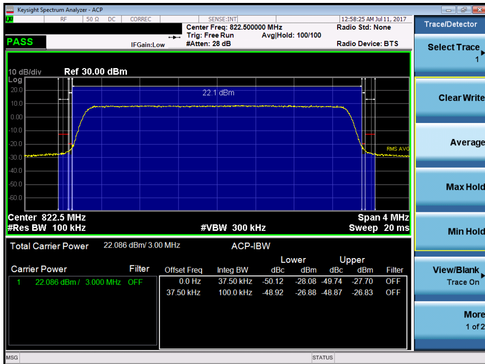
Plot 7-26. Channel Edge Plot (3MHz QPSK – RB Size 15 – High Channel)
