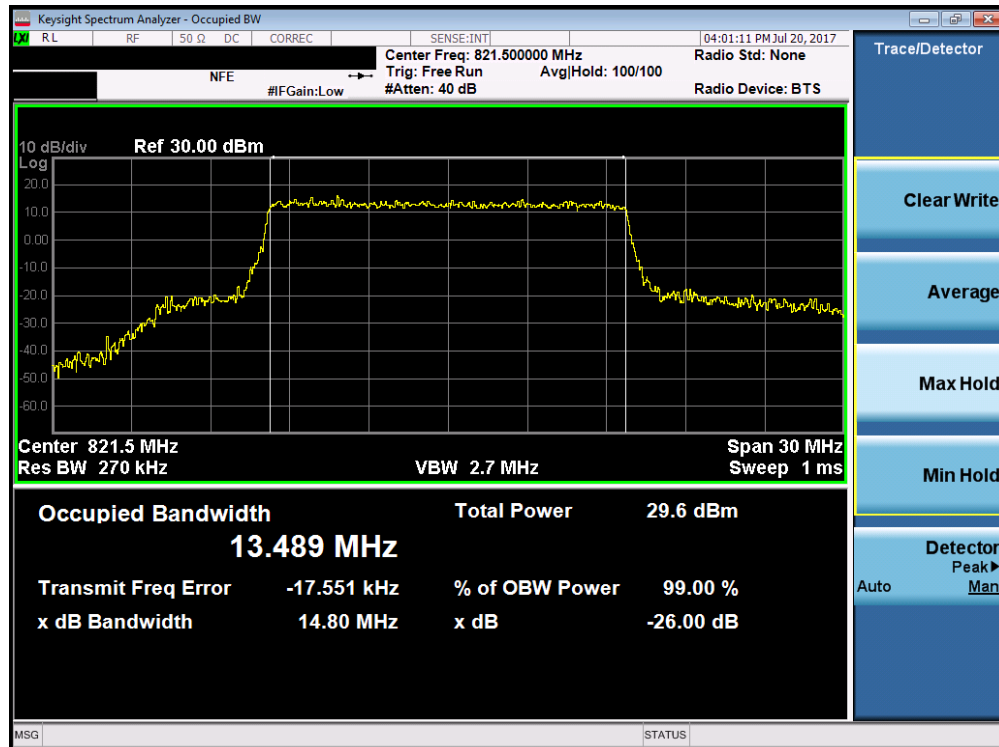
Plot 7-12. Occupied Bandwidth Plot (15MHz 16-QAM – RB Size 75)
