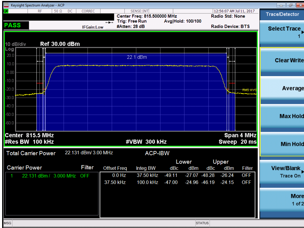
Plot 7-25. Channel Edge Plot (3MHz QPSK – RB Size 15– Low Channel)
