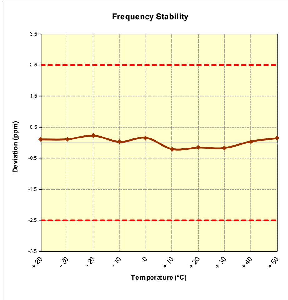
Figure 7-6. CDMA BC10 Frequency Stability Graph (Ch. 476)
