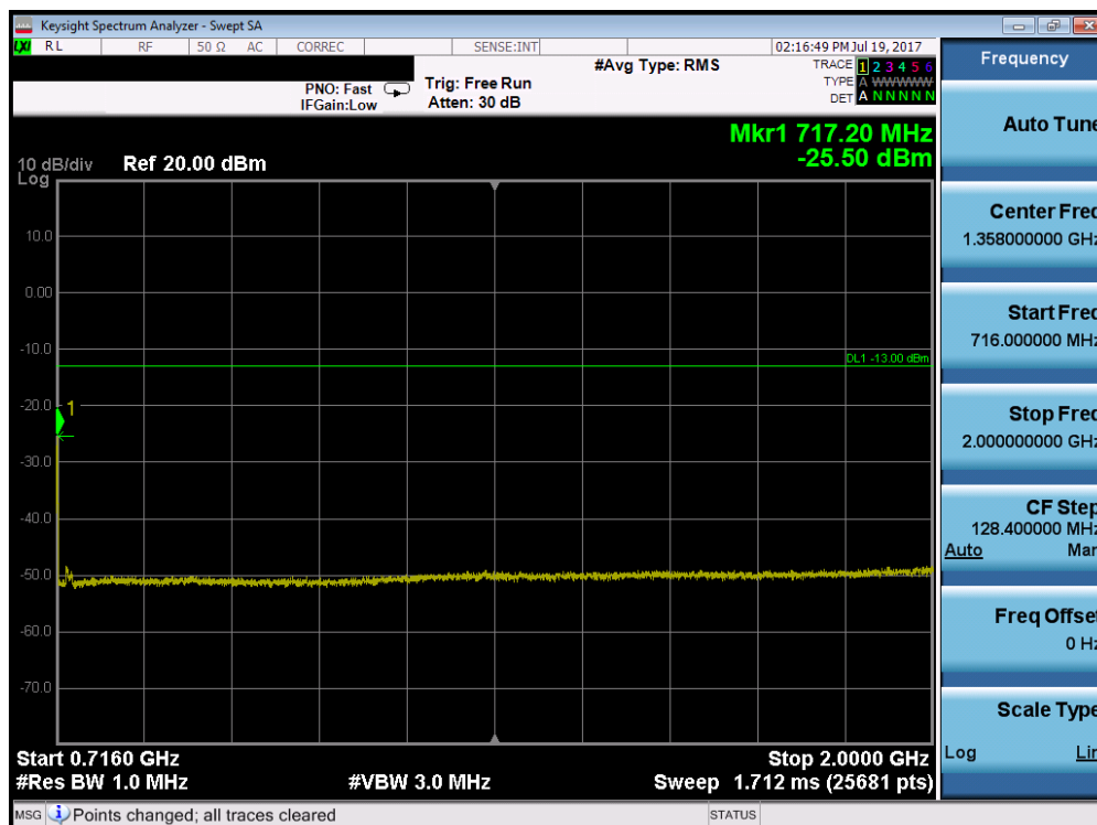
Plot 7-56. Conducted Spurious Plot (Band 12 – 10.0MHz QPSK – RB Size 1, RB Offset 0 – Low Channel)
