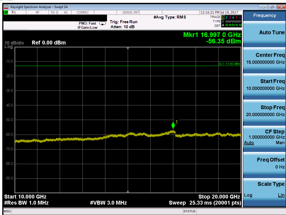
Plot 7-93. Conducted Spurious Plot (Band 2/25 – 10.0MHz QPSK – RB Size 1, RB Offset 0 – Low Channel)
