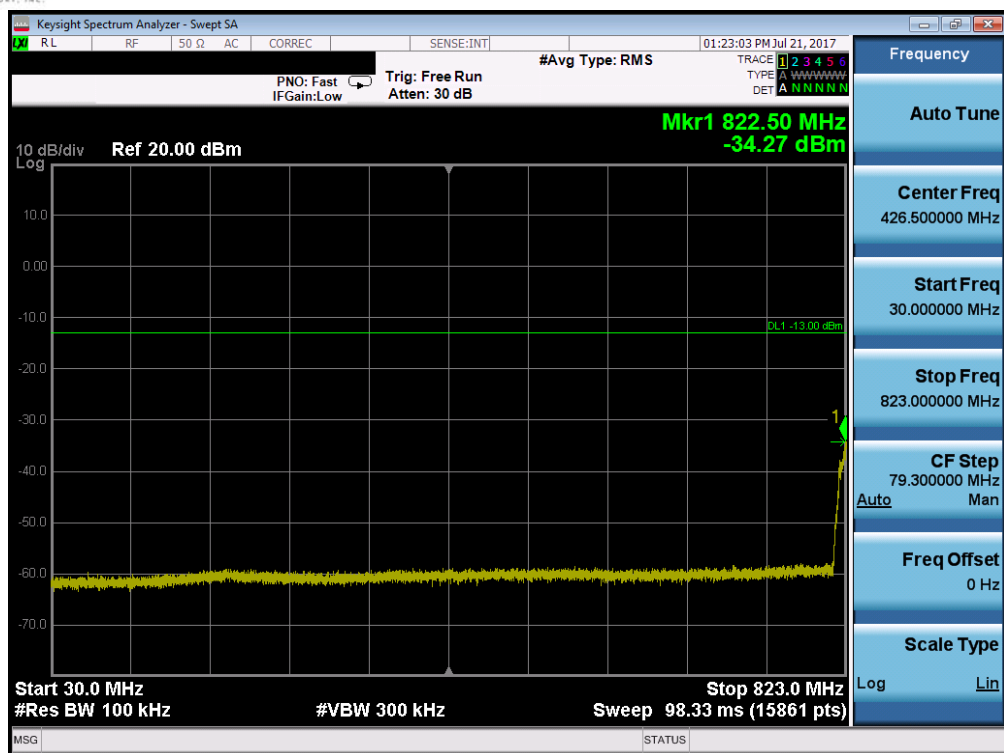
Plot 7-73. Conducted Spurious Plot (Band 5/26 – 10.0MHz QPSK – RB Size 1, RB Offset 0– Low Channel)
