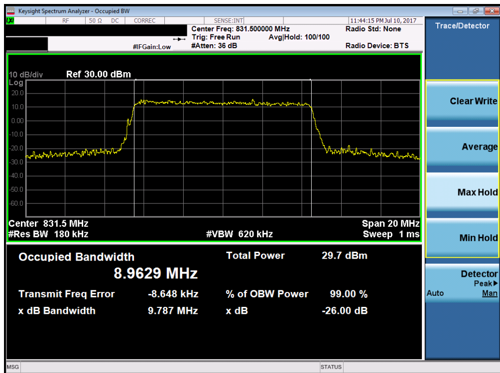
Plot 7-20. Occupied Bandwidth Plot (Band 26/5 – 10.0MHz 16-QAM – RB Size 50)
