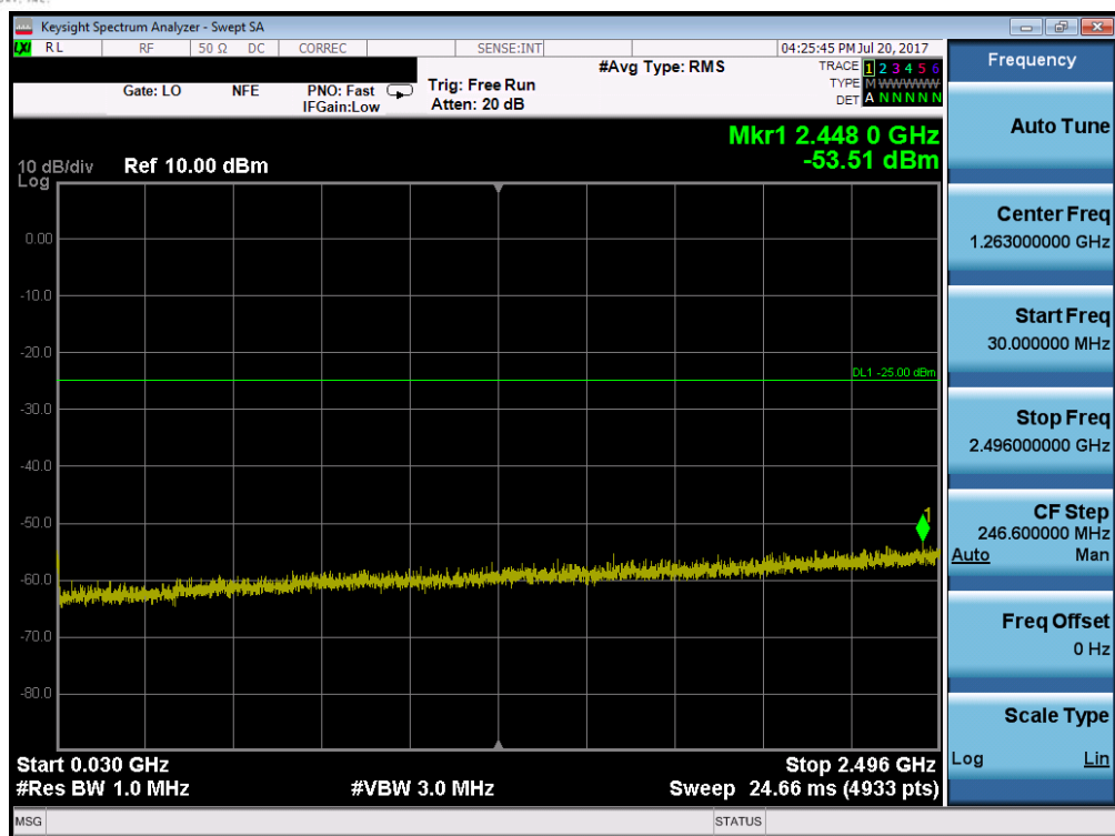
Plot 7-103. Conducted Spurious Plot (Band 41 – 15.0MHz QPSK – RB Size 1, RB Offset 0 – Mid Channel)
