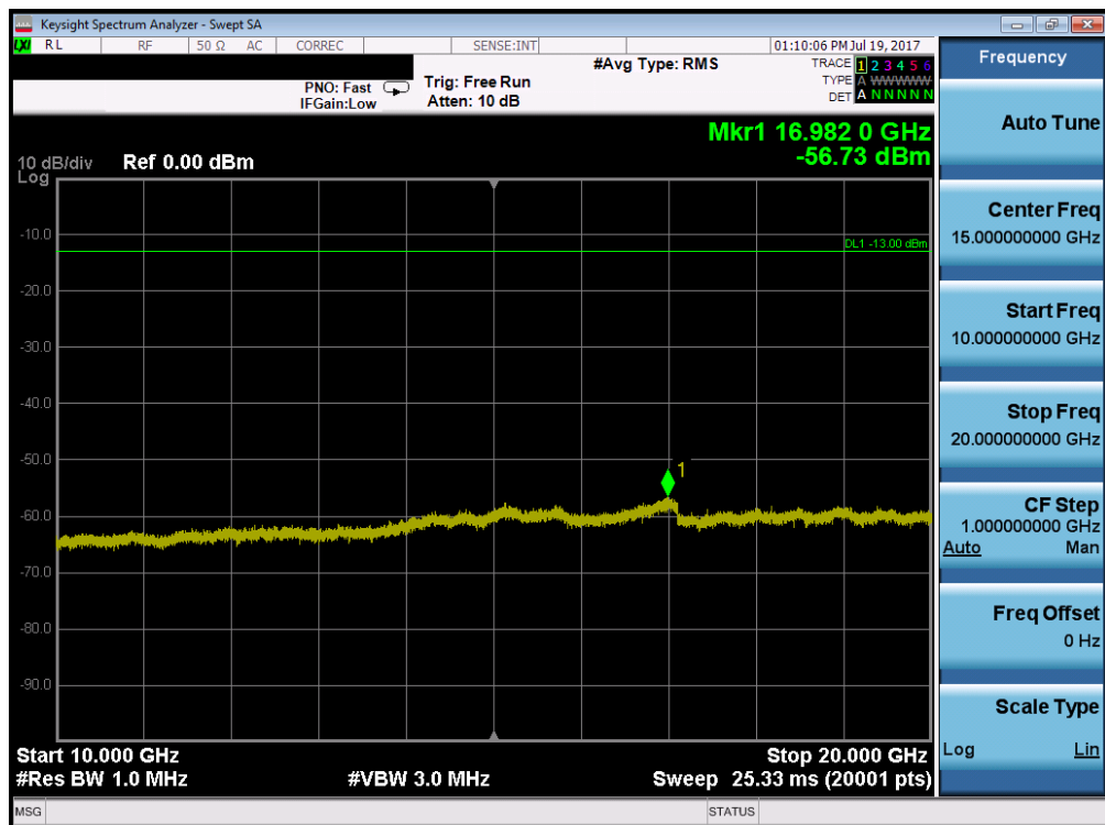
Plot 7-90. Conducted Spurious Plot (Band 4 – 15.0MHz QPSK – RB Size 1, RB Offset 0 – High Channel)
