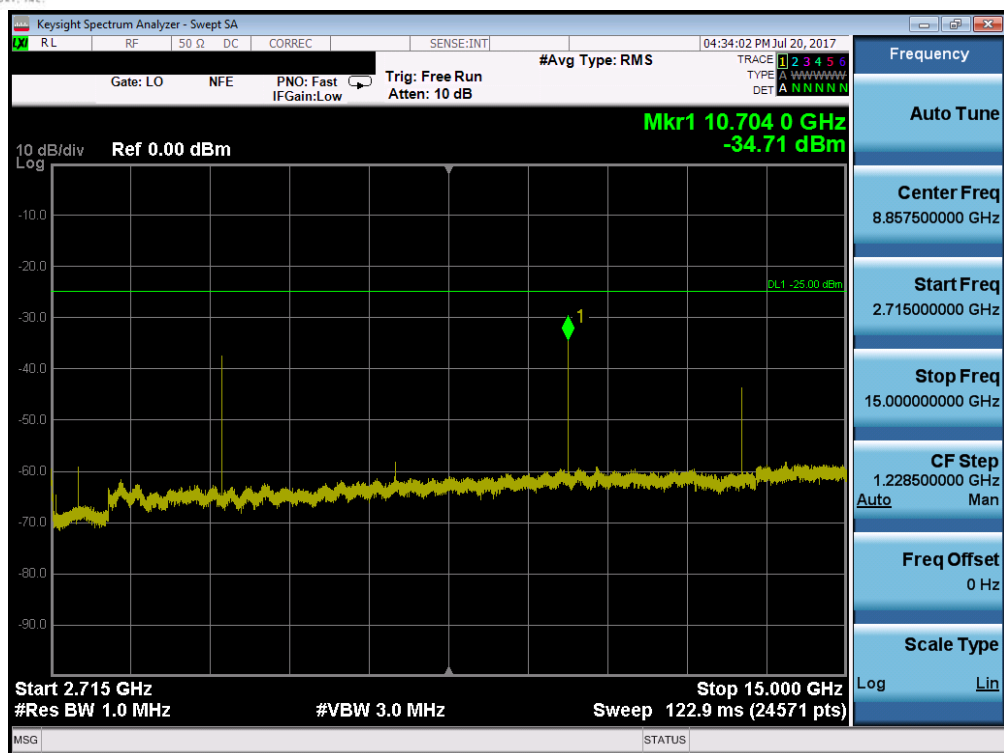
Plot 7-107. Conducted Spurious Plot (Band 41 – 15.0MHz QPSK – RB Size 1, RB Offset 0 – High Channel)
