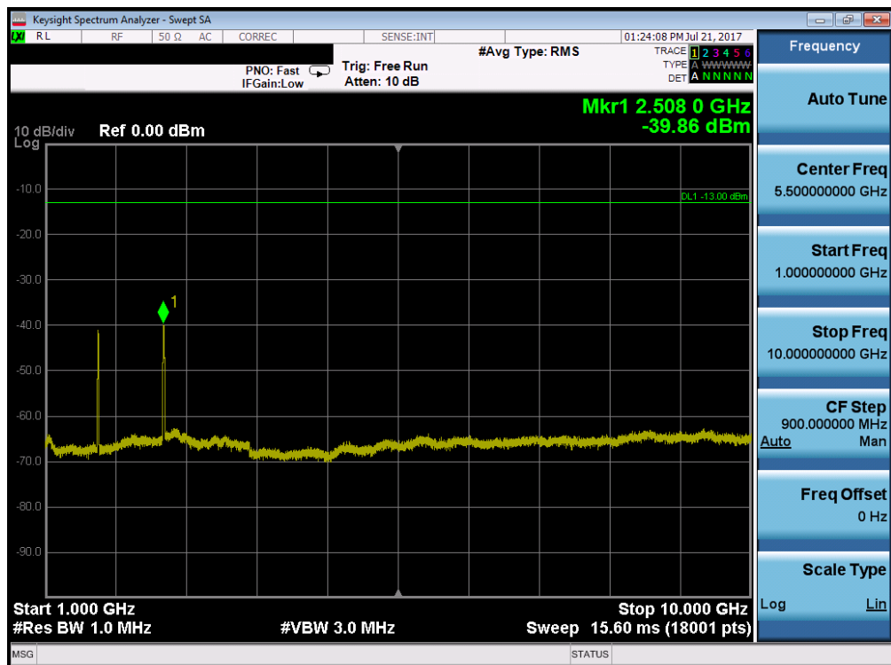
Plot 7-78. Conducted Spurious Plot (Band 5/26 – 10.0MHz QPSK – RB Size 1, RB Offset 0 – Mid Channel)
