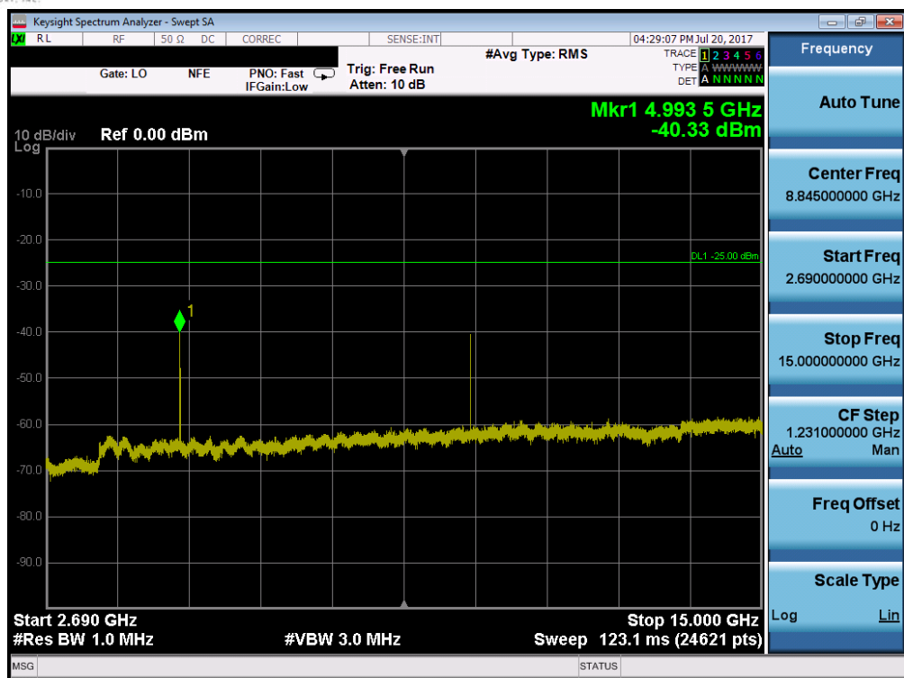
Plot 7-101. Conducted Spurious Plot (Band 41 – 15.0MHz QPSK – RB Size 1, RB Offset 0 – Low Channel)
