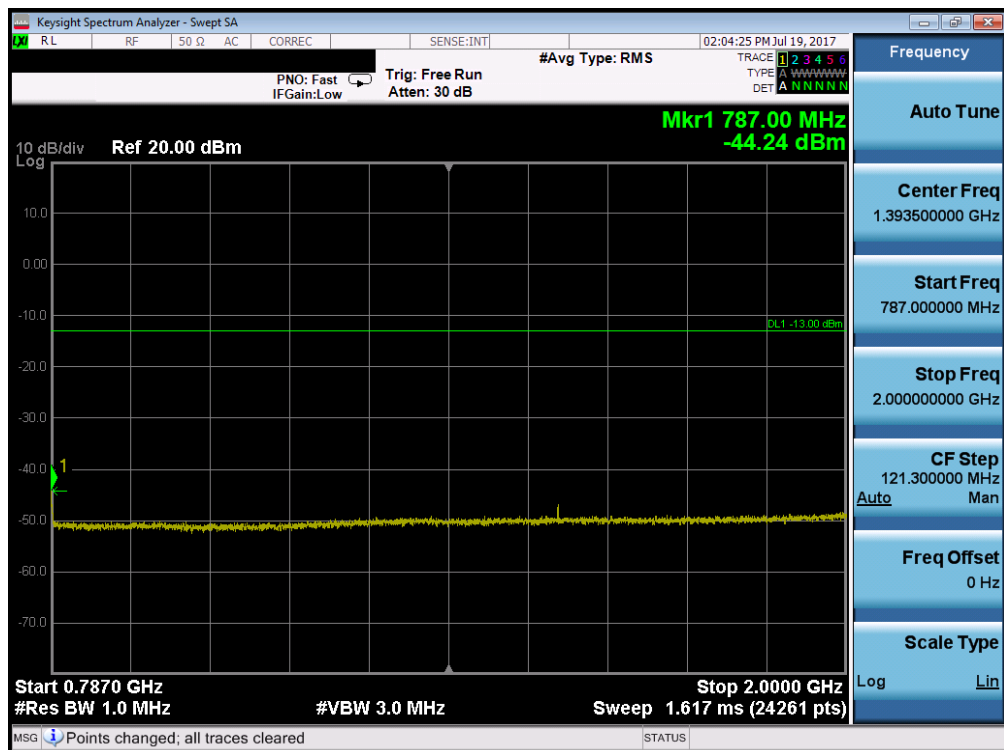
Plot 7-68. Conducted Spurious Plot (Band 13 – 5.0MHz QPSK – RB Size 1, RB Offset 0 – Mid Channel)
