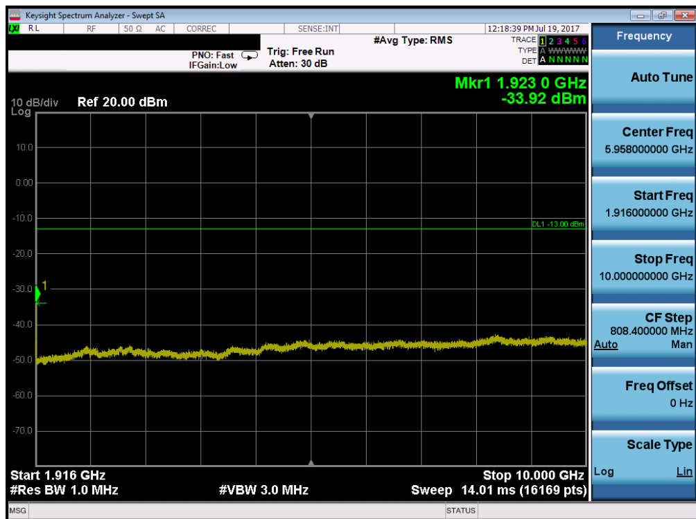
Plot 7-98. Conducted Spurious Plot (Band 2/25 – 10.0MHz QPSK – RB Size 1, RB Offset 0 – High Channel)
