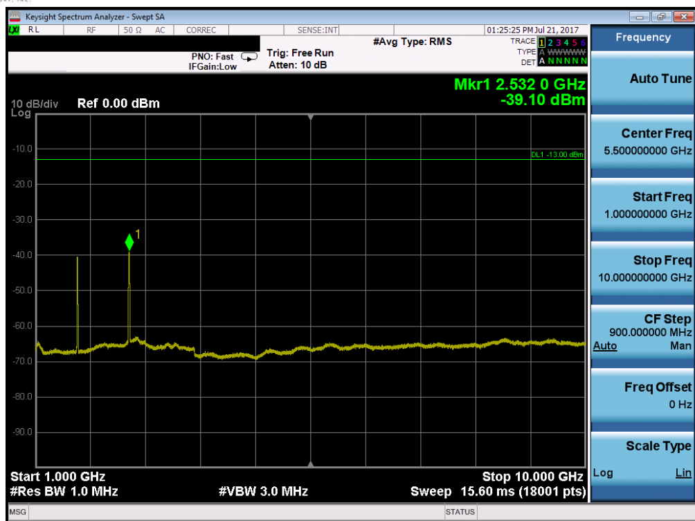
Plot 7-81. Conducted Spurious Plot (Band 5/26 – 10.0MHz QPSK – RB Size 1, RB Offset 0 – High Channel)
