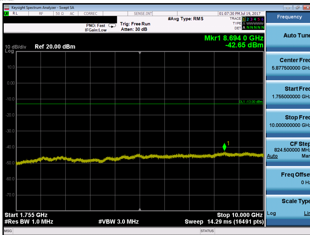
Plot 7-83. Conducted Spurious Plot (Band 4 – 15.0MHz QPSK – RB Size 1, RB Offset 0 – Low Channel)
