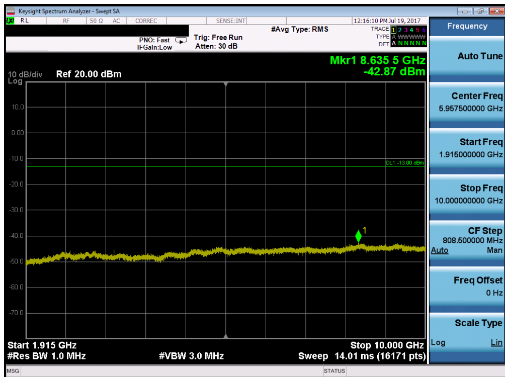
Plot 7-92. Conducted Spurious Plot (Band 2/25 – 10.0MHz QPSK – RB Size 1, RB Offset 0 – Low Channel)
