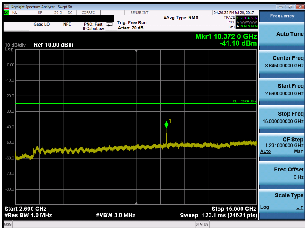
Plot 7-104. Conducted Spurious Plot (Band 41 – 15.0MHz QPSK – RB Size 1, RB Offset 0 – Mid Channel)
