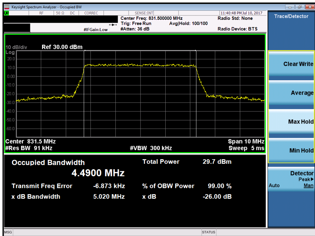
Plot 7-18. Occupied Bandwidth Plot (Band 26/5 – 5.0MHz 16-QAM – RB Size 25)
