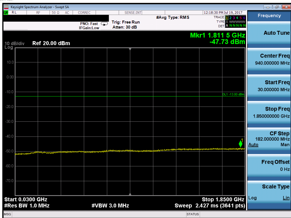
Plot 7-97. Conducted Spurious Plot (Band 2/25 – 10.0MHz QPSK – RB Size 1, RB Offset 0 – High Channel)
