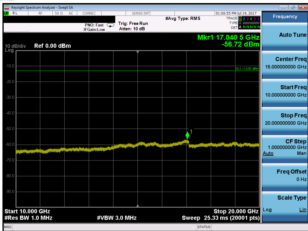
Plot 7-87. Conducted Spurious Plot (Band 4 – 15.0MHz QPSK – RB Size 1, RB Offset 0 – Mid Channel)
