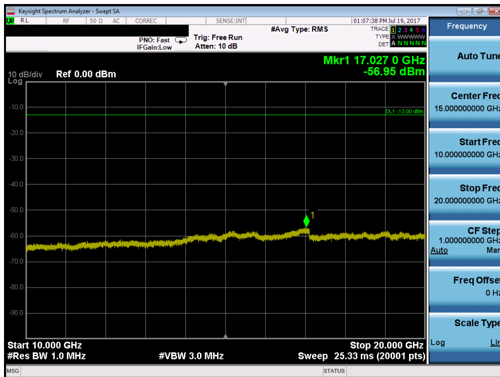
Plot 7-84. Conducted Spurious Plot (Band 4 – 15.0MHz QPSK – RB Size 1, RB Offset 0 – Low Channel)
