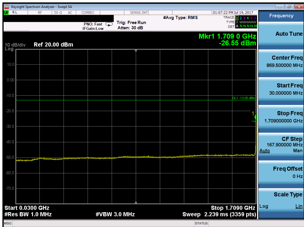
Plot 7-82. Conducted Spurious Plot (Band 4 – 15.0MHz QPSK – RB Size 1, RB Offset 0 – Low Channel)
