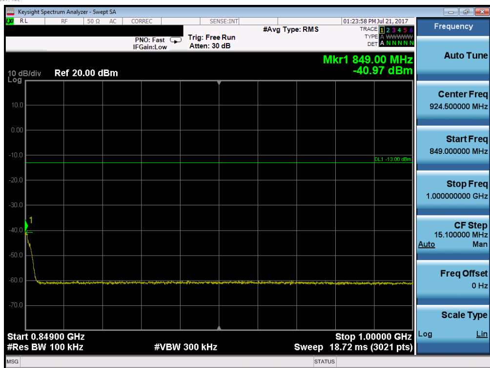
Plot 7-77. Conducted Spurious Plot (Band 5/26 – 10.0MHz QPSK – RB Size 1, RB Offset 0 – Mid Channel)
