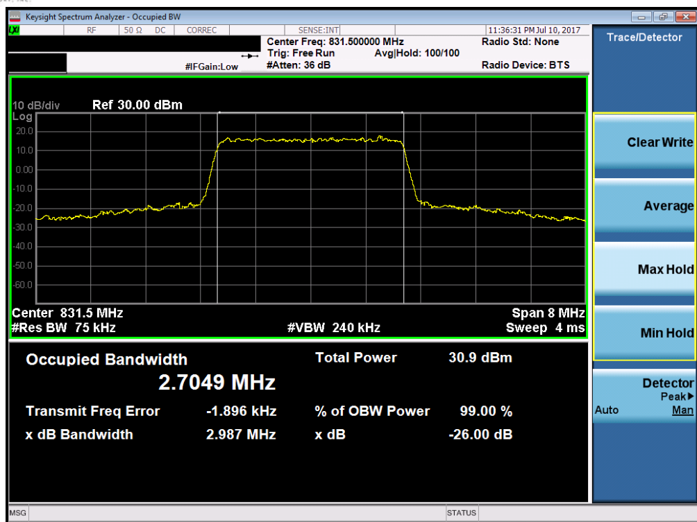
Plot 7-15. Occupied Bandwidth Plot (Band 26/5 – 3.0MHz QPSK – RB Size 15)
