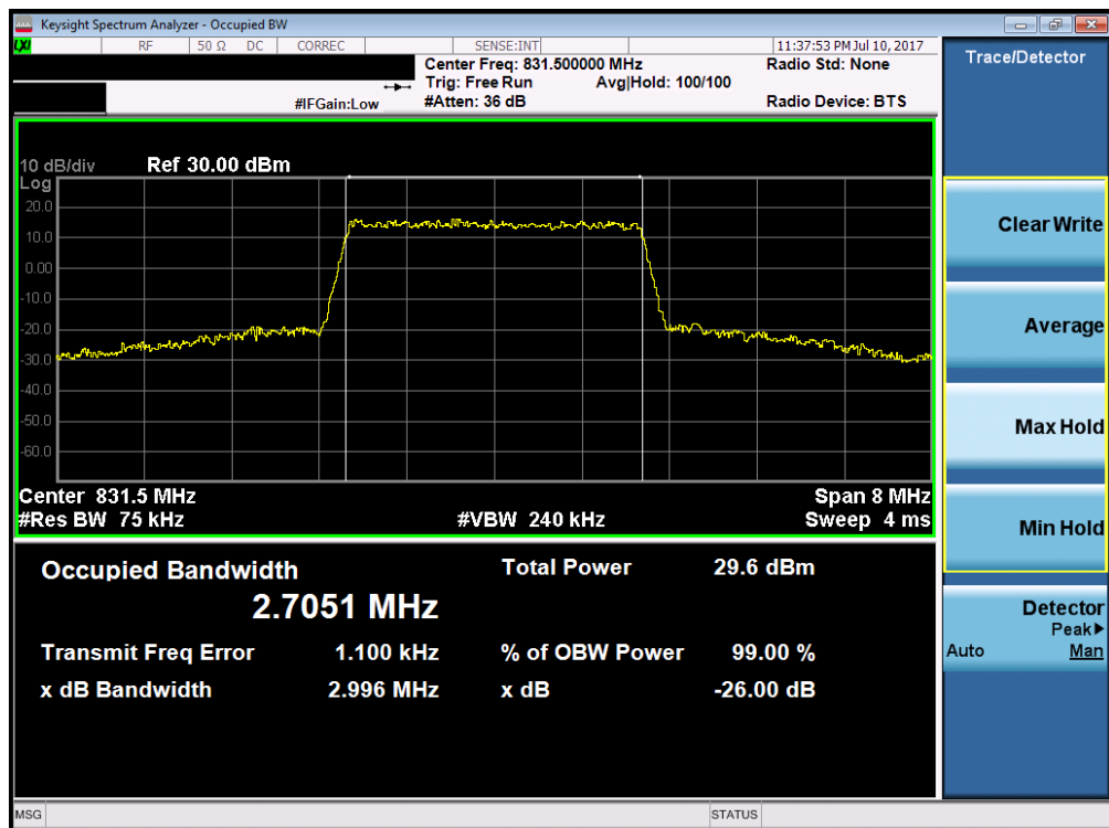
Plot 7-16. Occupied Bandwidth Plot (Band 26/5 – 3.0MHz 16-QAM – RB Size 15)
