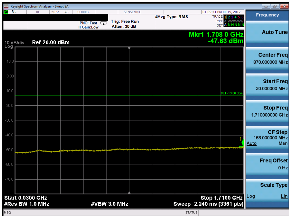
Plot 7-88. Conducted Spurious Plot (Band 4 – 15.0MHz QPSK – RB Size 1, RB Offset 0 – High Channel)
