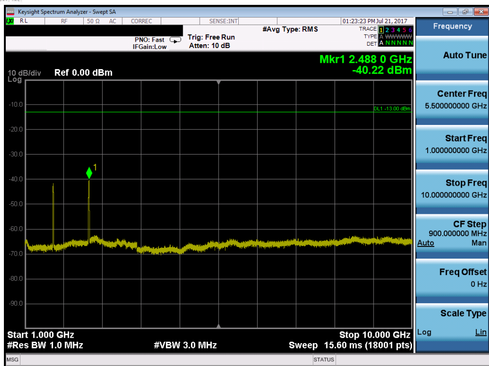
Plot 7-75. Conducted Spurious Plot (Band 5/26 – 10.0MHz QPSK – RB Size 1, RB Offset 0 – Low Channel)
