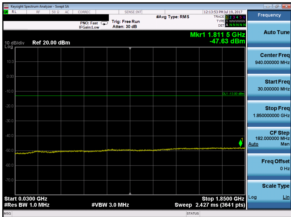
Plot 7-94. Conducted Spurious Plot (Band 2/25 – 10.0MHz QPSK – RB Size 1, RB Offset 0 – Mid Channel)
