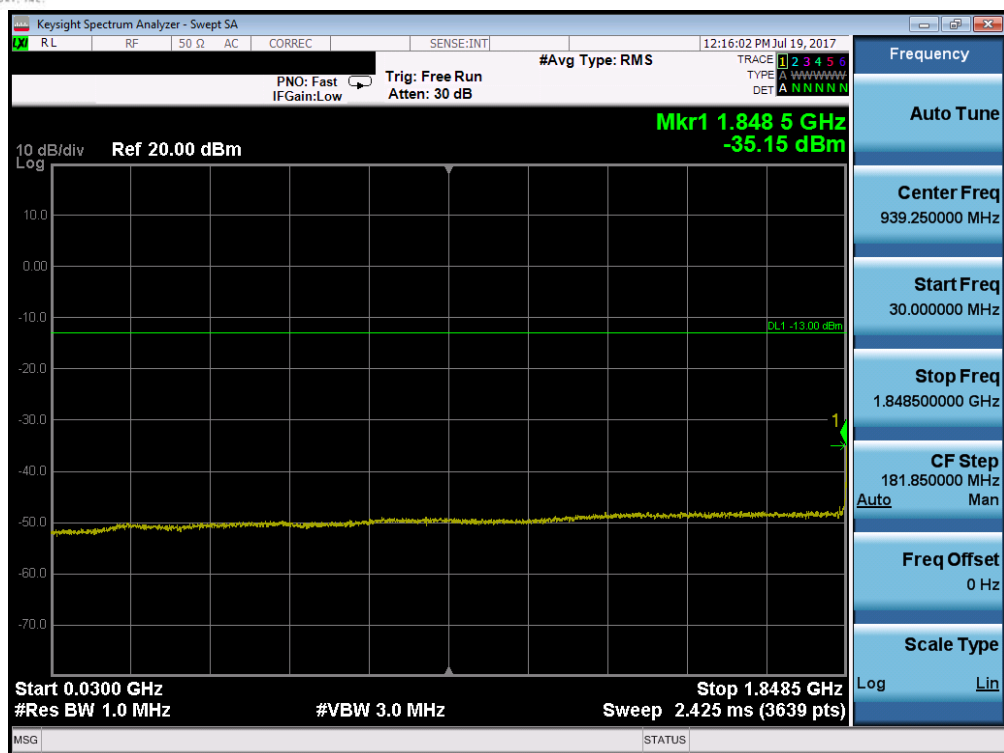
Plot 7-91. Conducted Spurious Plot (Band 2/25 – 10.0MHz QPSK – RB Size 1, RB Offset 0– Low Channel)
