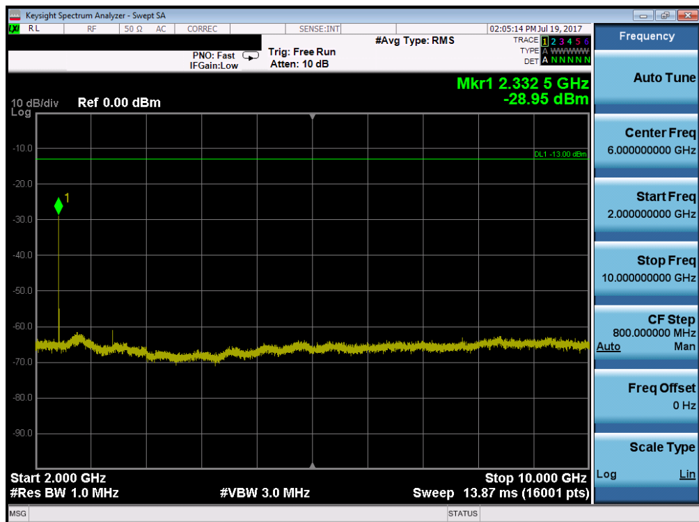
Plot 7-66. Conducted Spurious Plot (Band 13 – 5.0MHz QPSK – RB Size 1, RB Offset 0 – Low Channel)
