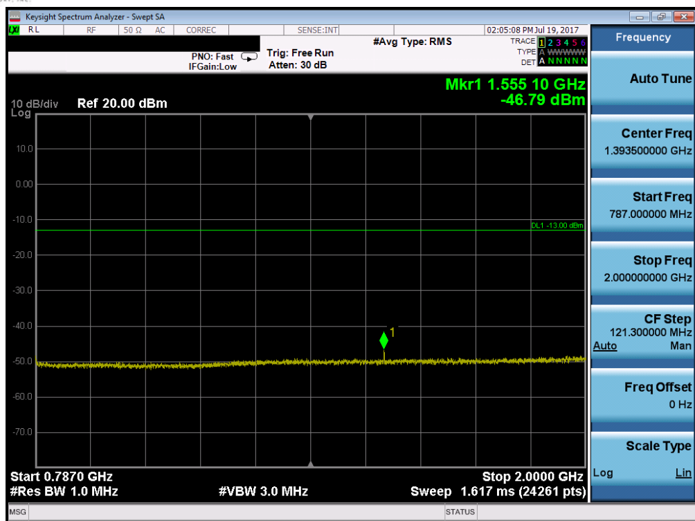
Plot 7-65. Conducted Spurious Plot (Band 13 – 5.0MHz QPSK – RB Size 1, RB Offset 0 – Low Channel)
