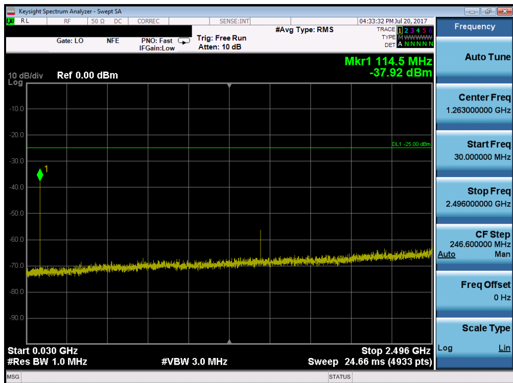
Plot 7-106. Conducted Spurious Plot (Band 41 – 15.0MHz QPSK – RB Size 1, RB Offset 0 – High Channel)
