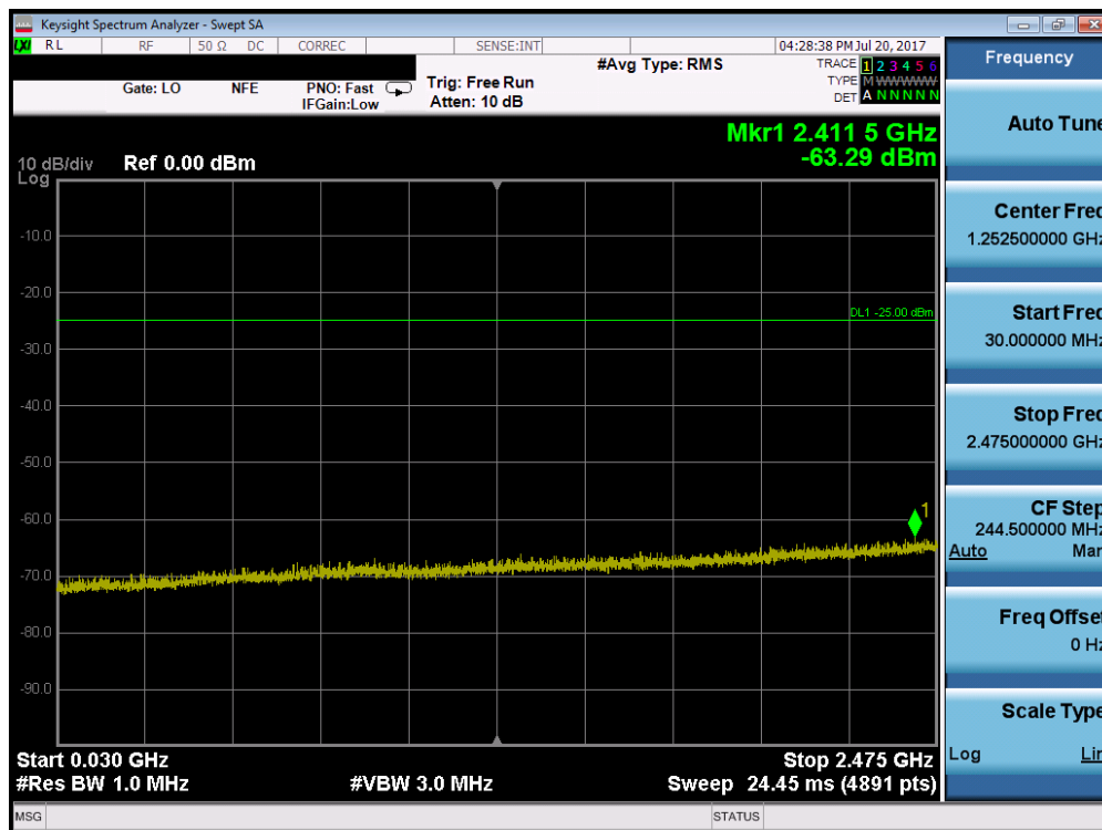
Plot 7-100. Conducted Spurious Plot (Band 41 – 15.0MHz QPSK – RB Size 1, RB Offset 0 – Low Channel)
