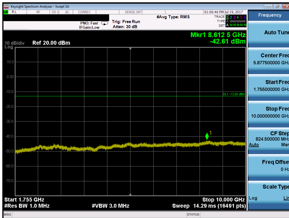
Plot 7-86. Conducted Spurious Plot (Band 4 – 15.0MHz QPSK – RB Size 1, RB Offset 0 – Mid Channel)
