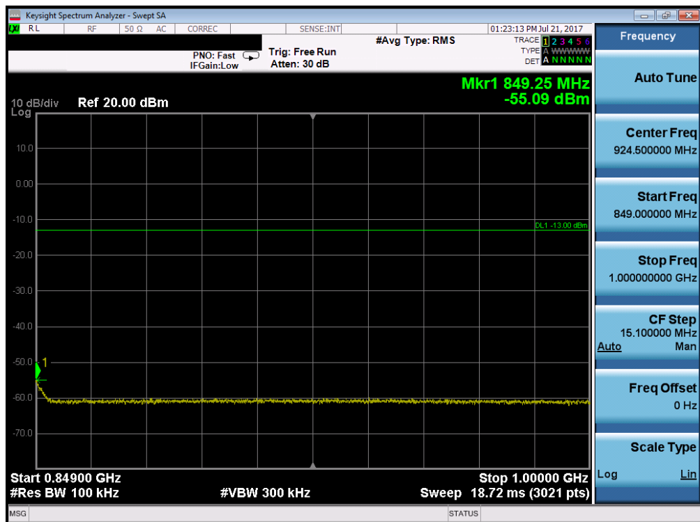
Plot 7-74. Conducted Spurious Plot (Band 5/26 – 10.0MHz QPSK – RB Size 1, RB Offset 0 – Low Channel)
