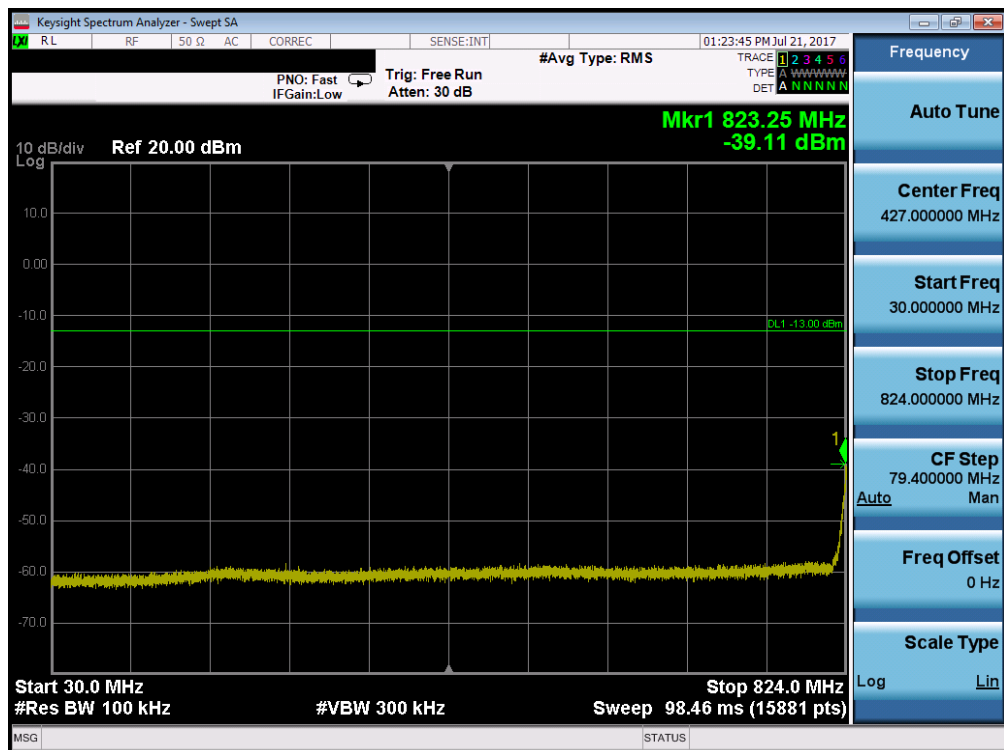
Plot 7-76. Conducted Spurious Plot (Band 5/26 – 10.0MHz QPSK – RB Size 1, RB Offset 0 – Mid Channel)
