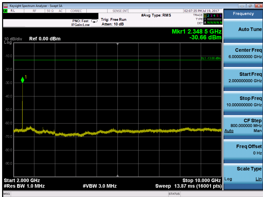
Plot 7-72. Conducted Spurious Plot (Band 13 – 5.0MHz QPSK – RB Size 1, RB Offset 0 – High Channel)
