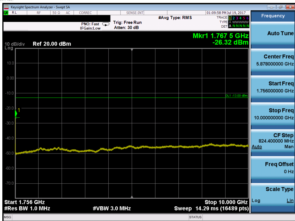
Plot 7-89. Conducted Spurious Plot (Band 4 – 15.0MHz QPSK – RB Size 1, RB Offset 0 – High Channel)
