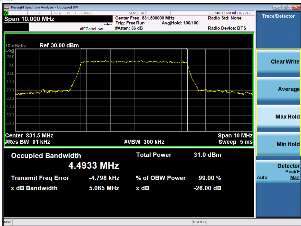
Plot 7-17. Occupied Bandwidth Plot (Band 26/5 – 5.0MHz QPSK – RB Size 25)
