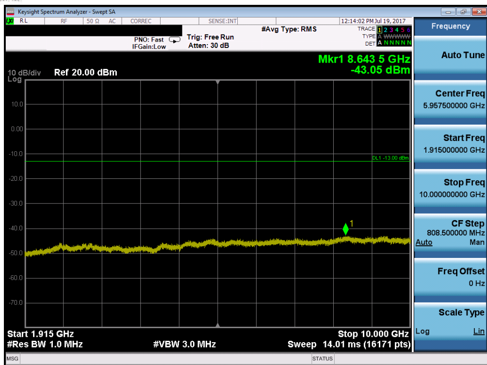
Plot 7-95. Conducted Spurious Plot (Band 2/25 – 10.0MHz QPSK – RB Size 1, RB Offset 0 – Mid Channel)
