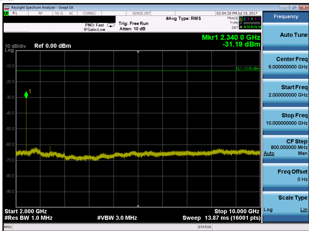
Plot 7-69. Conducted Spurious Plot (Band 13 – 5.0MHz QPSK – RB Size 1, RB Offset 0 – Mid Channel)
