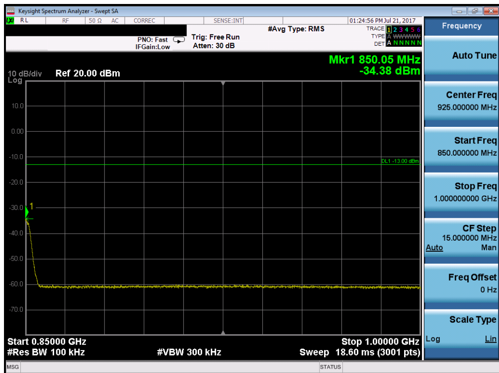
Plot 7-80. Conducted Spurious Plot (Band 5/26 – 10.0MHz QPSK – RB Size 1, RB Offset 0 – High Channel)
