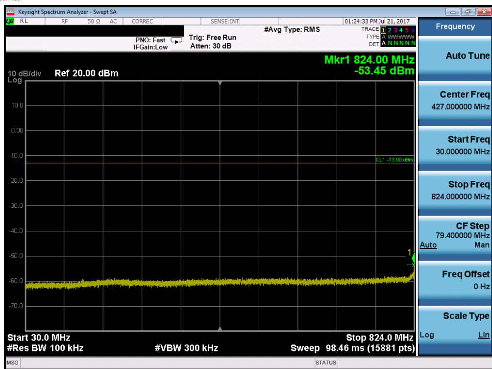
Plot 7-79. Conducted Spurious Plot (Band 5/26 – 10.0MHz QPSK – RB Size 1, RB Offset 0 – High Channel)
