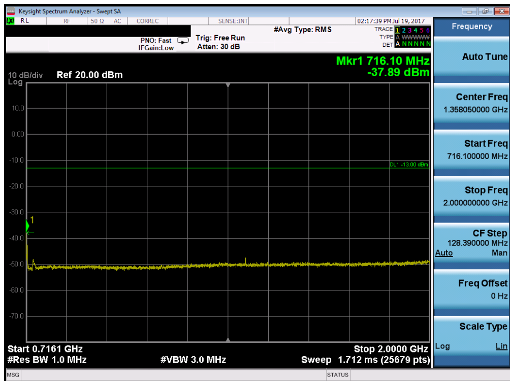
Plot 7-62. Conducted Spurious Plot (Band 12 – 10.0MHz QPSK – RB Size 1, RB Offset 0 – High Channel)
