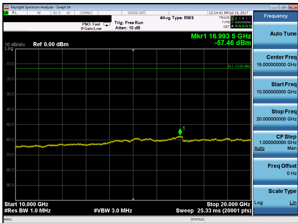
Plot 7-96. Conducted Spurious Plot (Band 2/25 – 10.0MHz QPSK – RB Size 1, RB Offset 0 – Mid Channel)
