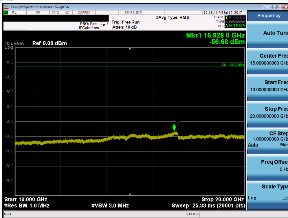
Plot 7-99. Conducted Spurious Plot (Band 2/25 – 10.0MHz QPSK – RB Size 1, RB Offset 0 – High Channel)
