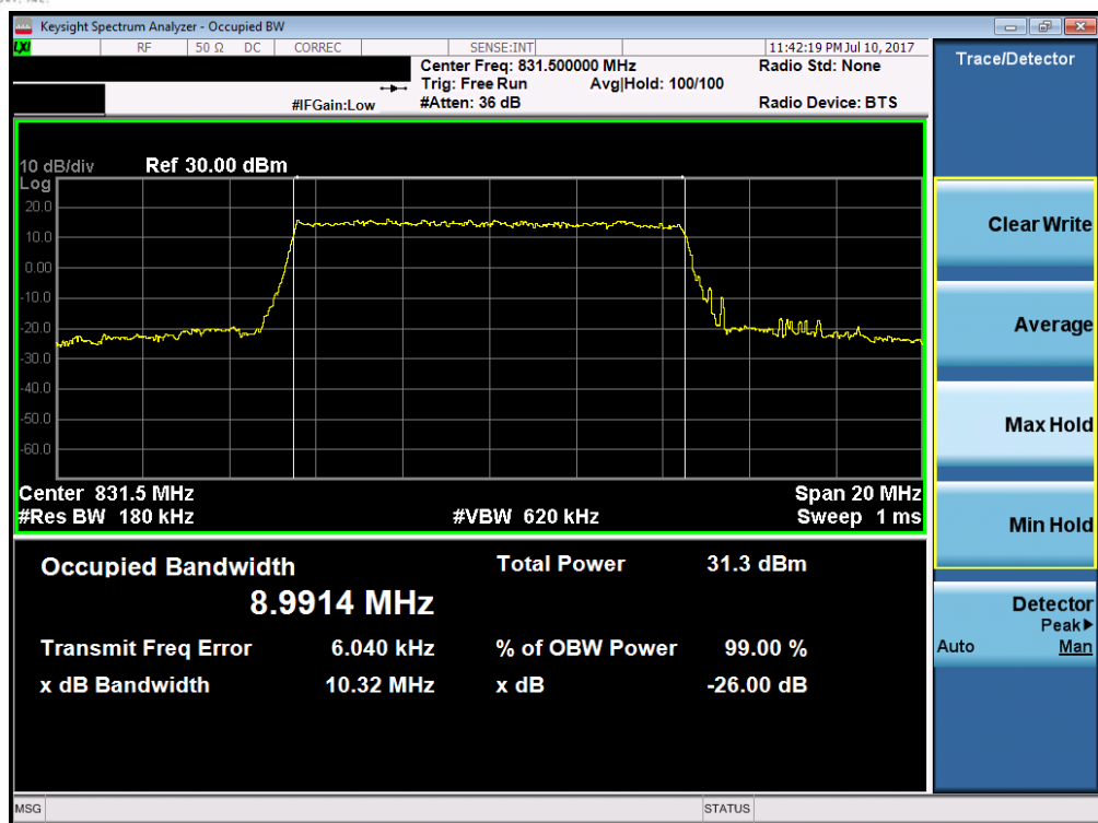
Plot 7-19. Occupied Bandwidth Plot (Band 26/5 – 10.0MHz QPSK – RB Size 50)
