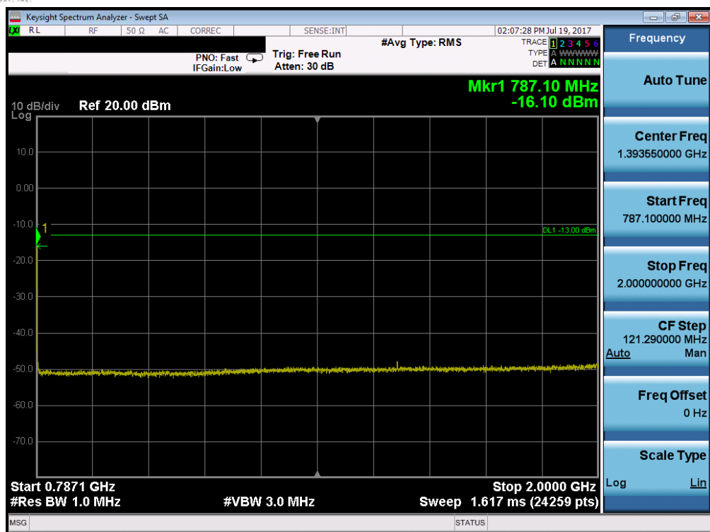
Plot 7-71. Conducted Spurious Plot (Band 13 – 5.0MHz QPSK – RB Size 1, RB Offset 0 – High Channel)
