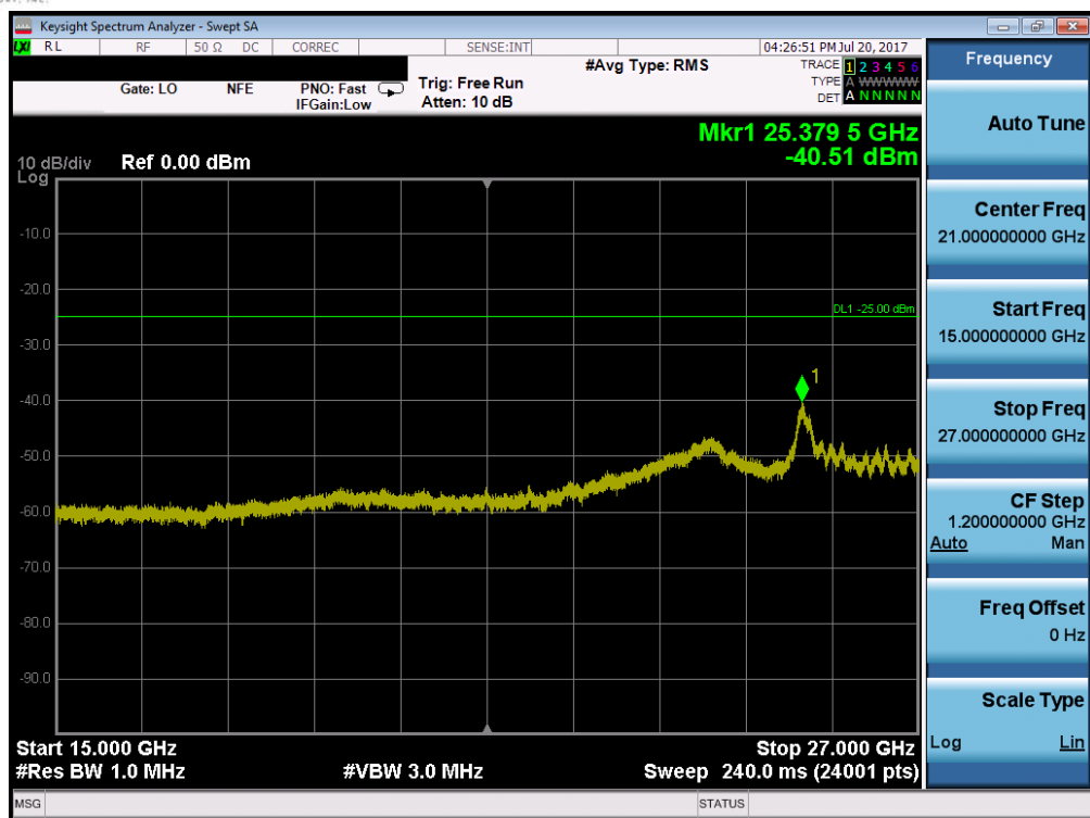
Plot 7-105. Conducted Spurious Plot (Band 41 – 15.0MHz QPSK – RB Size 1, RB Offset 0 – Mid Channel)
