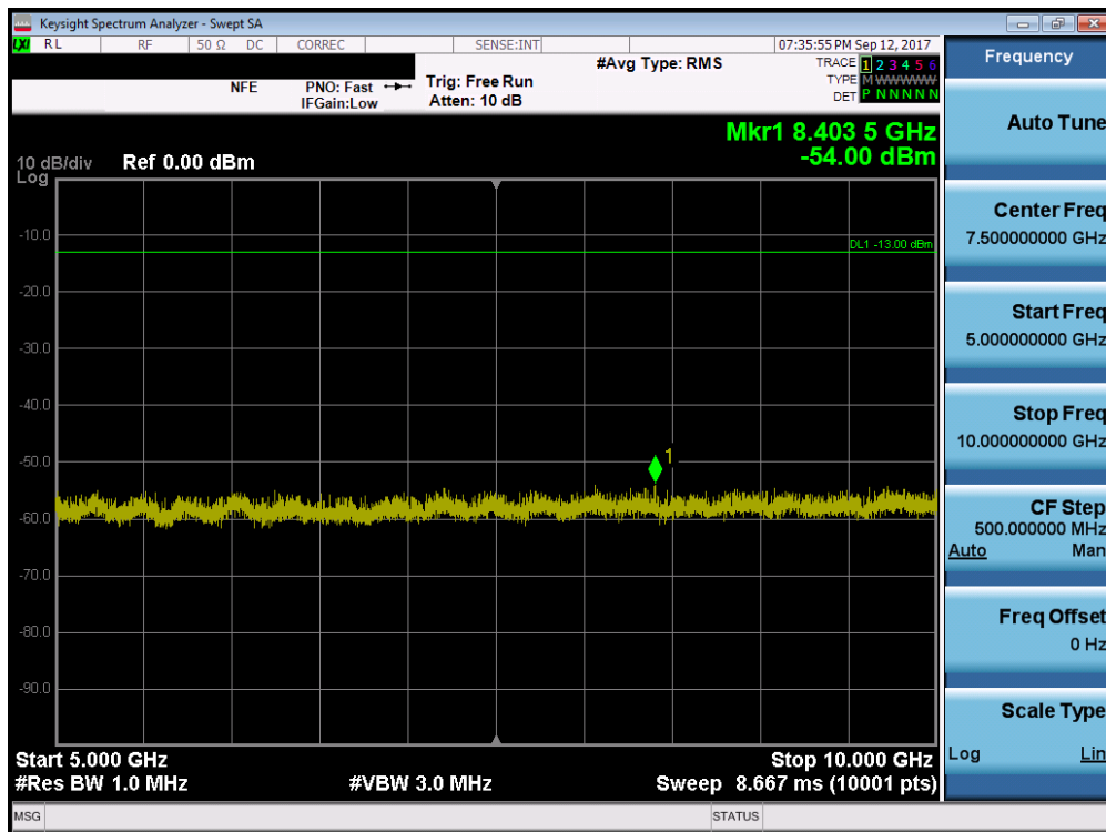
Plot 7-14. CDMA BC10 Conducted Spurious Plot (Ch. 476)
