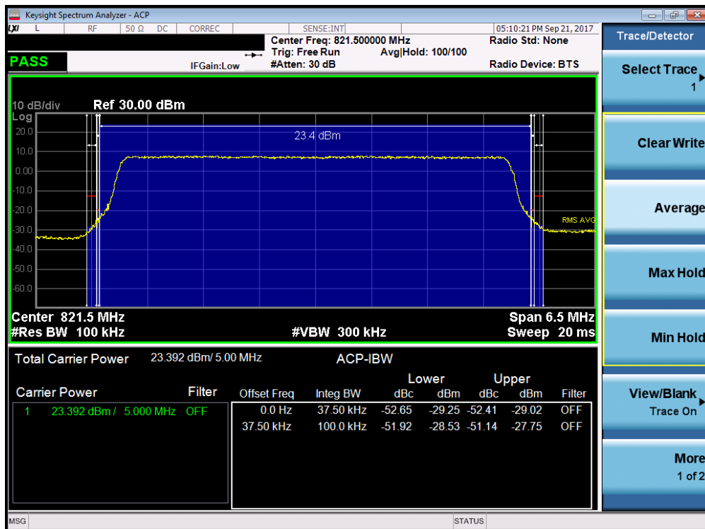
Plot 7-28. LTE Band 26 Channel Edge Plot (5MHz QPSK – RB Size 25 – High Channel)
