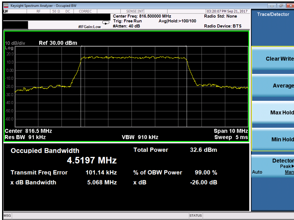
Plot 7-7. LTE Band 26 Occupied Bandwidth Plot (5MHz QPSK – RB Size 25– Low Channel)
