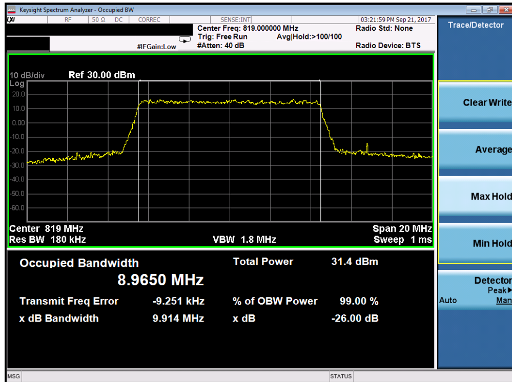
Plot 7-10. LTE Band 26 Occupied Bandwidth Plot (10MHz 16-QAM – RB Size 50)
