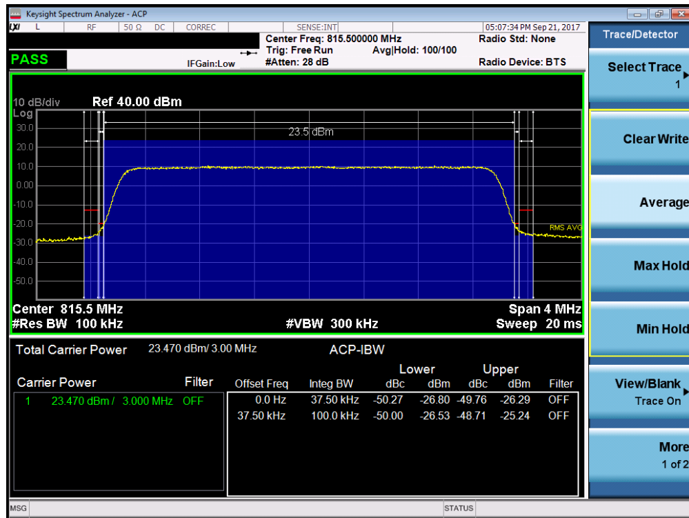
Plot 7-25. LTE Band 26 Channel Edge Plot (3MHz QPSK – RB Size 15– Low Channel)
