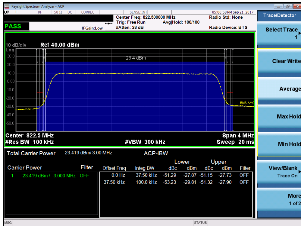
Plot 7-26. LTE Band 26 Channel Edge Plot (3MHz QPSK – RB Size 15 – High Channel)
