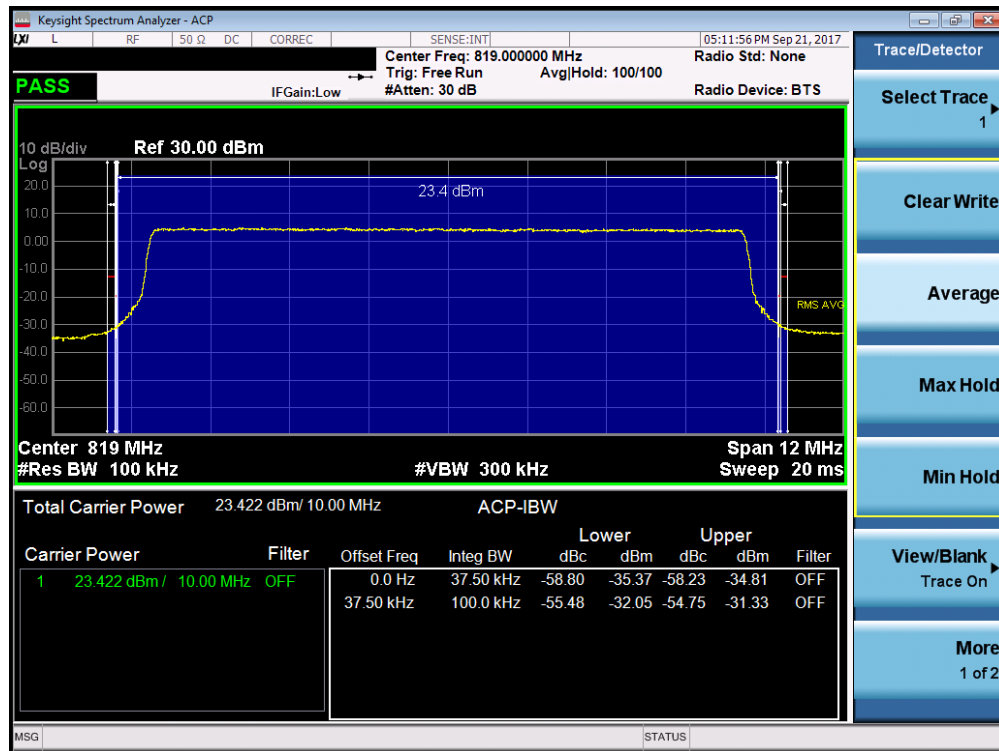
Plot 7-29. LTE Band 26 Channel Edge Plot (10MHz QPSK – RB Size 50)
