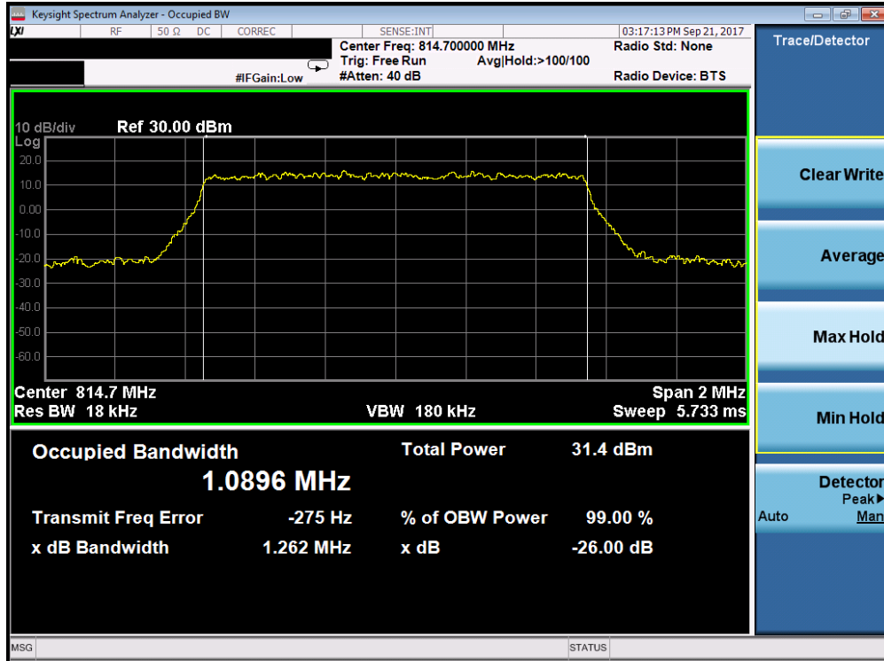
Plot 7-3. LTE Band 26 Occupied Bandwidth Plot (1.4MHz QPSK – RB Size 6– Low Channel)
