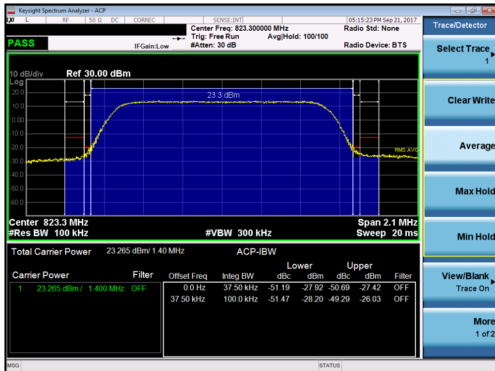
Plot 7-24. LTE Band 26 Channel Edge Plot (1.4MHz QPSK – RB Size 6 – High Channel)
