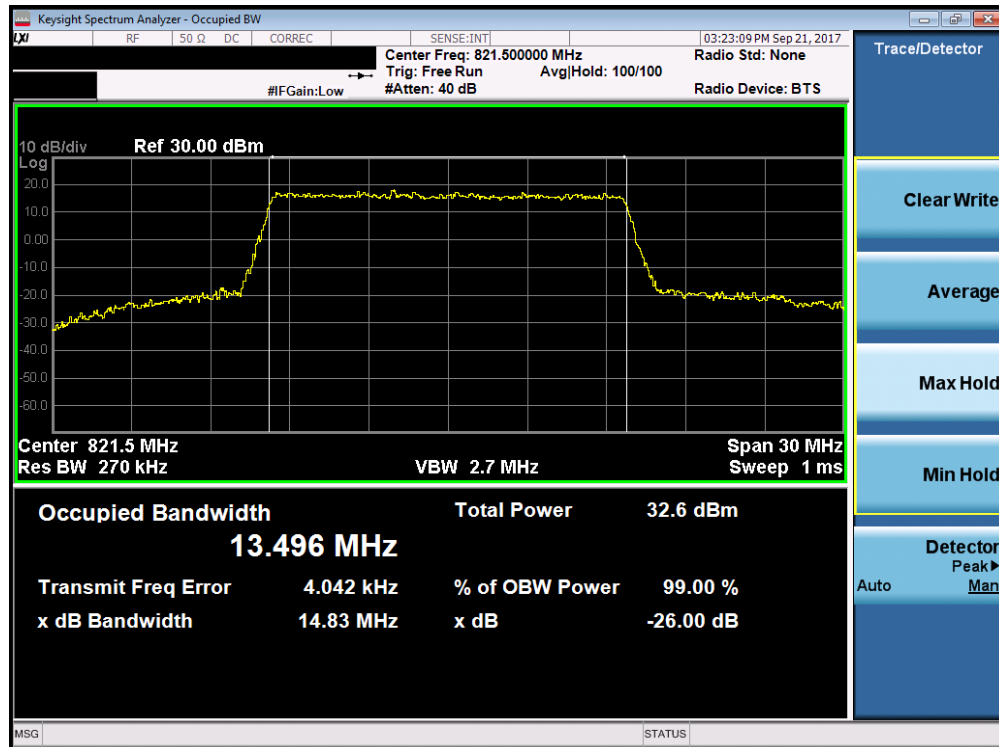
Plot 7-11. LTE Band 26 Occupied Bandwidth Plot (15MHz QPSK – RB Size 75)
