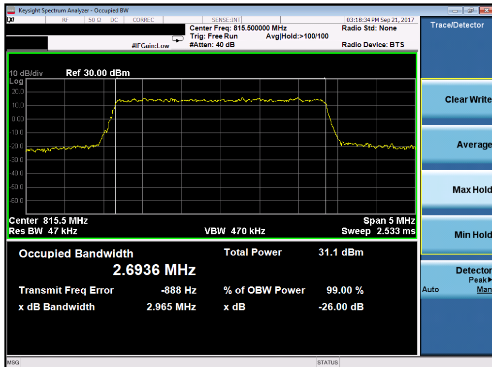
Plot 7-6. LTE Band 26 Occupied Bandwidth Plot (3MHz 16-QAM – RB Size 15– Low Channel)
