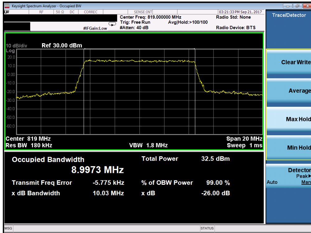
Plot 7-9. LTE Band 26 Occupied Bandwidth Plot (10MHz QPSK – RB Size 50)
