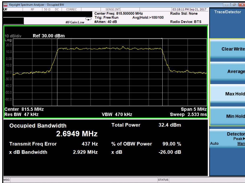
Plot 7-5. LTE Band 26 Occupied Bandwidth Plot (3MHz QPSK – RB Size 15– Low Channel)
