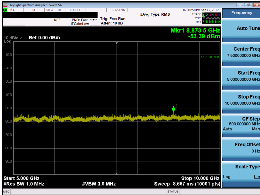
Plot 7-16. CDMA BC10 Conducted Spurious Plot (Ch. 684)
