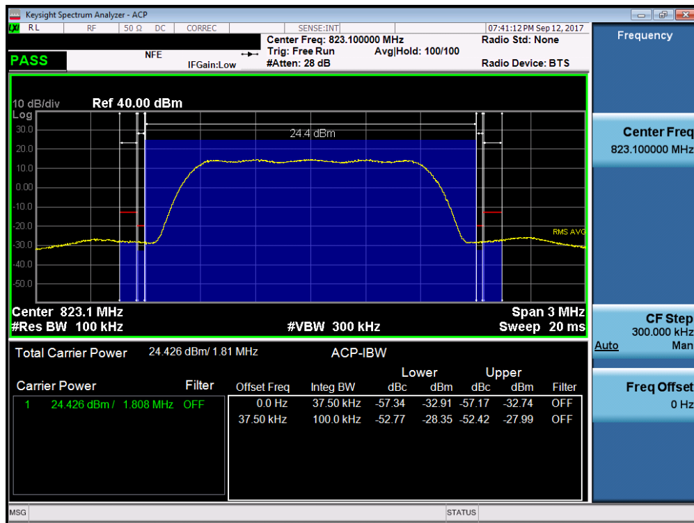
Plot 7-22. CDMA BC10 Channel Edge Plot (Ch. 684)
