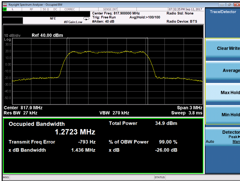
Plot 7-1. CDMA BC10 Occupied Bandwidth Plot (Ch. 476)
