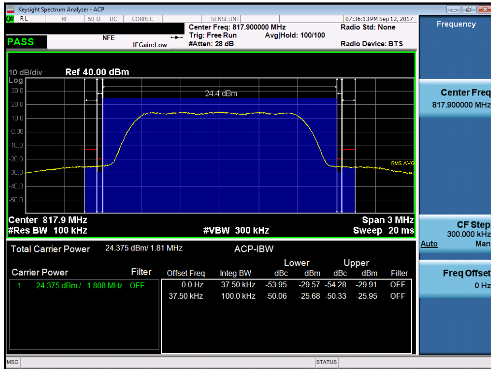
Plot 7-21. CDMA BC10 Channel Edge Plot (Ch. 476)
