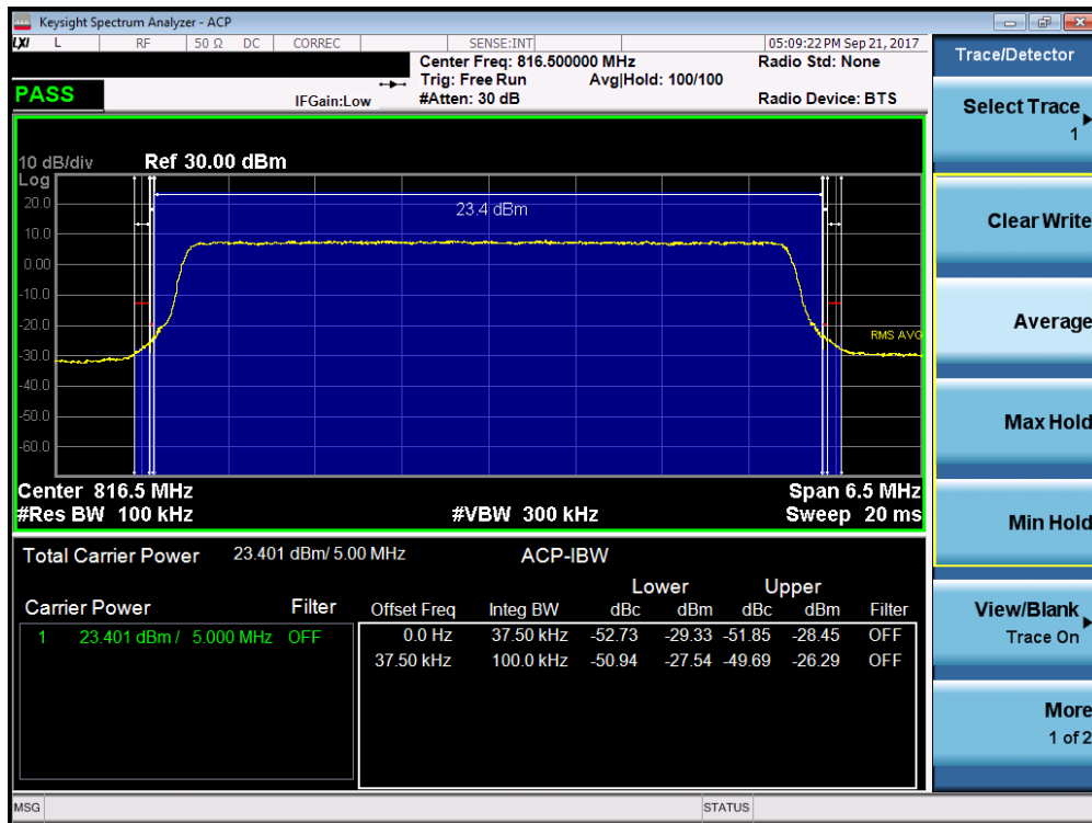
Plot 7-27. LTE Band 26 Channel Edge Plot (5MHz QPSK – RB Size 25– Low Channel)
