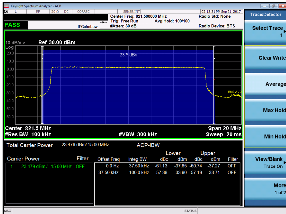
Plot 7-30. LTE Band 26 Channel Edge Plot (15MHz QPSK – RB Size 75)
