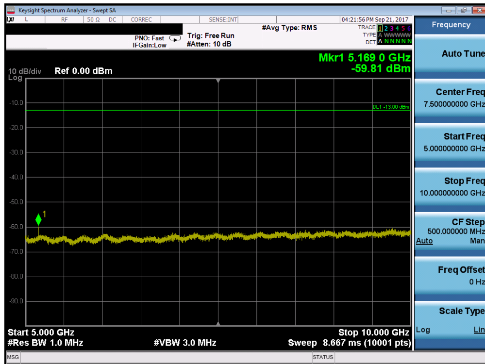
Plot 7-18. LTE Band 26 Conducted Spurious Plot (5MHz QPSK – RB Size 1, RB Offset 0 – Low Channel)
