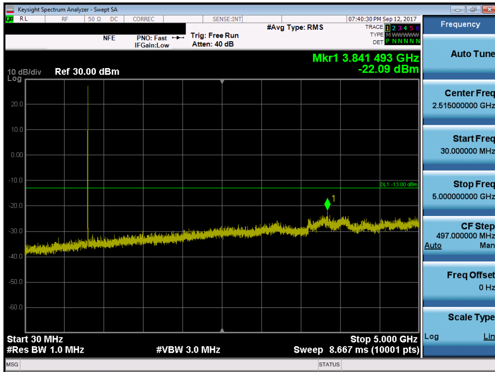
Plot 7-15. CDMA BC10 Conducted Spurious Plot (Ch. 684)
