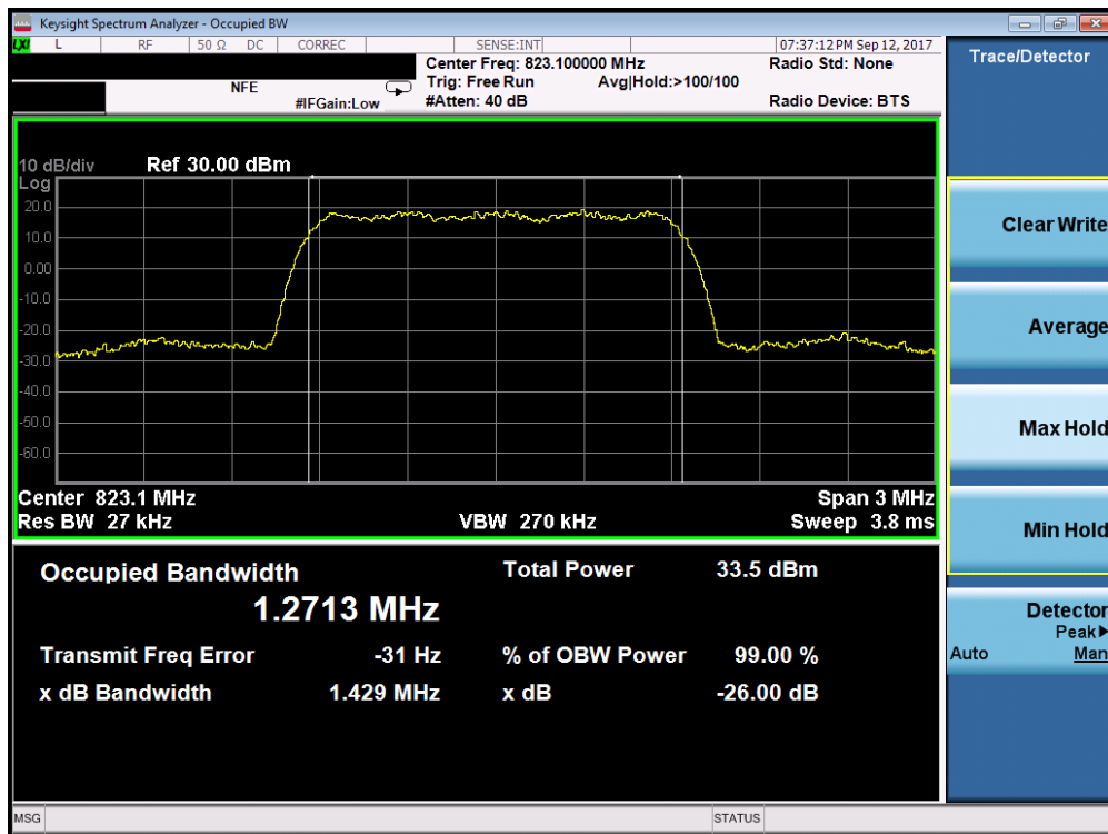
Plot 7-2. CDMA BC10 Occupied Bandwidth Plot (Ch. 684)
