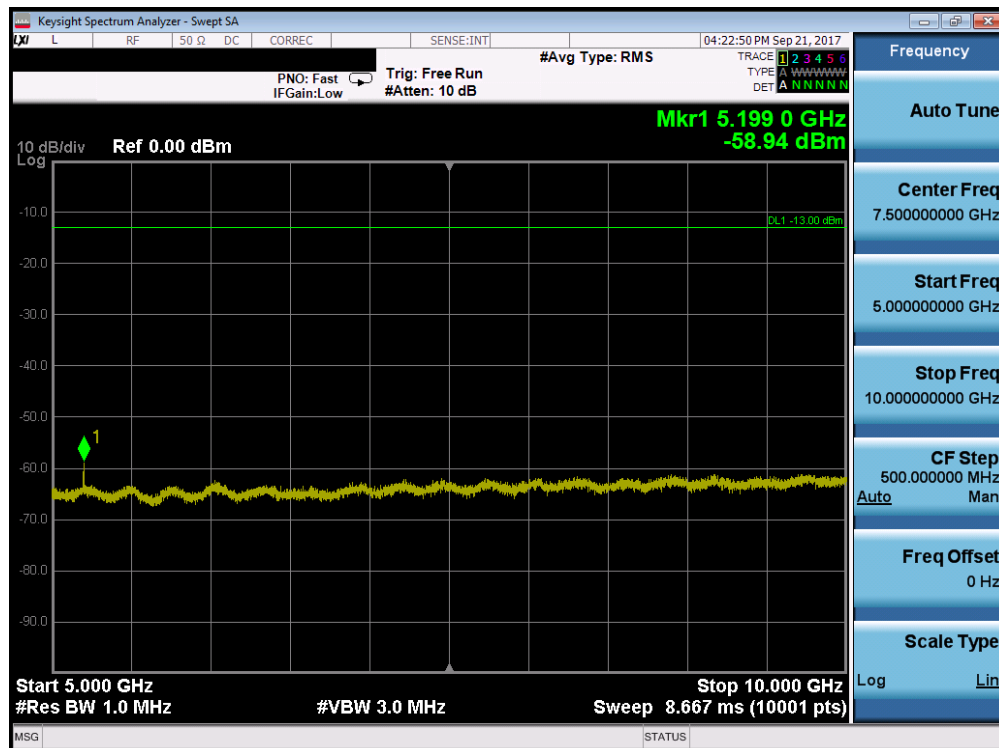
Plot 7-20. LTE Band 26 Conducted Spurious Plot (5MHz QPSK – RB Size 1, RB Offset 0 – High Channel)
