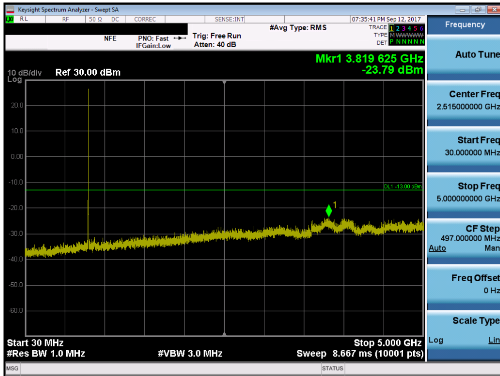
Plot 7-13. CDMA BC10 Conducted Spurious Plot (Ch. 476)
