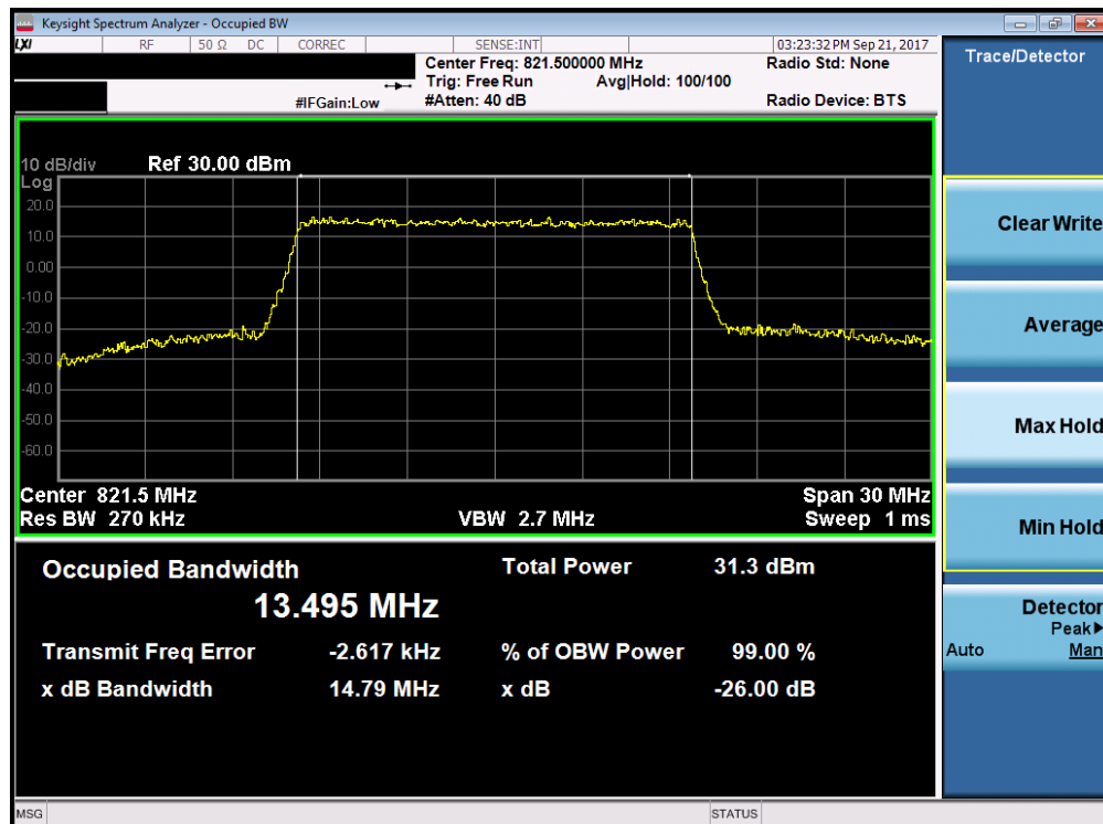
Plot 7-12. LTE Band 26 Occupied Bandwidth Plot (15MHz 16-QAM – RB Size 75)
