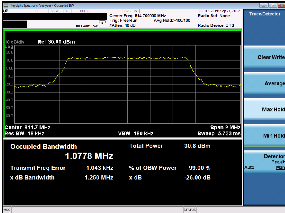
Plot 7-4. LTE Band 26 Occupied Bandwidth Plot (1.4MHz 16-QAM – RB Size 6– Low Channel)
