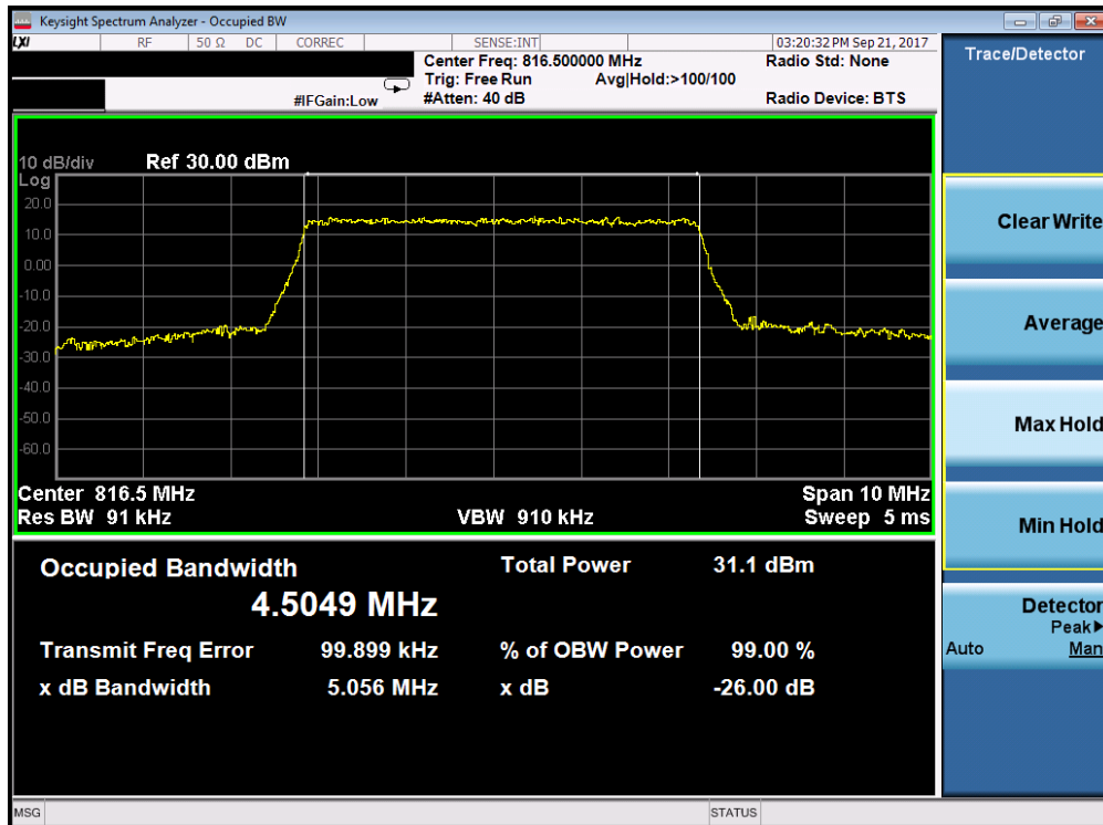
Plot 7-8. LTE Band 26 Occupied Bandwidth Plot (5MHz 16-QAM – RB Size 25– Low Channel)
