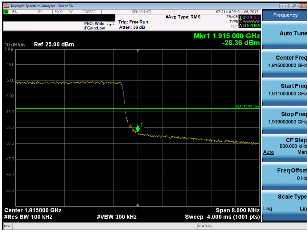
Plot 7-164. Upper Band Edge Plot (Band 25 - 10.0MHz QPSK - Full RB Configuration)
