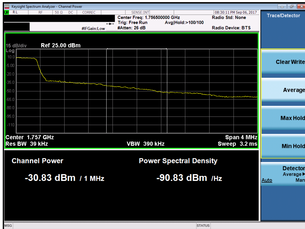
Plot 7-129. . Upper Extended Band Edge Plot (Band 4 – 1.4MHz QPSK - Full RB Configuration)
