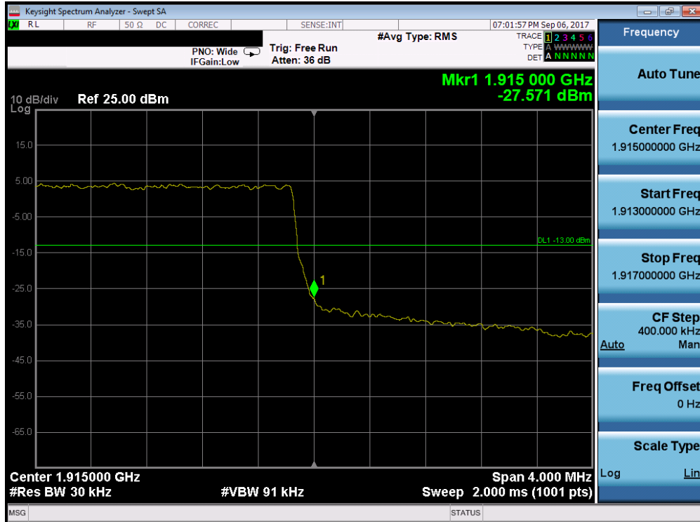
Plot 7-156. Upper Band Edge Plot (Band 25 - 3.0MHz QPSK - Full RB Configuration)
