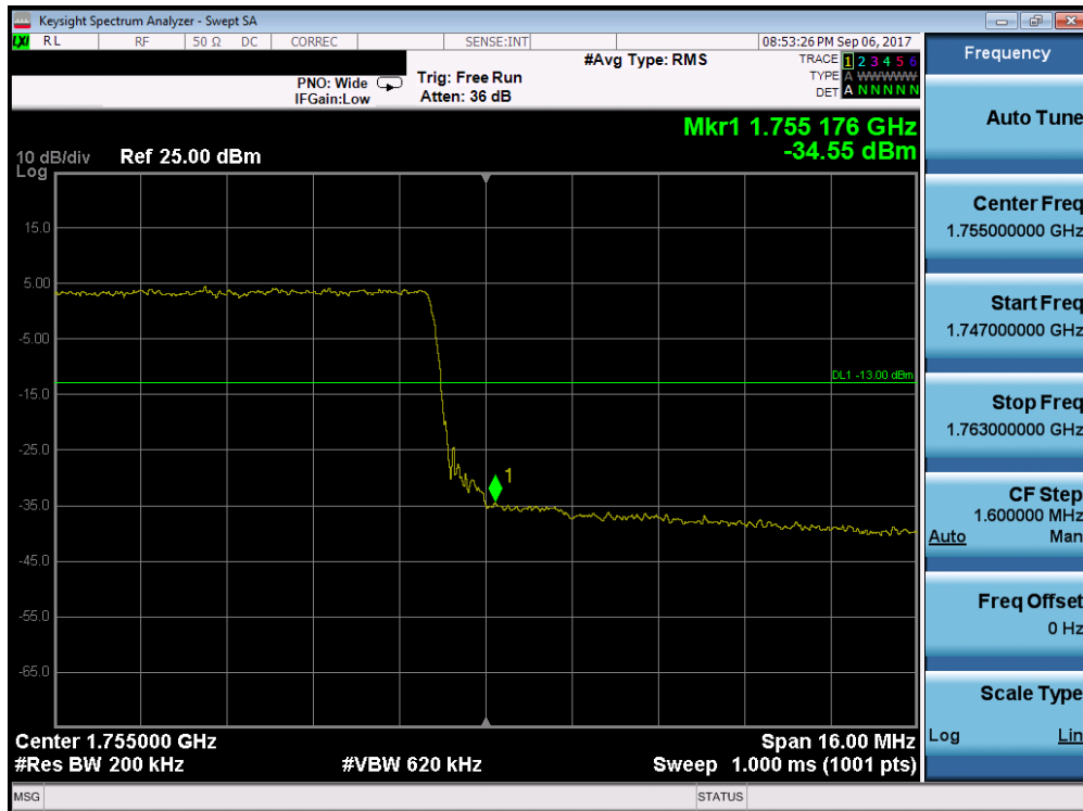
Plot 7-148. Upper Band Edge Plot (Band 4 - 20.0MHz QPSK - Full RB Configuration)
