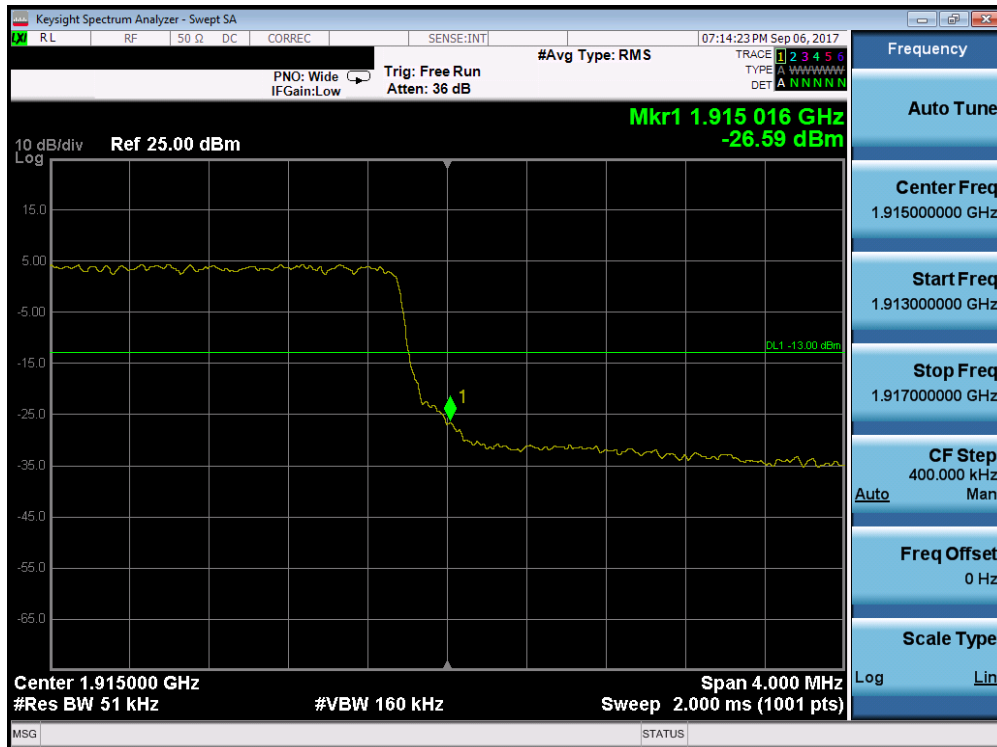
Plot 7-160. Upper Band Edge Plot (Band 25 - 5.0MHz QPSK - Full RB Configuration)
