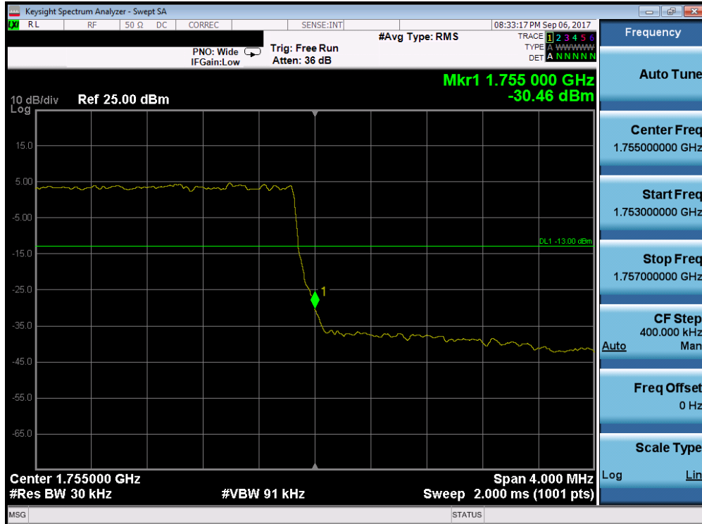
Plot 7-132. Upper Band Edge Plot (Band 4 - 3.0MHz QPSK - Full RB Configuration)
