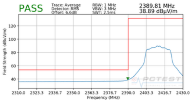
Plot 7-13. Radiated Restricted Lower Band Edge Measurement SISO ANT2 (Average)
