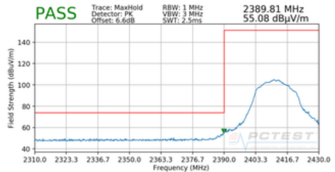
Plot 7-18. Radiated Restricted Lower Band Edge Measurement CDD (Peak)
