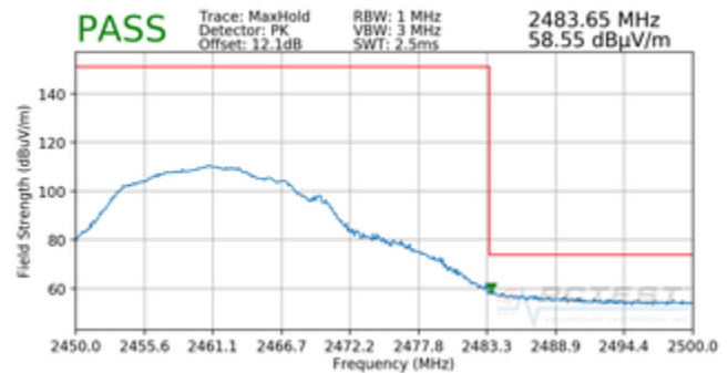
Plot 7-20. Radiated Restricted Upper Band Edge Measurement CDD (Peak)
