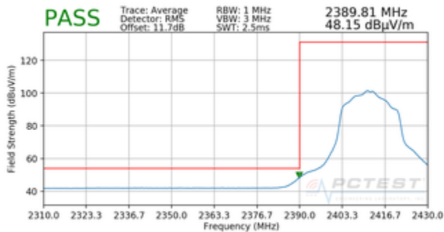
Plot 7-17. Radiated Restricted Lower Band Edge Measurement CDD (Average)
