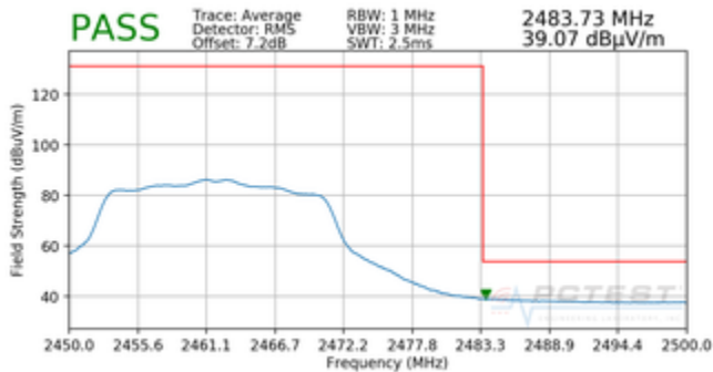
Plot 7-15. Radiated Restricted Upper Band Edge Measurement SISO ANT2 (Average)
