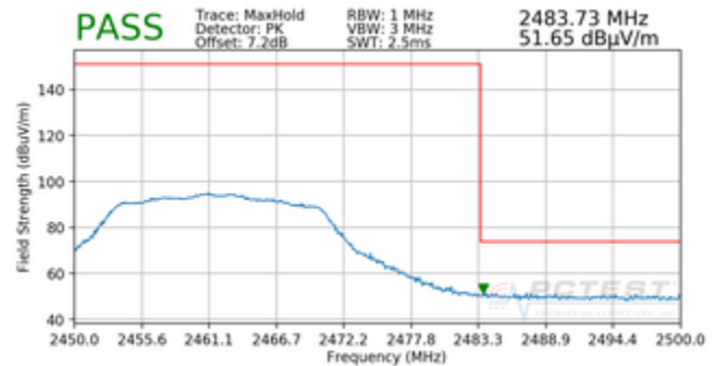
Plot 7-16. Radiated Restricted Upper Band Edge Measurement SISO ANT2 (Peak)
