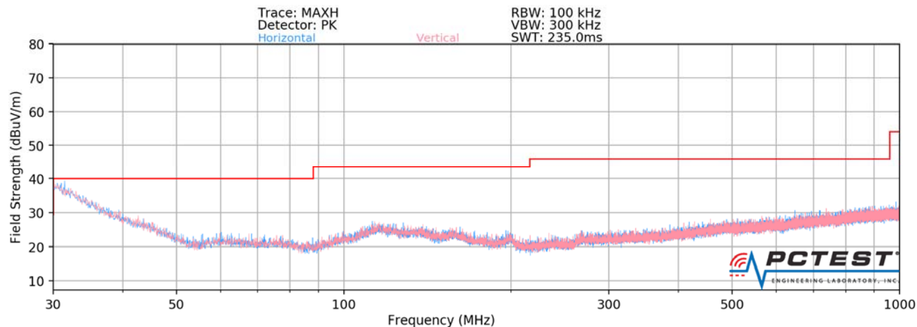
Plot 7-25. Radiated Spurious Plot below 1GHz SISO ANT1
