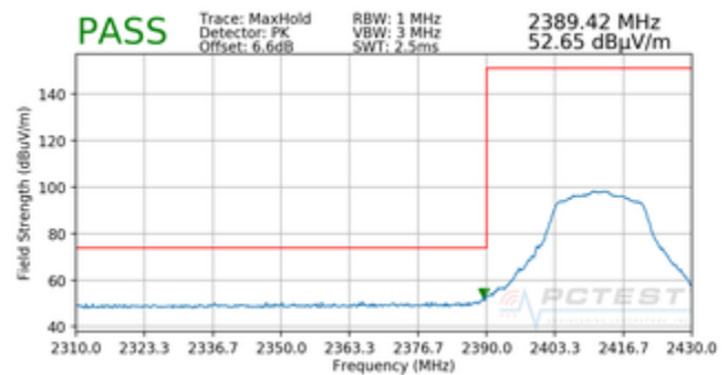
Plot 7-14. Radiated Restricted Lower Band Edge Measurement SISO ANT2 (Peak)
