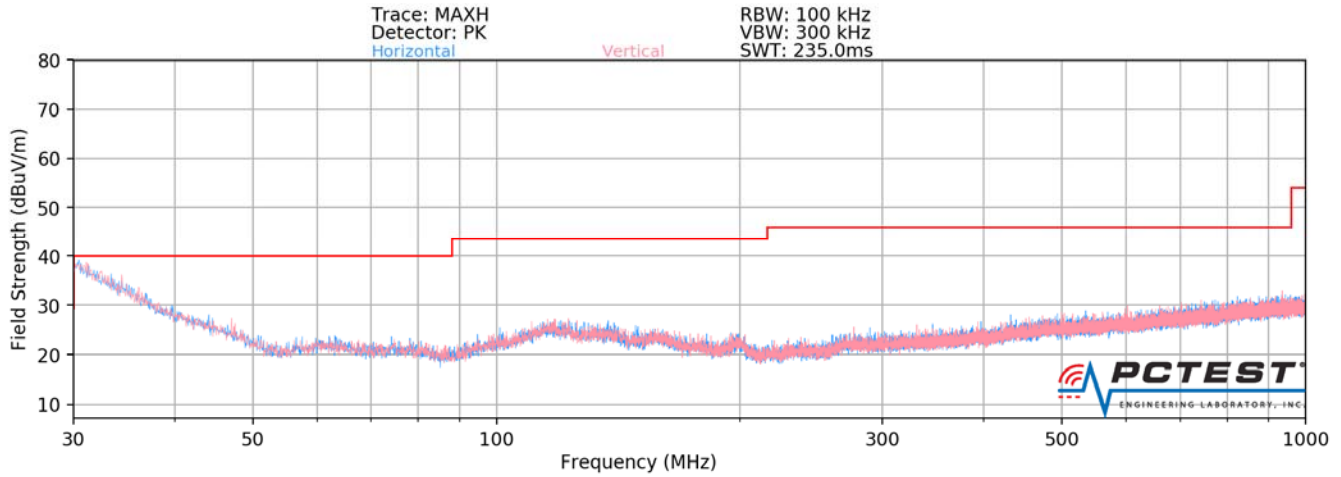
Plot 7-26. Radiated Spurious Plot below 1GHz SISO ANT2
