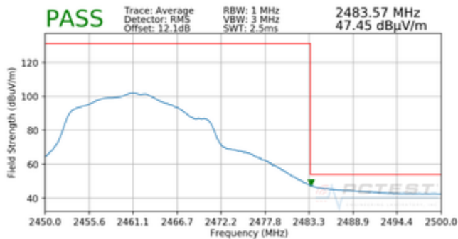
Plot 7-19. Radiated Restricted Upper Band Edge Measurement CDD (Average)
