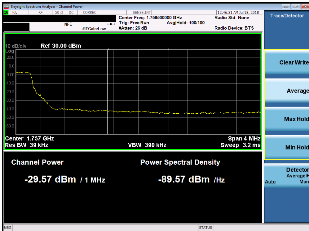
Plot 7-204. Upper Extended Band Edge Plot (Band 4 - 5.0MHz QPSK - Full RB Configuration)
