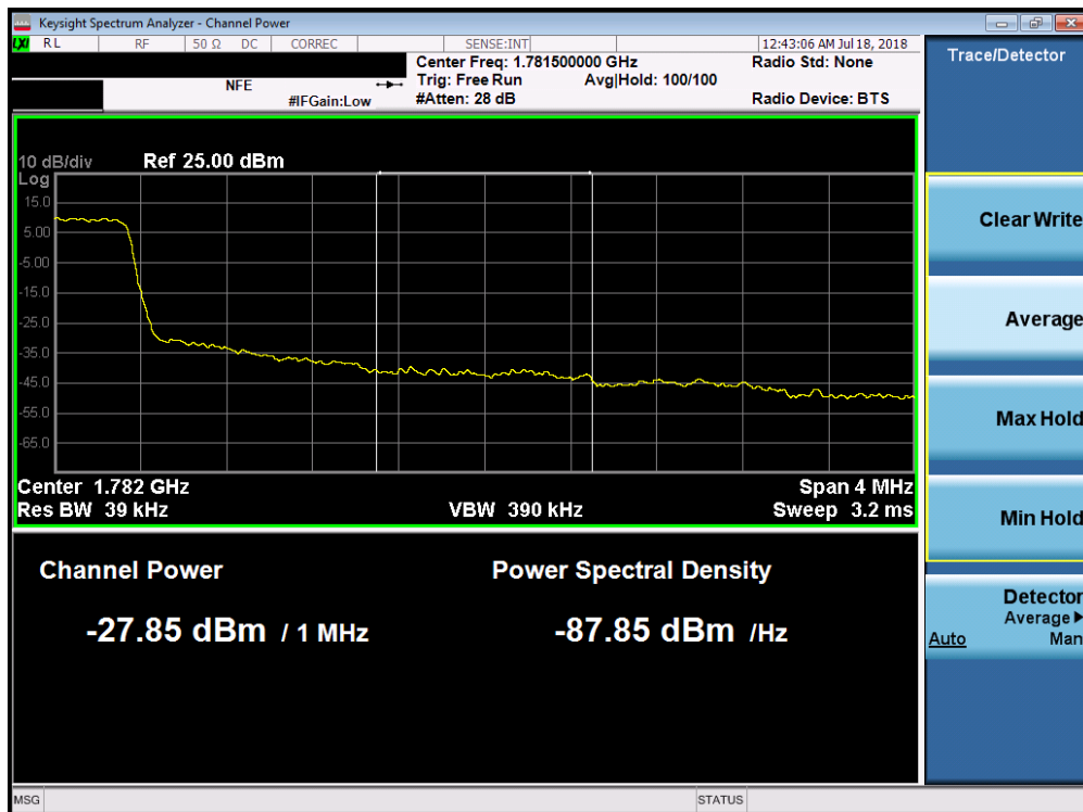
Plot 7-194. Upper Extended Band Edge Plot (Band 66 - 1.4MHz QPSK - Full RB Configuration)
