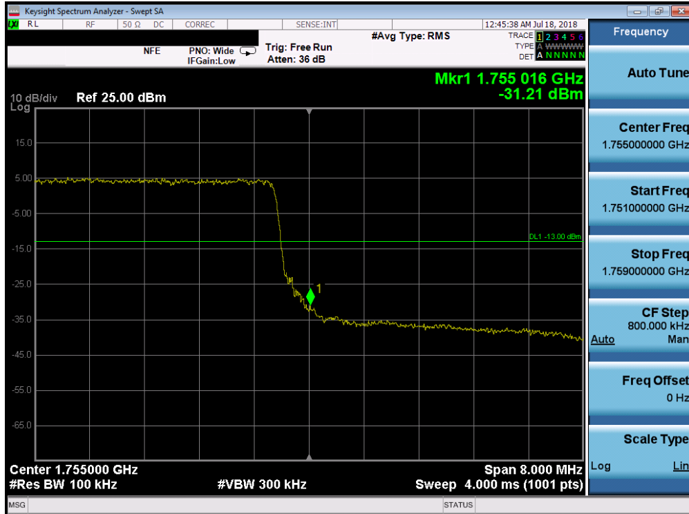
Plot 7-209. Upper Band Edge Plot (Band 4 - 10.0MHz QPSK - Full RB Configuration)
