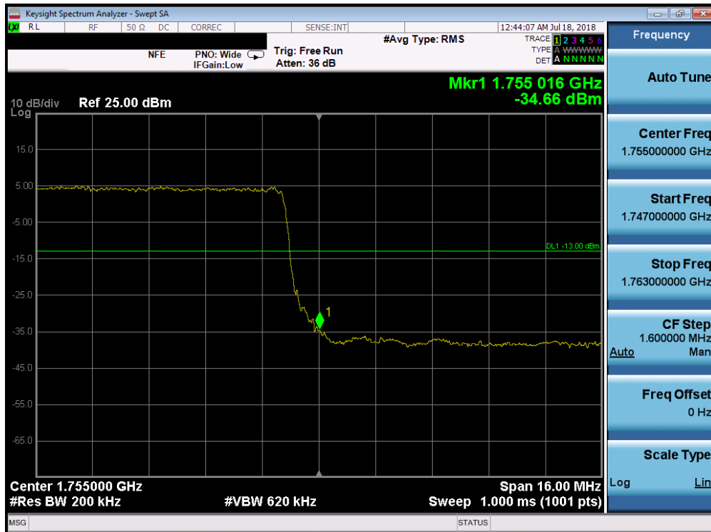
Plot 7-221. Upper Band Edge Plot (Band 4 - 20.0MHz QPSK - Full RB Configuration)
