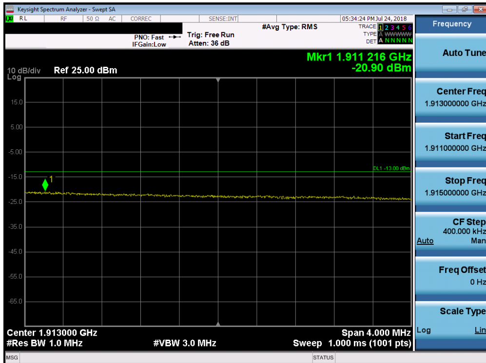
Plot 7-258. Upper Extended Band Edge Plot (Band 2 - 20.0MHz QPSK - Full RB Configuration)
