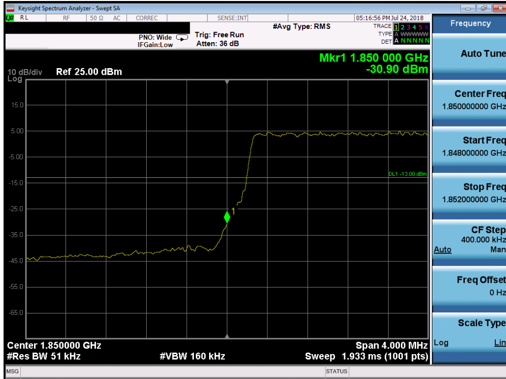
Plot 7-237. Lower Band Edge Plot (Band 25/2 - 5.0MHz QPSK - Full RB Configuration)
