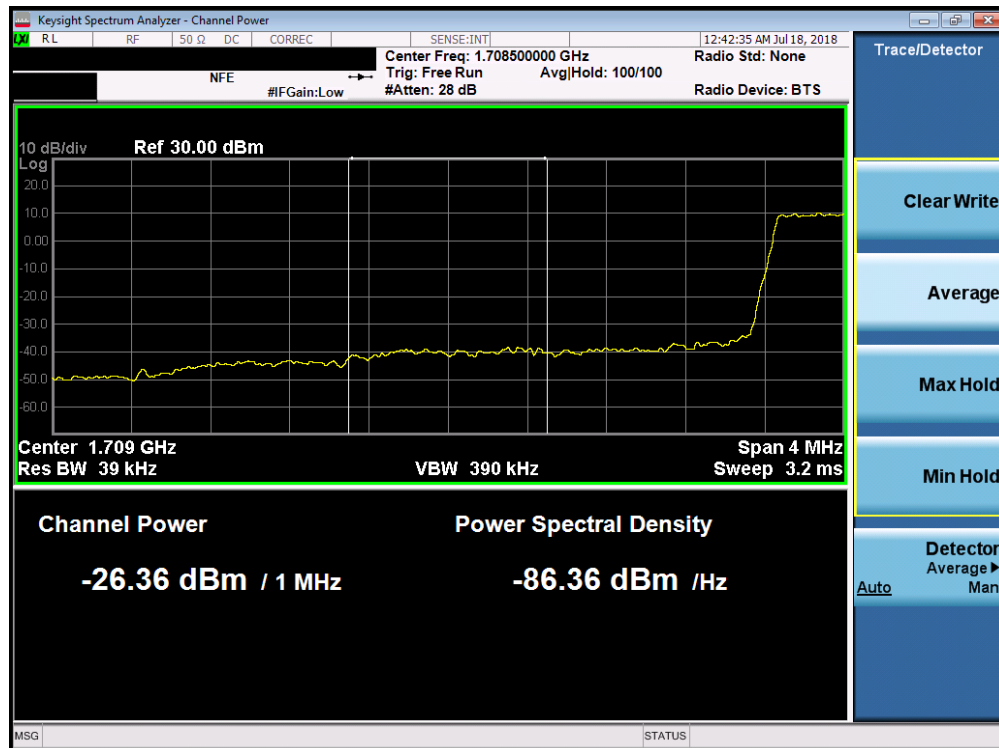
Plot 7-190. Lower Extended Band Edge Plot (Band 66/4 - 1.4MHz QPSK - Full RB Configuration)
