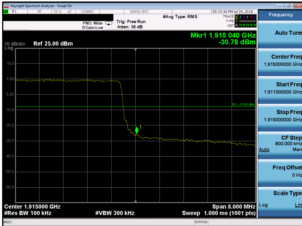
Plot 7-247. Upper Band Edge Plot (Band 25 - 10.0MHz QPSK - Full RB Configuration)
