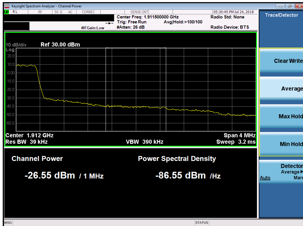
Plot 7-228. Upper Extended Band Edge Plot (Band 2 - 1.4MHz QPSK - Full RB Configuration)
