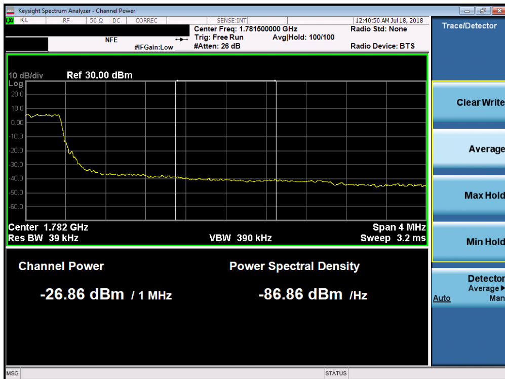
Plot 7-200. Upper Extended Band Edge Plot (Band 66 - 3.0MHz QPSK - Full RB Configuration)
