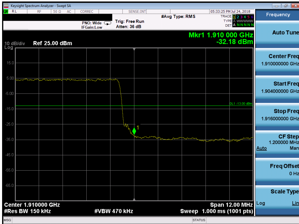
Plot 7-251. Upper Band Edge Plot (Band 2 - 15.0MHz QPSK - Full RB Configuration)
