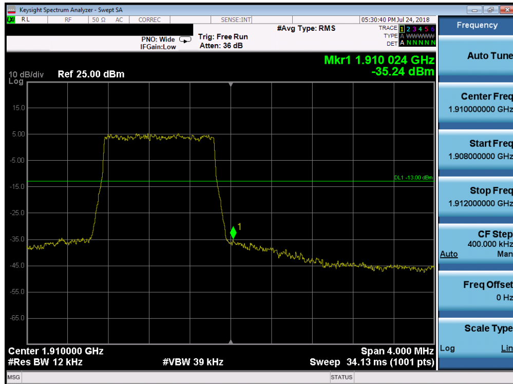
Plot 7-227. Upper Band Edge Plot (Band 2 - 1.4MHz QPSK - Full RB Configuration)
