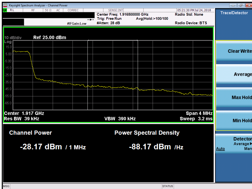
Plot 7-230. Upper Extended Band Edge Plot (Band 25 - 1.4MHz QPSK - Full RB Configuration)
