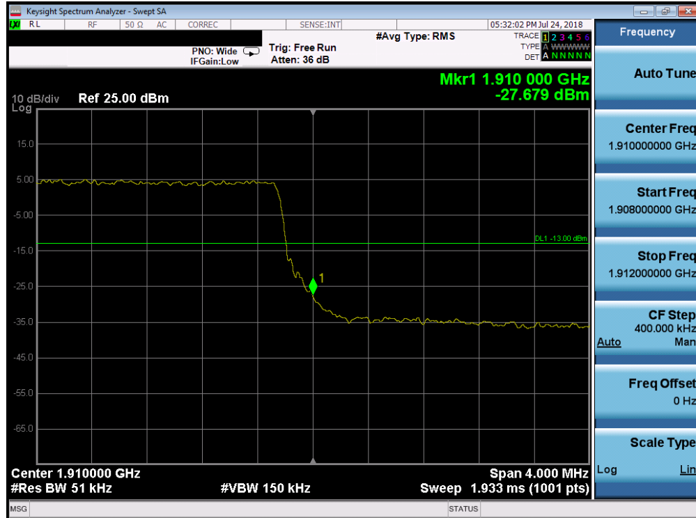
Plot 7-239. Upper Band Edge Plot (Band 2 - 5.0MHz QPSK - Full RB Configuration)
