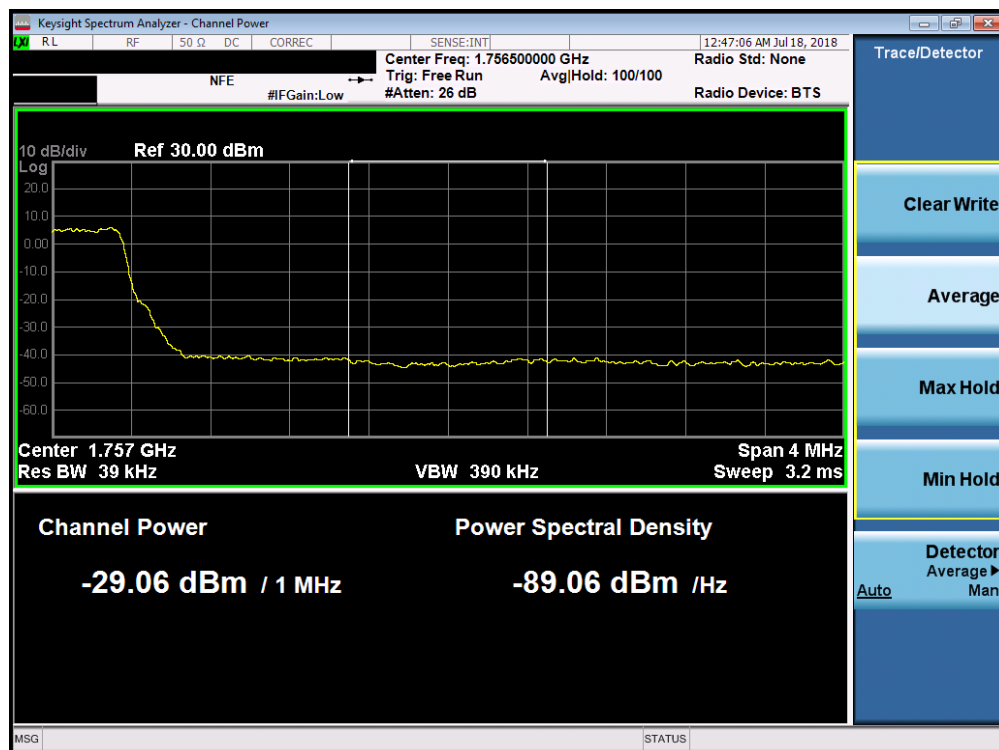
Plot 7-198. Upper Extended Band Edge Plot (Band 4 - 3.0MHz QPSK - Full RB Configuration)
