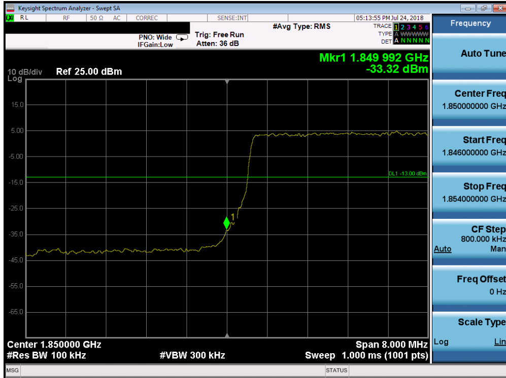
Plot 7-243. Lower Band Edge Plot (Band 25/2 - 10.0MHz QPSK - Full RB Configuration)
