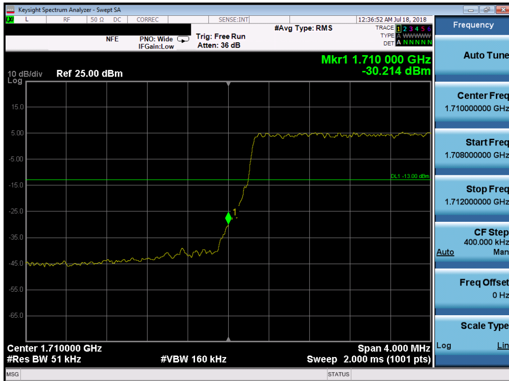
Plot 7-201. Lower Band Edge Plot (Band 66/4 - 5.0MHz QPSK - Full RB Configuration)
