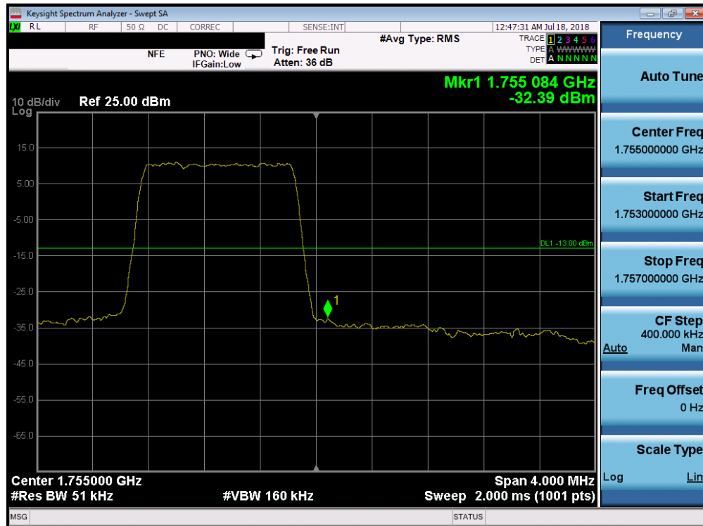
Plot 7-191. Upper Band Edge Plot (Band 4 - 1.4MHz QPSK - Full RB Configuration)
