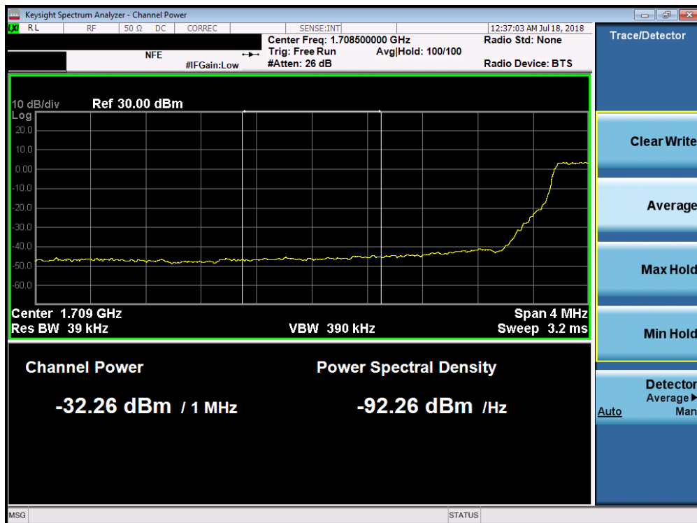
Plot 7-202. Lower Extended Band Edge Plot (Band 66/4 - 5.0MHz QPSK - Full RB Configuration)
