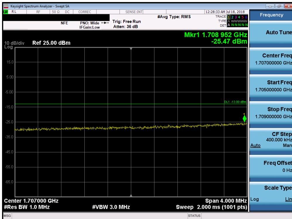
Plot 7-220. Lower Extended Band Edge Plot (Band 66/4 - 20.0MHz QPSK - Full RB Configuration)
