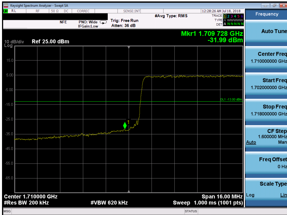
Plot 7-219. Lower Band Edge Plot (Band 66/4 - 20.0MHz QPSK - Full RB Configuration)
