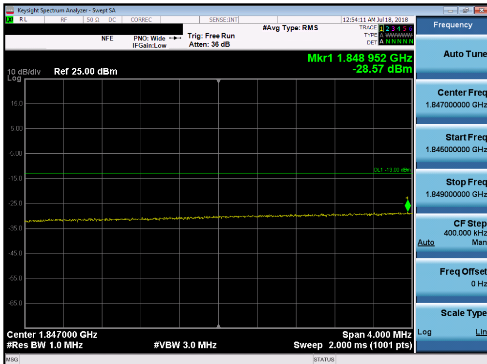
Plot 7-256. Lower Extended Band Edge Plot (Band 25/2 - 20.0MHz QPSK - Full RB Configuration)
