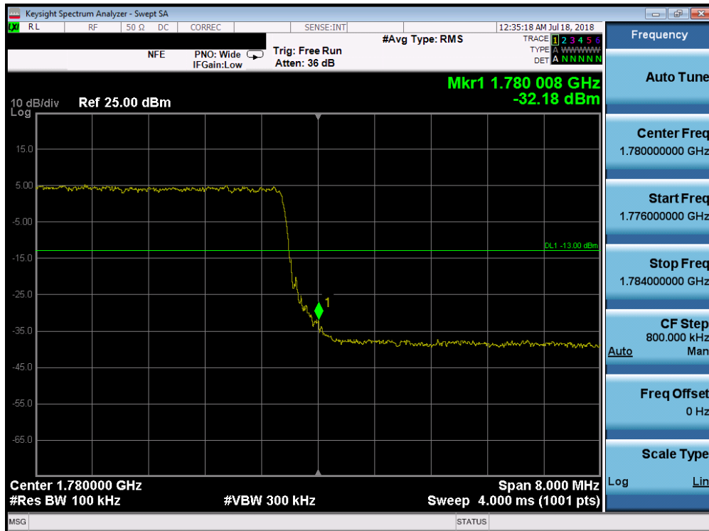
Plot 7-211. Upper Band Edge Plot (Band 66 - 10.0MHz QPSK - Full RB Configuration)
