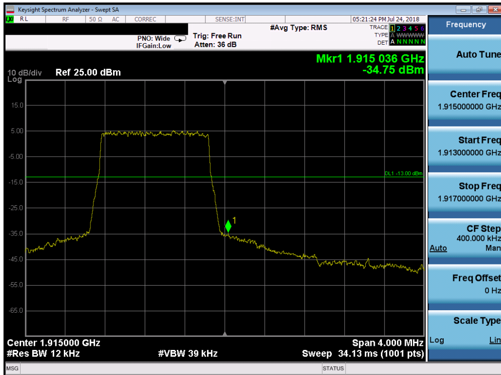
Plot 7-229. Upper Band Edge Plot (Band 25 - 1.4MHz QPSK - Full RB Configuration)
