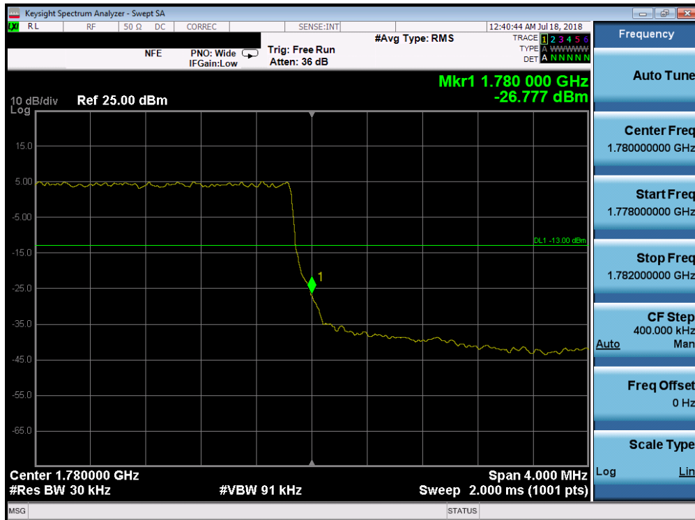
Plot 7-199. Upper Band Edge Plot (Band 66 - 3.0MHz QPSK - Full RB Configuration)
