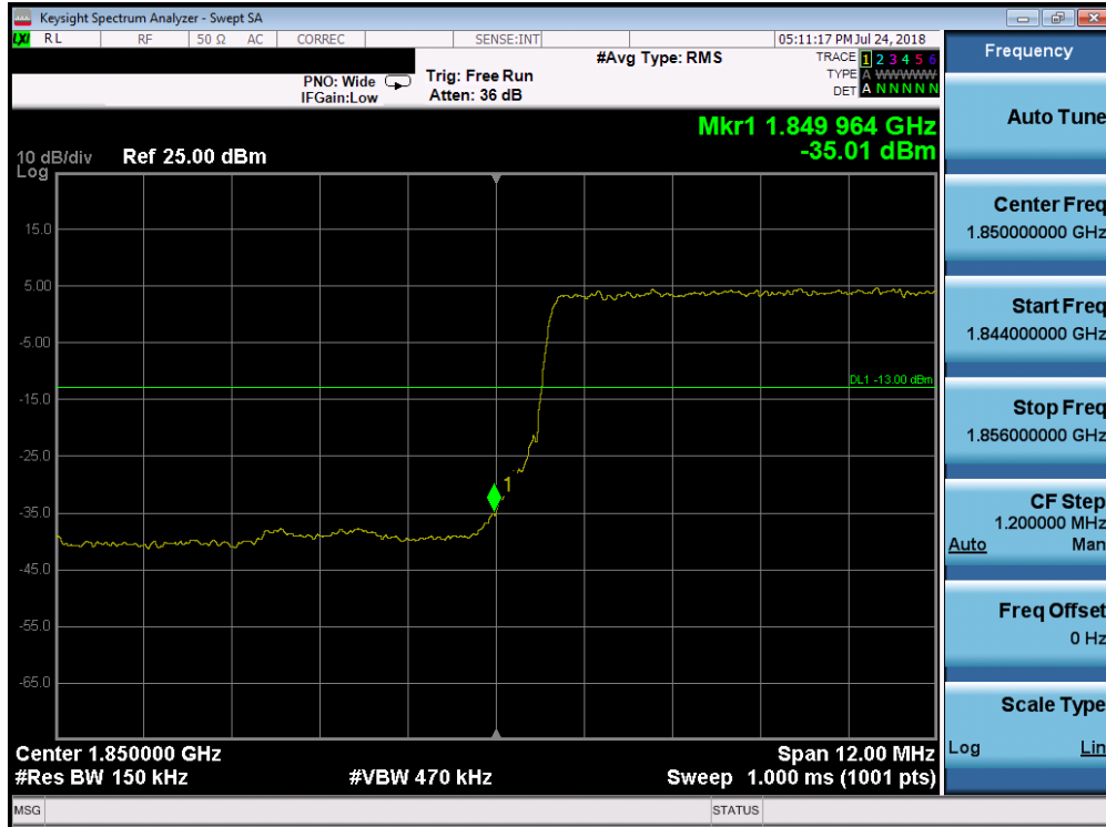
Plot 7-249. Lower Band Edge Plot (Band 25/2 - 15.0MHz QPSK - Full RB Configuration)
