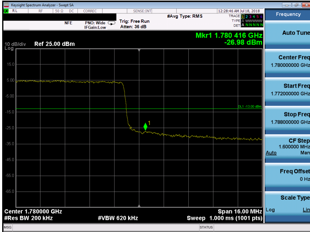
Plot 7-223. Upper Band Edge Plot (Band 66 - 20.0MHz QPSK - Full RB Configuration)
