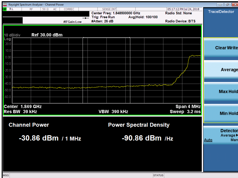
Plot 7-238. Lower Extended Band Edge Plot (Band 25/2 - 5.0MHz QPSK - Full RB Configuration)
