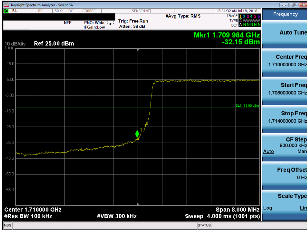
Plot 7-207. Lower Band Edge Plot (Band 66/4 - 10.0MHz QPSK - Full RB Configuration)
