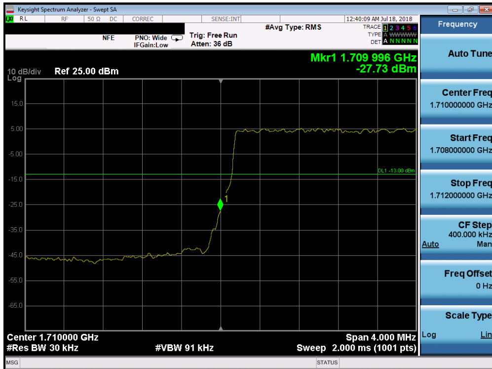
Plot 7-195. Lower Band Edge Plot (Band 66/4 - 3.0MHz QPSK - Full RB Configuration)
