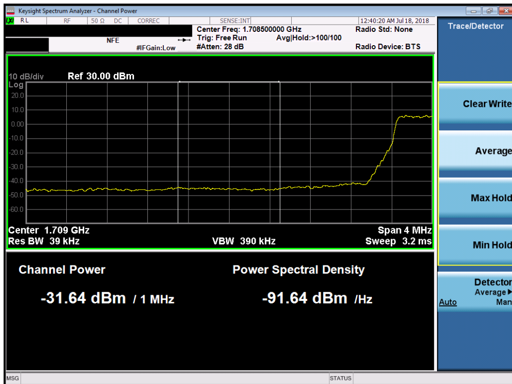
Plot 7-196. Lower Extended Band Edge Plot (Band 66/4 - 3.0MHz QPSK - Full RB Configuration)
