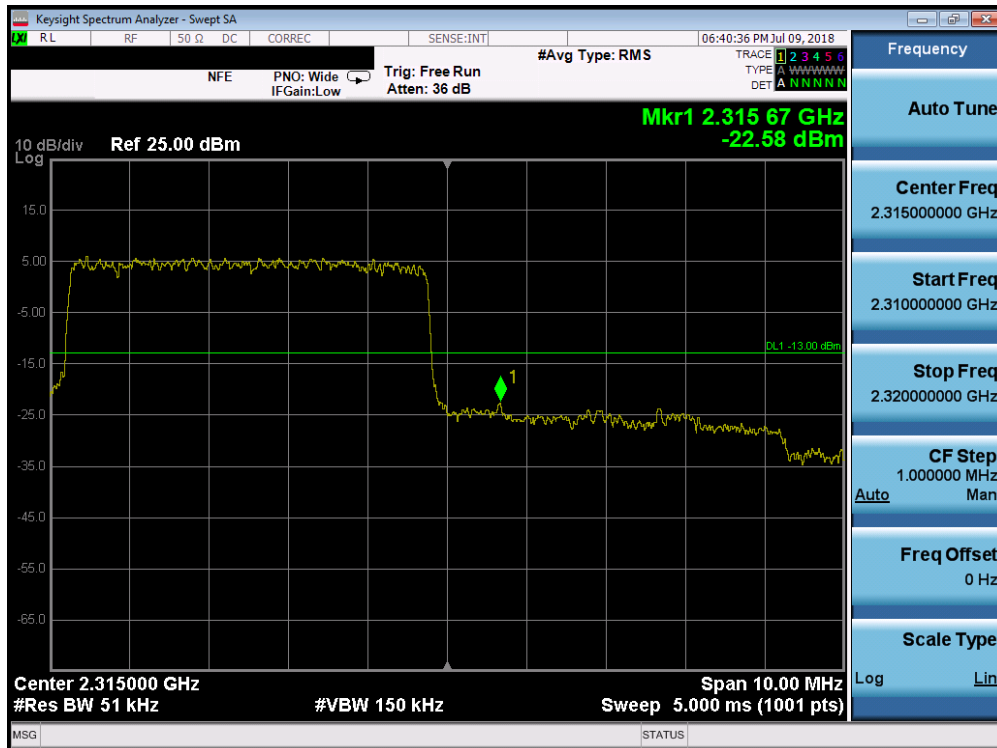
Plot 7-263. Upper Band Edge Plot (Band 30 - 5.0MHz QPSK - Full RB Configuration)
