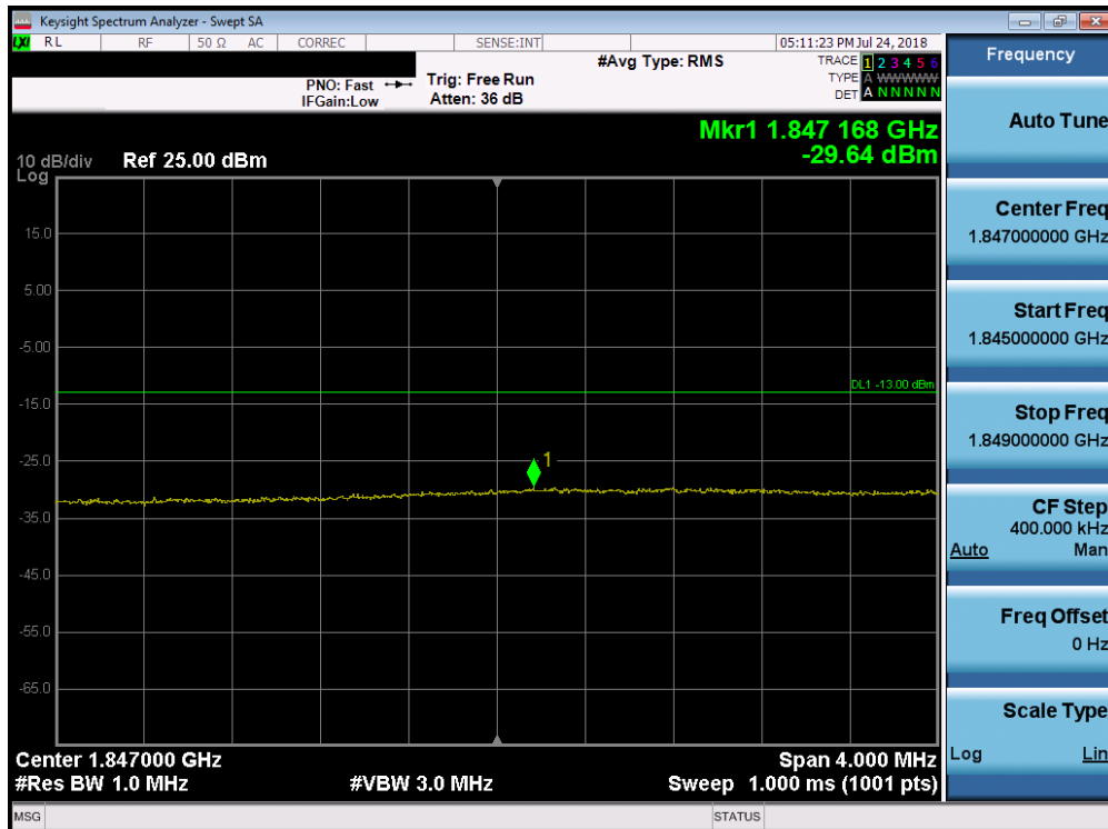
Plot 7-250. Lower Extended Band Edge Plot (Band 25/2 - 15.0MHz QPSK - Full RB Configuration)
