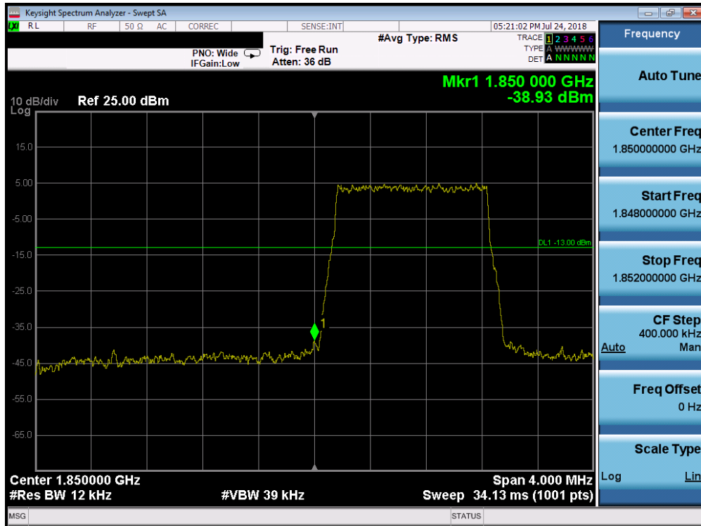
Plot 7-225. Lower Band Edge Plot (Band 25/2 - 1.4MHz QPSK - Full RB Configuration)
