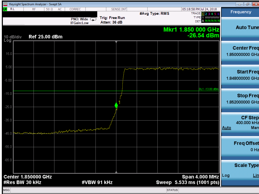
Plot 7-231. Lower Band Edge Plot (Band 25/2 - 3.0MHz QPSK - Full RB Configuration)
