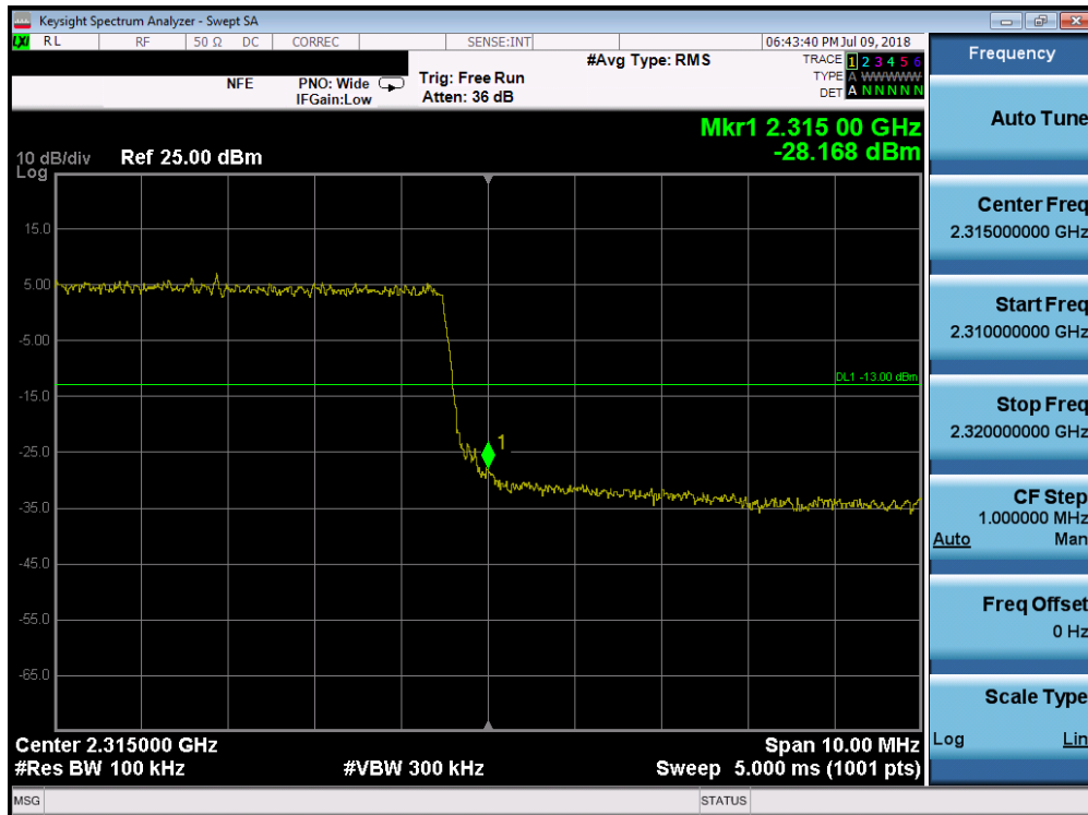
Plot 7-267. Upper Band Edge Plot (Band 30 - 10.0MHz QPSK - Full RB Configuration)
