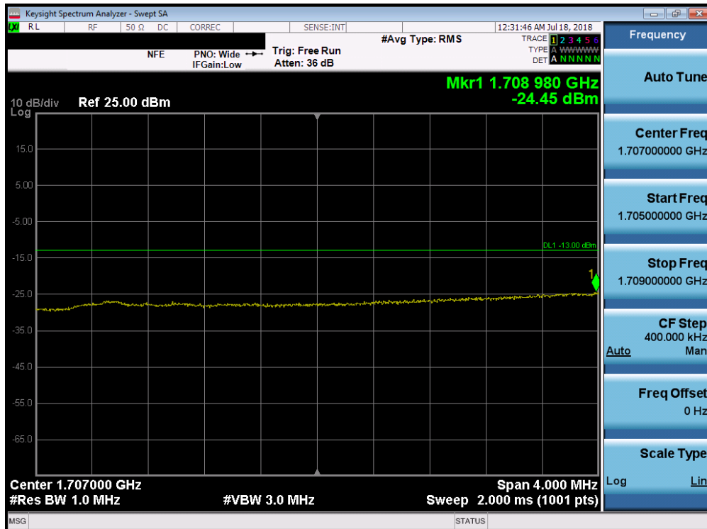
Plot 7-214. Lower Extended Band Edge Plot (Band 66/4 - 15.0MHz QPSK - Full RB Configuration)
