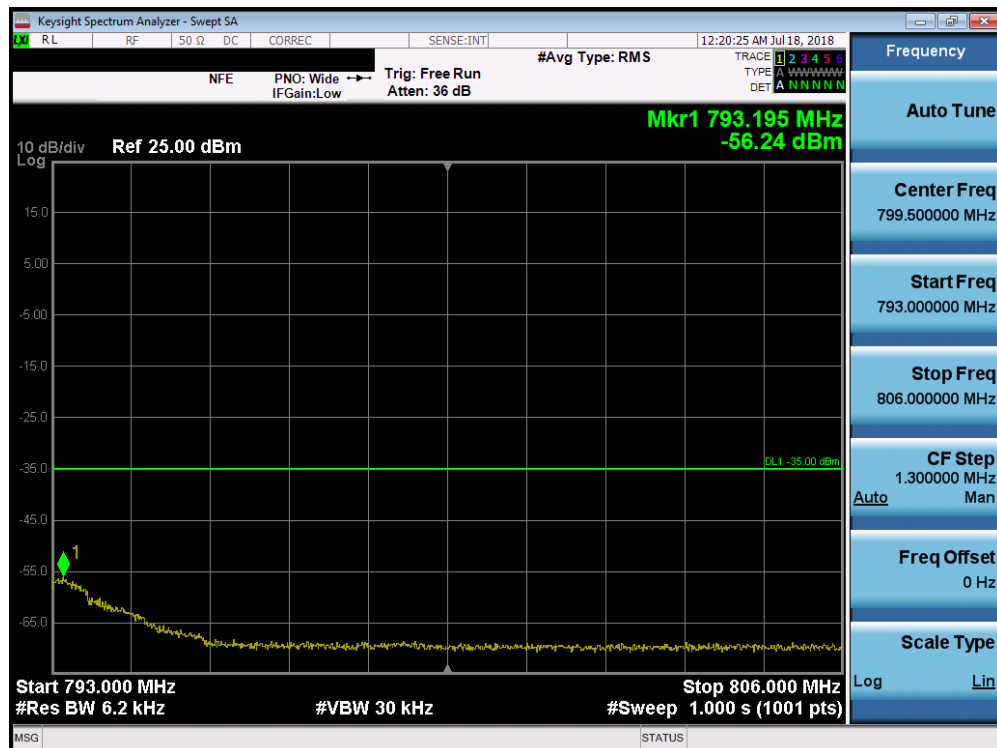
Plot 7-180. Upper Emission Mask Plot (Band 13 - 10.0MHz QPSK - Full RB Configuration)
