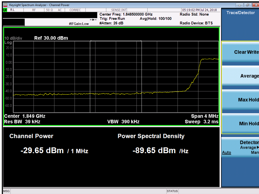
Plot 7-232. Lower Extended Band Edge Plot (Band 25/2 - 3.0MHz QPSK - Full RB Configuration)
