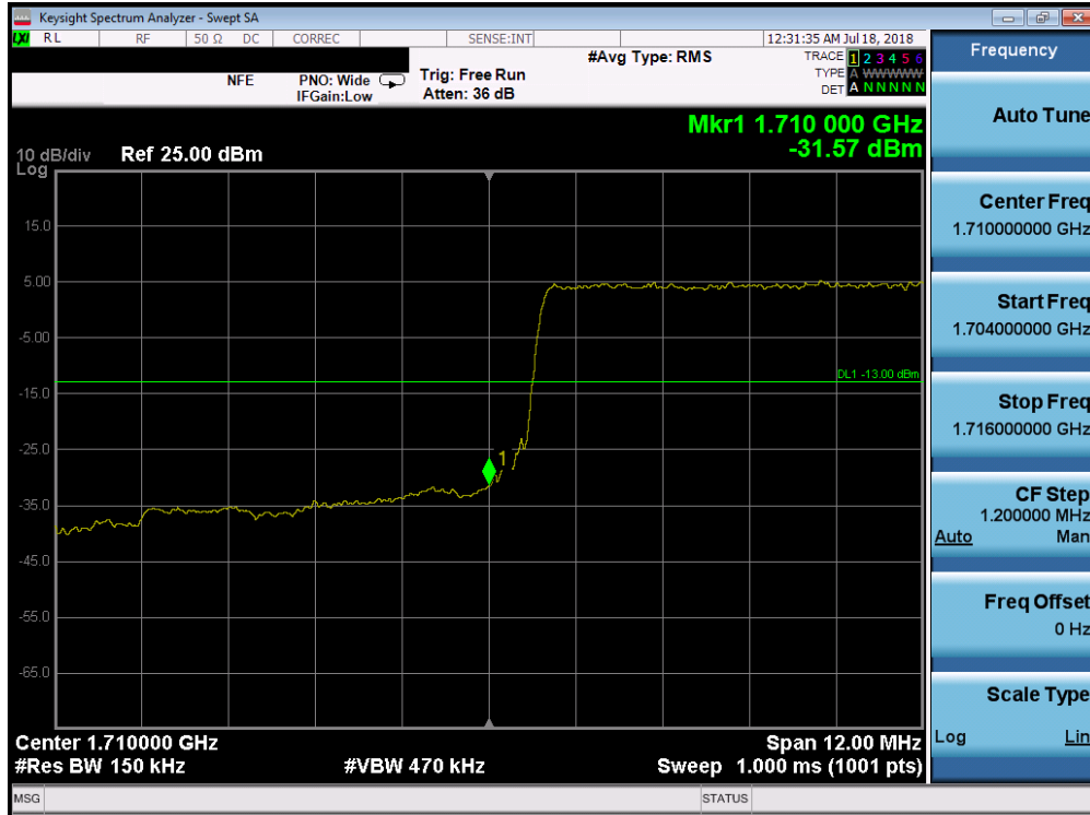
Plot 7-213. Lower Band Edge Plot (Band 66/4 - 15.0MHz QPSK - Full RB Configuration)
