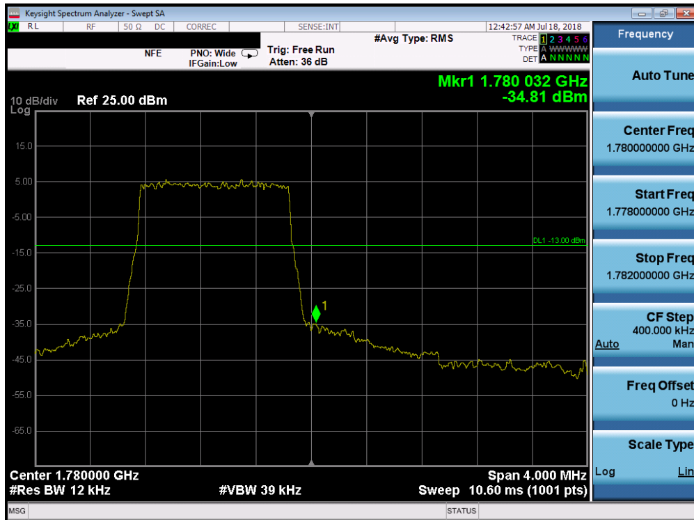
Plot 7-193. Upper Band Edge Plot (Band 66 - 1.4MHz QPSK - Full RB Configuration)
