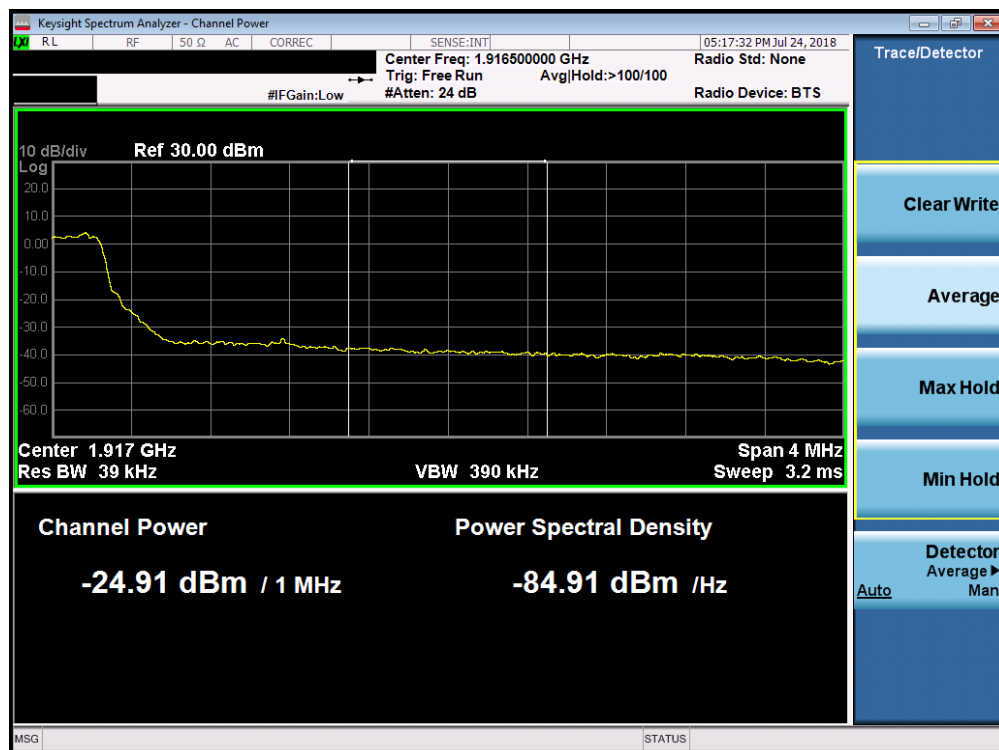
Plot 7-242. Upper Extended Band Edge Plot (Band 25 - 5.0MHz QPSK - Full RB Configuration)
