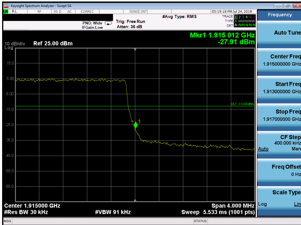
Plot 7-235. Upper Band Edge Plot (Band 25 - 3.0MHz QPSK - Full RB Configuration)
