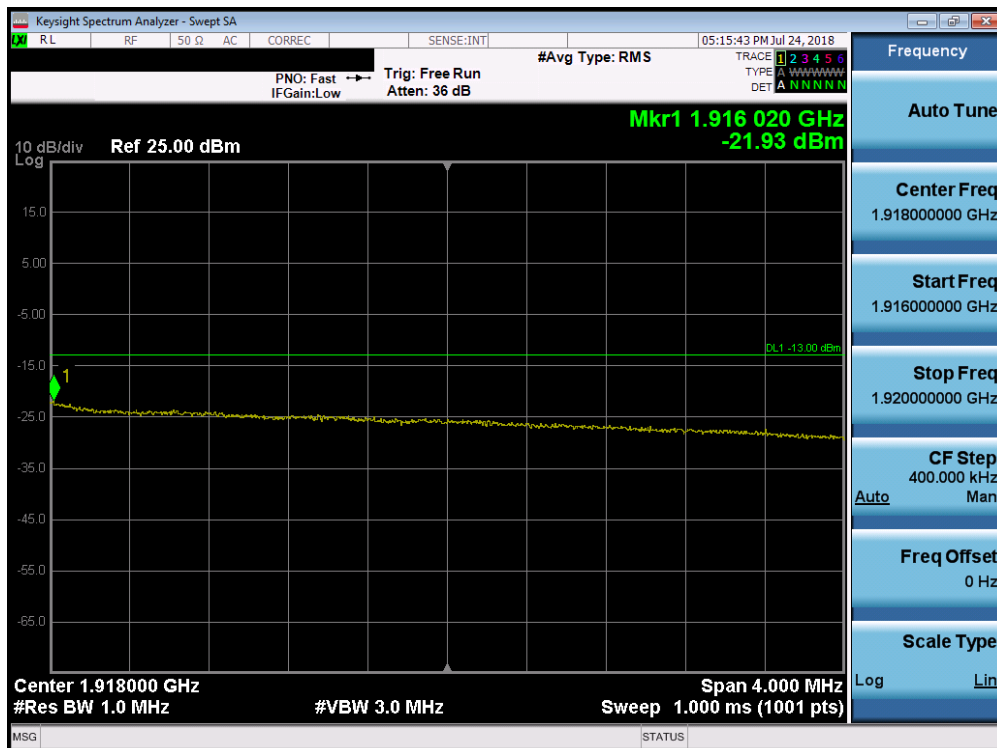
Plot 7-248. Upper Extended Band Edge Plot (Band 25 - 10.0MHz QPSK - Full RB Configuration)
