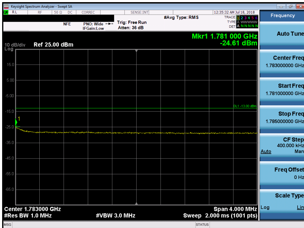
Plot 7-212. Upper Extended Band Edge Plot (Band 66 - 10.0MHz QPSK - Full RB Configuration)
