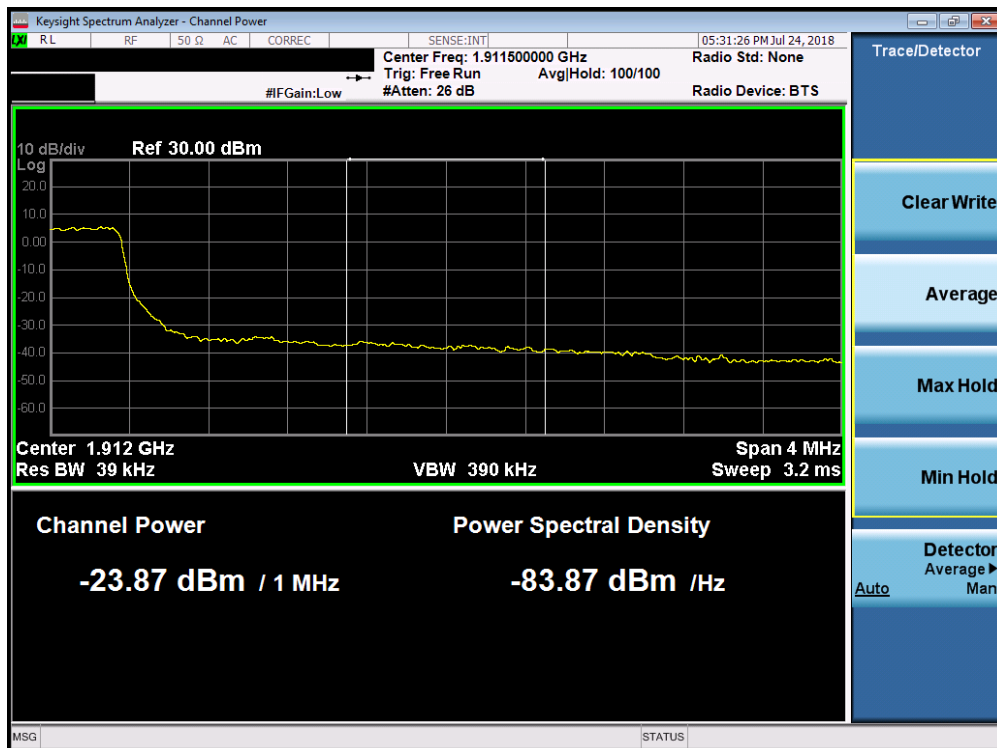
Plot 7-234. Upper Extended Band Edge Plot (Band 2 - 3.0MHz QPSK - Full RB Configuration)
