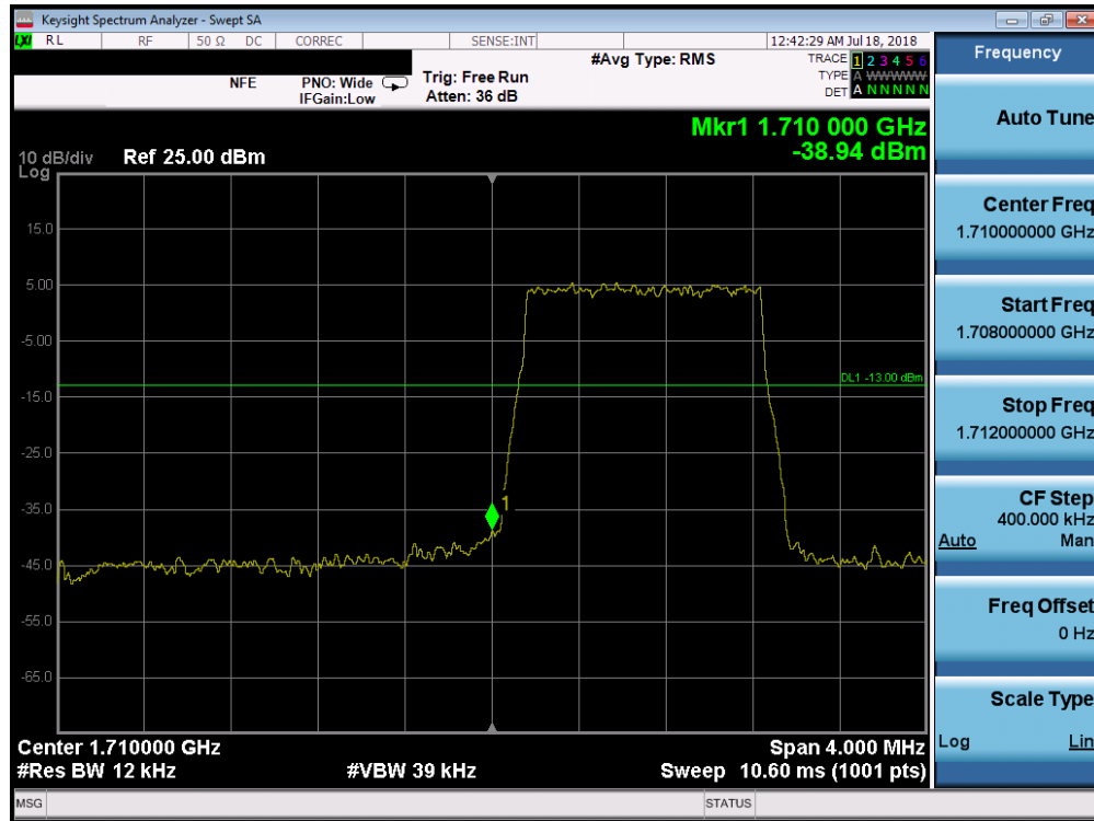
Plot 7-189. Lower Band Edge Plot (Band 66/4 - 1.4MHz QPSK - Full RB Configuration)
