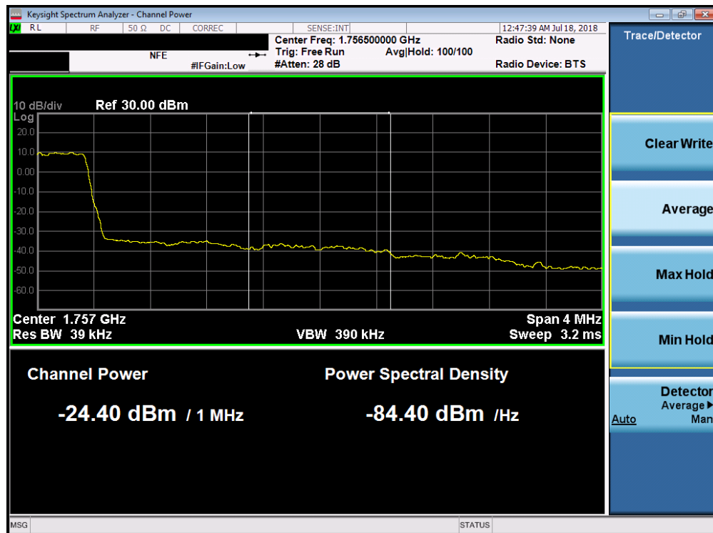
Plot 7-192. Upper Extended Band Edge Plot (Band 4 - 1.4MHz QPSK - Full RB Configuration)
