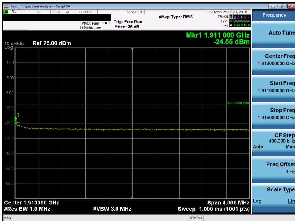
Plot 7-246. Upper Extended Band Edge Plot (Band 2 - 10.0MHz QPSK - Full RB Configuration)
