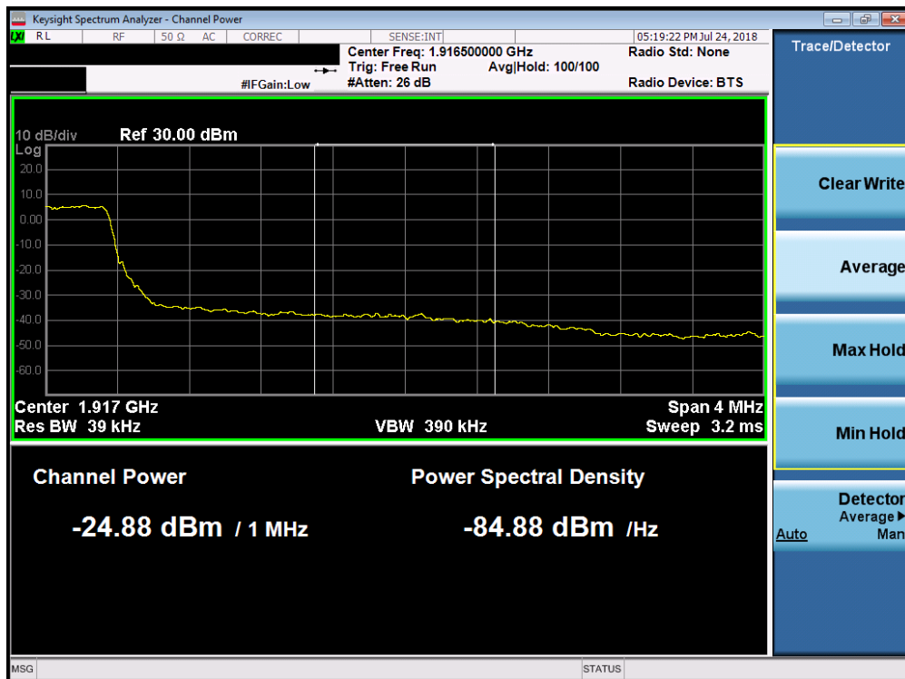
Plot 7-236. Upper Extended Band Edge Plot (Band 25 - 3.0MHz QPSK - Full RB Configuration)
