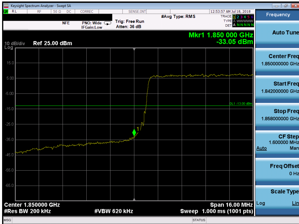
Plot 7-255. Lower Band Edge Plot (Band 25/2 - 20.0MHz QPSK - Full RB Configuration)
