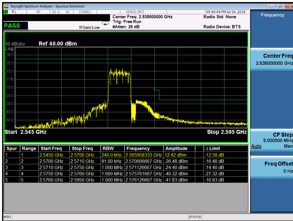
Plot 7-270. Upper ACP Plot (Band 7 - 5.0MHz QPSK - RB Size 25)
