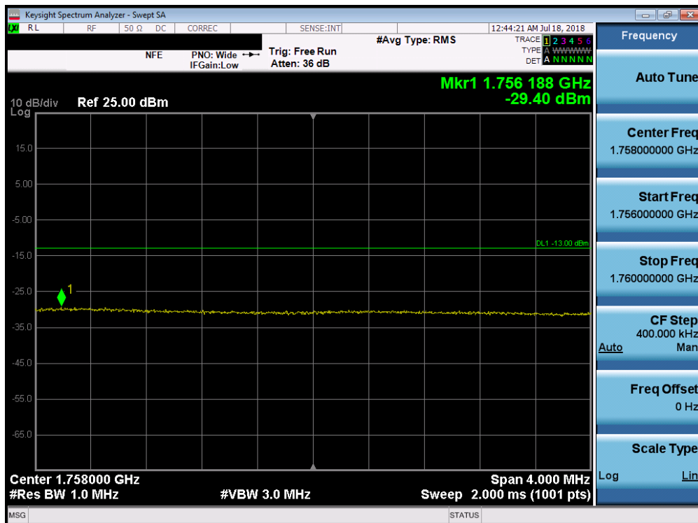
Plot 7-222. Upper Extended Band Edge Plot (Band 4 - 20.0MHz QPSK - Full RB Configuration)
