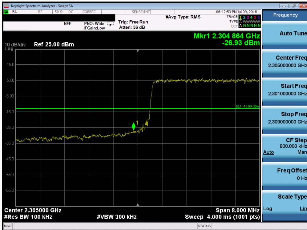
Plot 7-265. Lower Band Edge Plot (Band 30 - 10.0MHz QPSK - Full RB Configuration)
