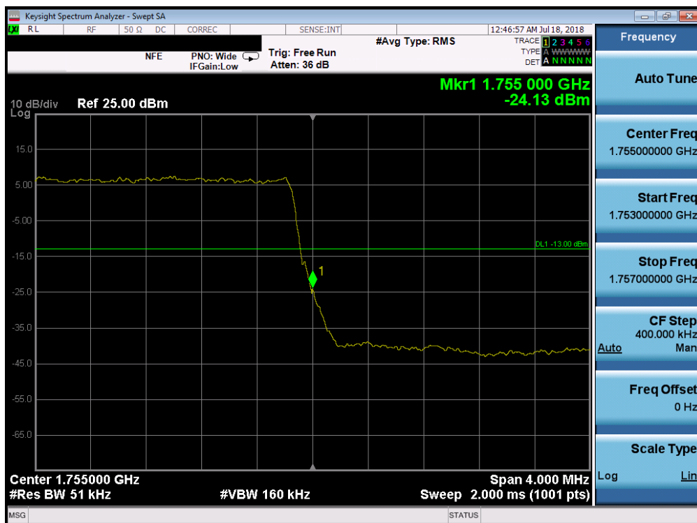
Plot 7-197. Upper Band Edge Plot (Band 4 - 3.0MHz QPSK - Full RB Configuration)
