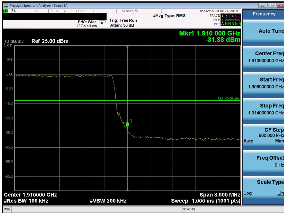
Plot 7-245. Upper Band Edge Plot (Band 2 - 10.0MHz QPSK - Full RB Configuration)
