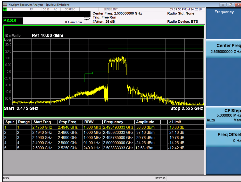
Plot 7-269. Lower ACP Plot (Band 7 - 5.0MHz QPSK - RB Size 25)
