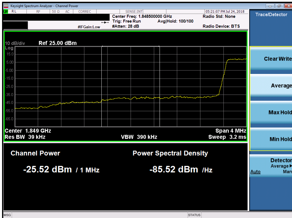
Plot 7-226. Lower Extended Band Edge Plot (Band 25/2 - 1.4MHz QPSK - Full RB Configuration)
