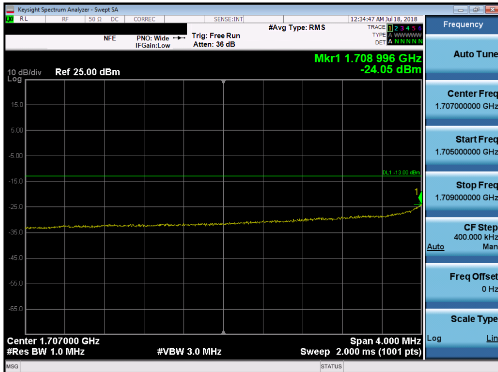
Plot 7-208. Lower Extended Band Edge Plot (Band 66/4 - 10.0MHz QPSK - Full RB Configuration)
