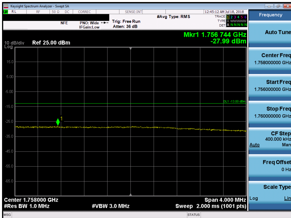
Plot 7-216. Upper Extended Band Edge Plot (Band 4 - 15.0MHz QPSK - Full RB Configuration)
