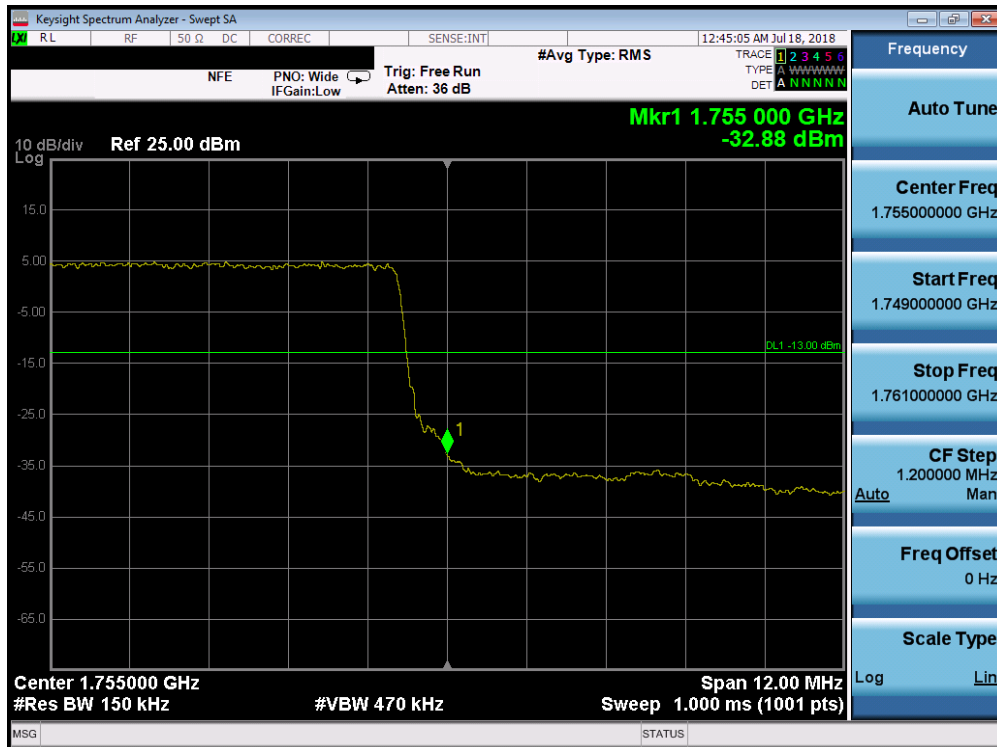
Plot 7-215. Upper Band Edge Plot (Band 4 - 15.0MHz QPSK - Full RB Configuration)
