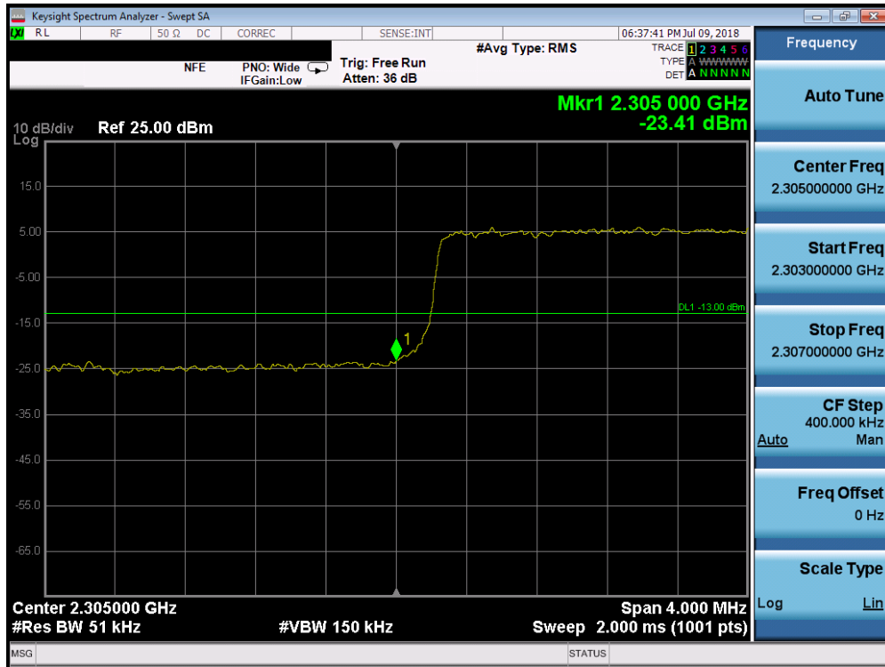
Plot 7-261. Lower Band Edge Plot (Band 30 - 5.0MHz QPSK - Full RB Configuration)
