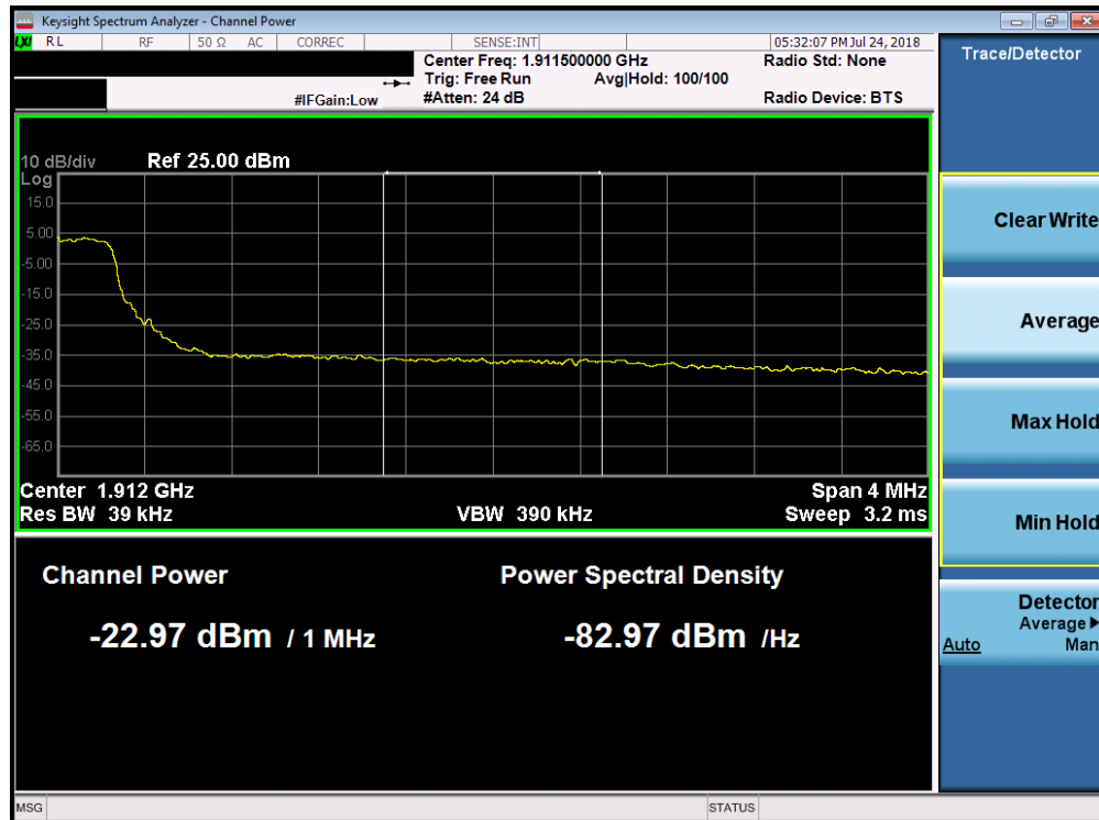
Plot 7-240. Upper Extended Band Edge Plot (Band 2 - 5.0MHz QPSK - Full RB Configuration)
