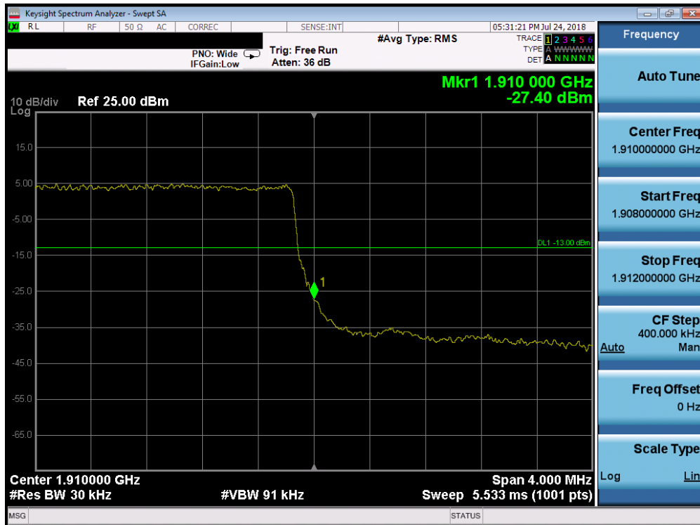
Plot 7-233. Upper Band Edge Plot (Band 2 - 3.0MHz QPSK - Full RB Configuration)
