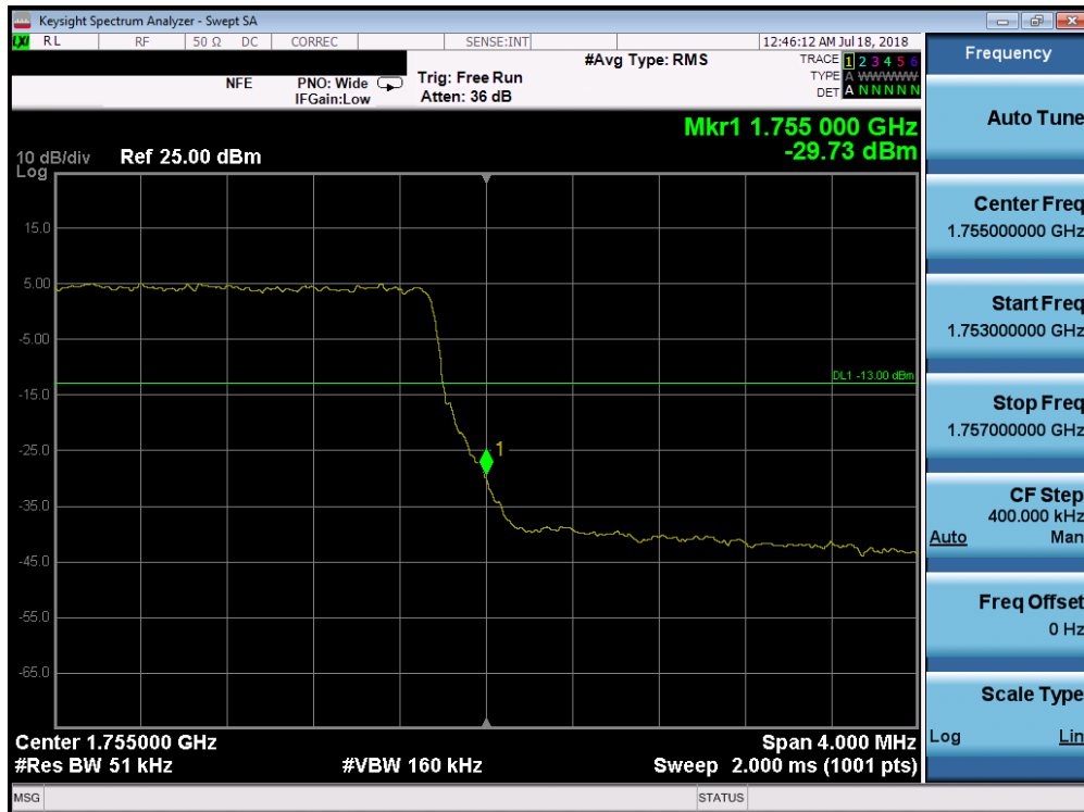
Plot 7-203. Upper Band Edge Plot (Band 4 - 5.0MHz QPSK - Full RB Configuration)
