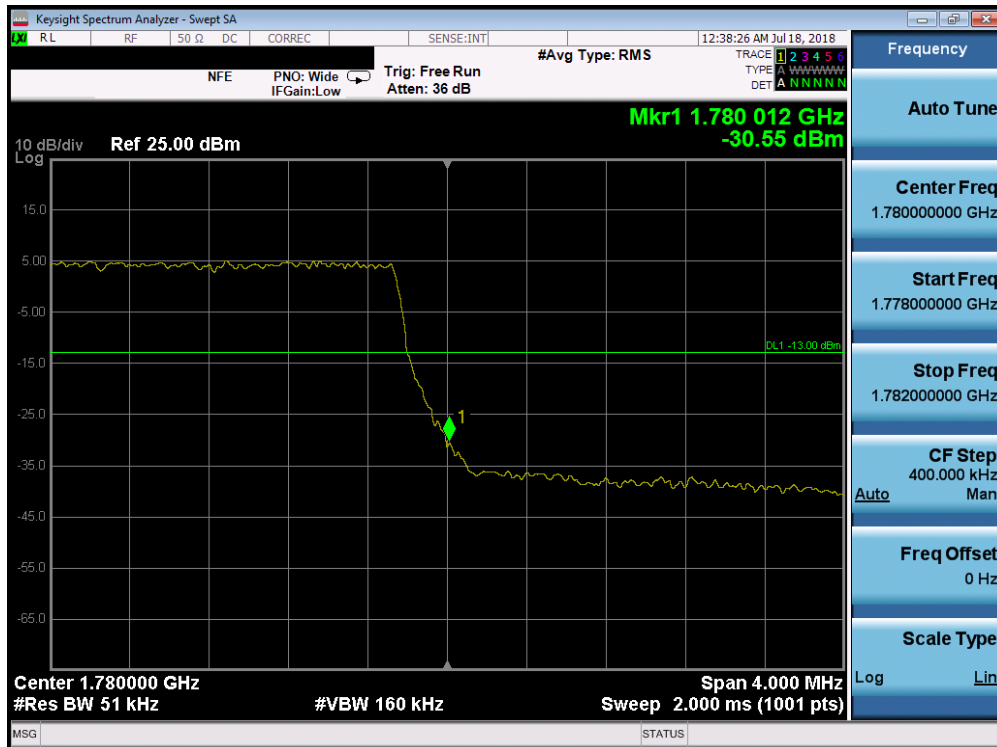
Plot 7-205. Upper Band Edge Plot (Band 66 - 5.0MHz QPSK - Full RB Configuration)
