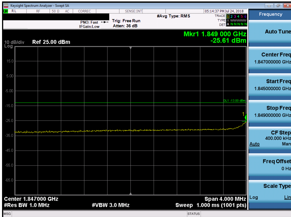
Plot 7-244. Lower Extended Band Edge Plot (Band 25/2 - 10.0MHz QPSK - Full RB Configuration)
