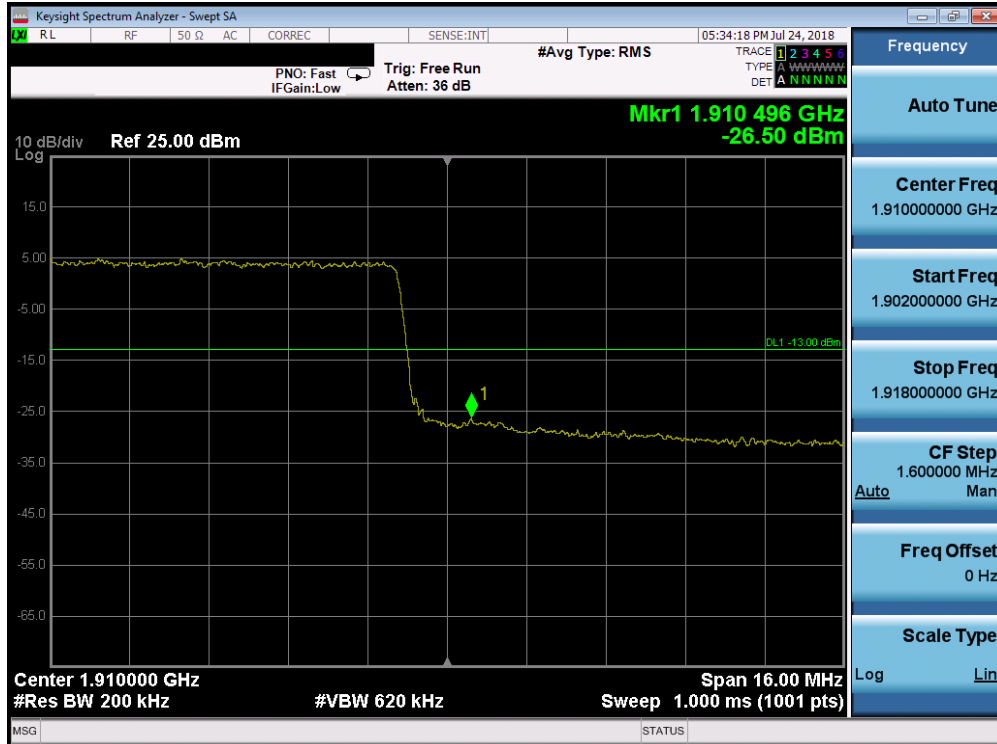
Plot 7-257. Upper Band Edge Plot (Band 2 - 20.0MHz QPSK - Full RB Configuration)
