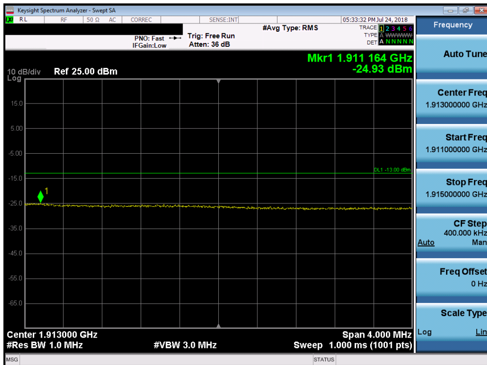
Plot 7-252. Upper Extended Band Edge Plot (Band 2 - 15.0MHz QPSK - Full RB Configuration)
