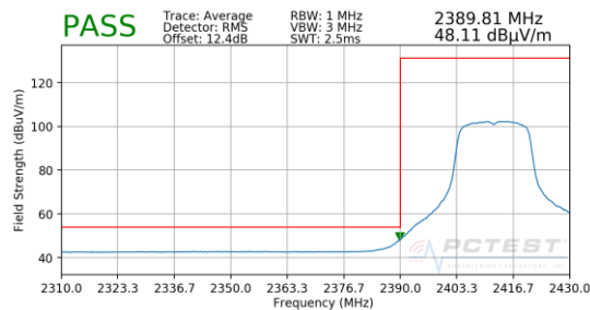
Plot 7-85. Radiated Restricted Lower Band Edge Measurement CDD (Average)
