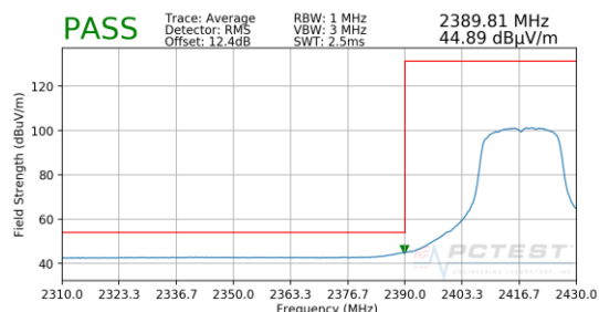
Plot 7-95. Radiated Restricted Lower Band Edge Measurement MIMO (Average)
