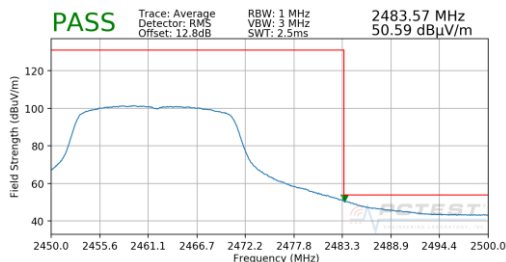
Plot 7-99. Radiated Restricted Upper Band Edge Measurement MIMO (Average)
