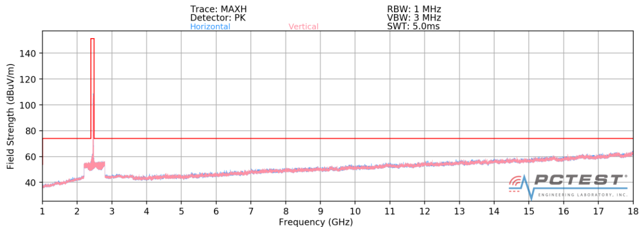
Plot 7-63. Radiated Spurious Plot above 1GHz SISO ANT1 (802.11b – Ch. 11)
