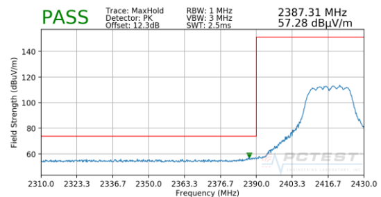
Plot 7-88. Radiated Restricted Lower Band Edge Measurement CDD (Peak)
