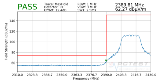
Plot 7-86. Radiated Restricted Lower Band Edge Measurement CDD (Peak)
