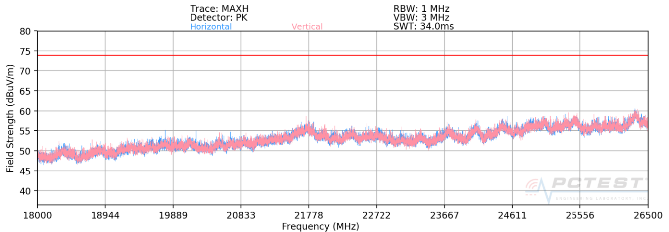
Plot 7-68. Radiated Spurious Plot above 18GHz SISO ANT2
