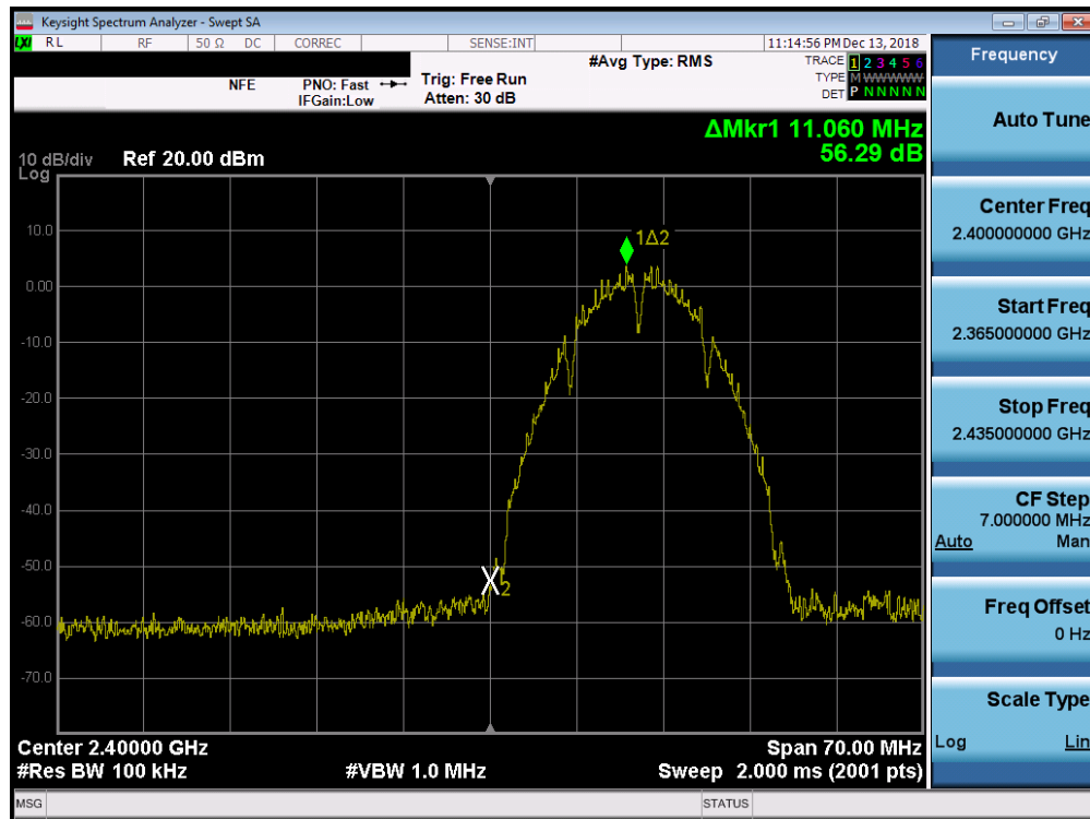
Plot 7-43. Band Edge Plot SISO ANT2 (802.11b – Ch. 1)
