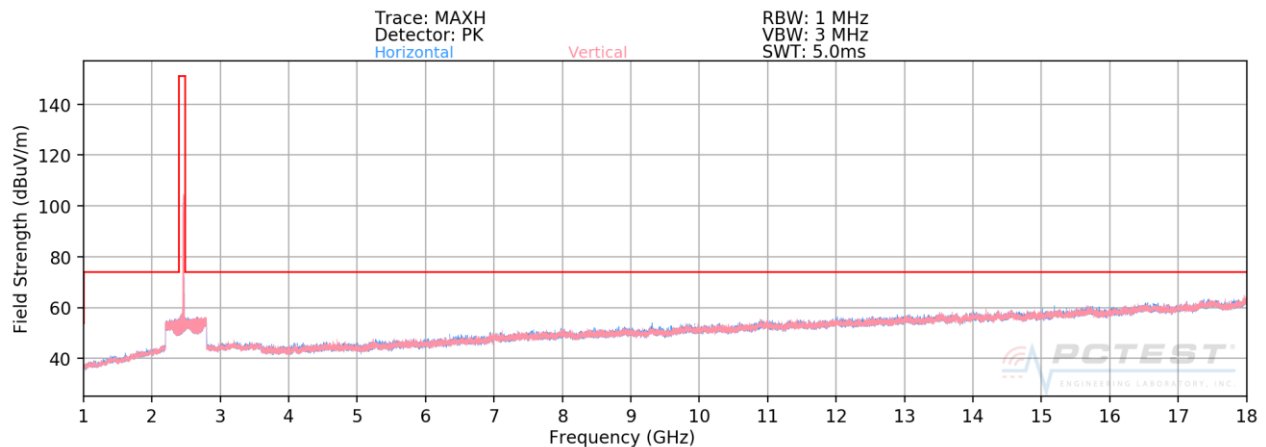
Plot 7-67. Radiated Spurious Plot above 1GHz SISO ANT2 (802.11b – Ch. 11)
