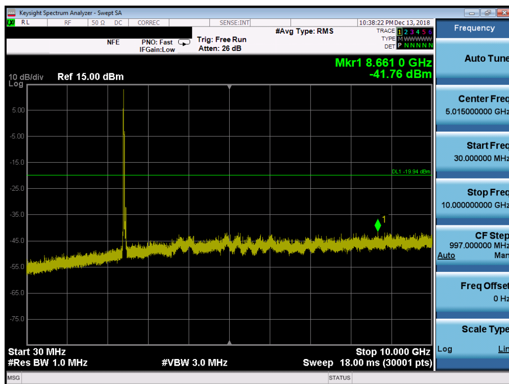
Plot 7-49. Conducted Spurious Plot SISO ANT1 (802.11b – Ch. 1)
