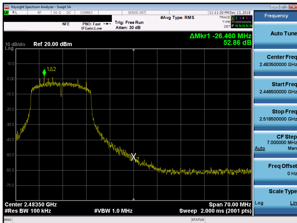
Plot 7-42. Band Edge Plot SISO ANT1 (802.11n (2.4GHz) – Ch. 11)
