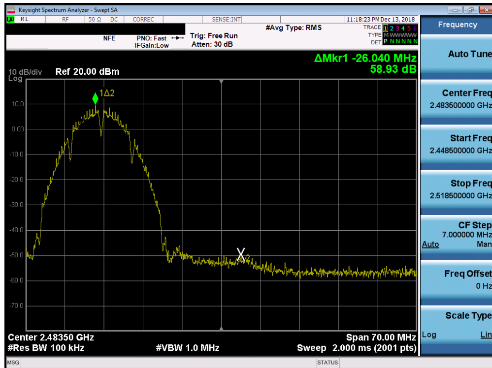
Plot 7-44. Band Edge Plot SISO ANT2 (802.11b – Ch. 11)
