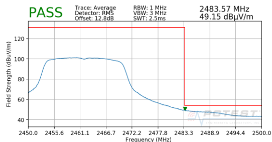
Plot 7-75. Radiated Restricted Upper Band Edge Measurement SISO ANT1 (Average)
