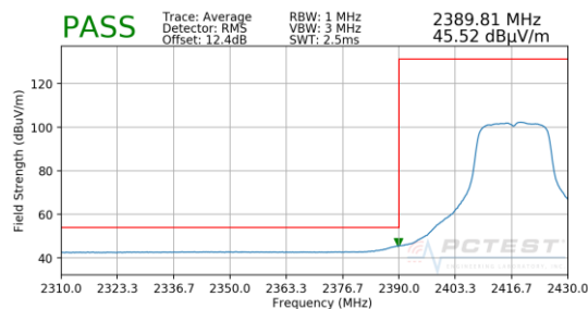
Plot 7-87. Radiated Restricted Lower Band Edge Measurement CDD (Average)
