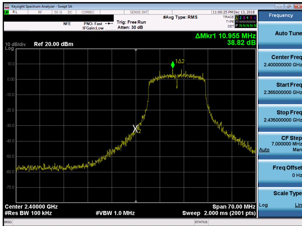
Plot 7-39. Band Edge Plot SISO ANT1 (802.11g- Ch. 1)
