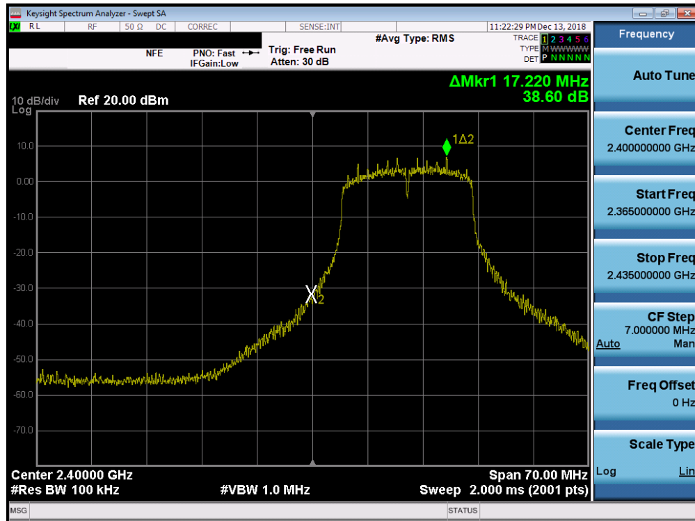
Plot 7-45. Band Edge Plot SISO ANT2 (802.11g- Ch. 1)
