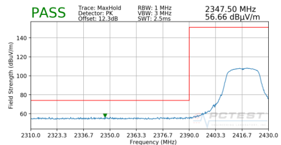
Plot 7-80. Radiated Restricted Lower Band Edge Measurement SISO ANT2 (Peak)
