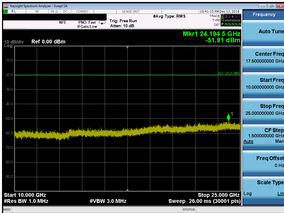
Plot 7-52. Conducted Spurious Plot SISO ANT1 (802.11b – Ch. 6)
