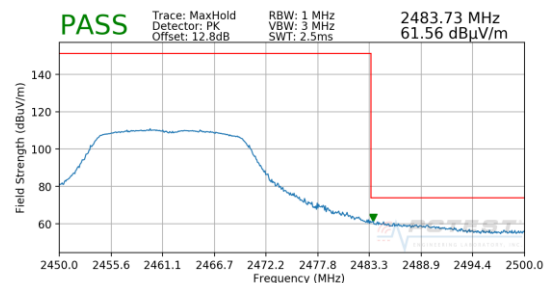
Plot 7-76. Radiated Restricted Upper Band Edge Measurement SISO ANT1 (Peak)
