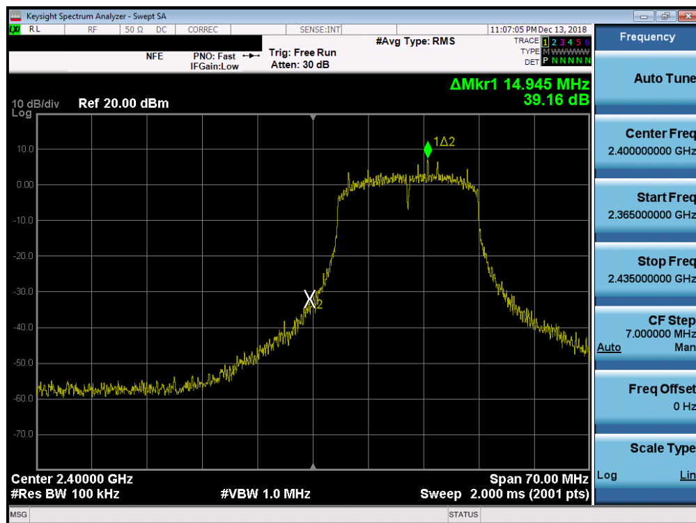
Plot 7-41. Band Edge Plot SISO ANT1 (802.11n (2.4GHz) – Ch. 1)
