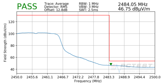
Plot 7-89. Radiated Restricted Upper Band Edge Measurement CDD (Average)
