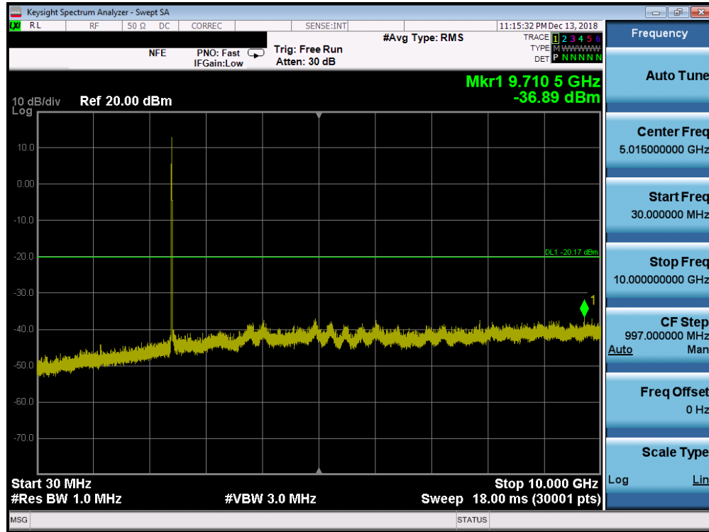
Plot 7-55. Conducted Spurious Plot SISO ANT2 (802.11b – Ch. 1)
