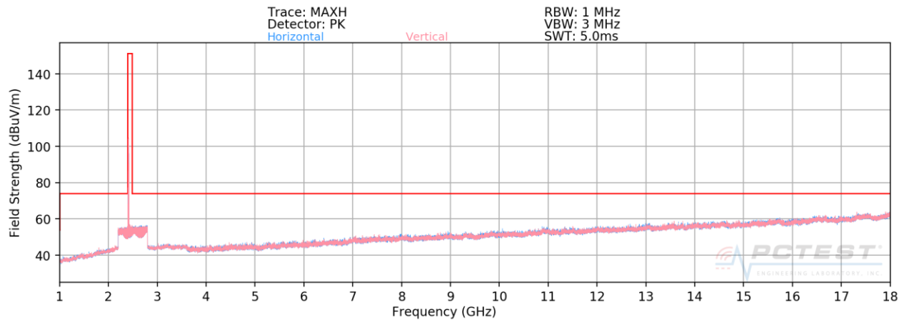
Plot 7-65. Radiated Spurious Plot above 1GHz SISO ANT2 (802.11b – Ch. 1)
