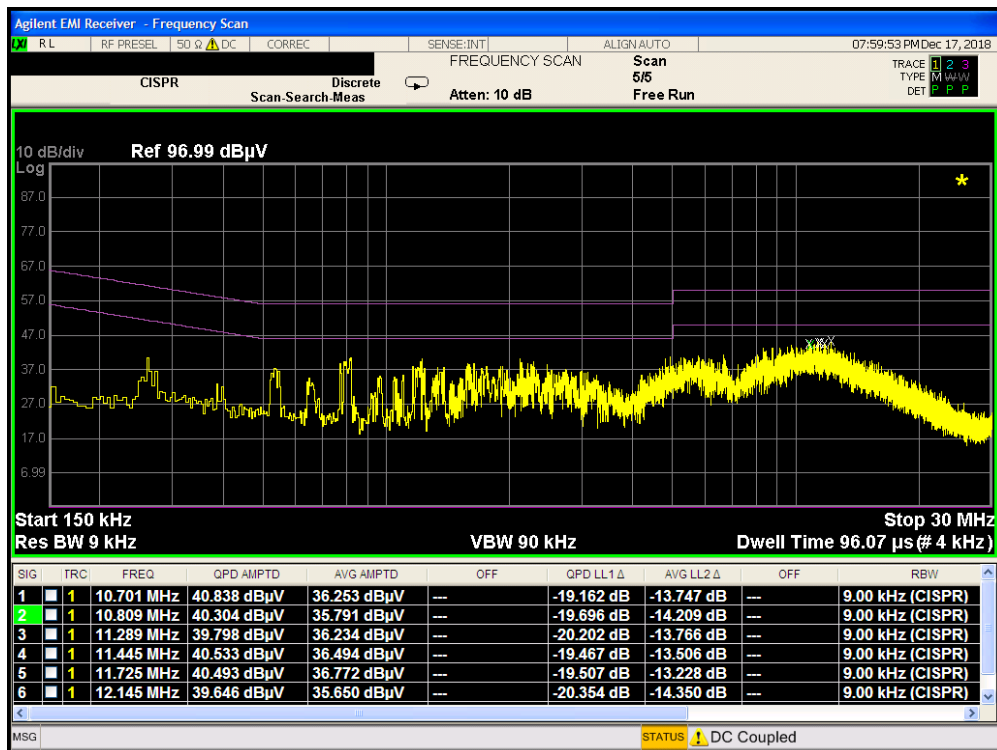
Plot 7-103. Line Conducted Plot with 802.11b (L1)
