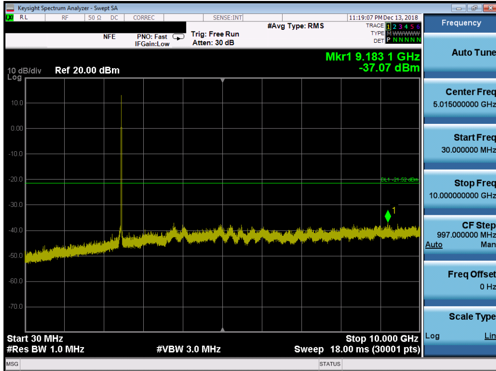
Plot 7-59. Conducted Spurious Plot SISO ANT2 (802.11b – Ch. 11)
