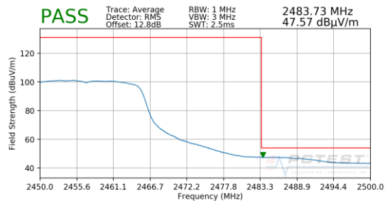
Plot 7-73. Radiated Restricted Upper Band Edge Measurement SISO ANT1 (Average)
