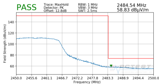
Plot 7-98. Radiated Restricted Upper Band Edge Measurement MIMO (Peak)
