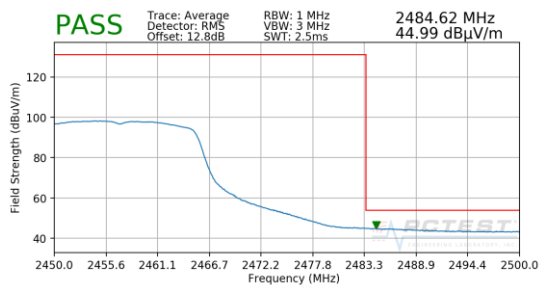
Plot 7-81. Radiated Restricted Upper Band Edge Measurement SISO ANT2 (Average)
