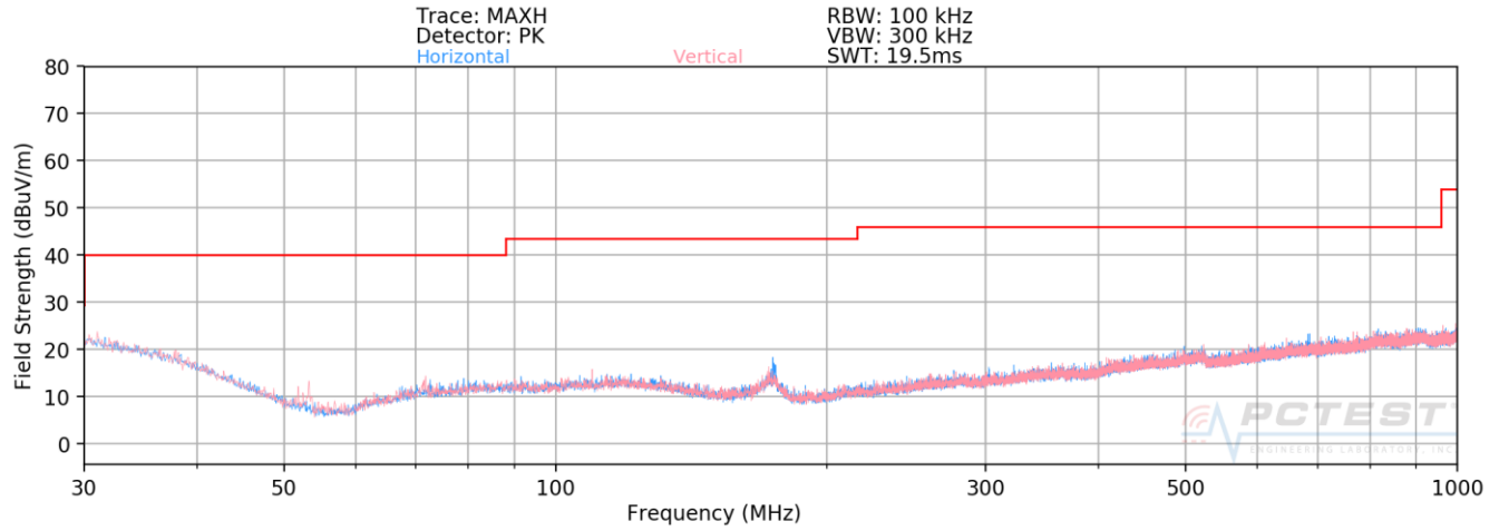
Plot 7-102. Radiated Spurious Plot below 1GHz SISO ANT2
