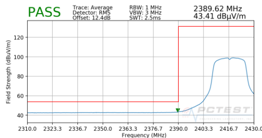
Plot 7-79. Radiated Restricted Lower Band Edge Measurement SISO ANT2 (Average)
