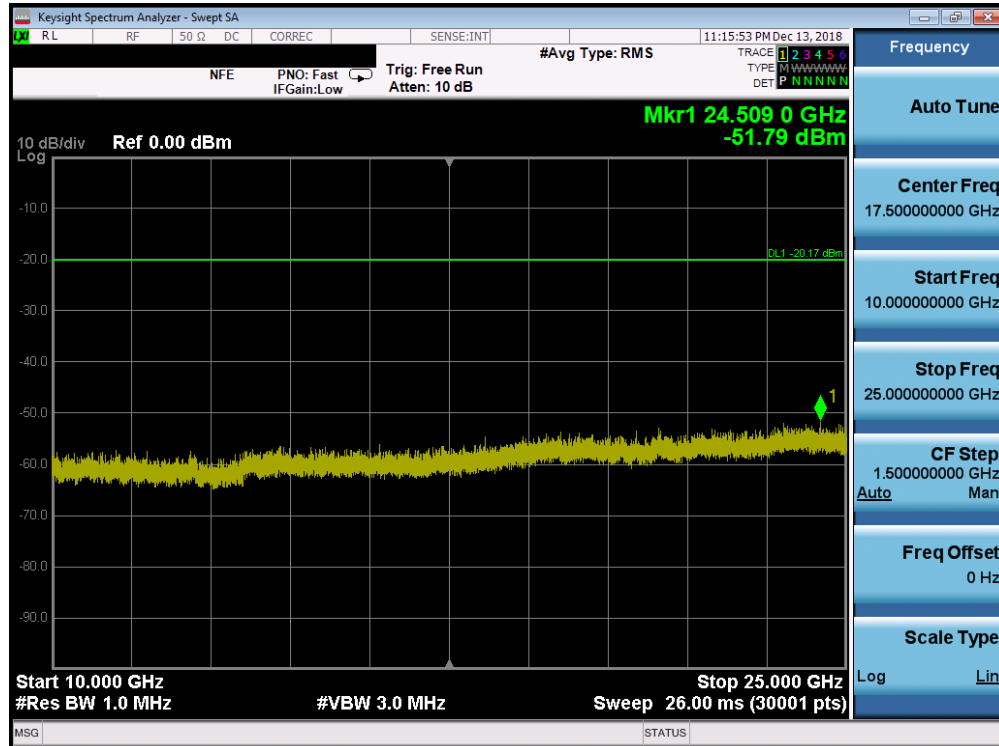
Plot 7-56. Conducted Spurious Plot SISO ANT2 (802.11b – Ch. 1)
