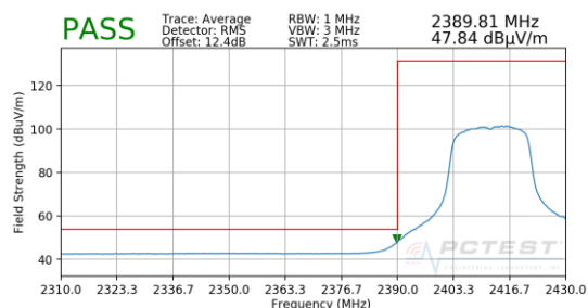
Plot 7-93. Radiated Restricted Lower Band Edge Measurement MIMO (Average)
