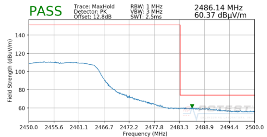
Plot 7-74. Radiated Restricted Upper Band Edge Measurement SISO ANT1 (Peak)
