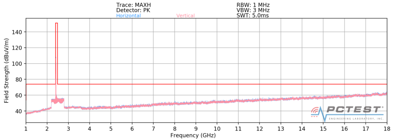
Plot 7-61. Radiated Spurious Plot above 1GHz SISO ANT1 (802.11b – Ch. 1)
