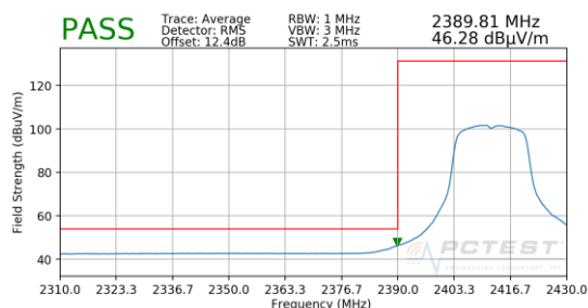
Plot 7-69. Radiated Restricted Lower Band Edge Measurement SISO ANT1 (Average)
