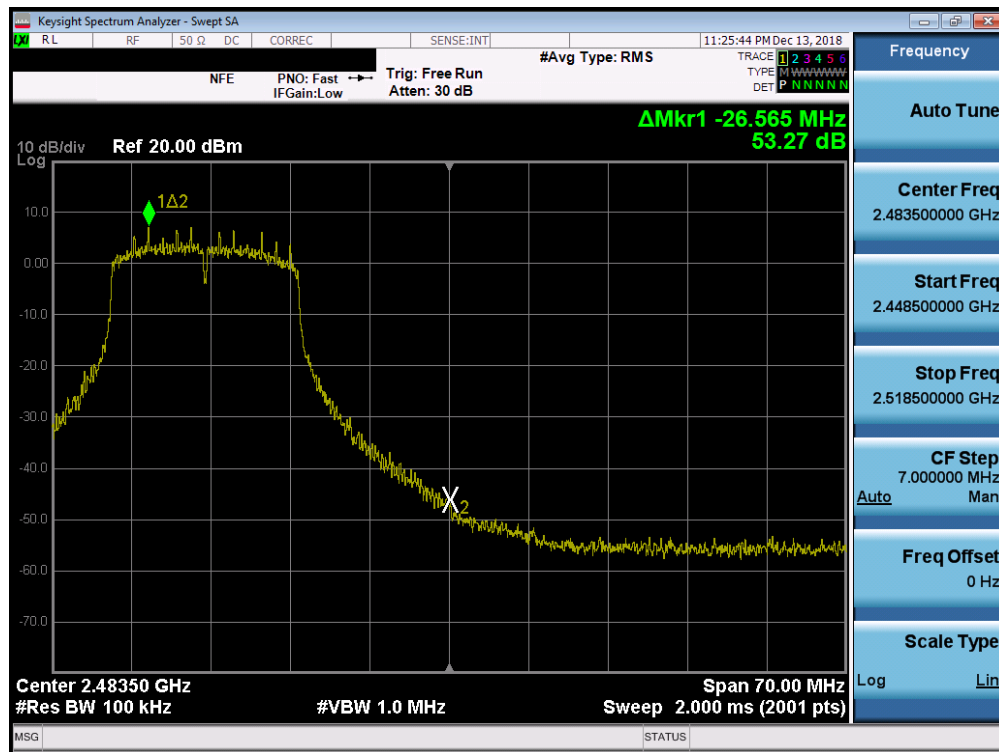
Plot 7-46. Band Edge Plot SISO ANT2 (802.11g - Ch. 11)
