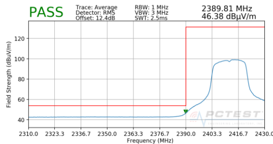
Plot 7-77. Radiated Restricted Lower Band Edge Measurement SISO ANT2 (Average)
