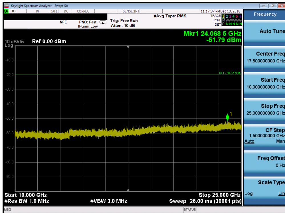
Plot 7-58. Conducted Spurious Plot SISO ANT2 (802.11b – Ch. 6)
