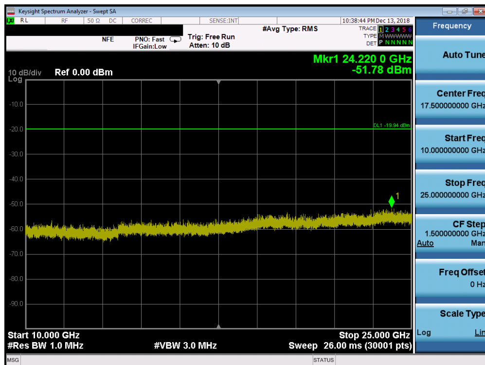
Plot 7-50. Conducted Spurious Plot SISO ANT1 (802.11b – Ch. 1)
