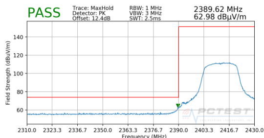
Plot 7-96. Radiated Restricted Lower Band Edge Measurement MIMO (Peak)
