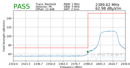
Plot 7-94. Radiated Restricted Lower Band Edge Measurement MIMO (Peak)
