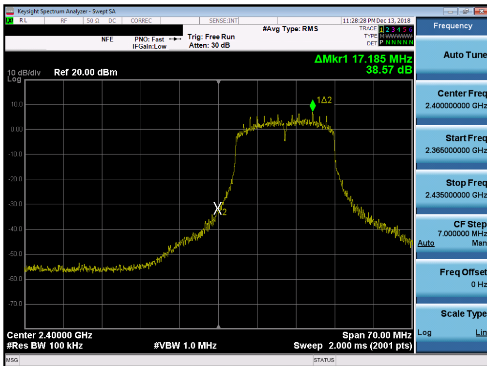
Plot 7-47. Band Edge Plot SISO ANT2 (802.11n (2.4GHz) – Ch. 1)
