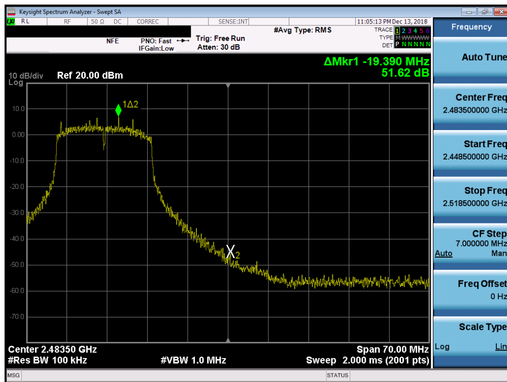
Plot 7-40. Band Edge Plot SISO ANT1 (802.11g - Ch. 11)
