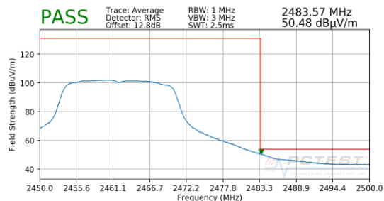
Plot 7-91. Radiated Restricted Upper Band Edge Measurement CDD (Average)
