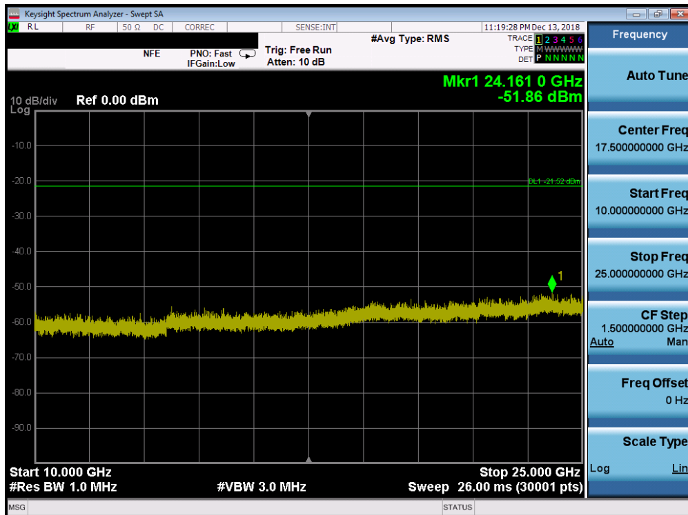
Plot 7-60. Conducted Spurious Plot SISO ANT2 (802.11b – Ch. 11)
