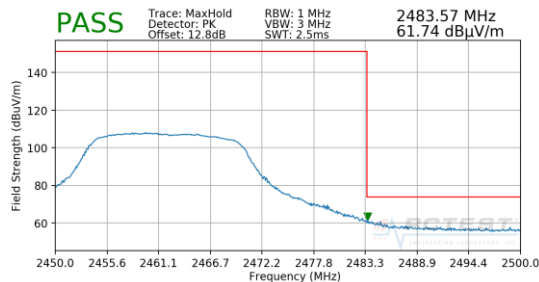
Plot 7-84. Radiated Restricted Upper Band Edge Measurement SISO ANT2 (Peak)
