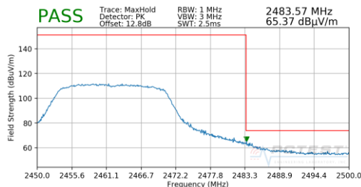
Plot 7-100. Radiated Restricted Upper Band Edge Measurement MIMO (Peak)
