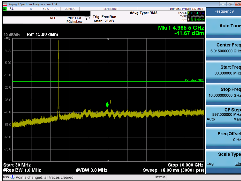
Plot 7-51. Conducted Spurious Plot SISO ANT1 (802.11b – Ch. 6)
