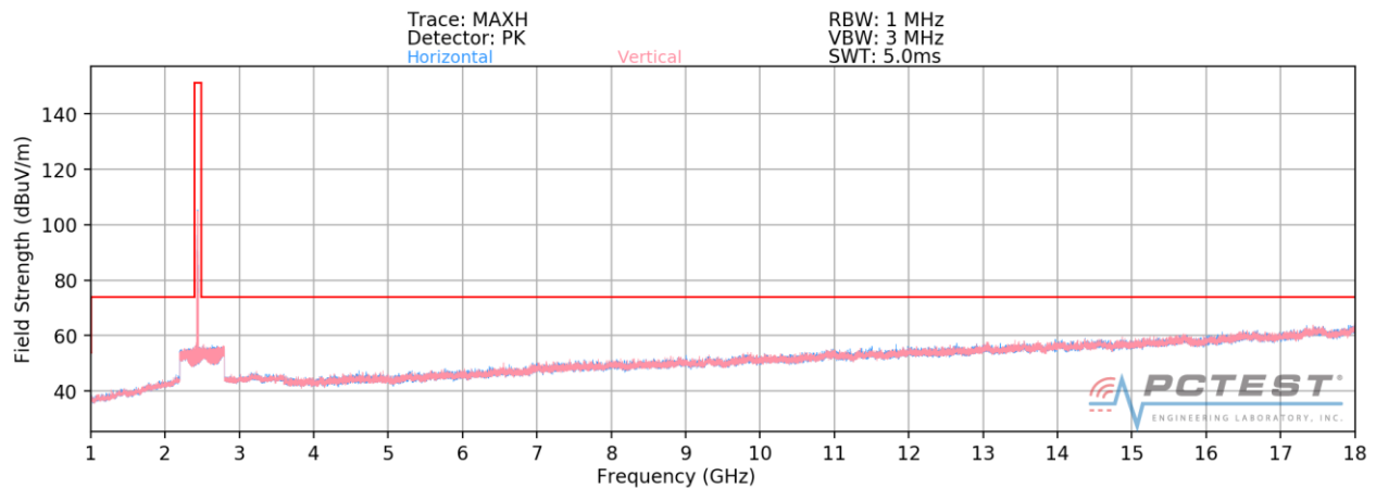
Plot 7-66. Radiated Spurious Plot above 1GHz SISO ANT2 (802.11b – Ch. 6)
