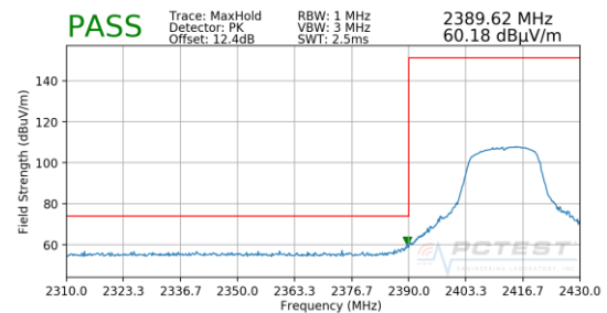
Plot 7-78. Radiated Restricted Lower Band Edge Measurement SISO ANT2 (Peak)
