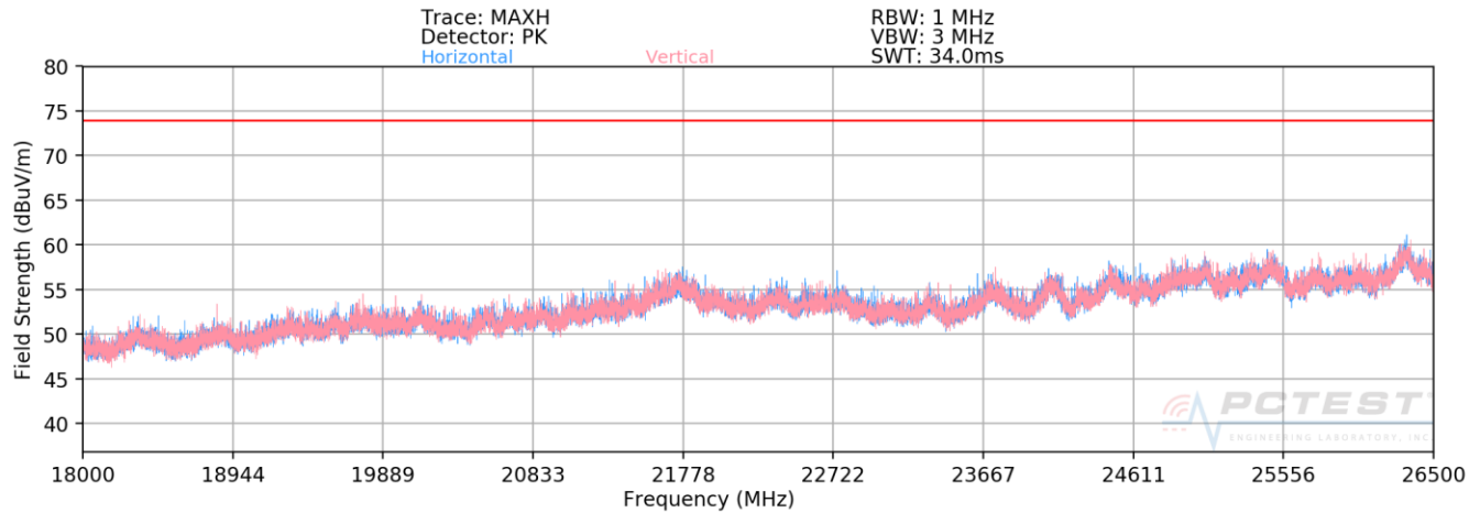
Plot 7-64. Radiated Spurious Plot above 18GHz SISO ANT1
