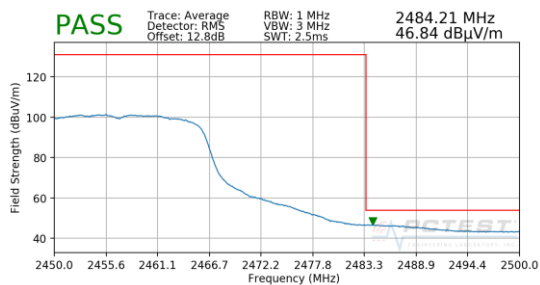
Plot 7-97. Radiated Restricted Upper Band Edge Measurement MIMO (Average)
