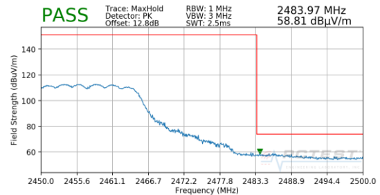
Plot 7-90. Radiated Restricted Upper Band Edge Measurement CDD (Peak)
