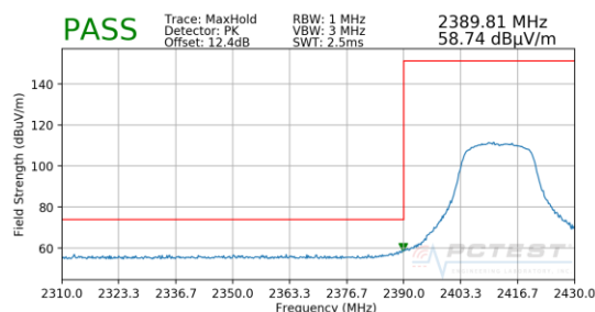
Plot 7-70. Radiated Restricted Lower Band Edge Measurement SISO ANT1 (Peak)
