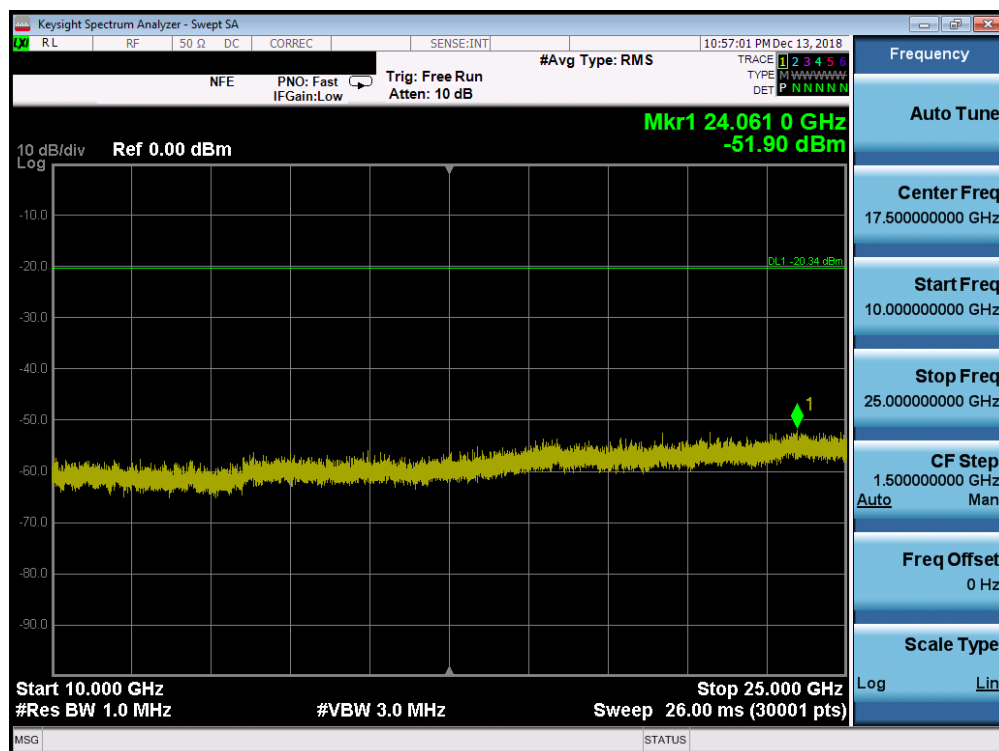
Plot 7-54. Conducted Spurious Plot SISO ANT1 (802.11b – Ch. 11)
