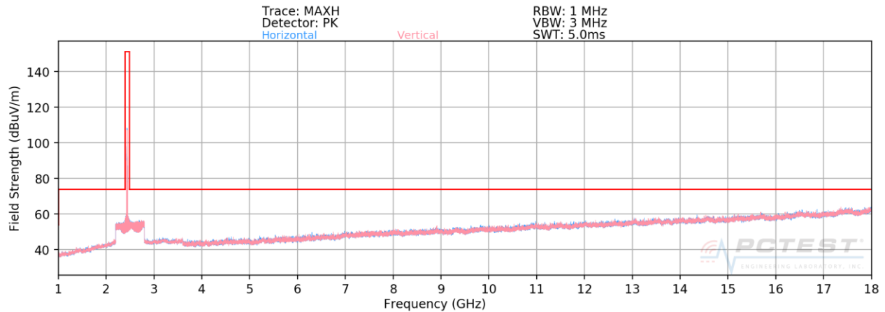
Plot 7-62. Radiated Spurious Plot above 1GHz SISO ANT1 (802.11b – Ch. 6)
