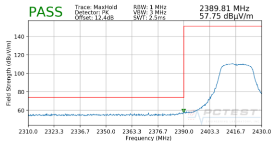
Plot 7-72. Radiated Restricted Lower Band Edge Measurement SISO ANT1 (Peak)
