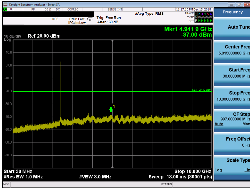
Plot 7-57. Conducted Spurious Plot SISO ANT2 (802.11b – Ch. 6)
