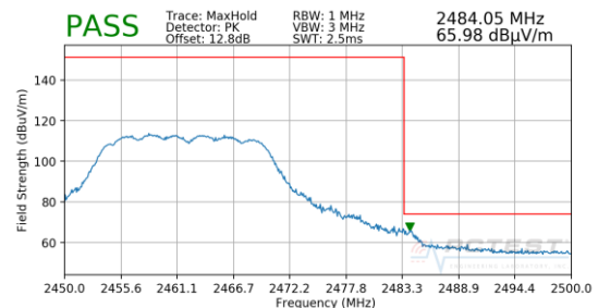
Plot 7-92. Radiated Restricted Upper Band Edge Measurement CDD (Peak)
