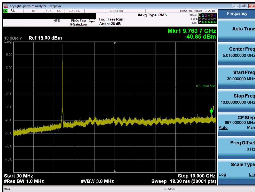
Plot 7-53. Conducted Spurious Plot SISO ANT1 (802.11b – Ch. 11)
