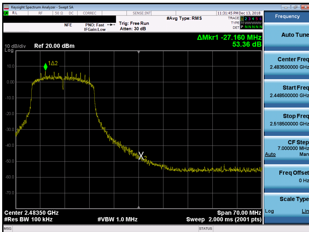
Plot 7-48. Band Edge Plot SISO ANT2 (802.11n (2.4GHz) – Ch. 11)
