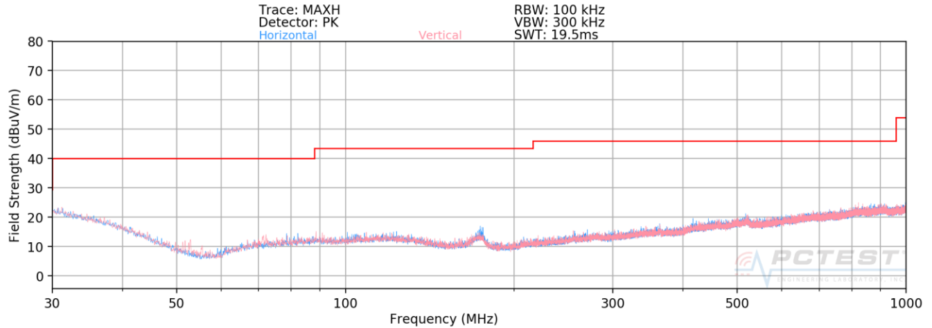
Plot 7-101. Radiated Spurious Plot below 1GHz SISO ANT1
