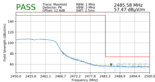
Plot 7-82. Radiated Restricted Upper Band Edge Measurement SISO ANT2 (Peak)
