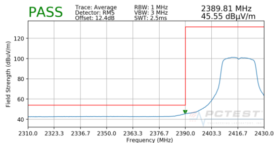
Plot 7-71. Radiated Restricted Lower Band Edge Measurement SISO ANT1 (Average)
