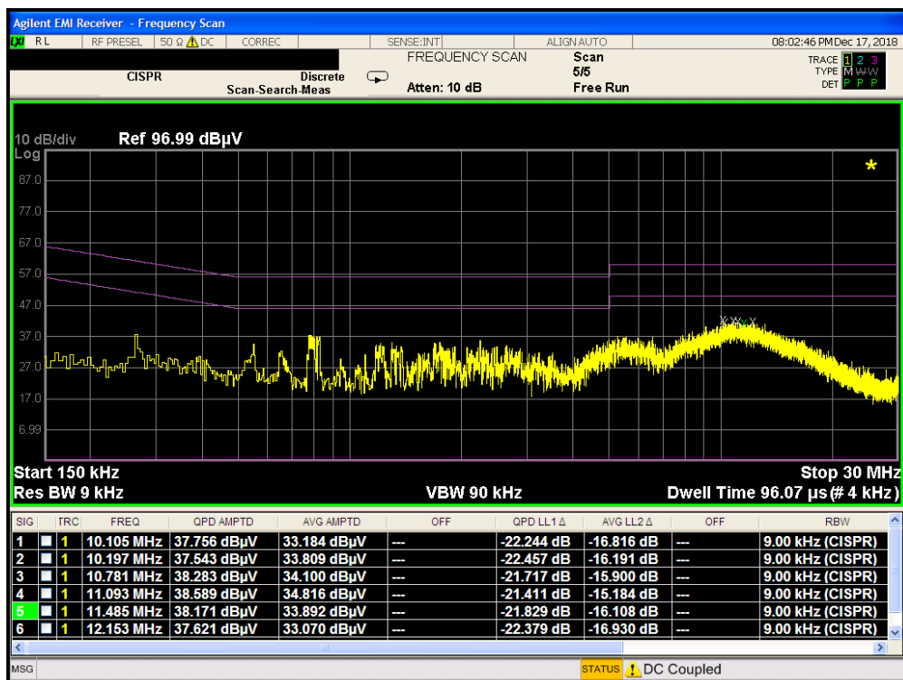
Plot 7-104. Line Conducted Plot with 802.11b (N)
