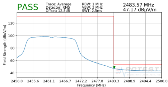
Plot 7-83. Radiated Restricted Upper Band Edge Measurement SISO ANT2 (Average)
