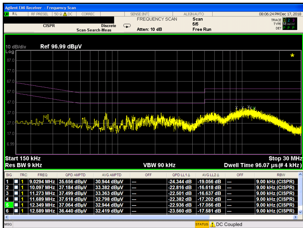
Plot 7-241. Line Conducted Plot with 802.11a UNII Band 1 (N)
