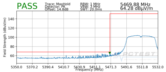
Plot 7-202. Radiated Lower Band Edge Plot SISO ANT2 (Peak – UNII Band 2C)
