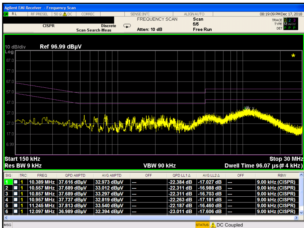
Plot 7-245. Line Conducted Plot with 802.11a UNII Band 2C (N)
