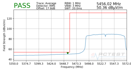
Plot 7-228. Radiated Lower Band Edge Plot MIMO (Average – UNII Band 2C)
