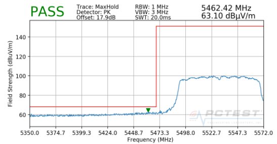
Plot 7-229. Radiated Lower Band Edge Plot MIMO (Peak – UNII Band 2C)
