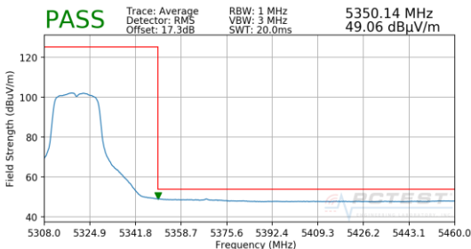
Plot 7-233. Radiated Upper Band Edge Plot MIMO (Average – UNII Band 2A)
