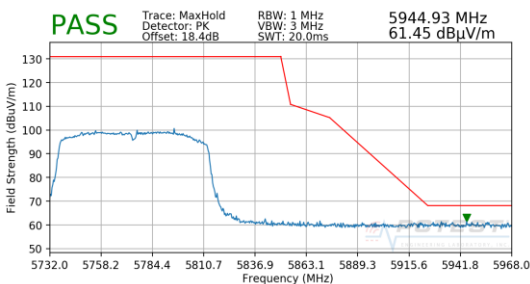
Plot 7-210. Radiated Upper Band Edge Plot SISO ANT2 (Peak – UNII Band 3)
