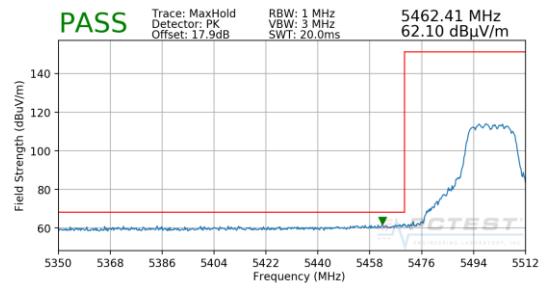
Plot 7-236. Radiated Lower Band Edge Plot MIMO (Peak – UNII Band 2C)
