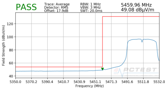
Plot 7-201. Radiated Lower Band Edge Plot SISO ANT2 (Average – UNII Band 2C)
