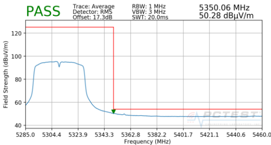
Plot 7-199. Radiated Upper Band Edge Plot SISO ANT2 (Average – UNII Band 2A)
