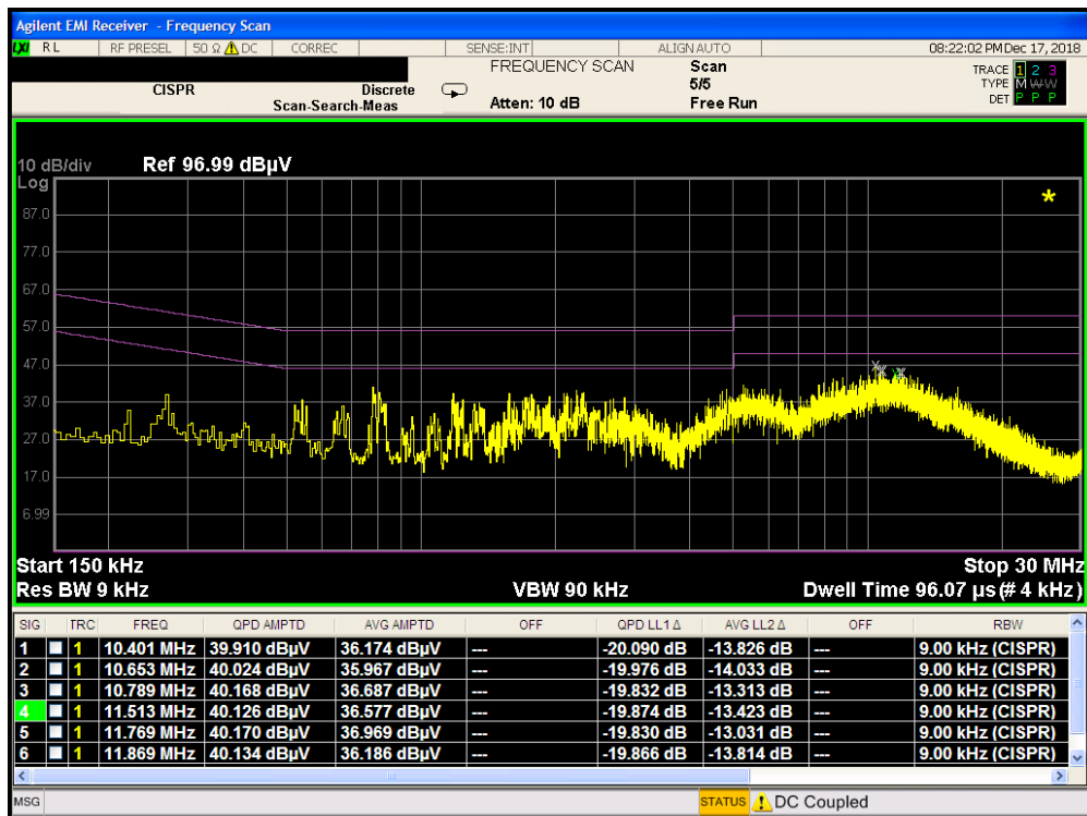
Plot 7-244. Line Conducted Plot with 802.11a UNII Band 2C (L1)
