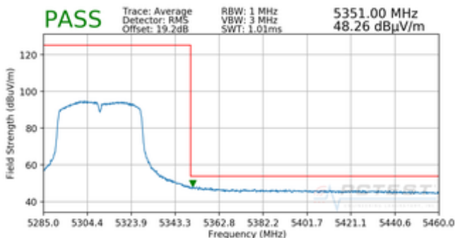
Plot 7-220. Radiated Upper Band Edge Plot MIMO (Average – UNII Band 2A)
