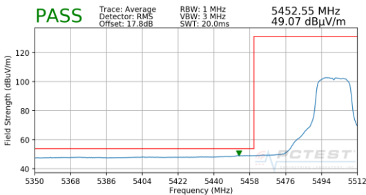
Plot 7-235. Radiated Lower Band Edge Plot MIMO (Average – UNII Band 2C)
