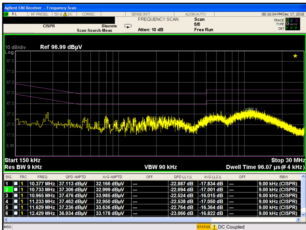
Plot 7-243. Line Conducted Plot with 802.11a UNII Band 2A (N)
