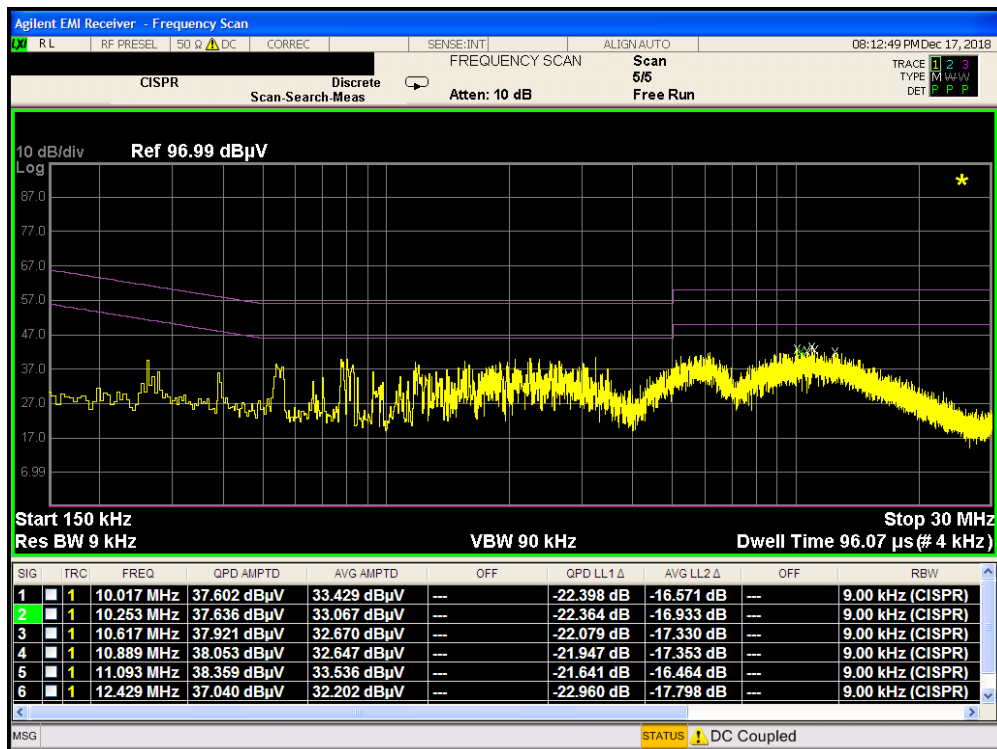
Plot 7-242. Line Conducted Plot with 802.11a UNII Band 2A (L1)
