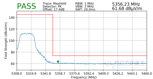
Plot 7-234. Radiated Upper Band Edge Plot MIMO (Peak – UNII Band 2A)
