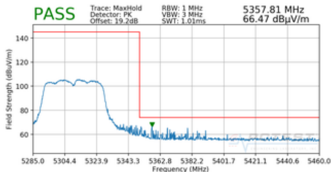
Plot 7-221. Radiated Upper Band Edge Plot MIMO (Peak – UNII Band 2A)
