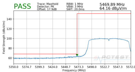
Plot 7-209. Radiated Lower Band Edge Plot SISO ANT2 (Peak – UNII Band 2C)
