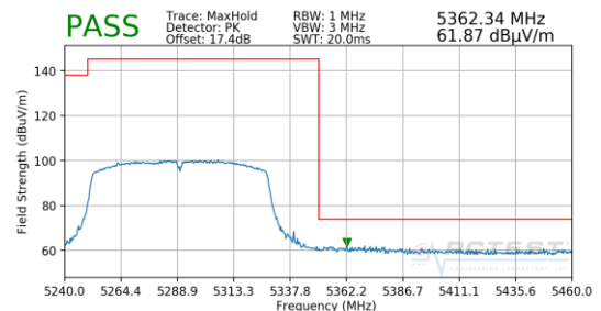
Plot 7-207. Radiated Upper Band Edge Plot SISO ANT2 (Peak – UNII Band 2A)
