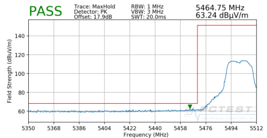
Plot 7-216. Radiated Lower Band Edge Plot MIMO (Peak – UNII Band 2C)
