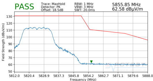
Plot 7-237. Radiated Upper Band Edge Plot MIMO (Peak – UNII Band 3)
