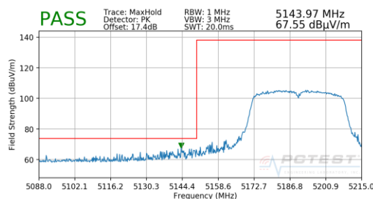
Plot 7-219. Radiated Lower Band Edge Plot MIMO (Peak – UNII Band 1)
