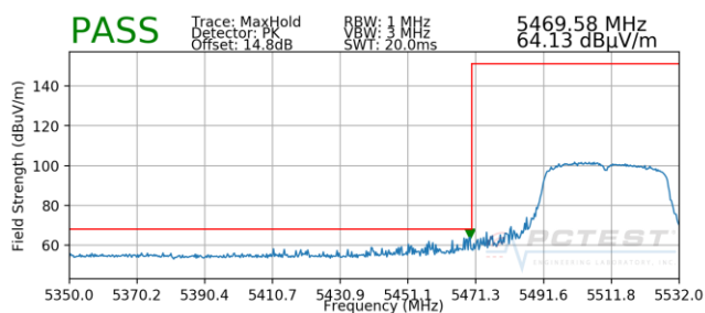
Plot 7-223. Radiated Lower Band Edge Plot MIMO (Peak – UNII Band 2C)
