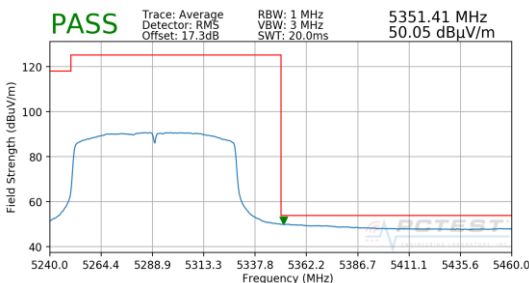
Plot 7-206. Radiated Upper Band Edge Plot SISO ANT2 (Average – UNII Band 2A)
