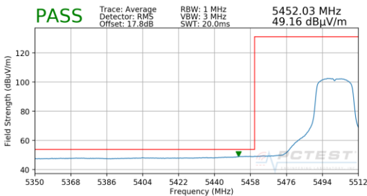
Plot 7-215. Radiated Lower Band Edge Plot MIMO (Average – UNII Band 2C)
