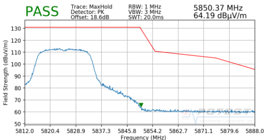
Plot 7-217. Radiated Upper Band Edge Plot MIMO (Peak – UNII Band 3)
