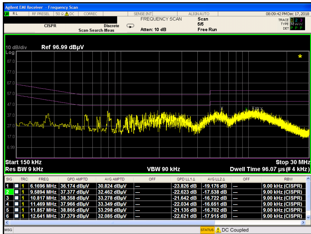
Plot 7-240. Line Conducted Plot with 802.11a UNII Band 1 (L1)
