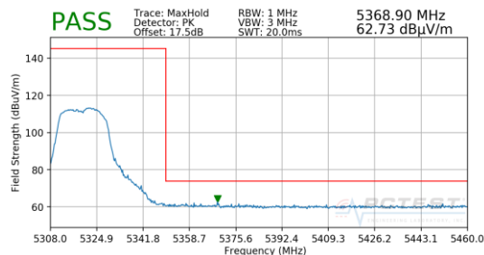
Plot 7-214. Radiated Upper Band Edge Plot MIMO (Peak – UNII Band 2A)
