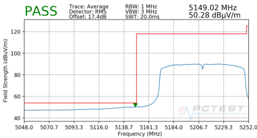
Plot 7-204. Radiated Lower Band Edge Plot SISO ANT2 (Average – UNII Band 1)
