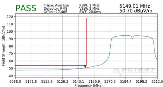
Plot 7-218. Radiated Lower Band Edge Plot MIMO (Average – UNII Band 1)
