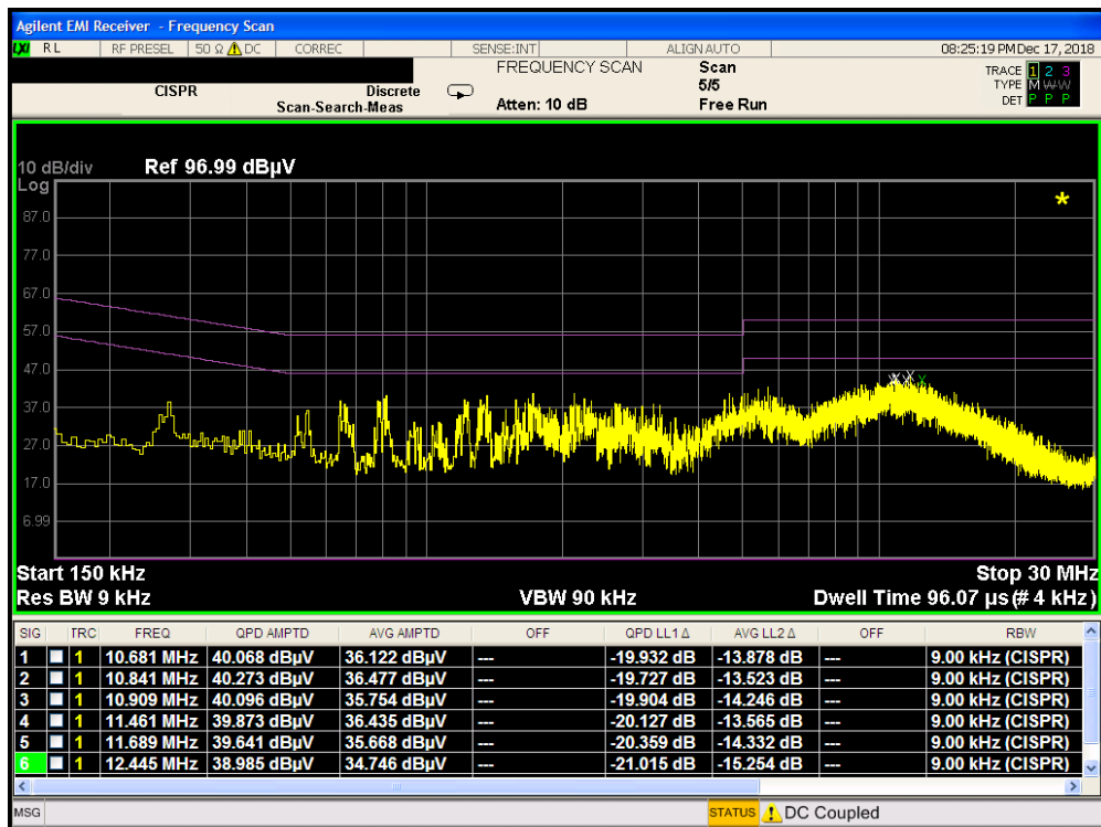
Plot 7-246. Line Conducted Plot with 802.11a UNII Band 3 (L1)
