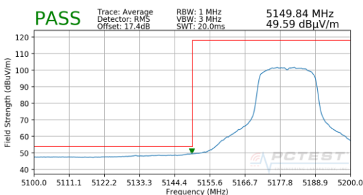
Plot 7-211. Radiated Lower Band Edge Plot MIMO (Average – UNII Band 1)
