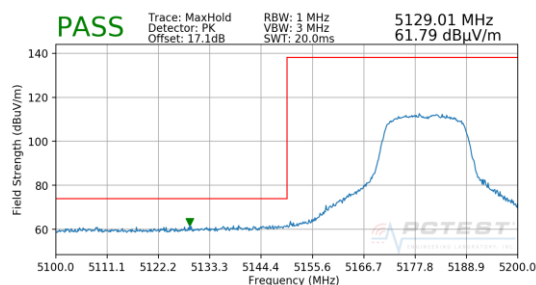
Plot 7-212. Radiated Lower Band Edge Plot MIMO (Peak – UNII Band 1)
