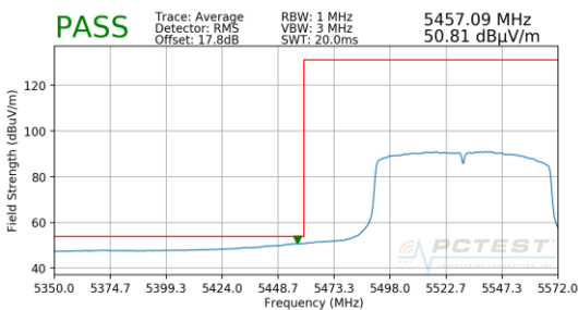
Plot 7-208. Radiated Lower Band Edge Plot SISO ANT2 (Average – UNII Band 2C)
