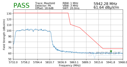
Plot 7-230. Radiated Upper Band Edge Plot MIMO (Peak – UNII Band 3)
