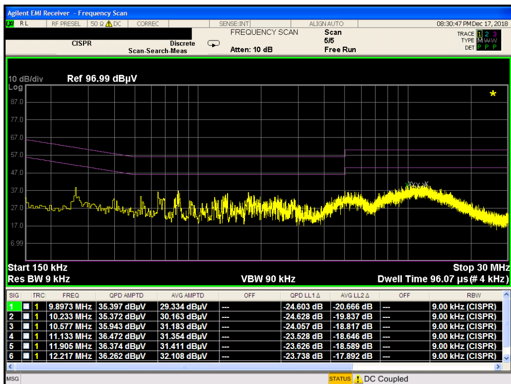
Plot 7-247. Line Conducted Plot with 802.11a UNII Band 3 (N)
