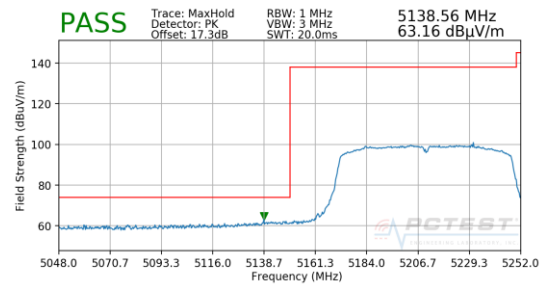
Plot 7-205. Radiated Lower Band Edge Plot SISO ANT2 (Peak – UNII Band 1)
