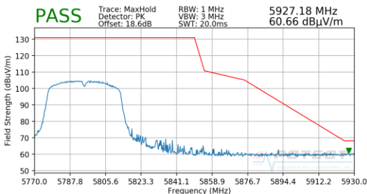
Plot 7-203. Radiated Upper Band Edge Plot SISO ANT2 (Peak – UNII Band 3)
