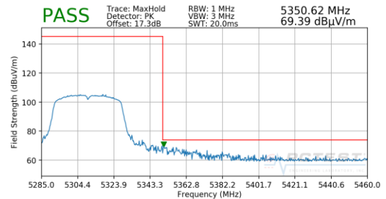
Plot 7-200. Radiated Upper Band Edge Plot SISO ANT2 (Peak – UNII Band 2A)
