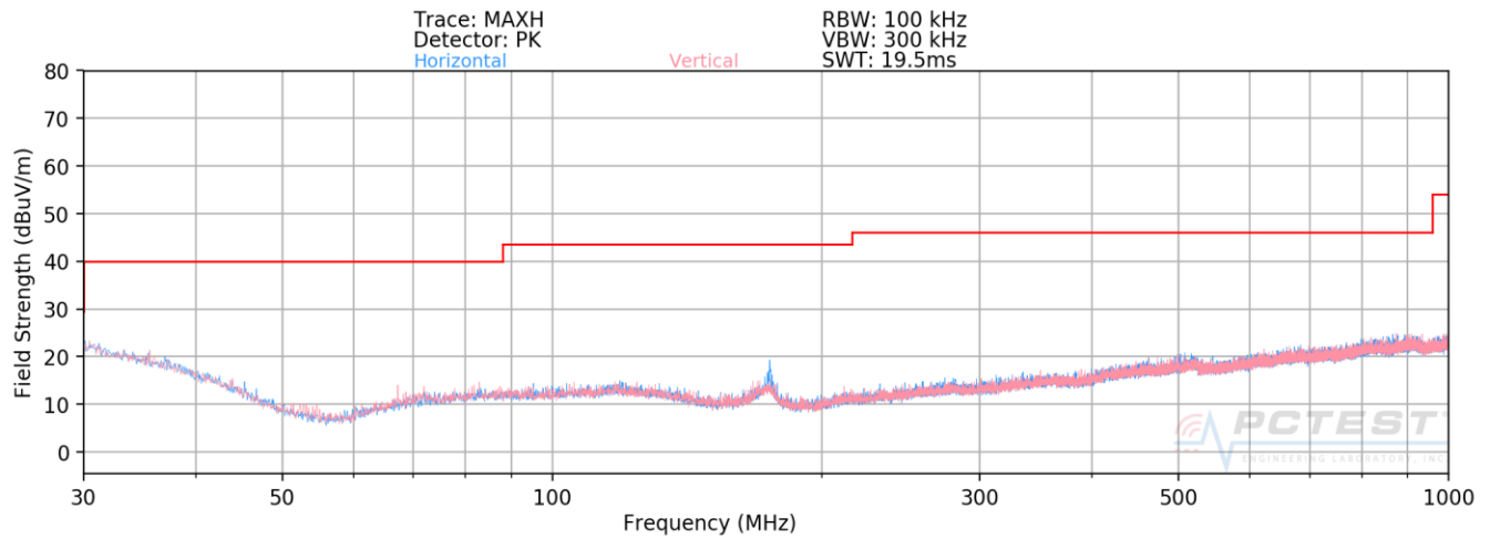
Plot 7-239. Radiated Spurious Plot below 1GHz SISO ANT2 (802.11a – U3 Ch. 157)
