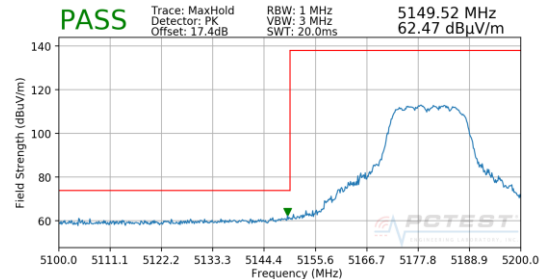
Plot 7-232. Radiated Lower Band Edge Plot MIMO (Peak – UNII Band 1)
