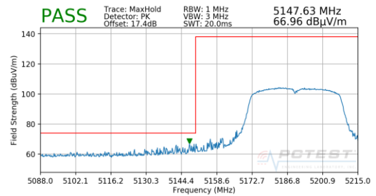
Plot 7-198. Radiated Lower Band Edge Plot SISO ANT2 (Peak – UNII Band 1)
