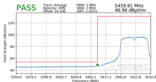
Plot 7-222. Radiated Lower Band Edge Plot MIMO (Average – UNII Band 2C)
