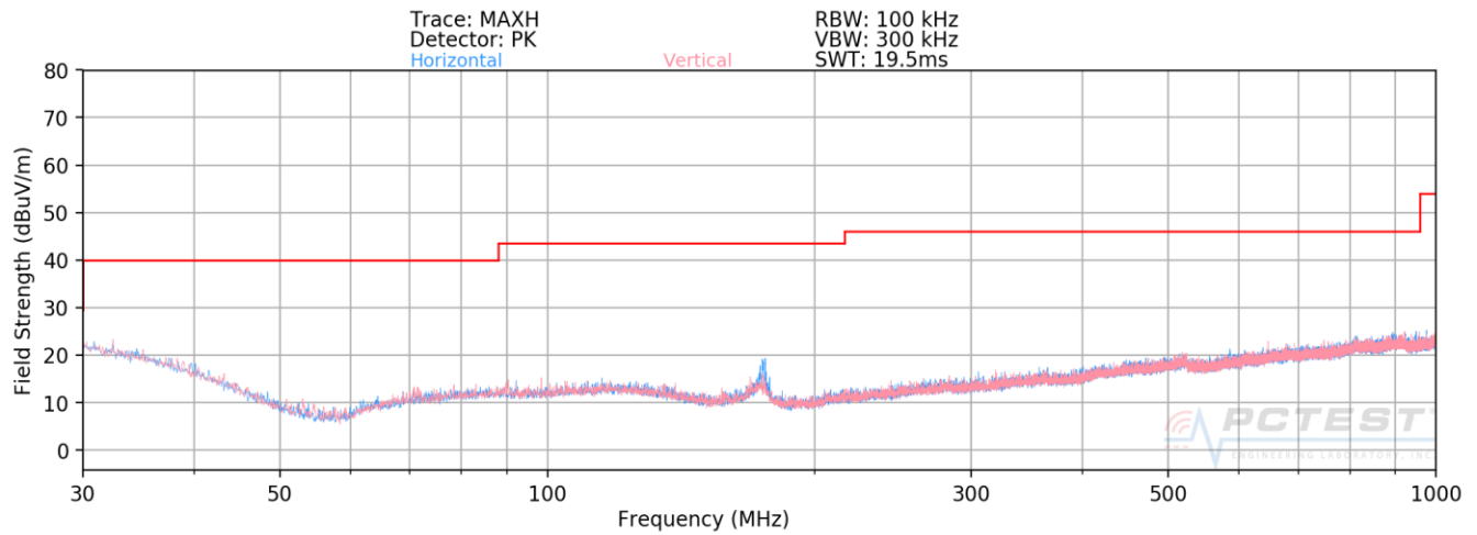
Plot 7-238. Radiated Spurious Plot below 1GHz SISO ANT1 (802.11a – U3 Ch. 157)
