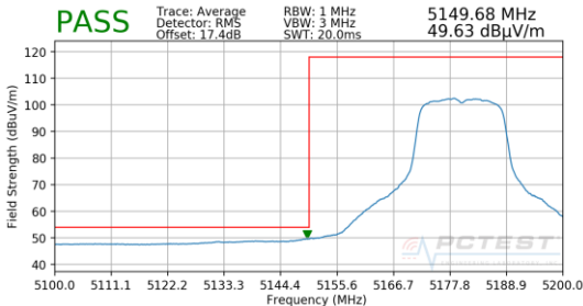
Plot 7-231. Radiated Lower Band Edge Plot MIMO (Average – UNII Band 1)
