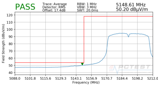
Plot 7-197. Radiated Lower Band Edge Plot SISO ANT2 (Average – UNII Band 1)
