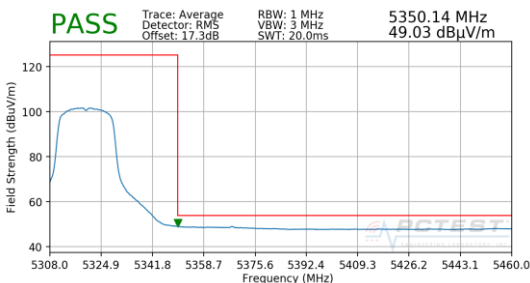
Plot 7-213. Radiated Upper Band Edge Plot MIMO (Average – UNII Band 2A)
