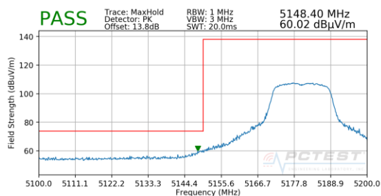
Plot 7-184. Radiated Lower Band Edge Plot SISO ANT1 (Peak – UNII Band 1)
