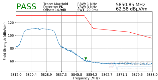
Plot 7-189. Radiated Upper Band Edge Plot SISO ANT1 (Peak – UNII Band 3)
