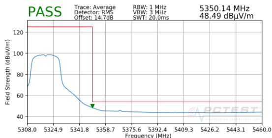
Plot 7-185. Radiated Upper Band Edge Plot SISO ANT1 (Average – UNII Band 2A)
