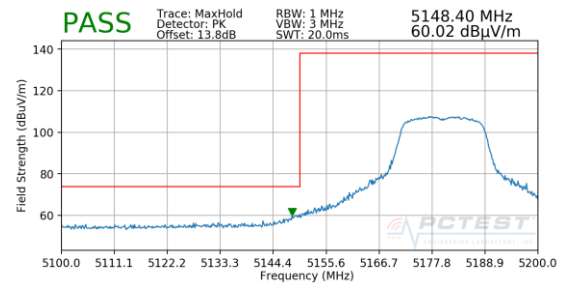
Plot 7-191. Radiated Lower Band Edge Plot SISO ANT2 (Peak – UNII Band 1)
