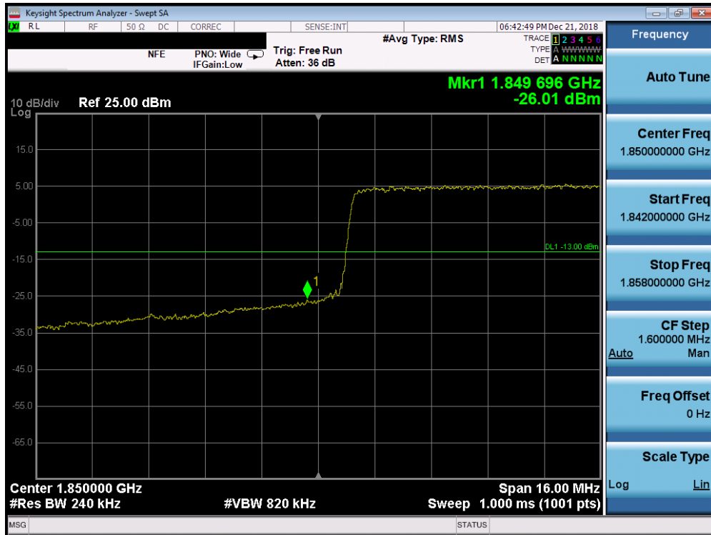
Plot 7-233. Lower Band Edge Plot (Band 25/2 – 20MHz QPSK - Full RB Configuration)
