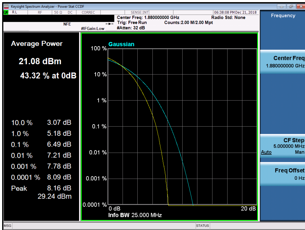
Plot 7-264. PAR Plot (Band 2/25 - 20.0MHz 64-QAM - Full RB Configuration)
