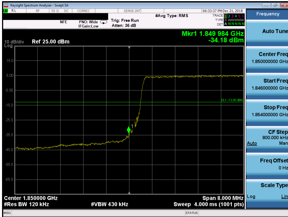
Plot 7-221. Lower Band Edge Plot (Band 25/2 - 10MHz QPSK - Full RB Configuration)
