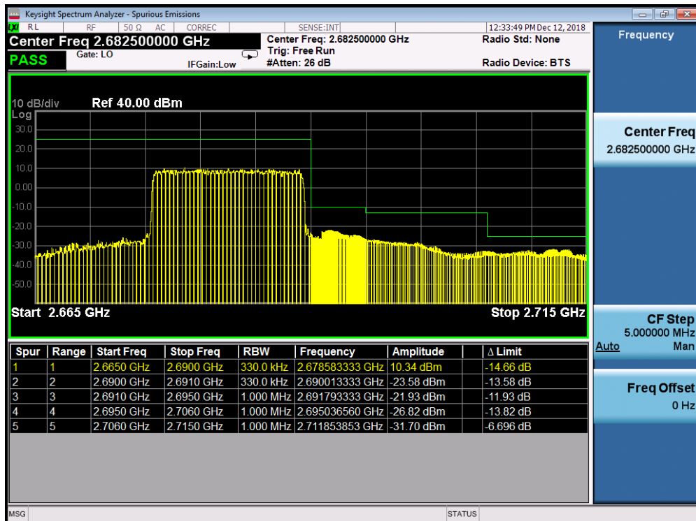
Plot 7-244. Upper ACP Plot (Band 41 PC2 - 15.0MHz QPSK - Full RB Configuration)
