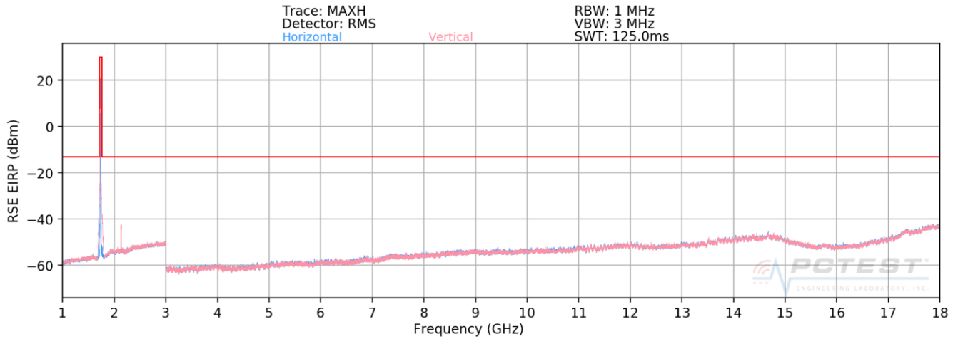
Plot 7-268. Radiated Spurious Plot above 1GHz (Band 66/4)
