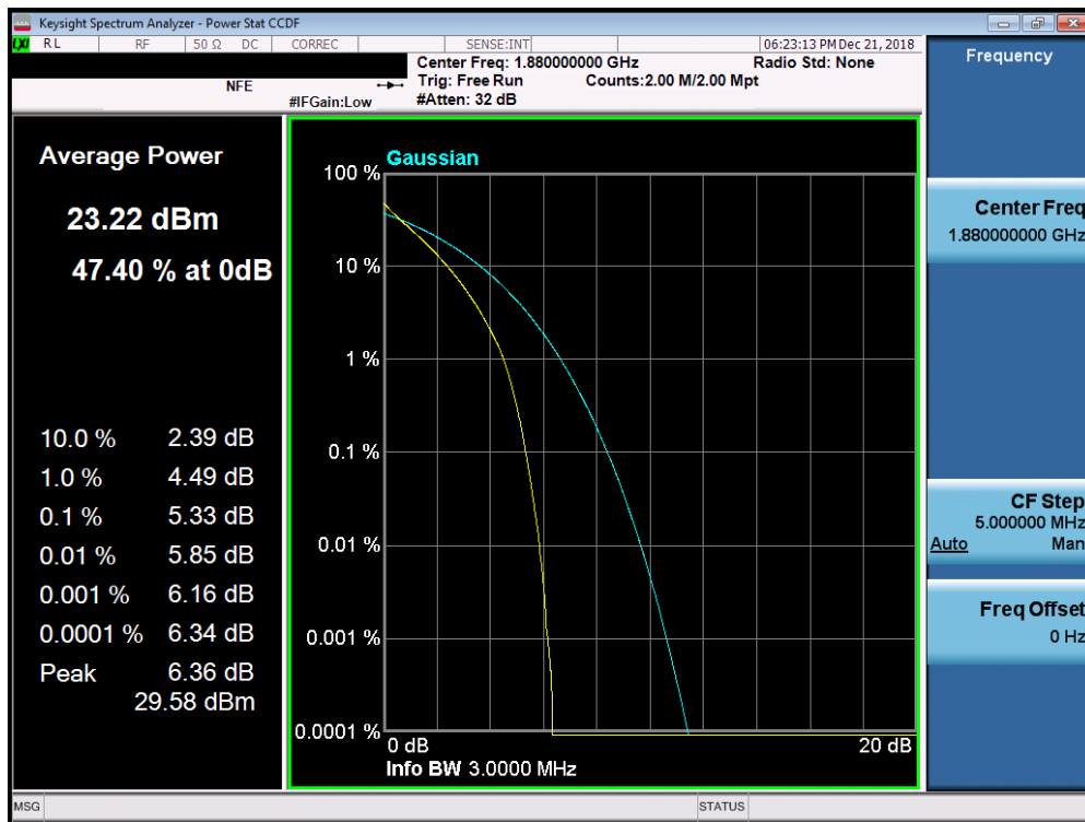
Plot 7-250. PAR Plot (Band 2/25 - 3.0MHz QPSK - Full RB Configuration)
