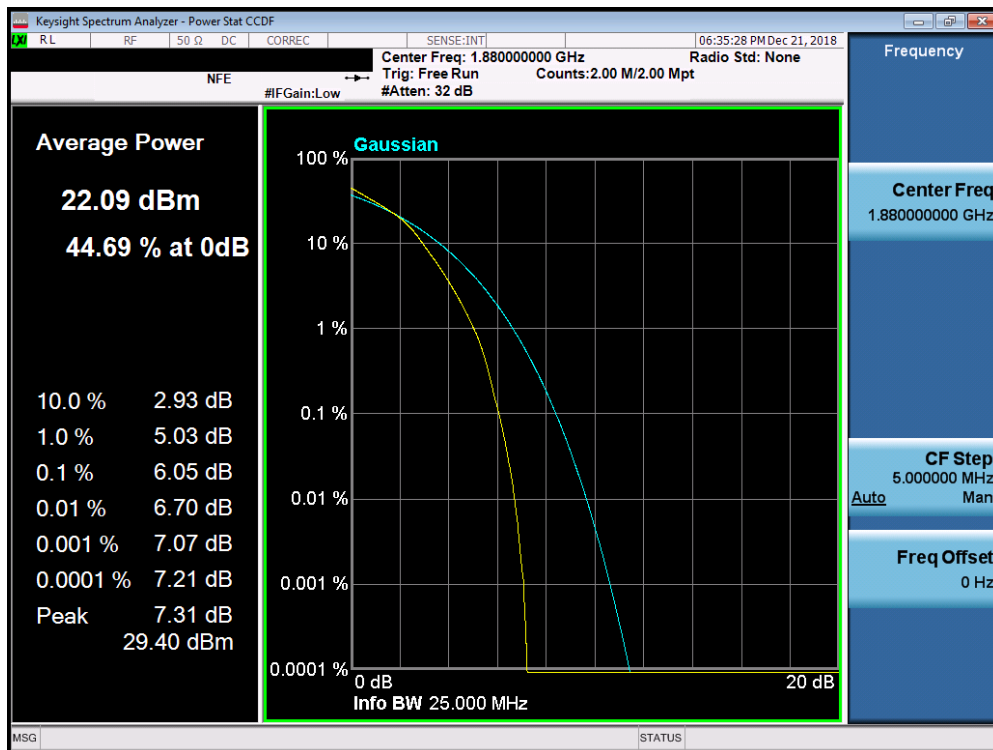
Plot 7-260. PAR Plot (Band 2/25 - 15.0MHz 16-QAM - Full RB Configuration)
