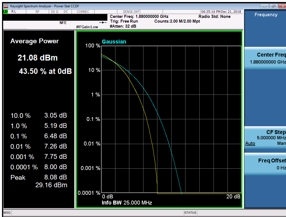
Plot 7-261. PAR Plot (Band 2/25 - 15.0MHz 64-QAM - Full RB Configuration)
