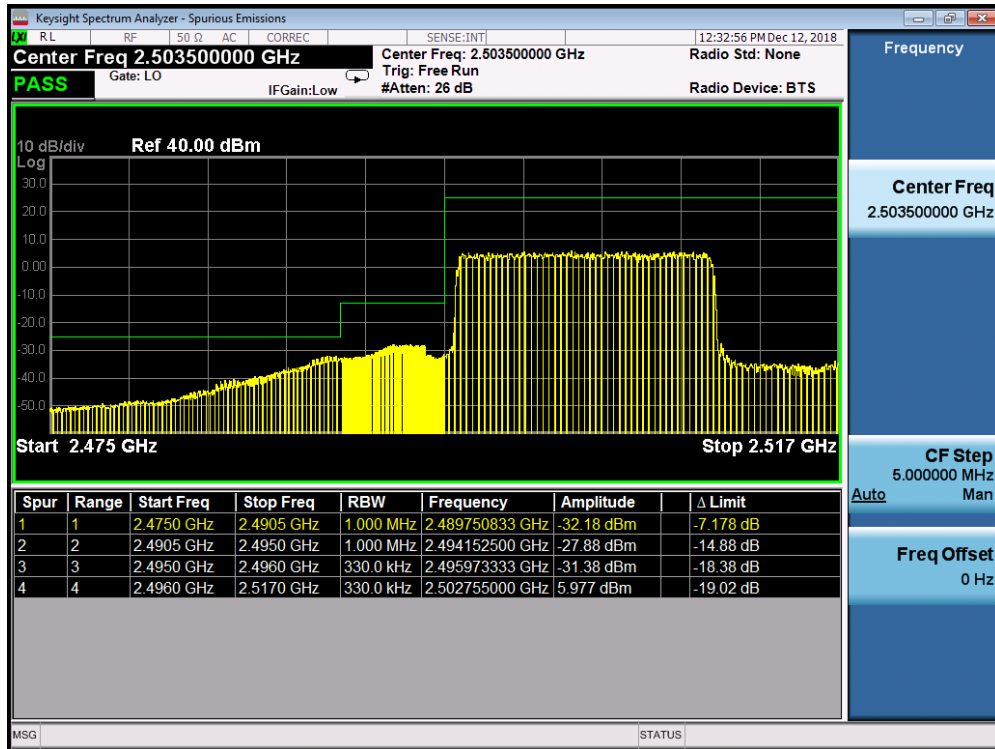
Plot 7-243. Lower ACP Plot at 2496 MHz (Band 41 PC2 - 15.0MHz QPSK - Full RB Configuration)
