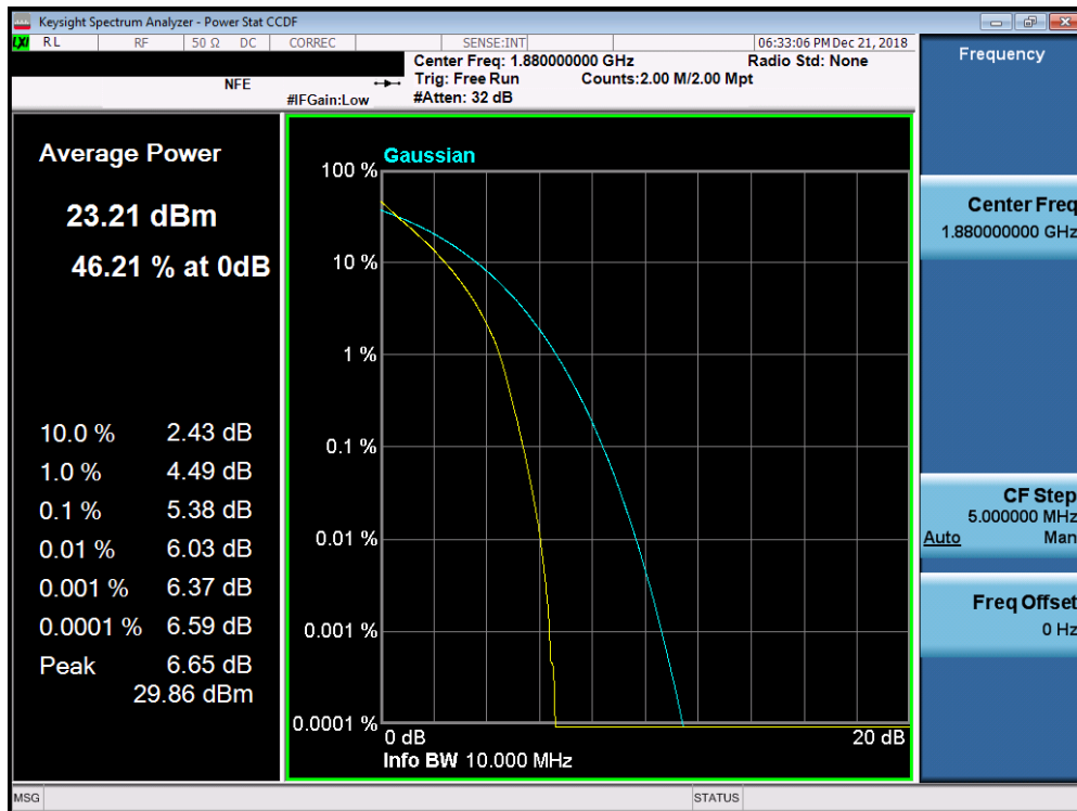
Plot 7-256. PAR Plot (Band 2/25 - 10.0MHz QPSK - Full RB Configuration)
