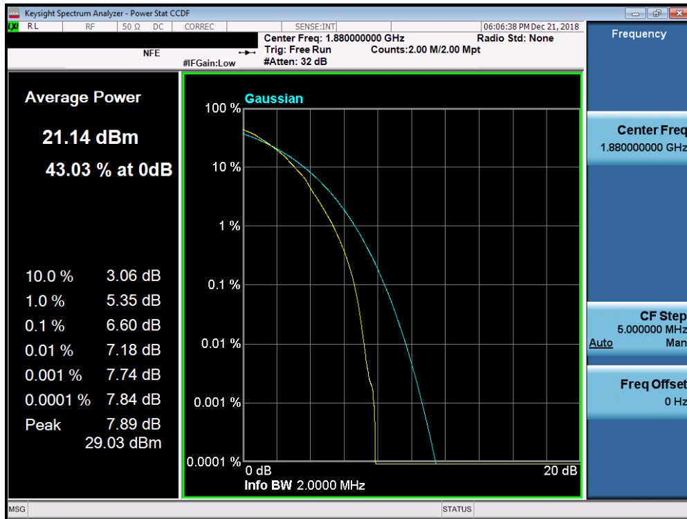
Plot 7-249. PAR Plot (Band 2/25 - 1.4MHz 64-QAM - Full RB Configuration)
