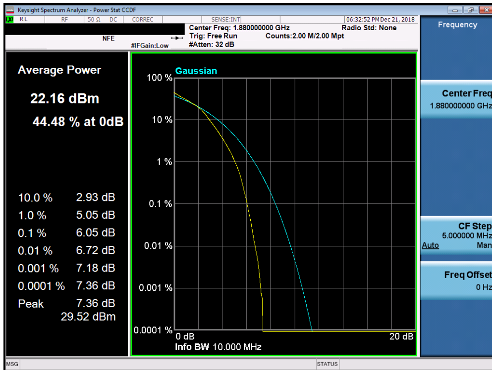
Plot 7-254. PAR Plot (Band 2/25 - 5.0MHz 16-QAM - Full RB Configuration)
