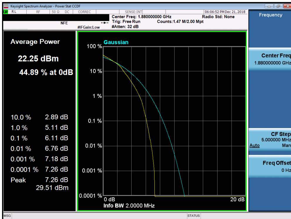
Plot 7-248. PAR Plot (Band 2/25 - 1.4MHz 16-QAM - Full RB Configuration)
