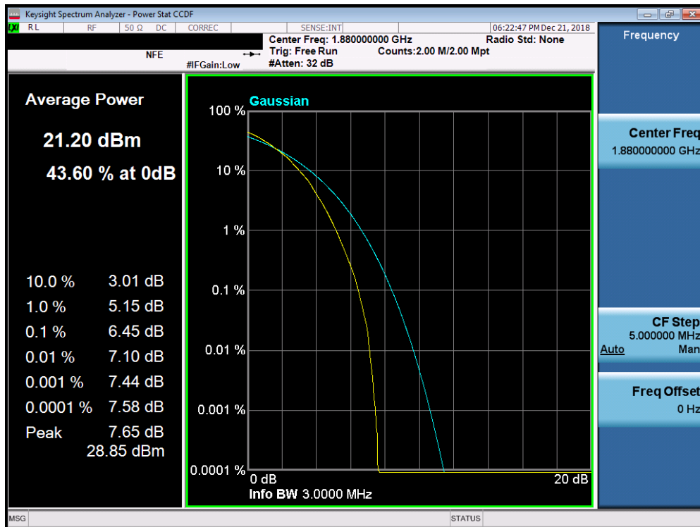
Plot 7-252. PAR Plot (Band 2/25 - 3.0MHz 64-QAM - Full RB Configuration)
