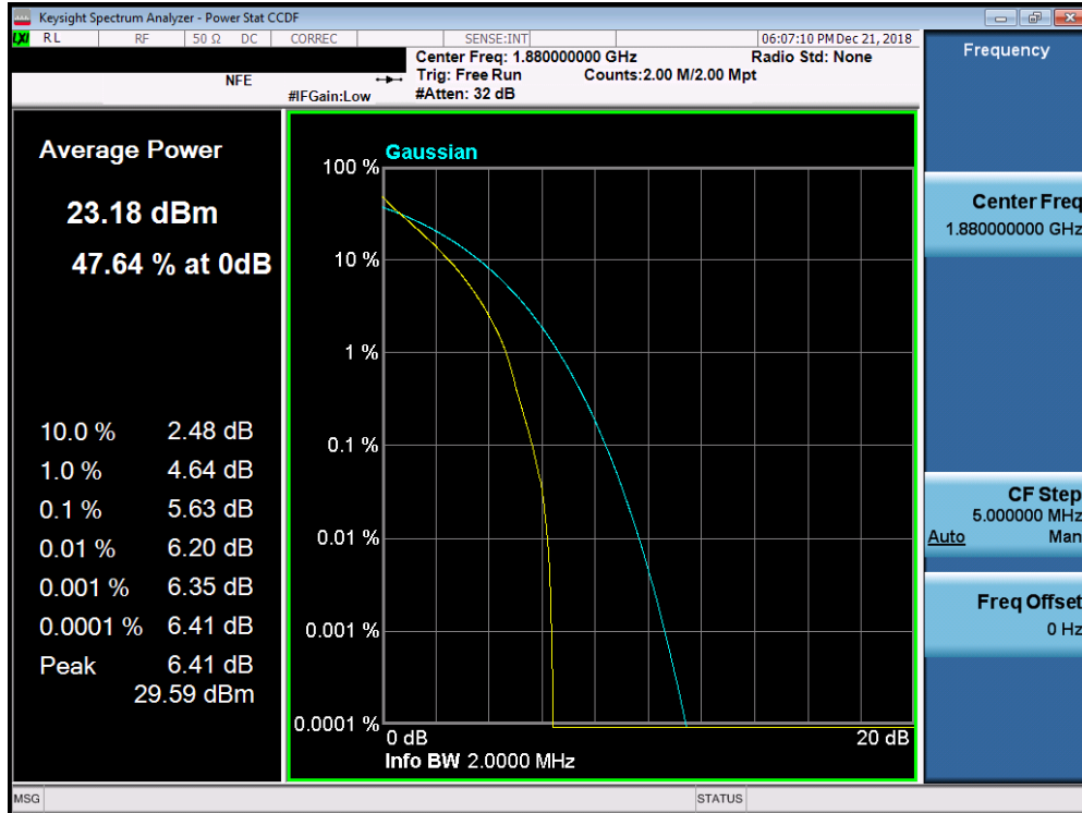
Plot 7-247. PAR Plot (Band 2/25- 1.4MHz QPSK - Full RB Configuration)
