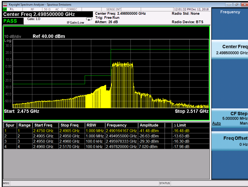
Plot 7-239. Lower ACP Plot at 2496 MHz (Band 41 PC2 - 5.0MHz QPSK - Full RB Configuration)
