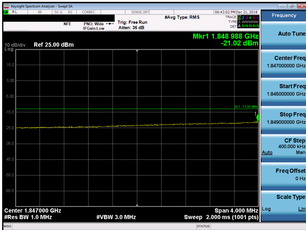
Plot 7-234. Lower Extended Band Edge Plot (Band 25/2 - 20MHz QPSK - Full RB Configuration)
