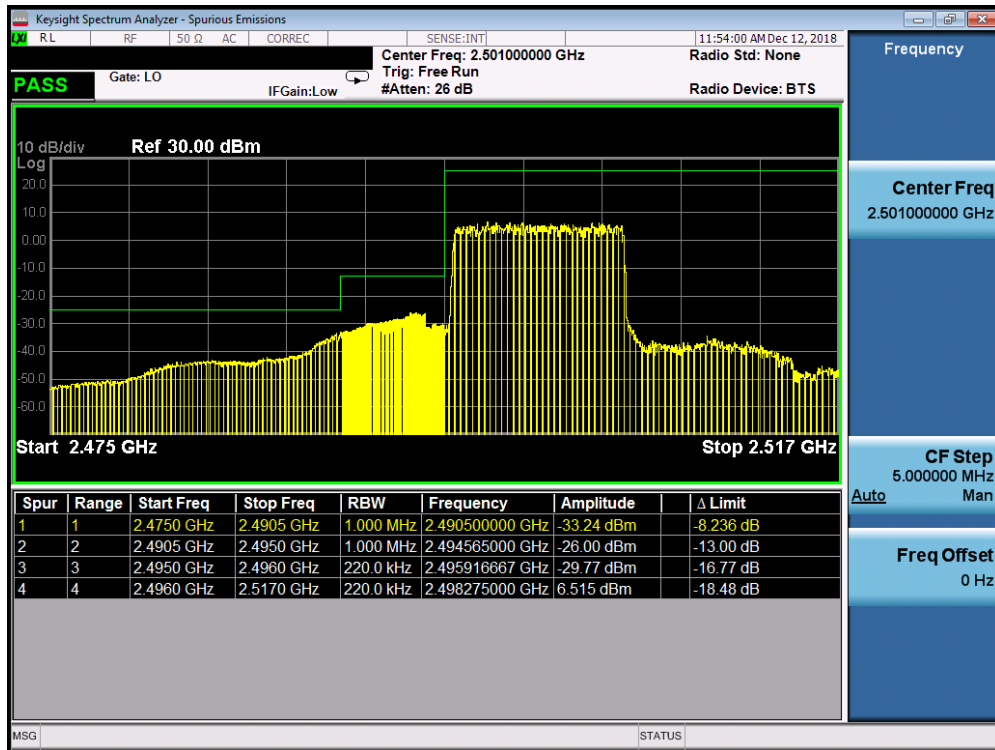
Plot 7-241. Lower ACP Plot at 2496 MHz (Band 41 PC2 - 10.0MHz QPSK - Full RB Configuration)
