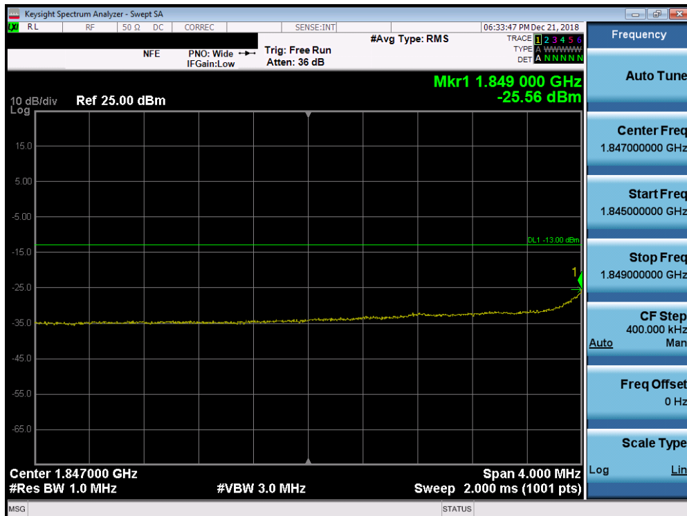
Plot 7-222. Lower Extended Band Edge Plot (Band 25/2 - 10MHz QPSK - Full RB Configuration)
