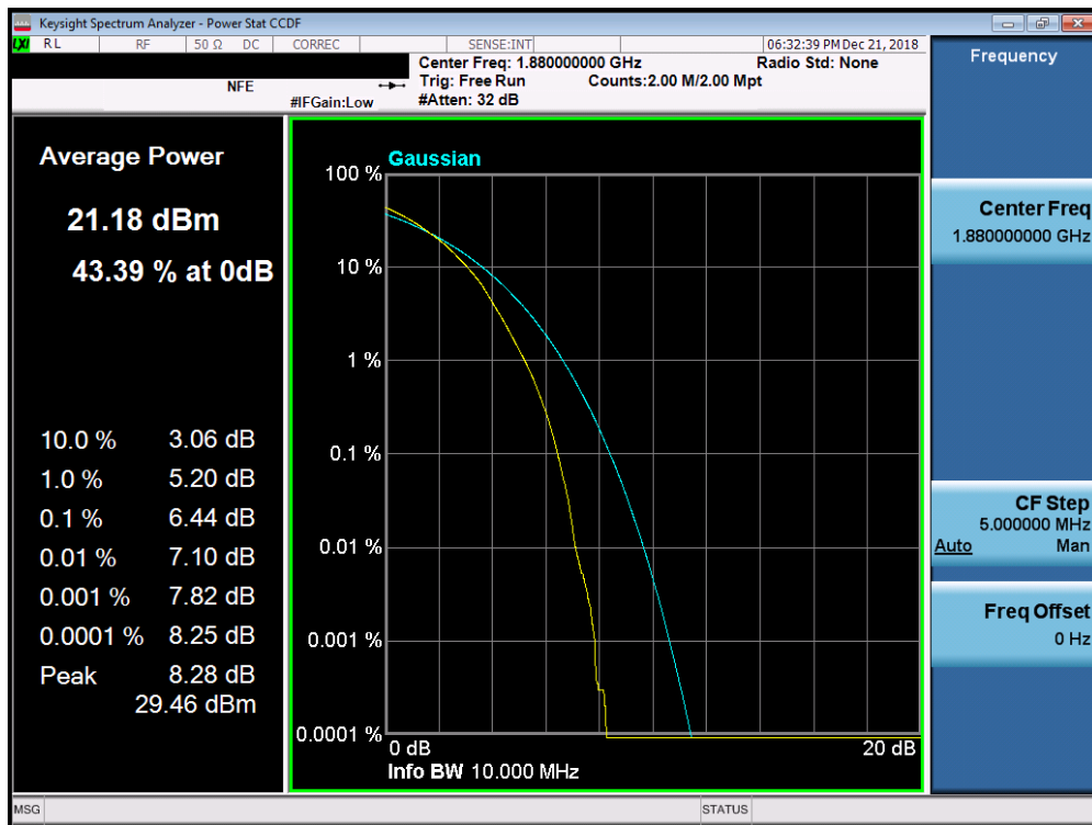
Plot 7-258. PAR Plot (Band 2/25 - 10.0MHz 64-QAM - Full RB Configuration)
