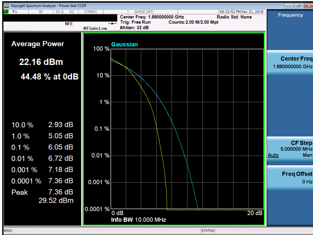
Plot 7-257. PAR Plot (Band 2/25 - 10.0MHz 16-QAM - Full RB Configuration)
