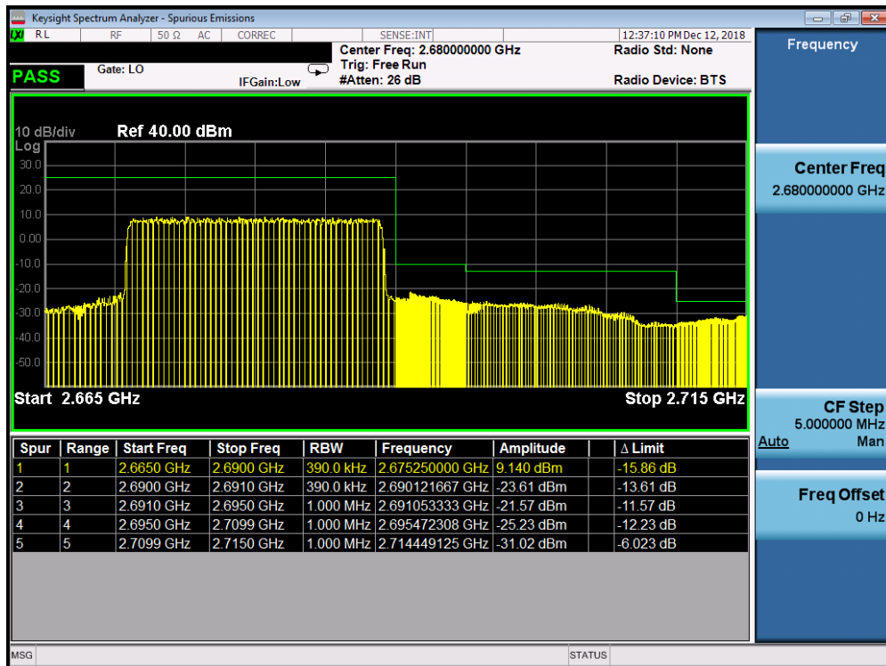
Plot 7-246. Upper ACP Plot (Band 41 PC2 - 20.0MHz QPSK - Full RB Configuration)
