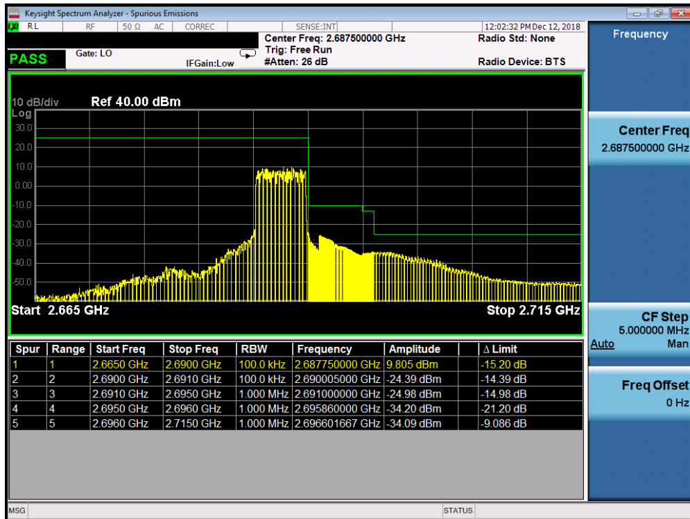
Plot 7-240. Upper ACP Plot (Band 41 PC2 - 5.0MHz QPSK - Full RB Configuration)
