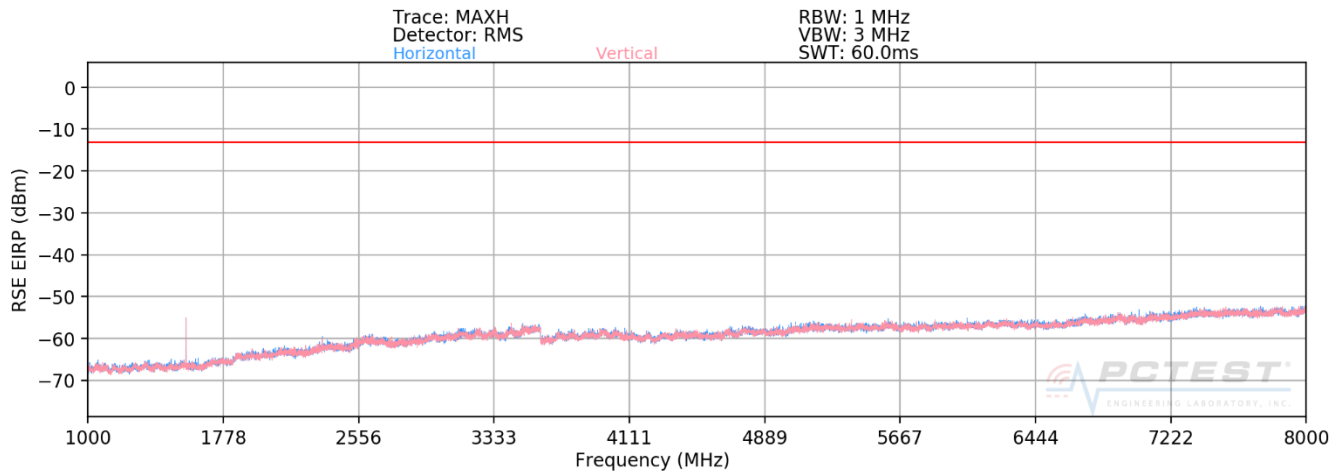
Plot 7-266. Radiated Spurious Plot above 1GHz (Band 13)
