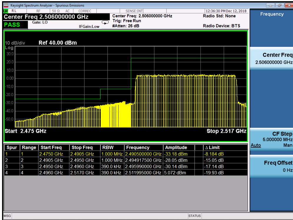
Plot 7-245. Lower ACP Plot at 2496 MHz (Band 41 PC2 - 20.0MHz QPSK - Full RB Configuration)
