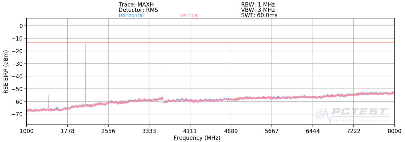
Plot 7-265. Radiated Spurious Plot above 1GHz (Band 12/17)
