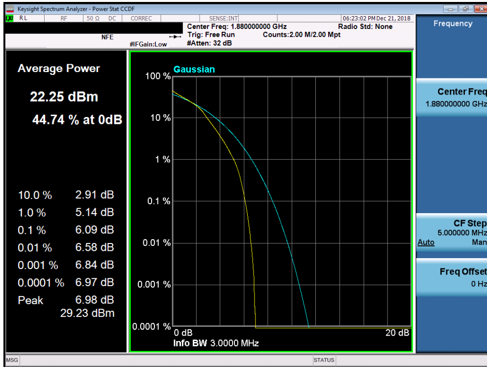
Plot 7-251. PAR Plot (Band 2/25 - 3.0MHz 16-QAM - Full RB Configuration)
