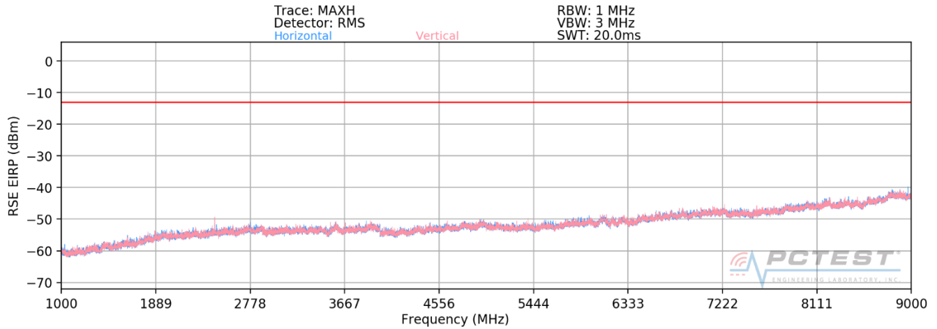
Plot 7-267. Radiated Spurious Plot above 1GHz (Band 26/5)
