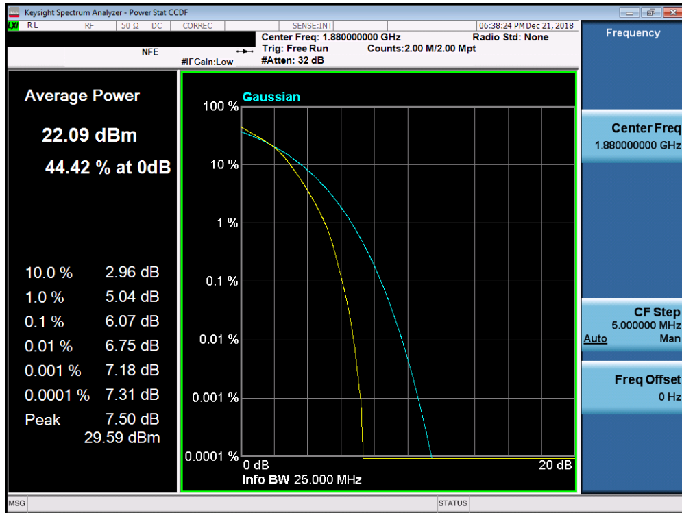
Plot 7-263. PAR Plot (Band 2/25 - 20.0MHz 16-QAM - Full RB Configuration)
