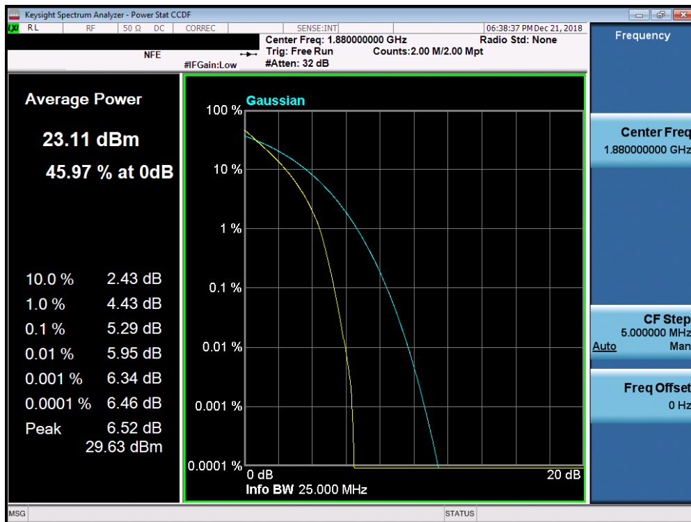
Plot 7-262. PAR Plot (Band 2/25 - 20.0MHz QPSK - Full RB Configuration)
