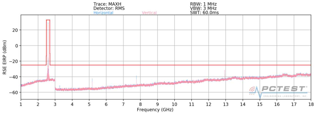
Plot 7-270. Radiated Spurious Plot 1GHz - 18GHz (Band 41)
