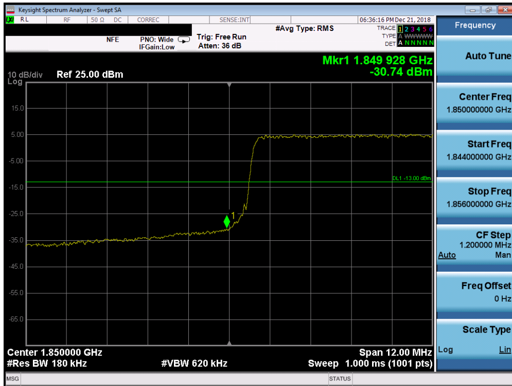
Plot 7-227. Lower Band Edge Plot (Band 25/2 - 15MHz QPSK - Full RB Configuration)
