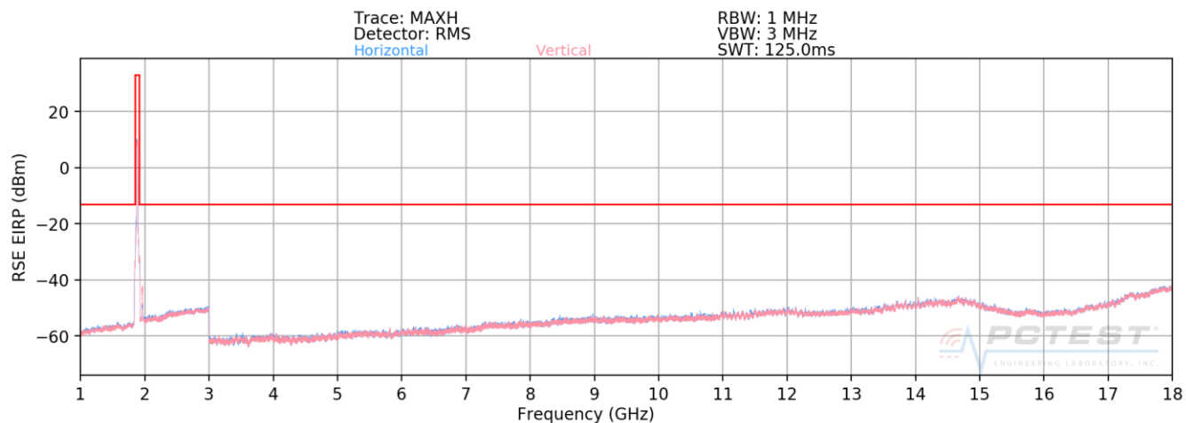
Plot 7-269. Radiated Spurious Plot above 1GHz (Band 25/2)
