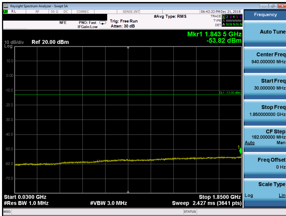
Plot 7-127. Conducted Spurious Plot (Band 2/25 - 20.0MHz QPSK - RB Size 1, RB Offset 0 - High Channel)
