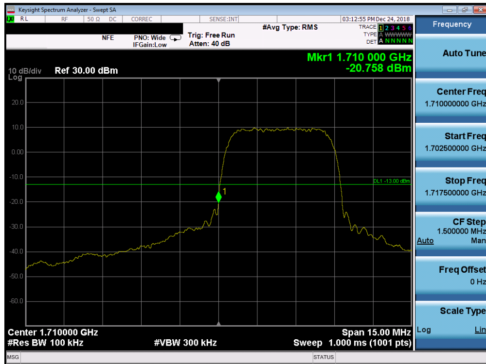
Plot 7-84. Band Edge Plot (AWS WCDMA Mode - Low Channel)
