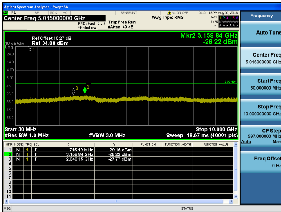
LTE Band 12 / 3MHz / 64QAM - RB Size/Offset (8/7) – High Channel
