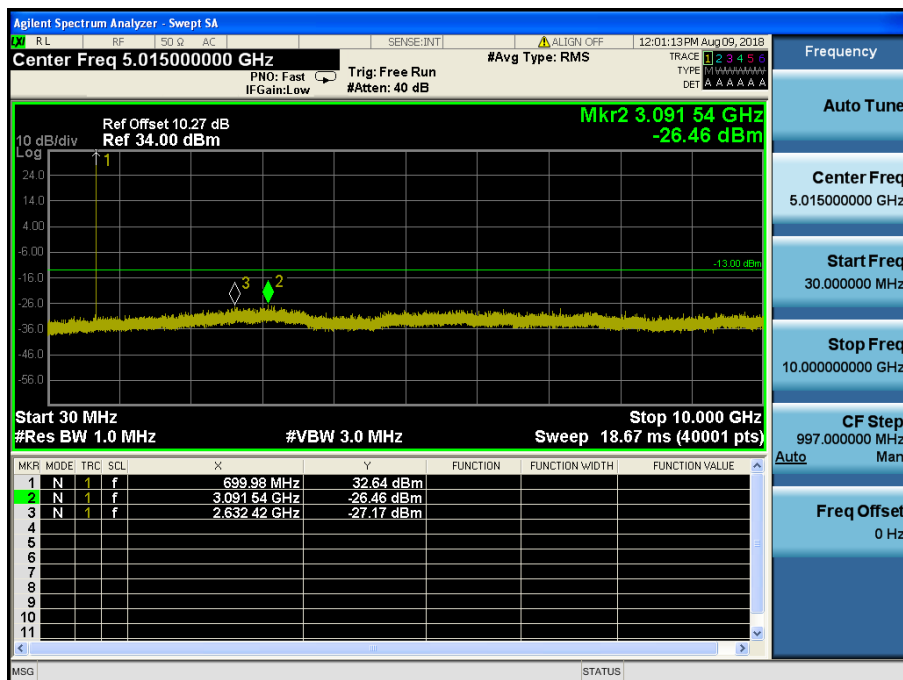
LTE Band 12 / 1.4MHz / 64QAM - RB Size/Offset (1/2) – Low Channel
