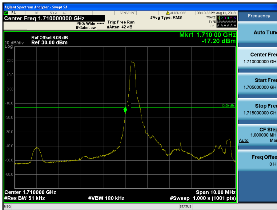
LTE Band 4,66 / 5MHz / 16QAM Offset/Size (1/0)
