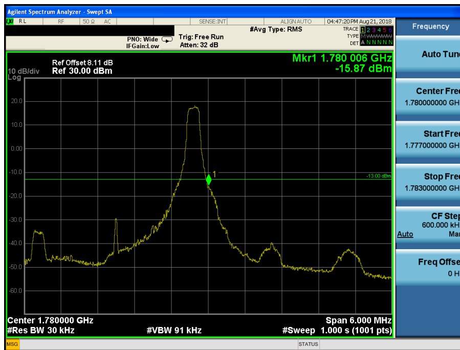
LTE Band 4,66 / 3MHz / QPSK - RB Size/Offset (1/14)
