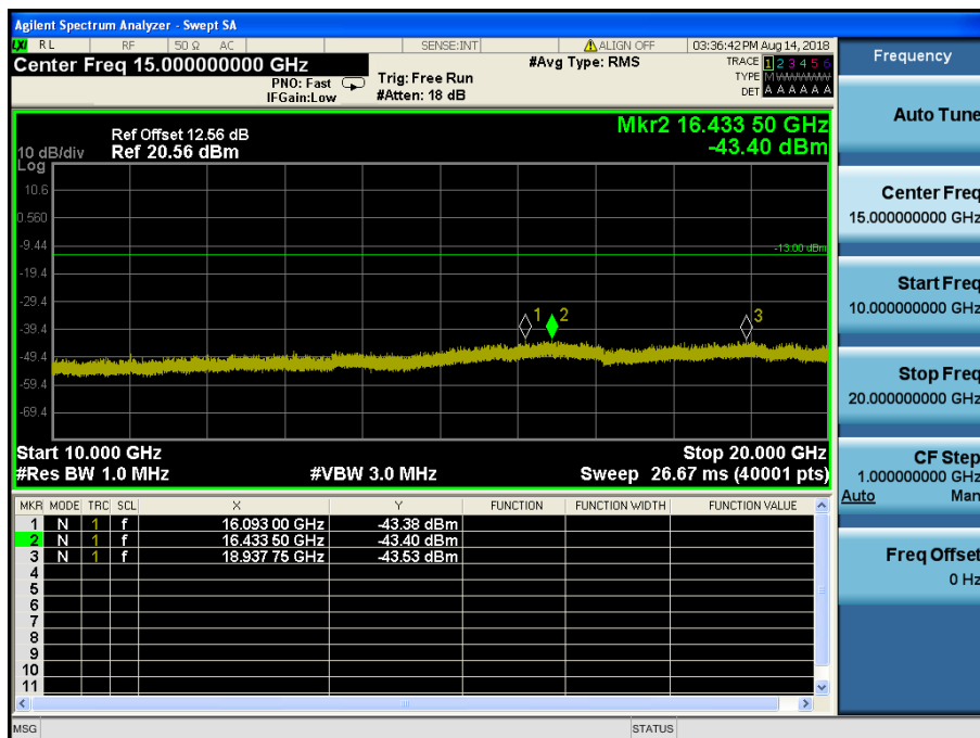
LTE Band 4,66 / 20MHz / QPSK - RB Size/Offset (50/0) – High Channel
