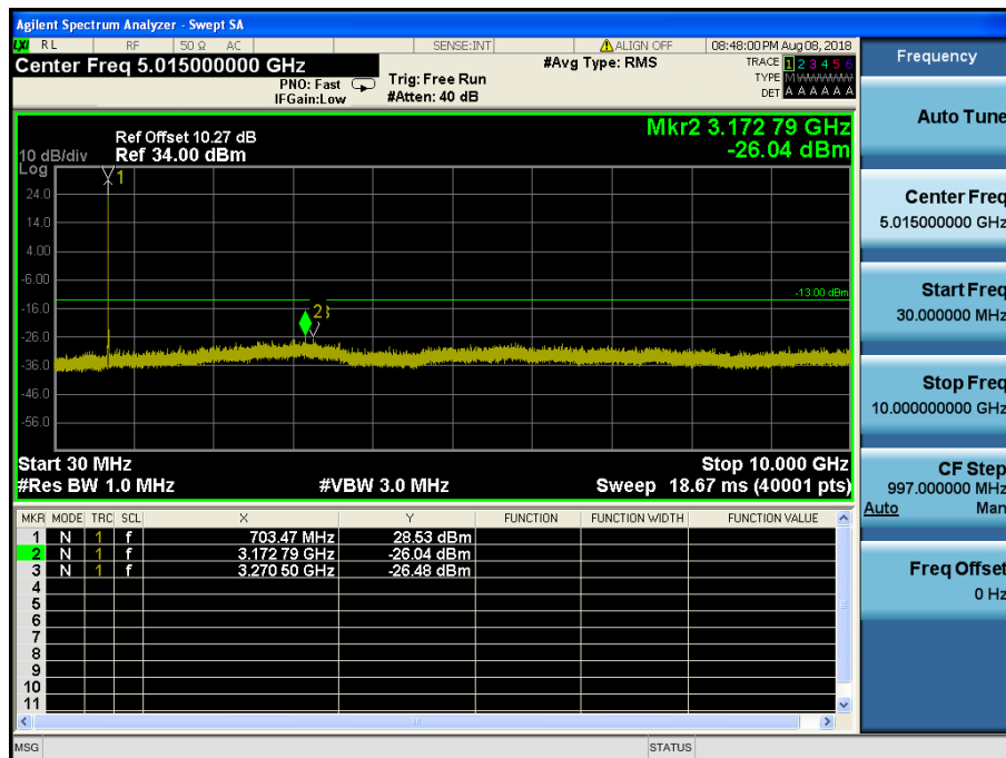
LTE Band 12,17 / 5MHz / QPSK - RB Size/Offset (12/13) – Low Channel
