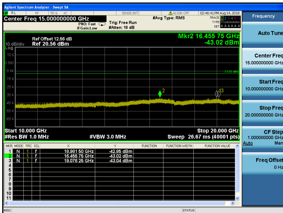
LTE Band 4,66 / 15MHz / QPSK - RB Size/Offset (75/0) – High Channel
