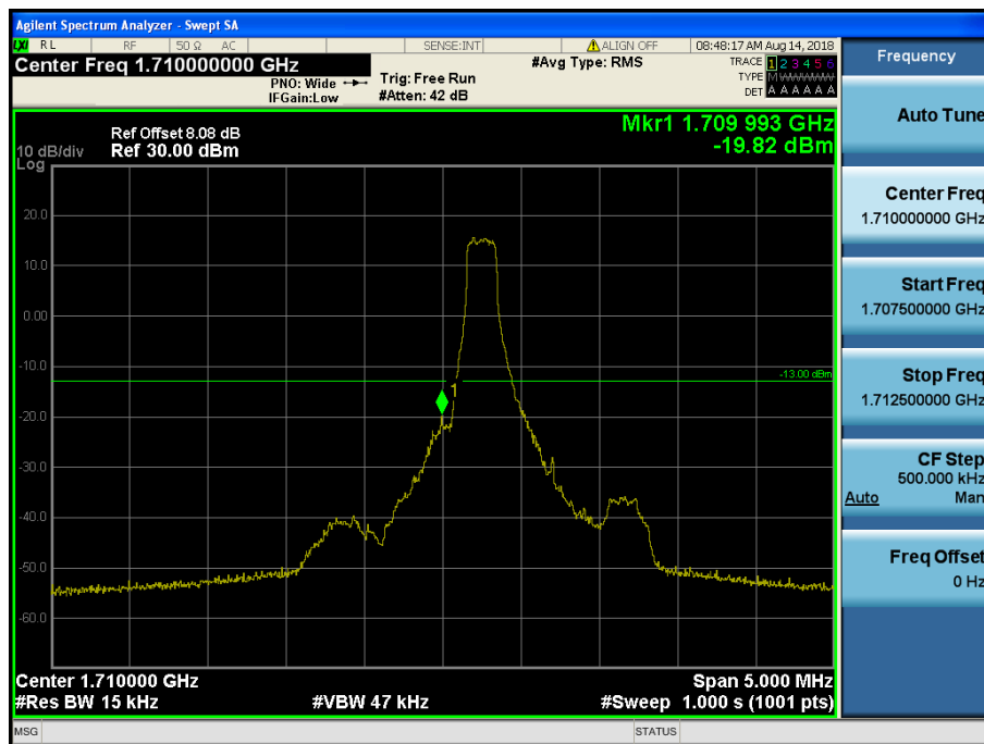
LTE Band 4,66 / 1.4MHz / QPSK - RB Size/Offset (1/0)
