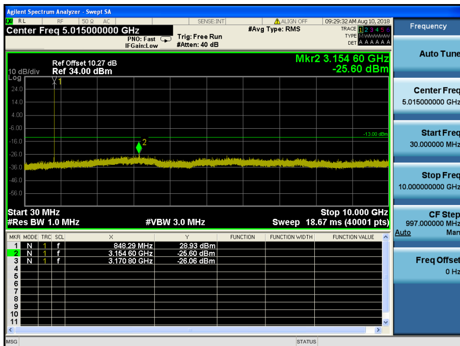
LTE Band 5 / 1.4MHz / 64QAM - RB Size/Offset (6/0) – High Channel
