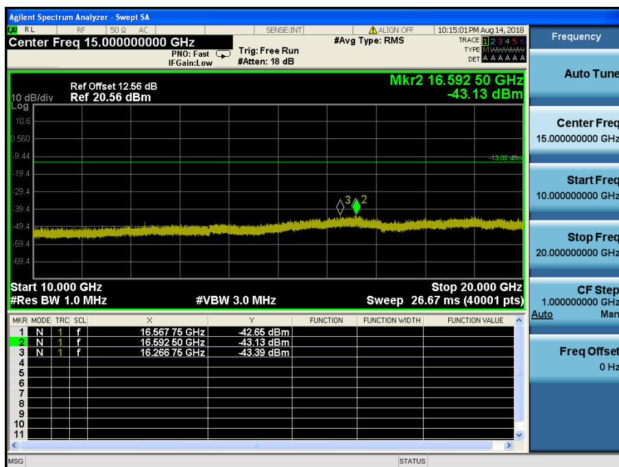
LTE Band 4,66 / 15MHz / 16QAM - RB Size/Offset (36/18)–Low Channel
