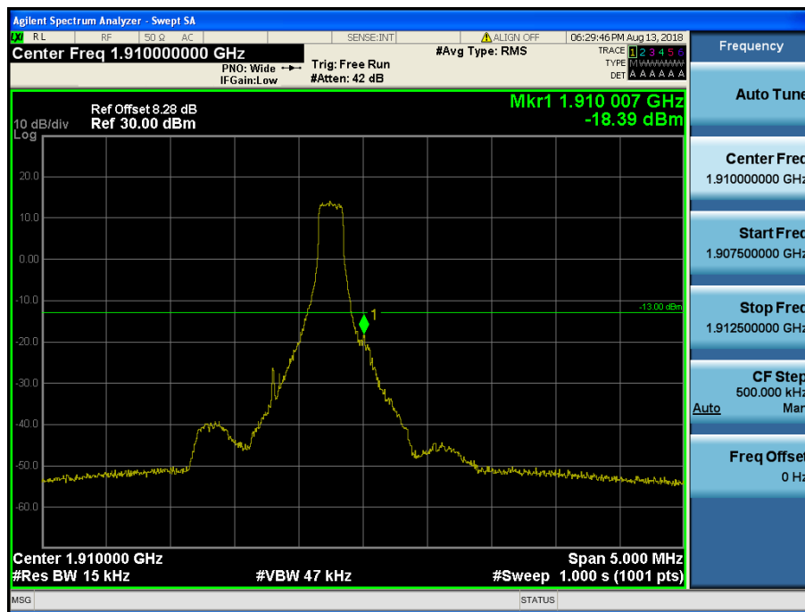
LTE Band 2 / 1.4MHz / 64QAM - RB Size/Offset (1/5)
