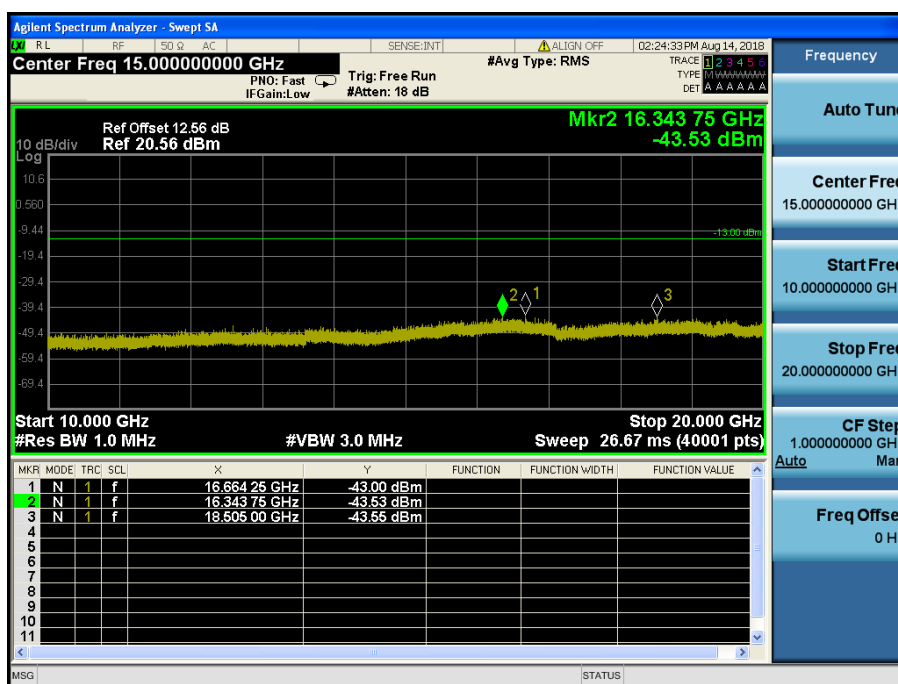
LTE Band 4,66 / 15MHz / QPSK - RB Size/Offset (1/36) – Mid Channel
