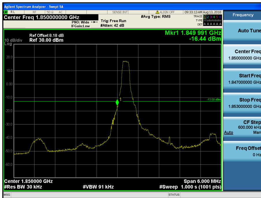
LTE Band 2 / 3MHz / 16QAM - RB Size/Offset (1/0)
