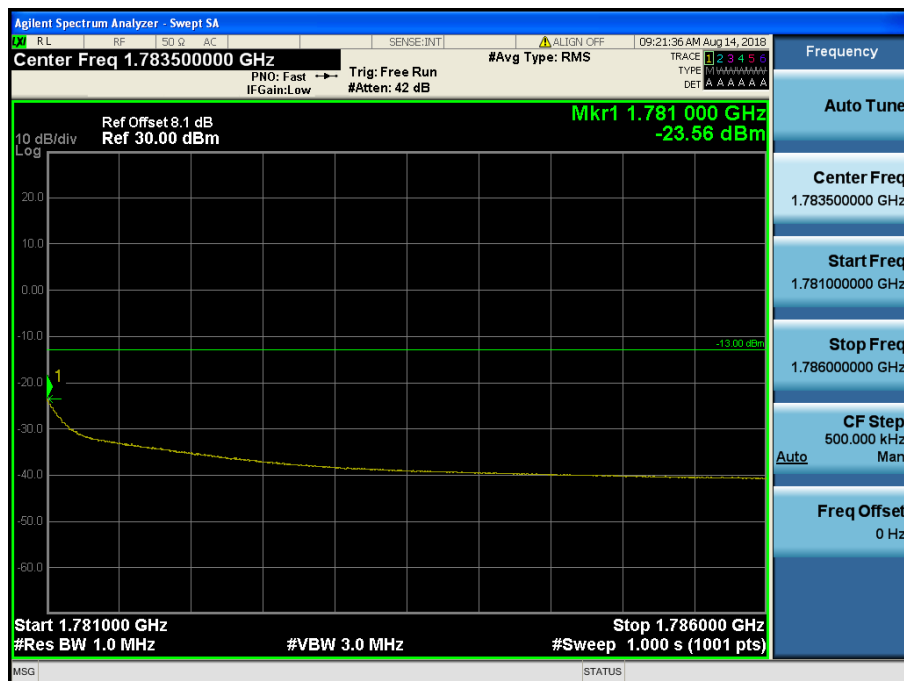
LTE Band 4,66 / 1.4MHz / QPSK - RB Size/Offset (3/0)
