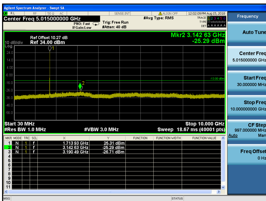
LTE Band 4,66 / 5MHz / 64QAM - RB Size/Offset (12/13) – Low Channel
