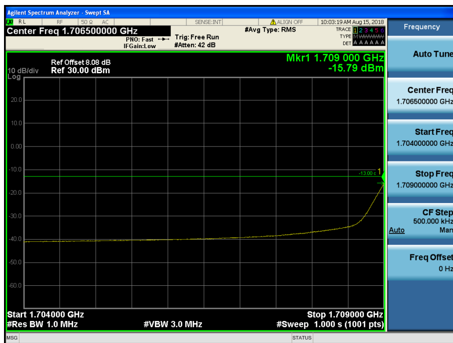
LTE Band 4,66 / 1.4MHz / 64QAM - RB Size/Offset (3/2)
