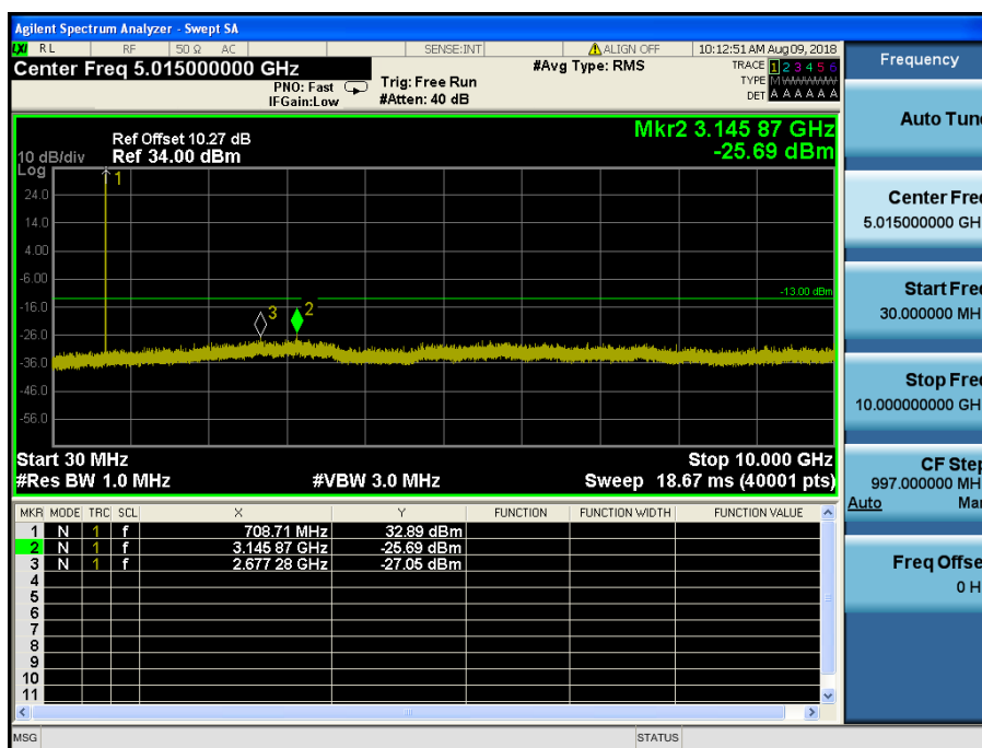
LTE Band 12,17 / 10MHz / 16QAM - RB Size/Offset (1/49) – Low Channel
