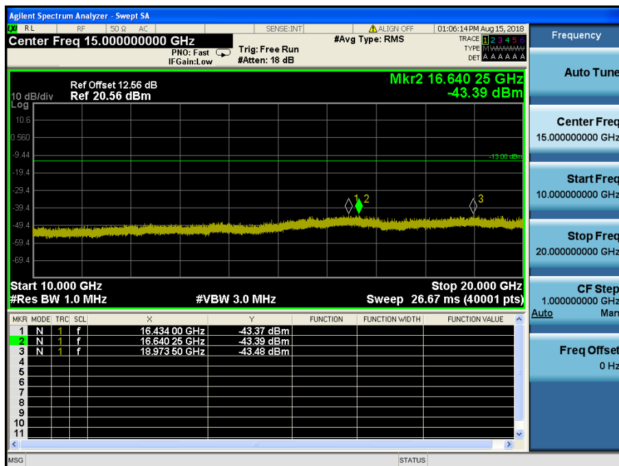
LTE Band 4,66 / 10MHz / 64QAM - RB Size/Offset (25/0) – Mid Channel
