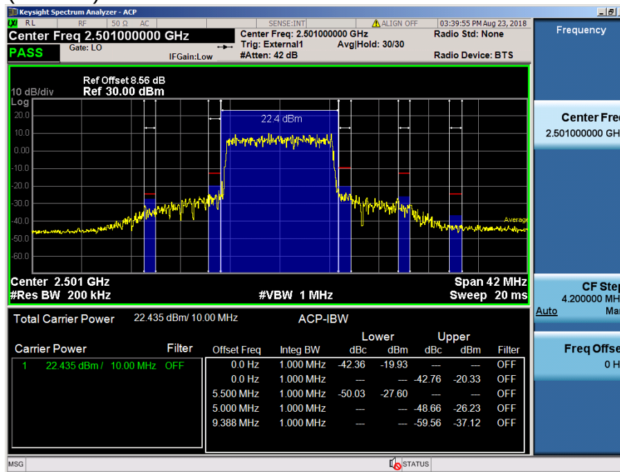
LTE Band 41 / 10MHz / QPSK - RB Size/Offset (50/0)
