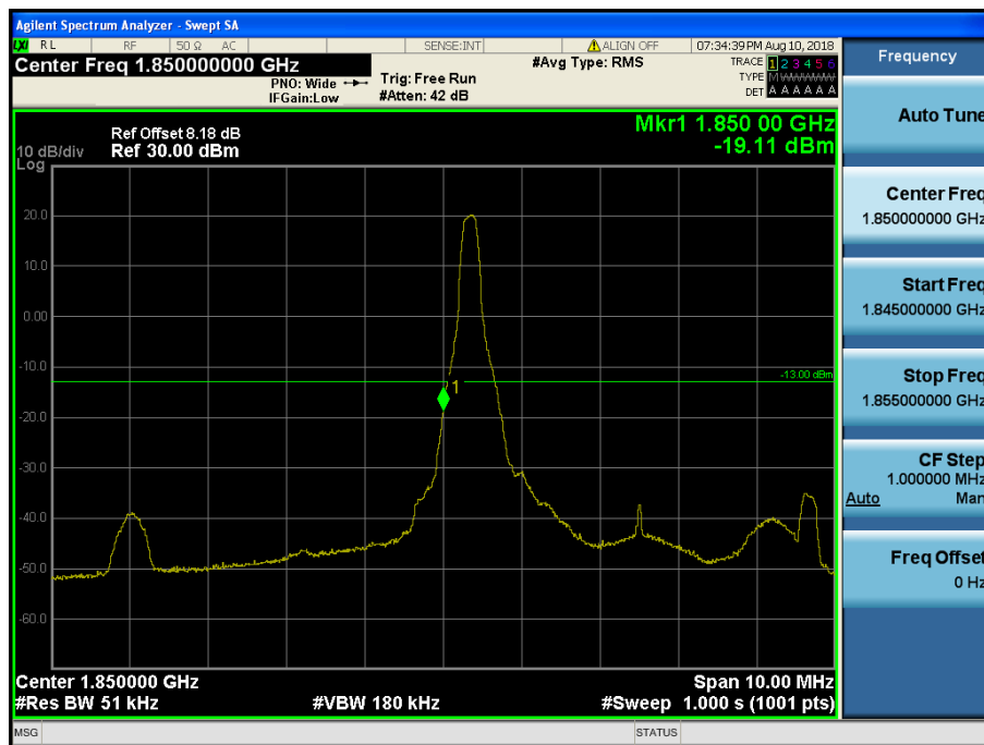
LTE Band 2 / 5MHz / QPSK Offset/Size (1/0)
