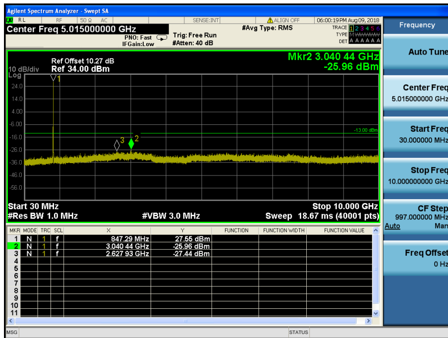
LTE Band 5 / 3MHz / QPSK - RB Size/Offset (15/0) – High Channel
