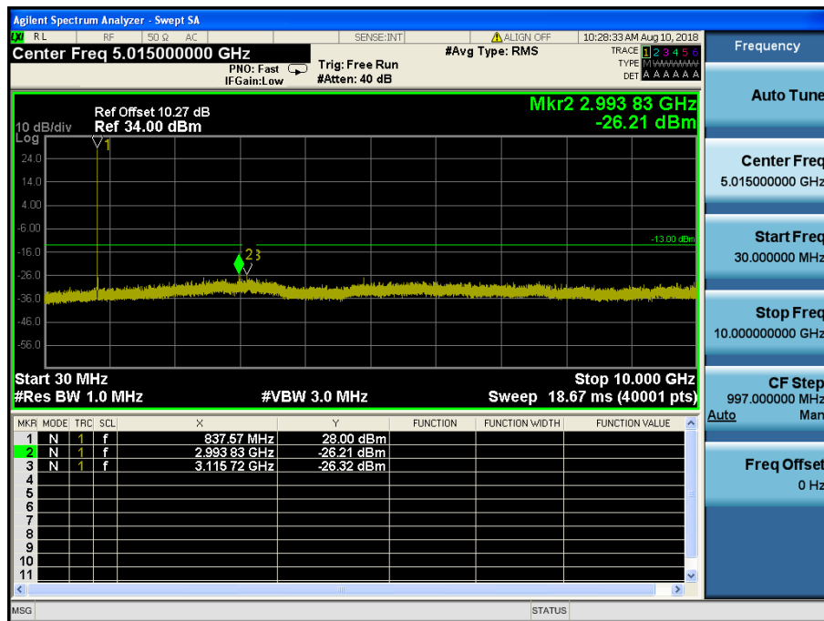
LTE Band 5 / 5MHz / 64QAM - RB Size/Offset (12/6) – Mid Channel
