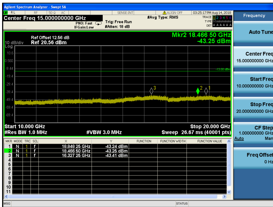
LTE Band 4,66 / 20MHz / QPSK - RB Size/Offset (100/0)–Mid Channel
