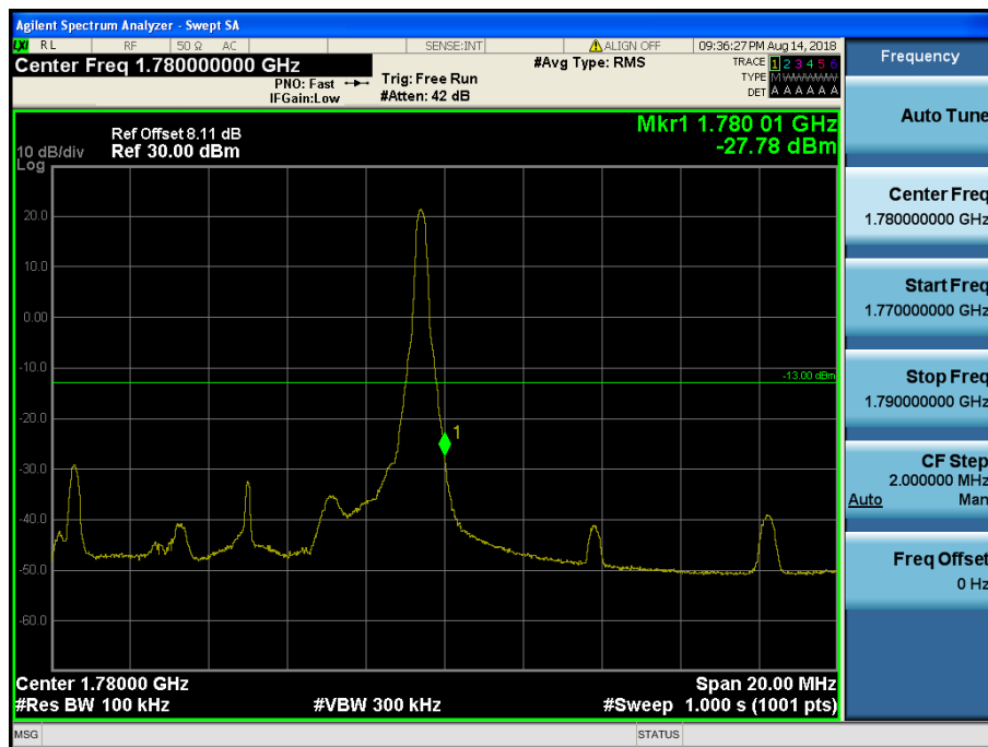
LTE Band 4,66 / 10MHz / 16QAM - RB Size/Offset (1/49)
