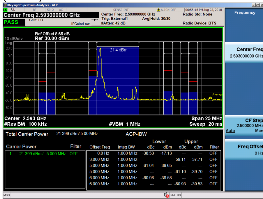
LTE Band 41 / 5MHz / 64QAM - RB Size/Offset (1/0)
