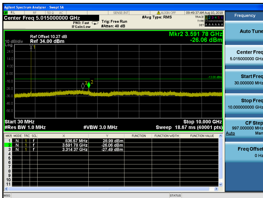
LTE Band 5 / 3MHz / 64QAM - RB Size/Offset (8/4) – Mid Channel
