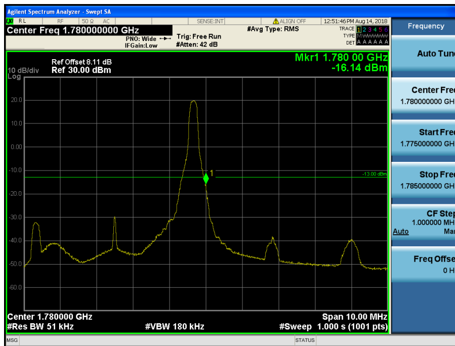
LTE Band 4,66 / 5MHz / QPSK - RB Size/Offset (1/24)
