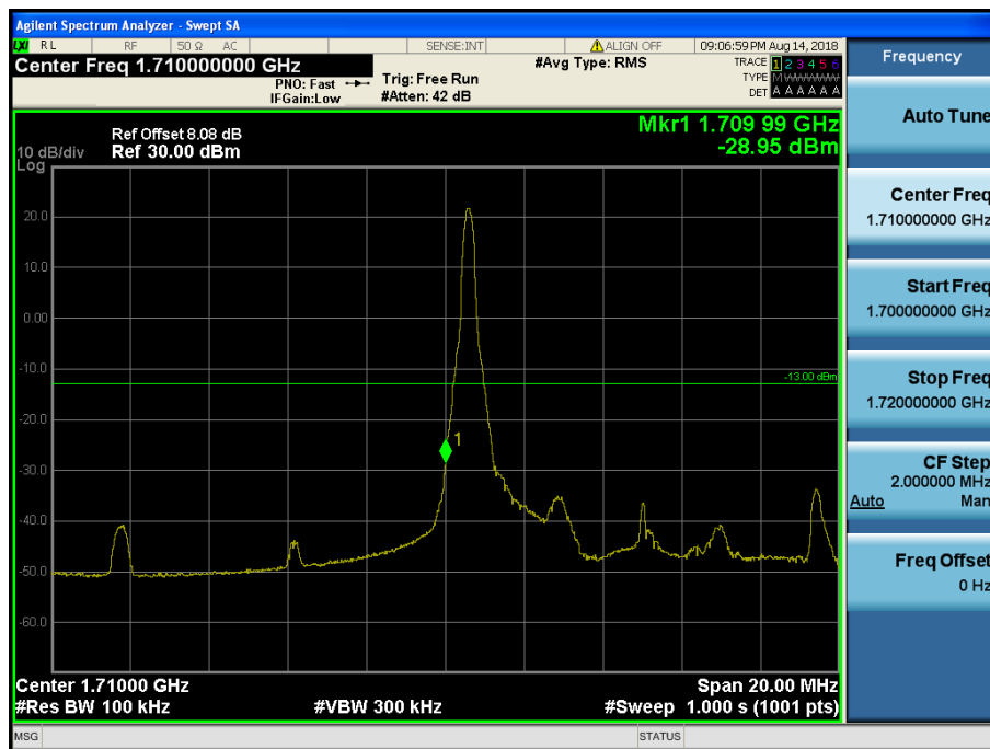
LTE Band 4,66 / 10MHz / 16QAM - RB Size/Offset (1/0)
