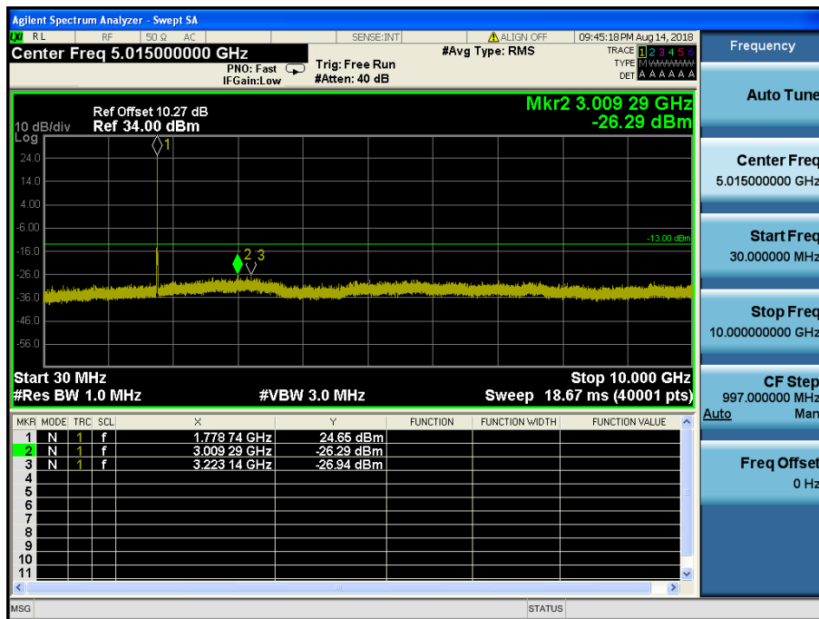
LTE Band 4,66 / 10MHz / 16QAM - RB Size/Offset (25/25) – High Channel
