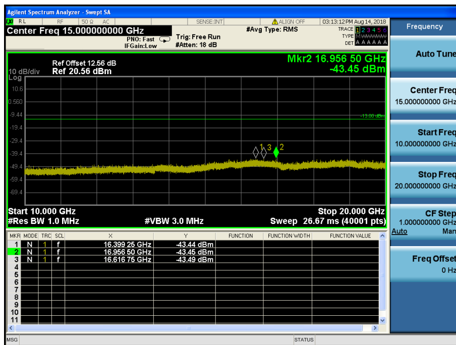
LTE Band 4,66 / 20MHz / QPSK - RB Size/Offset (50/25) –Low Channel
