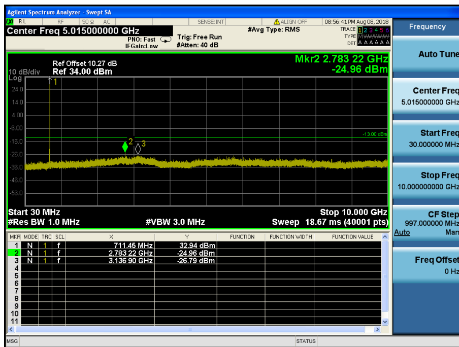
LTE Band 12,17 / 5MHz / QPSK - RB Size/Offset (1/0) – High Channel
