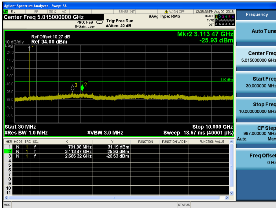
LTE Band 12 / 3MHz / 64QAM - RB Size/Offset (1/14) – Low Channel
