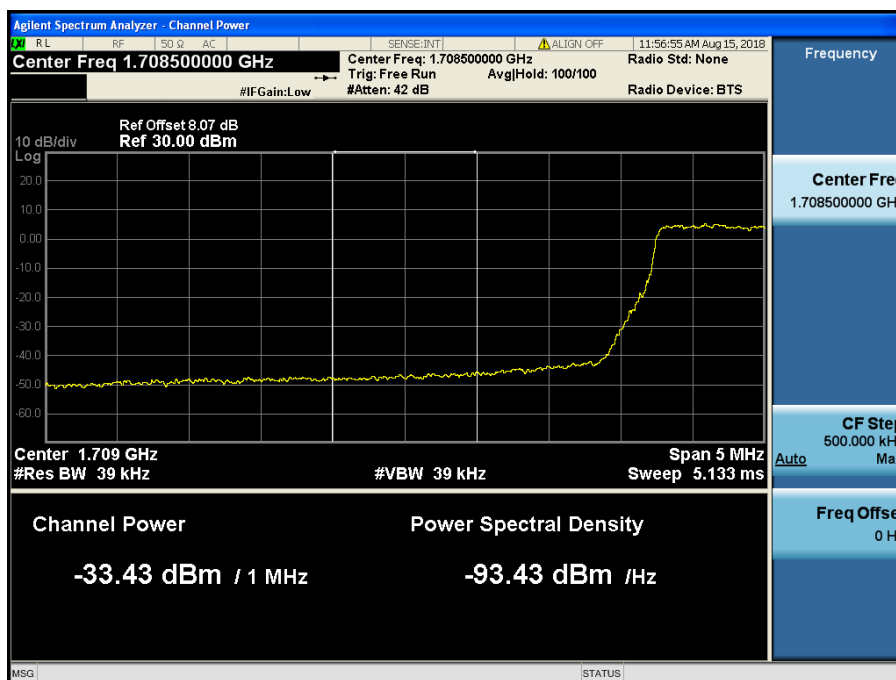
LTE Band 4,66 / 5MHz / 64QAM Offset/Size (12/0)
