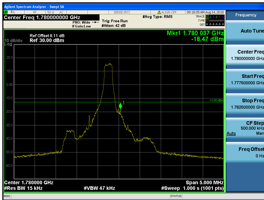
LTE Band 4,66 / 1.4MHz / QPSK - RB Size/Offset (1/5)
