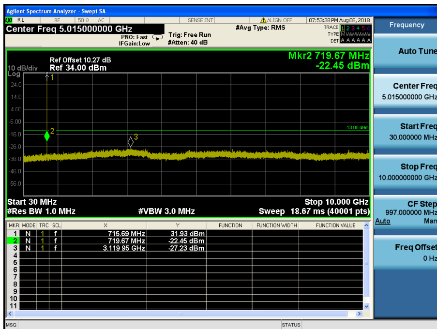
LTE Band 12 / 1.4MHz / QPSK - RB Size/Offset (3/2) – High Channel
