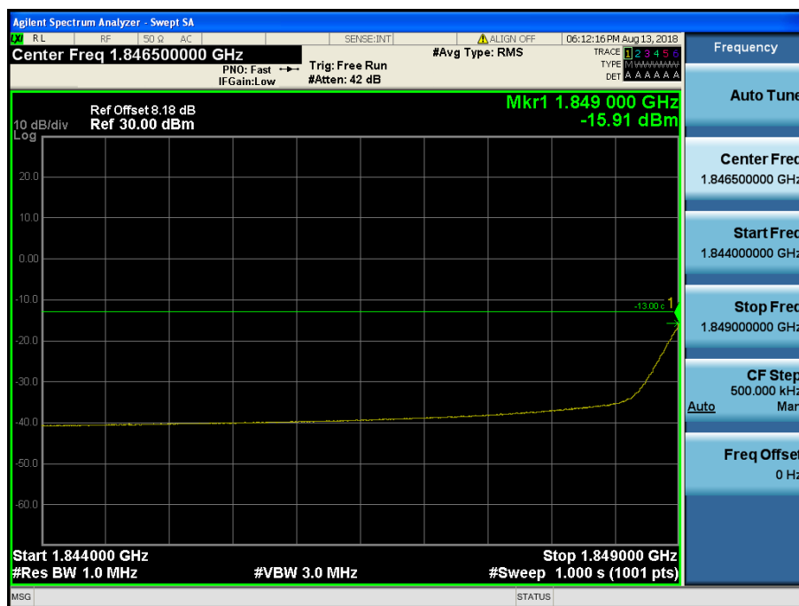
LTE Band 2 / 1.4MHz / 64QAM - RB Size/Offset (3/2)
