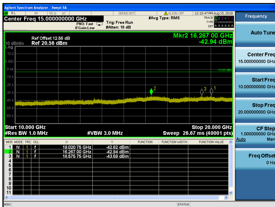
LTE Band 4,66 / 5MHz / 64QAM - RB Size/Offset (25/0) – Mid Channel
