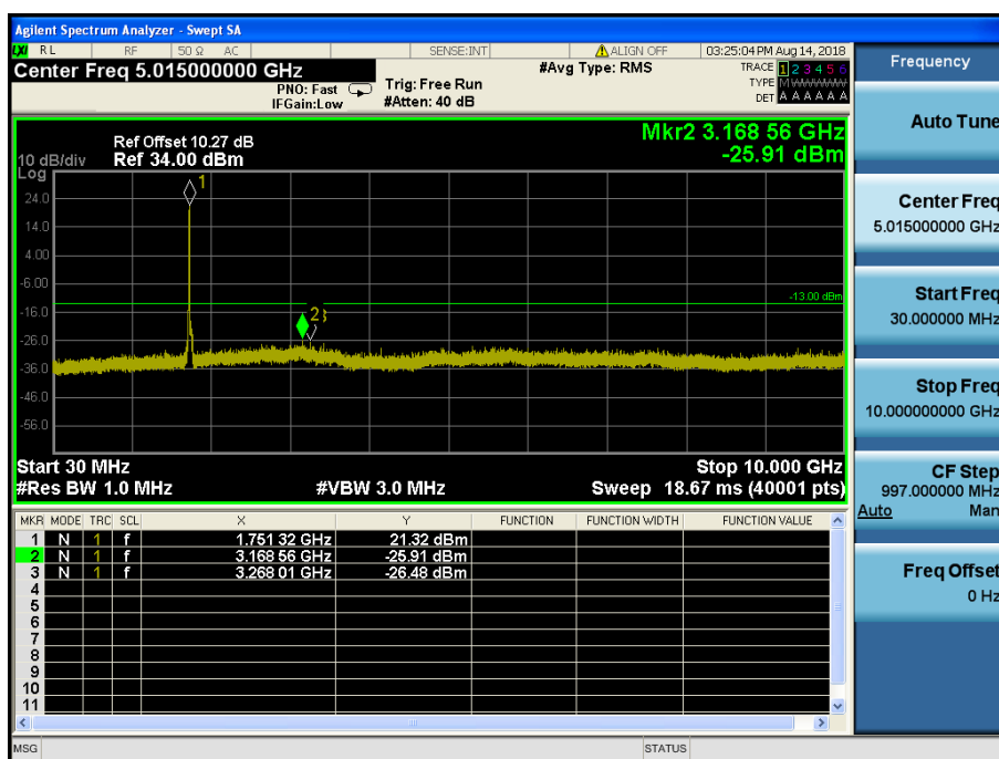
LTE Band 4,66 / 20MHz / QPSK - RB Size/Offset (100/0)–Mid Channel
