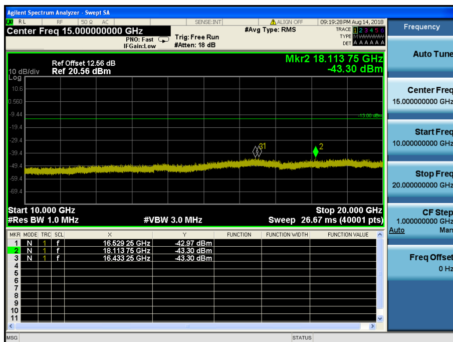
LTE Band 4,66/ 10MHz / 16QAM - RB Size/Offset (25/12) – Low Channel
