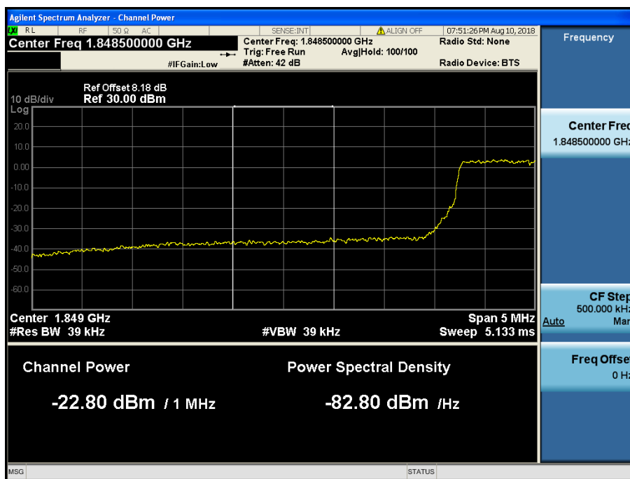
LTE Band 2 / 5MHz / QPSK Offset/Size (25/0)
