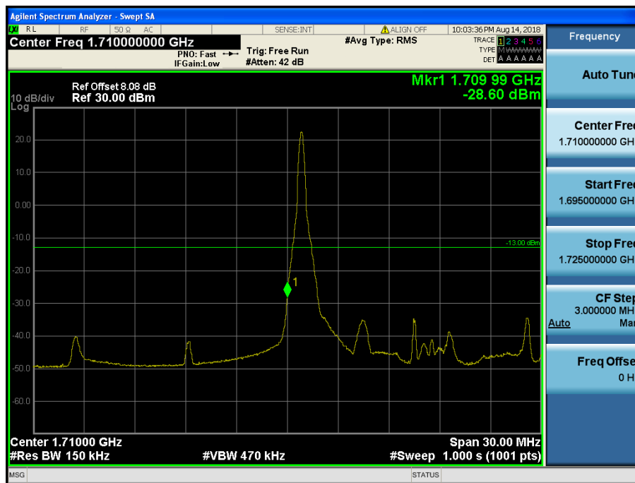
LTE Band 4,66 / 15MHz / 16QAM - RB Size/Offset (1/0)
