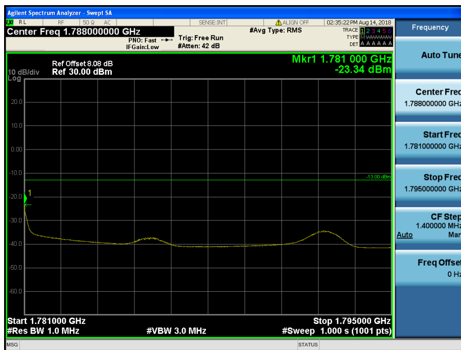
LTE Band 4,66 / 15MHz / QPSK - RB Size/Offset (1/74)
