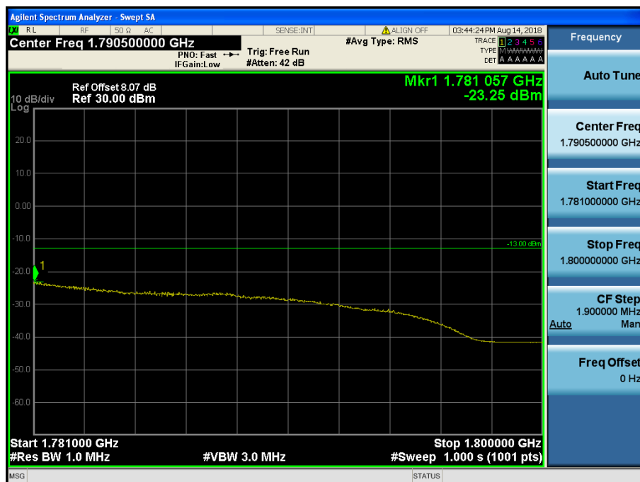
LTE Band 4,66 / 20MHz / QPSK - RB Size/Offset (100/0)
