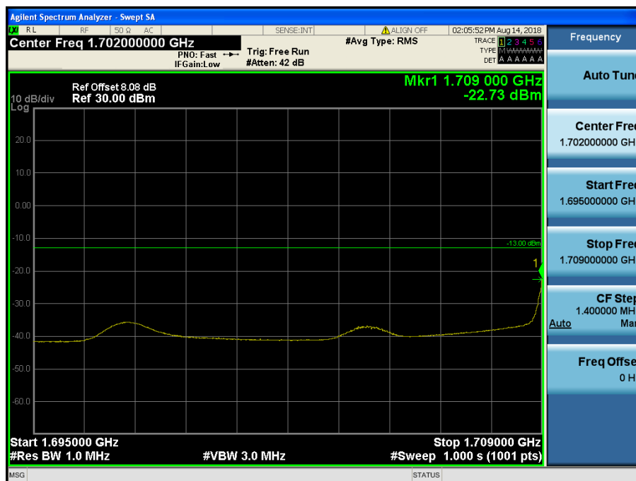
LTE Band 4,66 / 15MHz / QPSK - RB Size/Offset (1/0)
