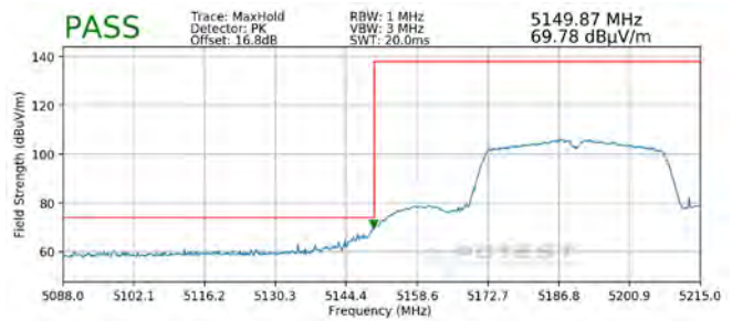
Plot 7-93. Radiated Lower Band Edge Plot (Peak – UNII Band 1)
