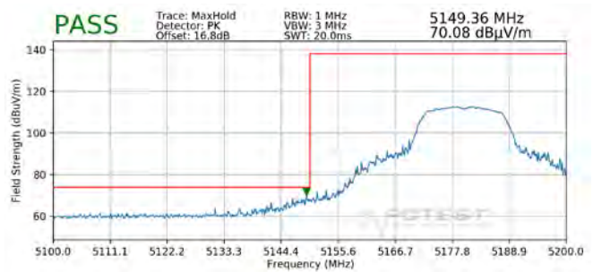
Plot 7-86. Radiated Lower Band Edge Plot (Peak – UNII Band 1)
