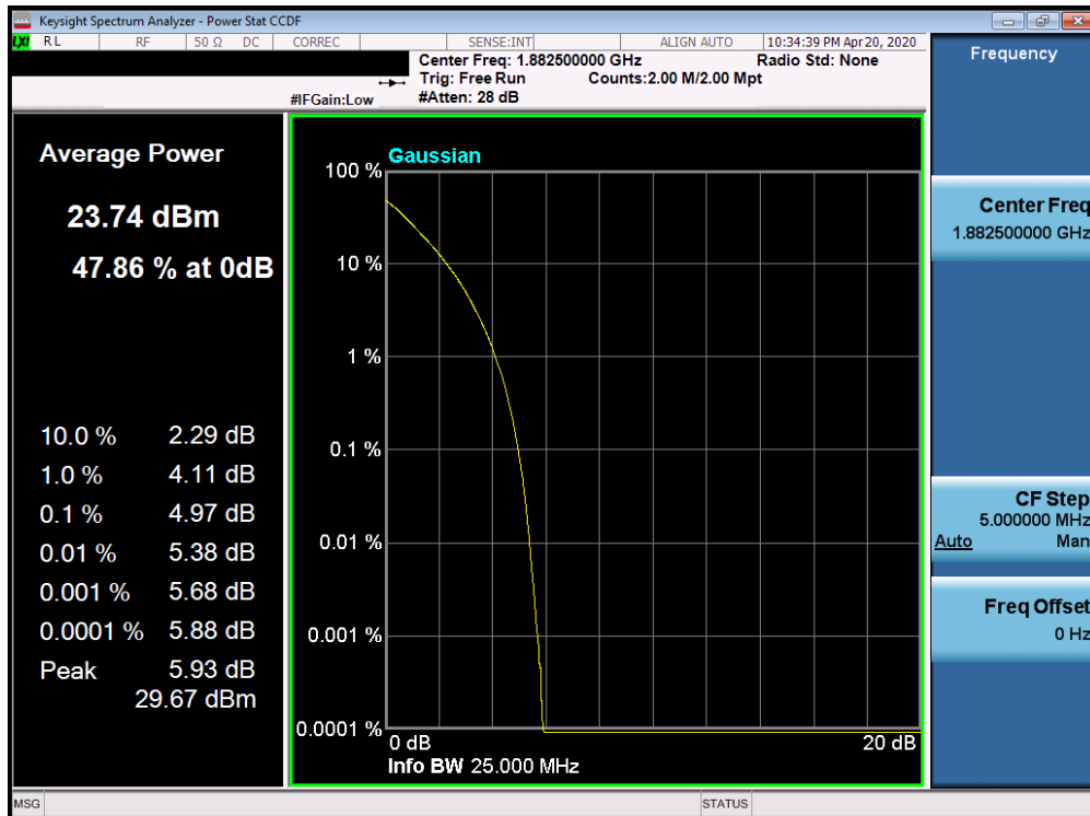
Plot 7-280. PAR Plot (Band 25/2 - 20.0MHz QPSK - Full RB Configuration)
