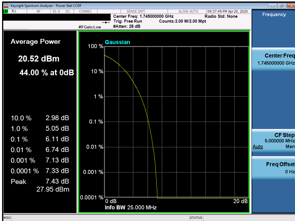
Plot 7-300. PAR Plot (Band 66/4 - 20.0MHz 64-QAM - Full RB Configuration)
