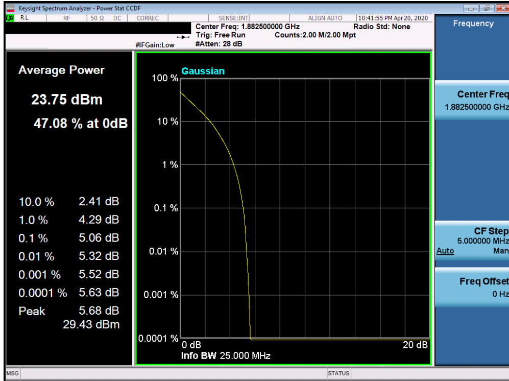
Plot 7-277. PAR Plot (Band 25/2 - 15.0MHz QPSK - Full RB Configuration)
