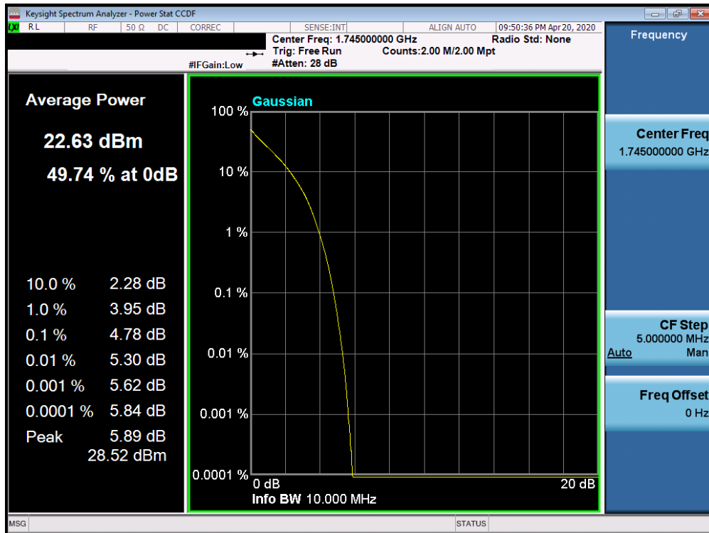
Plot 7-292. PAR Plot (Band 66/4 - 10.0MHz QPSK - Full RB Configuration)
