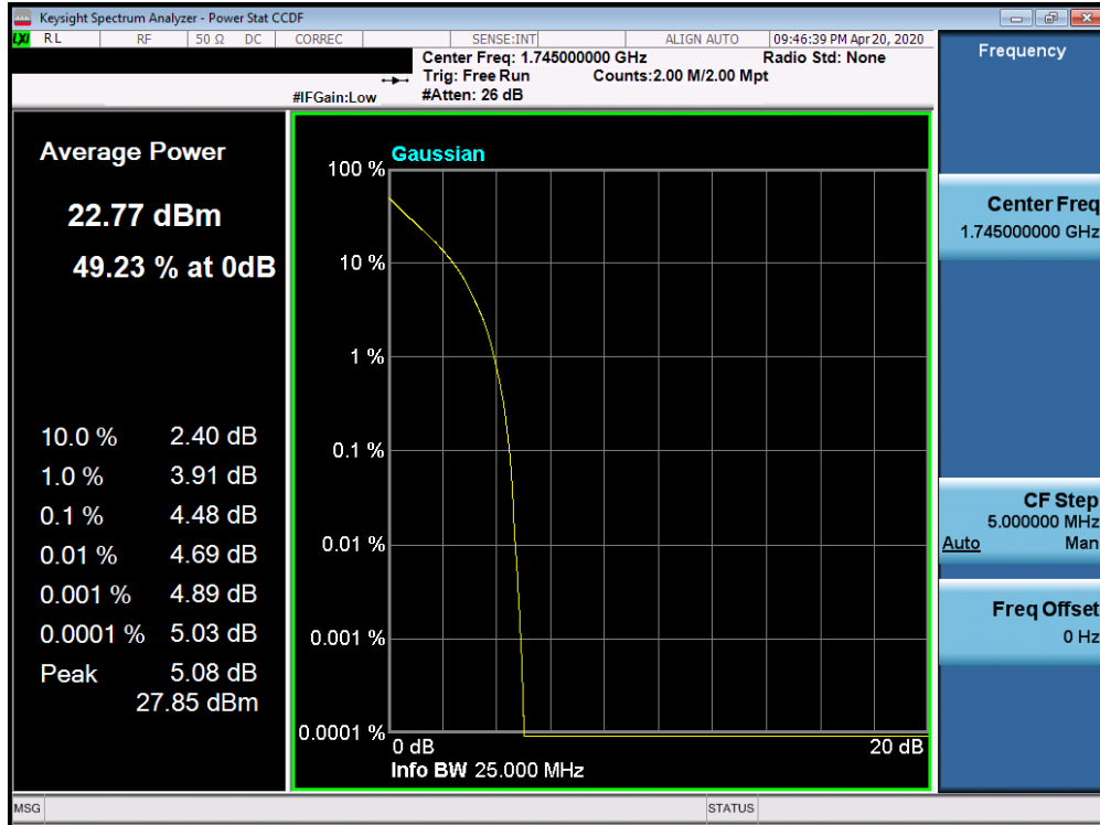
Plot 7-295. PAR Plot (Band 66/4 - 15.0MHz QPSK - Full RB Configuration)
