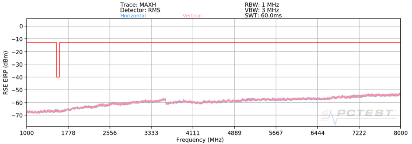
Plot 7-303. Radiated Spurious Plot above 1GHz (Band 13)
