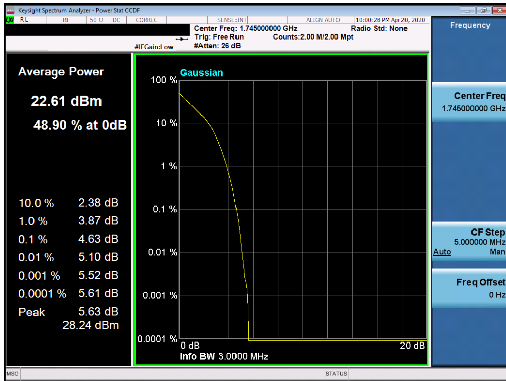
Plot 7-286. PAR Plot (Band 66/4 - 3.0MHz QPSK - Full RB Configuration)
