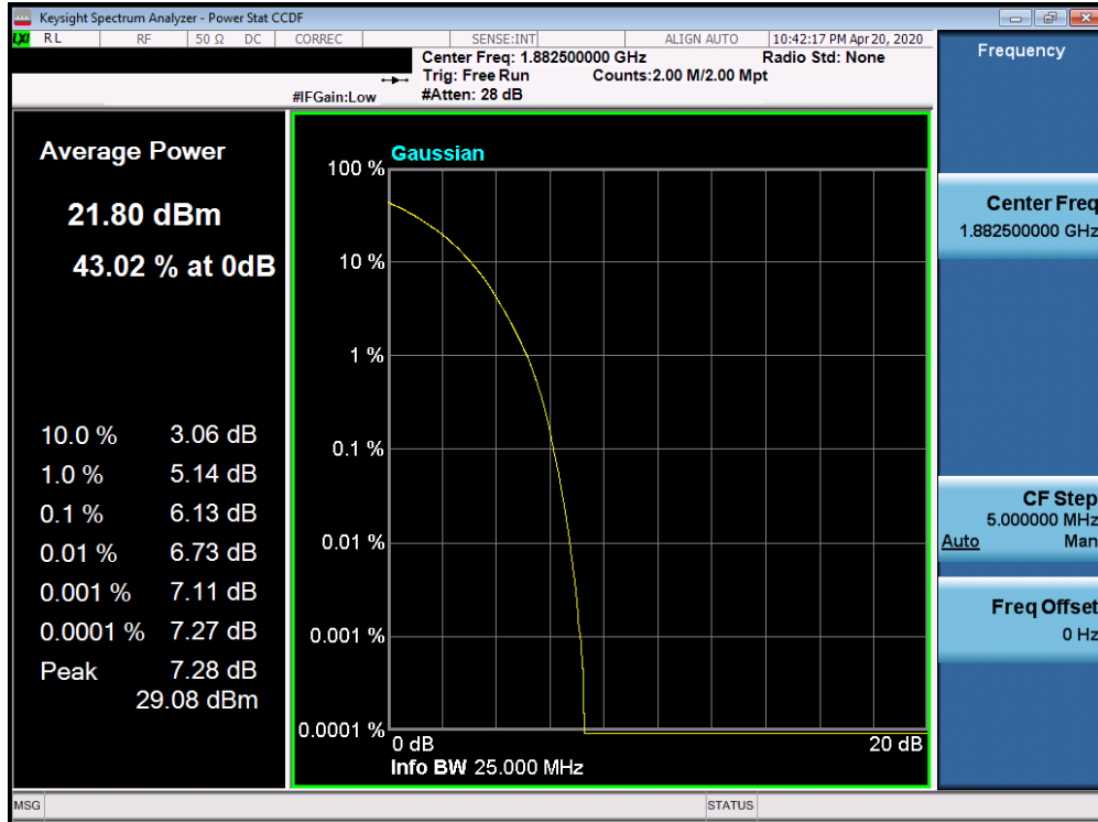
Plot 7-279. PAR Plot (Band 25/2 - 15.0MHz 64-QAM - Full RB Configuration)
