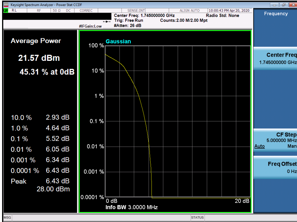
Plot 7-287. PAR Plot (Band 66/4 - 3.0MHz 16-QAM - Full RB Configuration)
