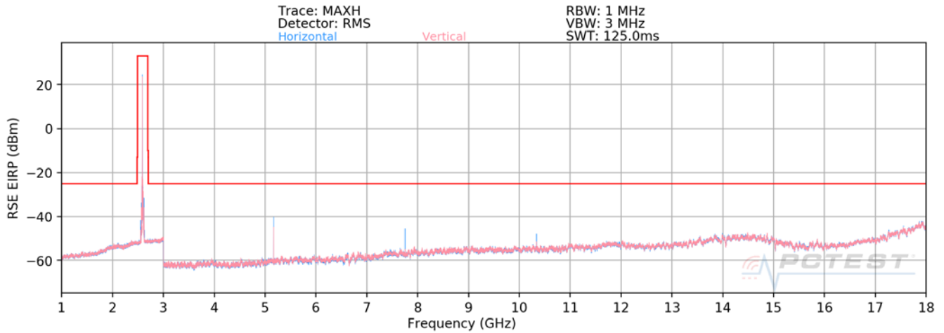
Plot 7-307. Radiated Spurious Plot 1GHz - 18GHz (Band 41)
