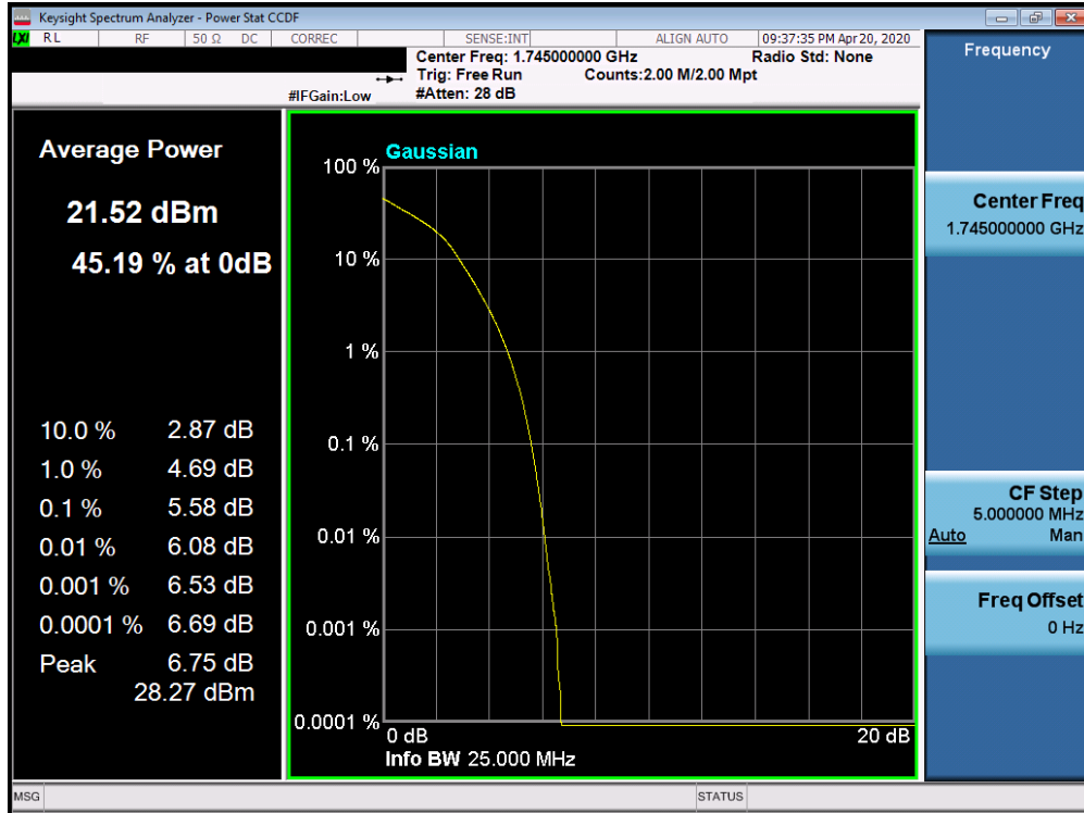
Plot 7-299. PAR Plot (Band 66/4 - 20.0MHz 16-QAM - Full RB Configuration)
