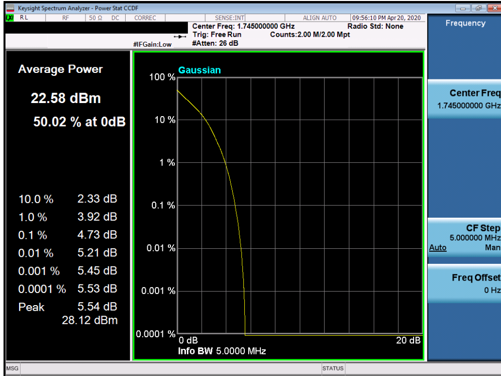
Plot 7-289. PAR Plot (Band 66/4 - 5.0MHz QPSK - Full RB Configuration)
