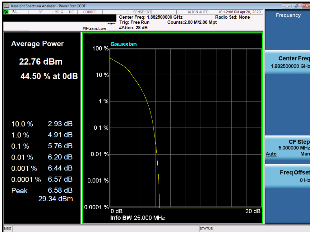
Plot 7-278. PAR Plot (Band 25/2 - 15.0MHz 16-QAM - Full RB Configuration)
