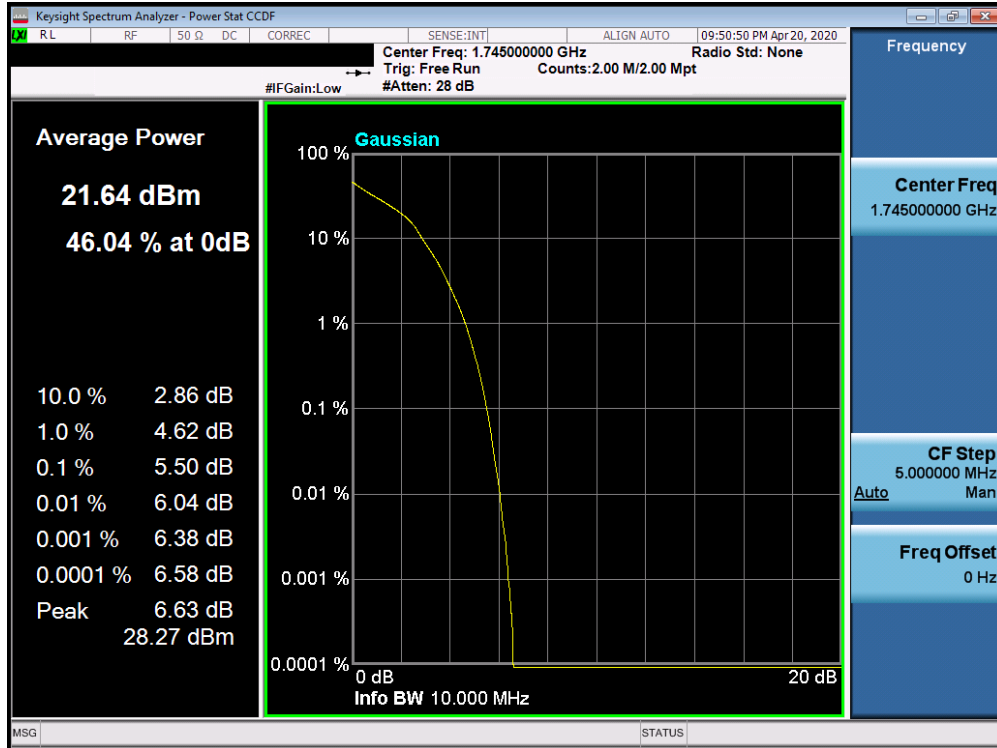
Plot 7-293. PAR Plot (Band 66/4 - 10.0MHz 16-QAM - Full RB Configuration)
