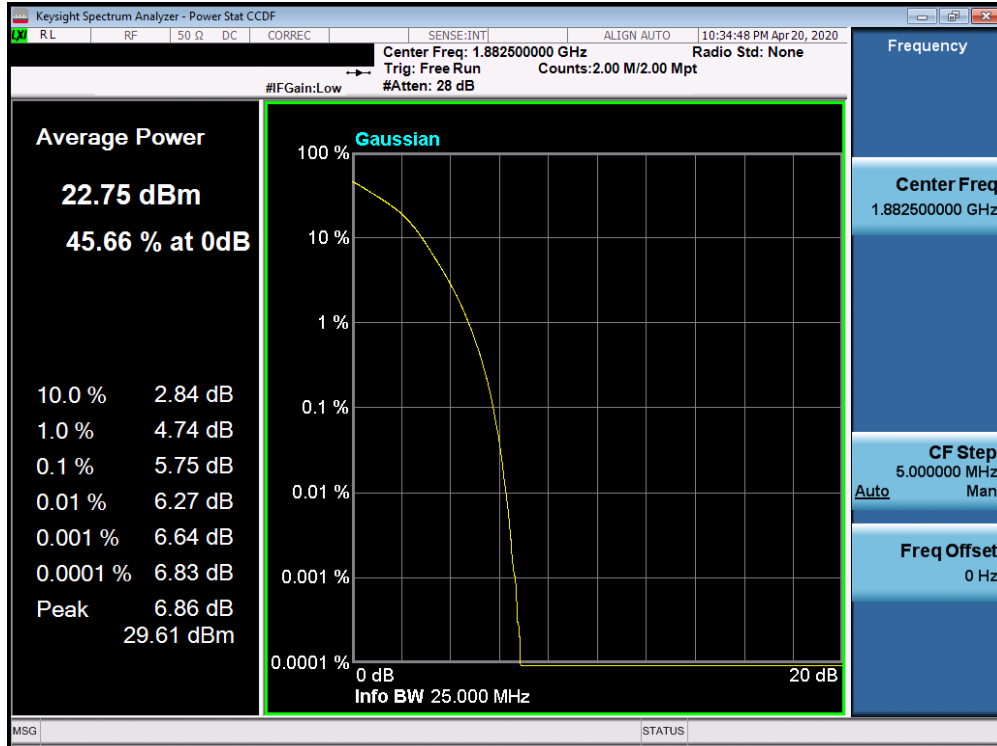
Plot 7-281. PAR Plot (Band 25/2 - 20.0MHz 16-QAM - Full RB Configuration)
