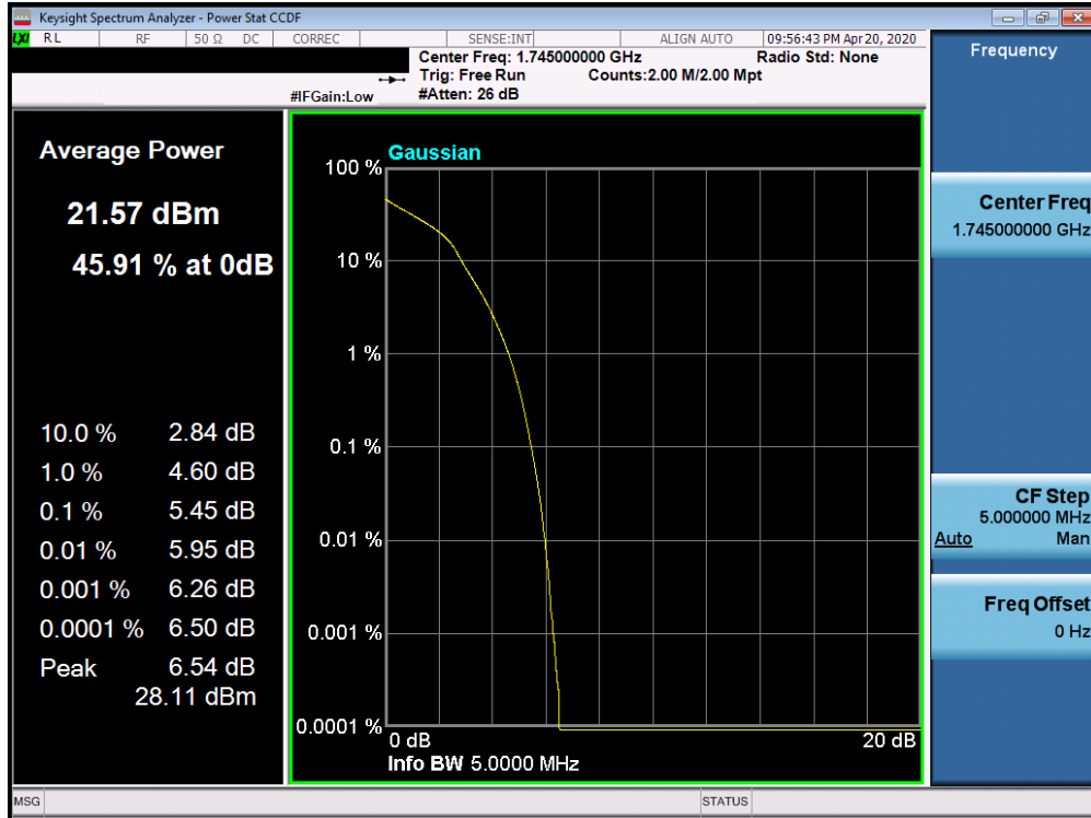
Plot 7-291. PAR Plot (Band 66/4 - 5.0MHz 64-QAM - Full RB Configuration)
