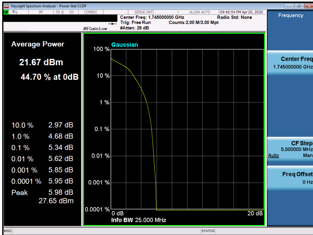
Plot 7-296. PAR Plot (Band 66/4 - 15.0MHz 16-QAM - Full RB Configuration)
