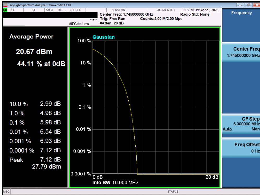
Plot 7-294. PAR Plot (Band 66/4 - 10.0MHz 64-QAM - Full RB Configuration)
