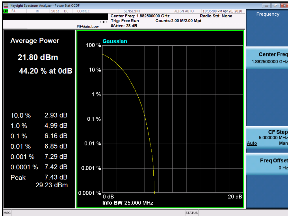
Plot 7-282. PAR Plot (Band 25/2 - 20.0MHz 64-QAM - Full RB Configuration)
