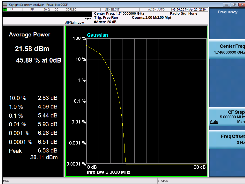
Plot 7-290. PAR Plot (Band 66/4 - 5.0MHz 16-QAM - Full RB Configuration)
