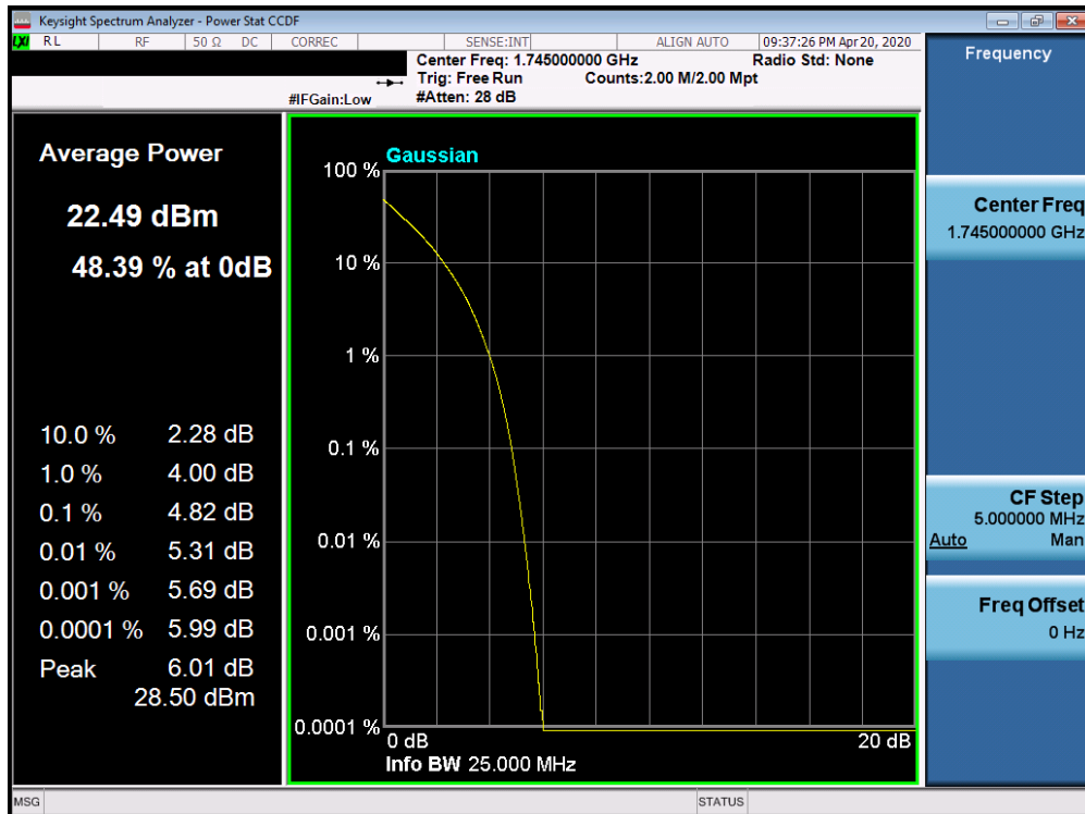
Plot 7-298. PAR Plot (Band 66/4 - 20.0MHz QPSK - Full RB Configuration)
