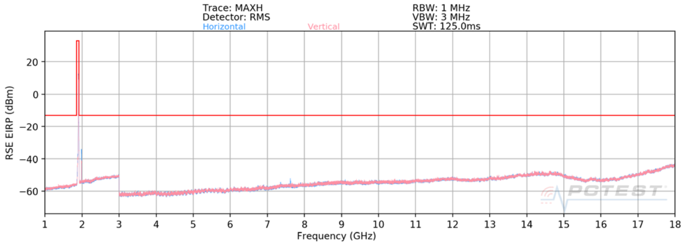
Plot 7-306. Radiated Spurious Plot above 1GHz (Band 25/2)
