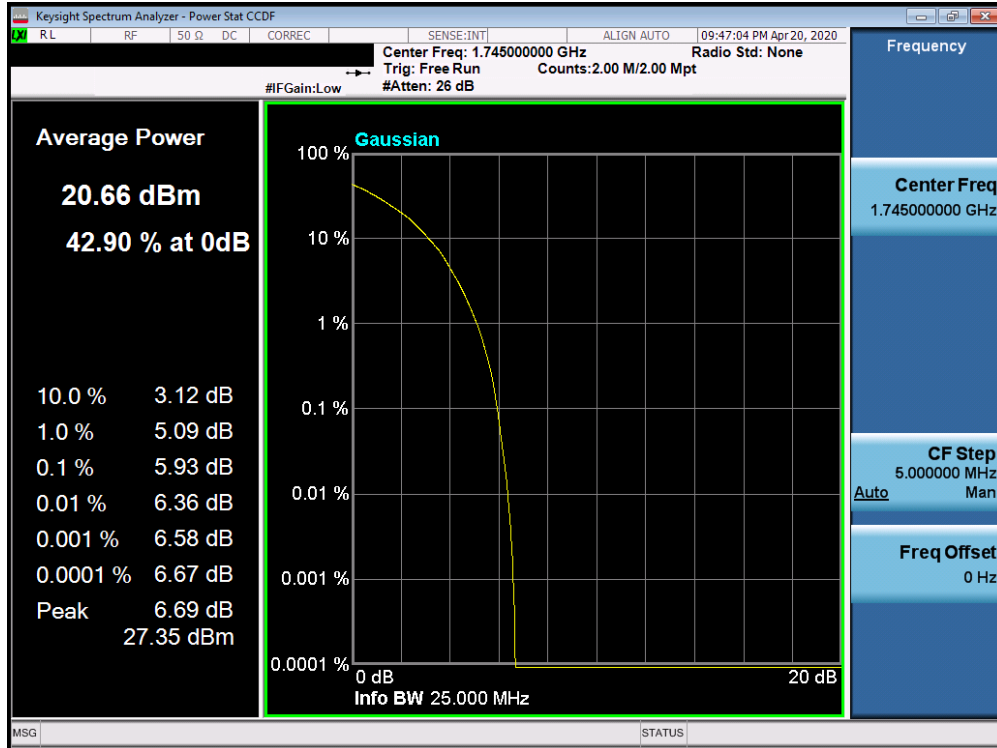
Plot 7-297. PAR Plot (Band 66/4 - 15.0MHz 64-QAM - Full RB Configuration)
