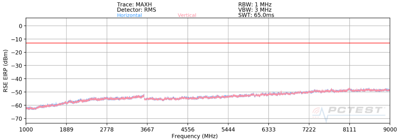
Plot 7-304. Radiated Spurious Plot above 1GHz (Band 26/5)
