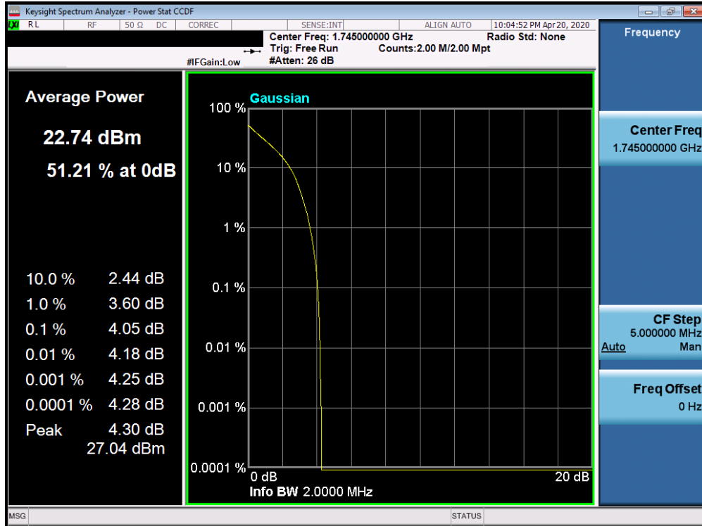
Plot 7-283. PAR Plot (Band 66/4 - 1.4MHz QPSK - Full RB Configuration)
