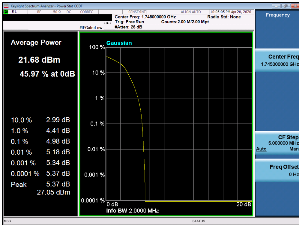
Plot 7-284. PAR Plot (Band 66/4 - 1.4MHz 16-QAM - Full RB Configuration)
