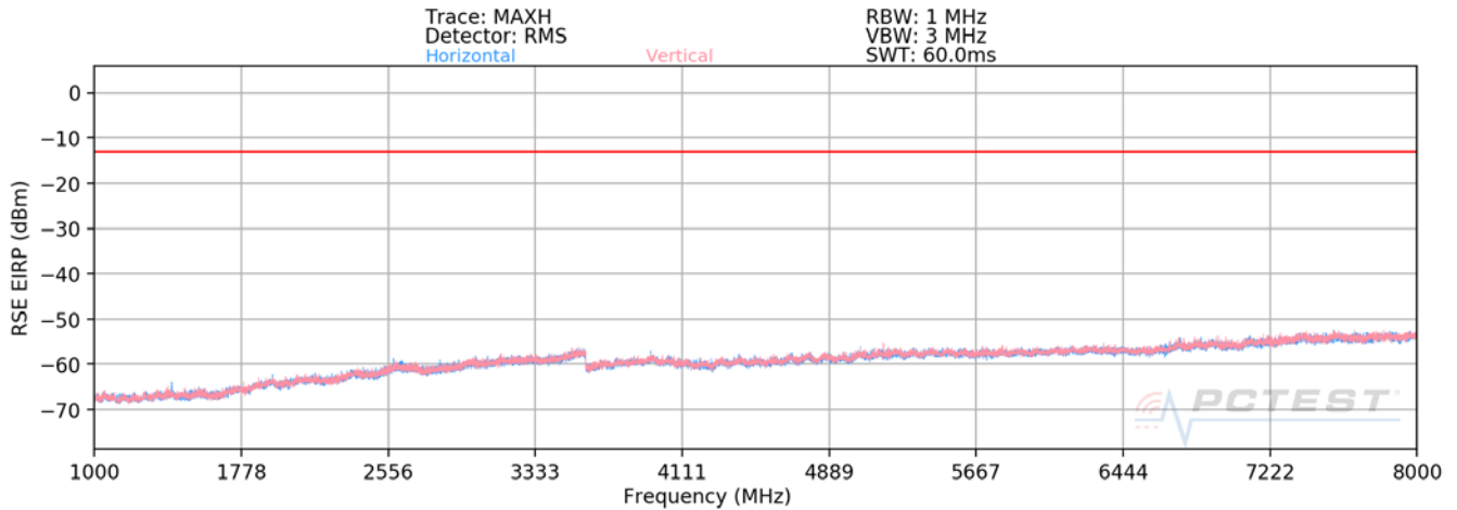
Plot 7-302. Radiated Spurious Plot above 1GHz (Band 12)
