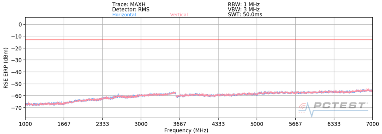
Plot 7-301. Radiated Spurious Plot above 1GHz (Band 71)
