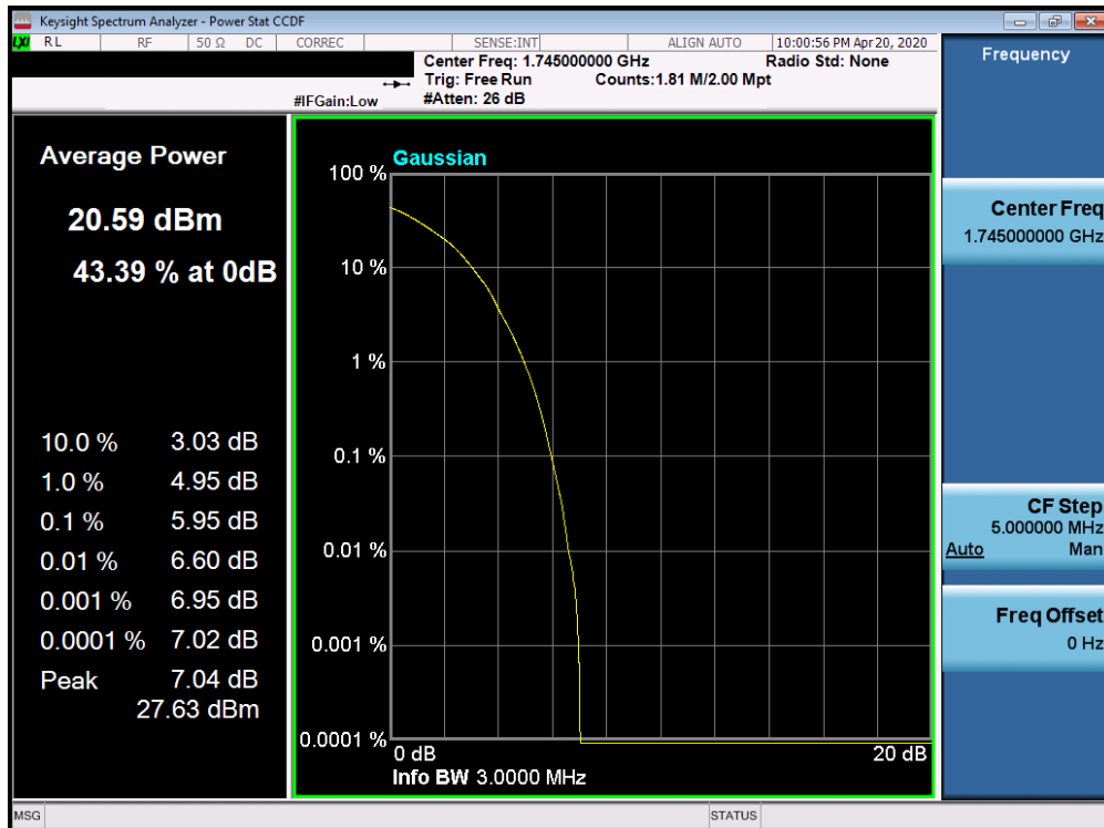
Plot 7-288. PAR Plot (Band 66/4 - 3.0MHz 64-QAM - Full RB Configuration)
