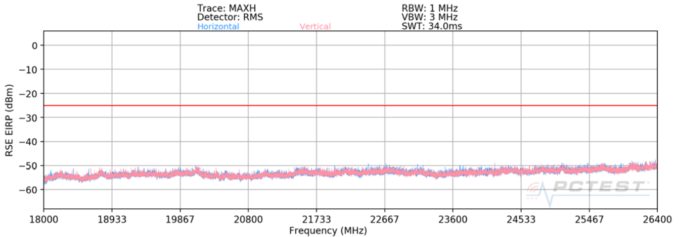
Plot 7-308. Radiated Spurious Plot 18GHz - 26.5GHz (Band 41)
