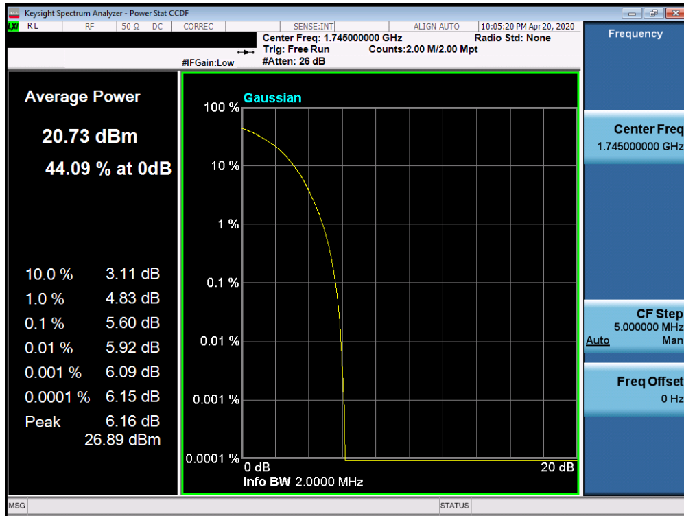
Plot 7-285. PAR Plot (Band 66/4 - 1.4MHz 64-QAM - Full RB Configuration)
