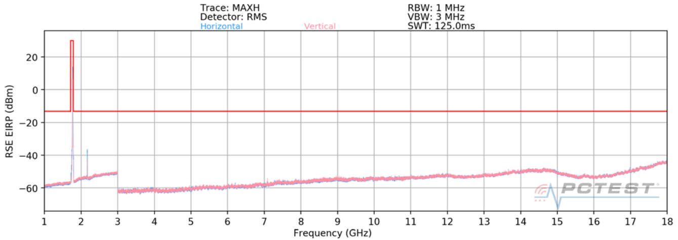
Plot 7-305. Radiated Spurious Plot above 1GHz (Band 66/4)
