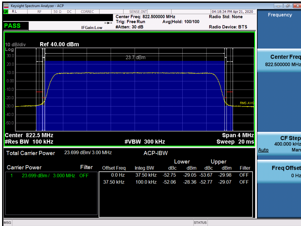
Plot 7-31. Channel Edge Plot (LTE Band 26 – 3.0MHz QPSK – High Channel)
