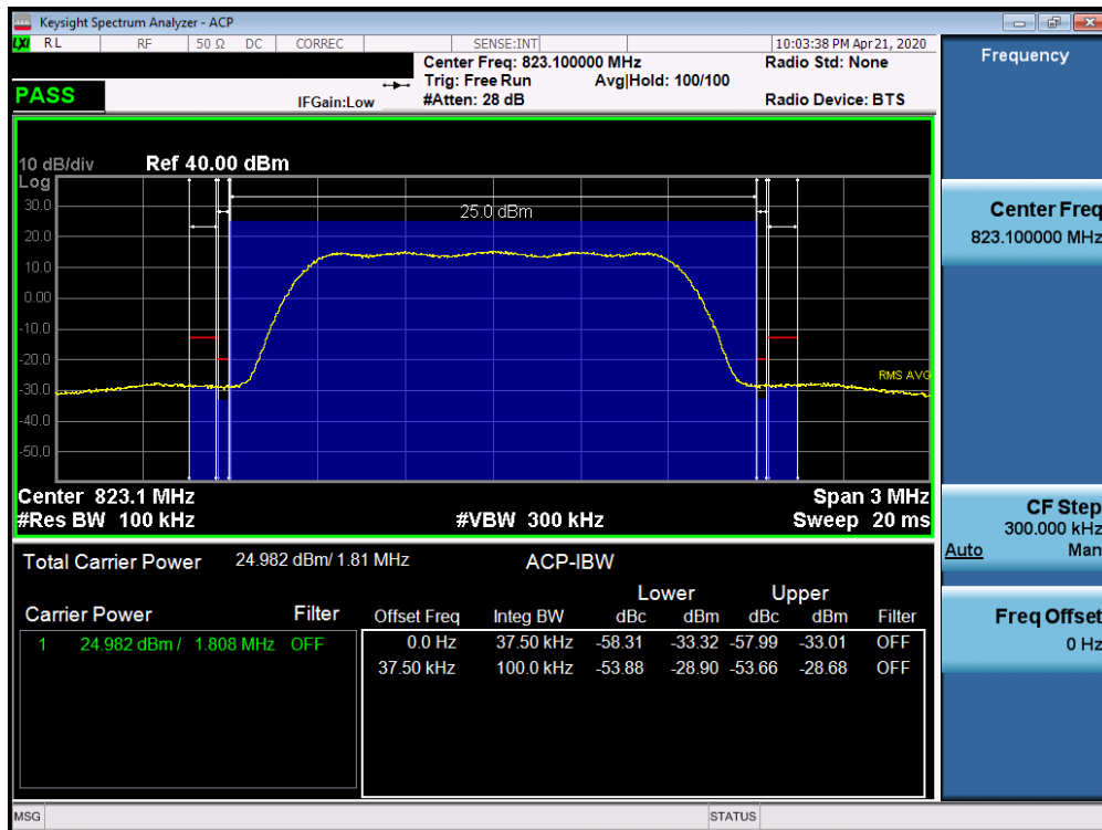
Plot 7-27. Channel Edge Plot (CDMA BC10 - Ch. 684)
