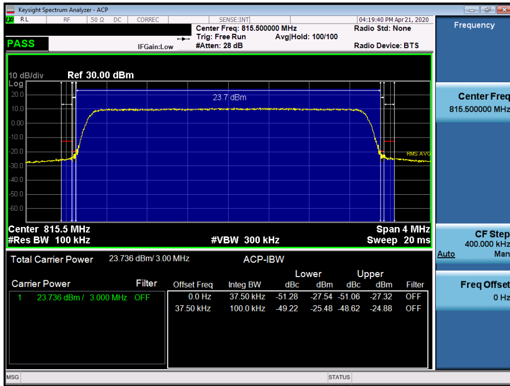
Plot 7-30. Channel Edge Plot (LTE Band 26 – 3.0MHz QPSK – Low Channel)
