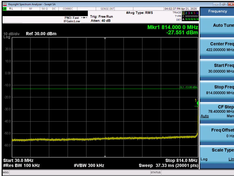
Plot 7-23. Conducted Spurious Plot (LTE Band 26 – 10MHz QPSK Size 1, RB Offset 0- Mid Channel)
