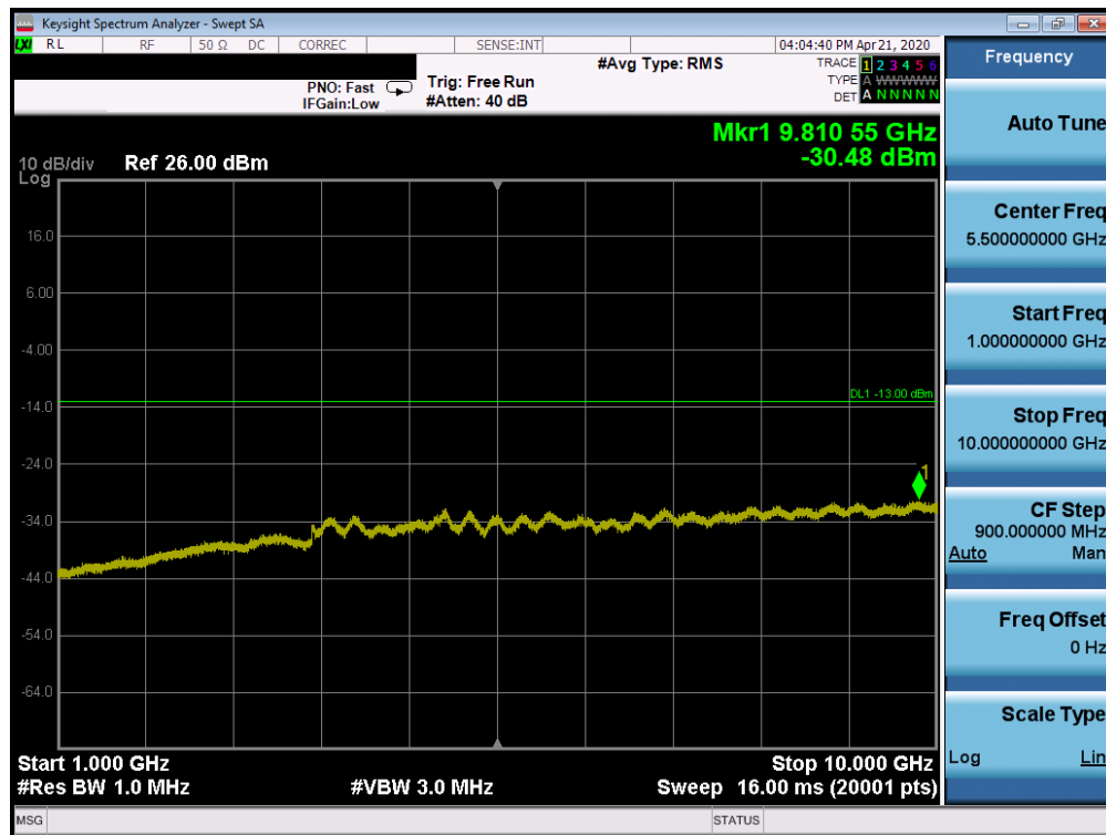
Plot 7-25. Conducted Spurious Plot (LTE Band 26 – 10MHz QPSK Size 1, RB Offset 0- Mid Channel)
