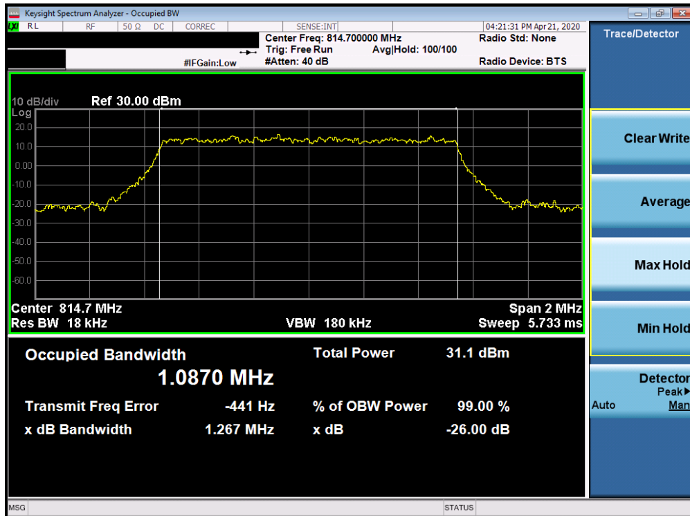
Plot 7-15. Occupied Bandwidth Plot (LTE Band 26 - 1.4MHz 16-QAM - Full RB Configuration)
