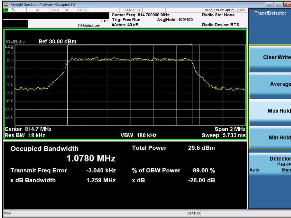
Plot 7-16. Occupied Bandwidth Plot (LTE Band 26 - 1.4MHz 64-QAM - Full RB Configuration)
