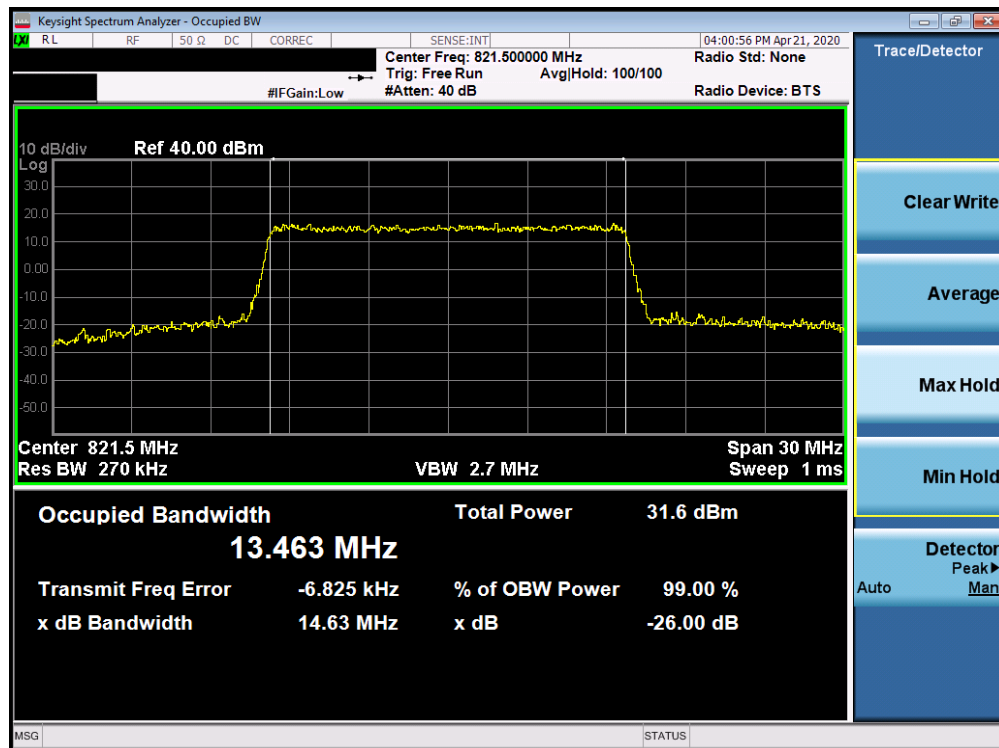
Plot 7-3. Occupied Bandwidth Plot (LTE Band 26 - 15MHz 16-QAM - Full RB Configuration)
