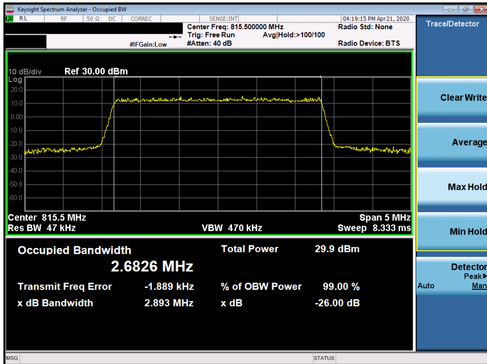
Plot 7-13. Occupied Bandwidth Plot (LTE Band 26 - 3MHz 64-QAM - Full RB Configuration)
