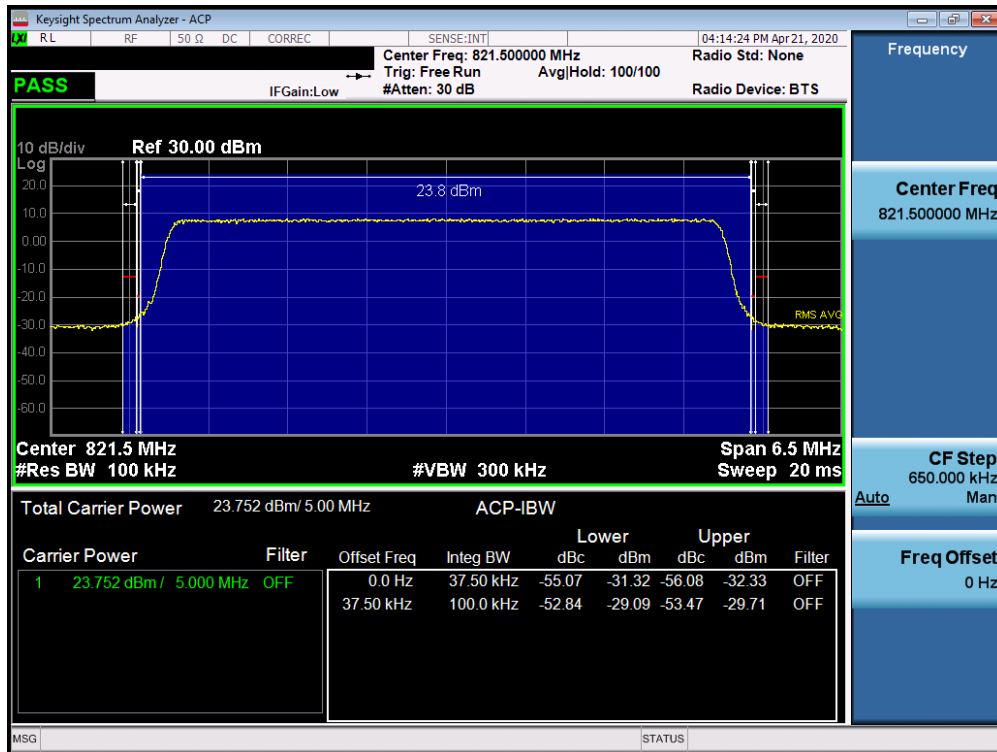
Plot 7-33. Channel Edge Plot (LTE Band 26 – 5MHz QPSK – High Channel)
