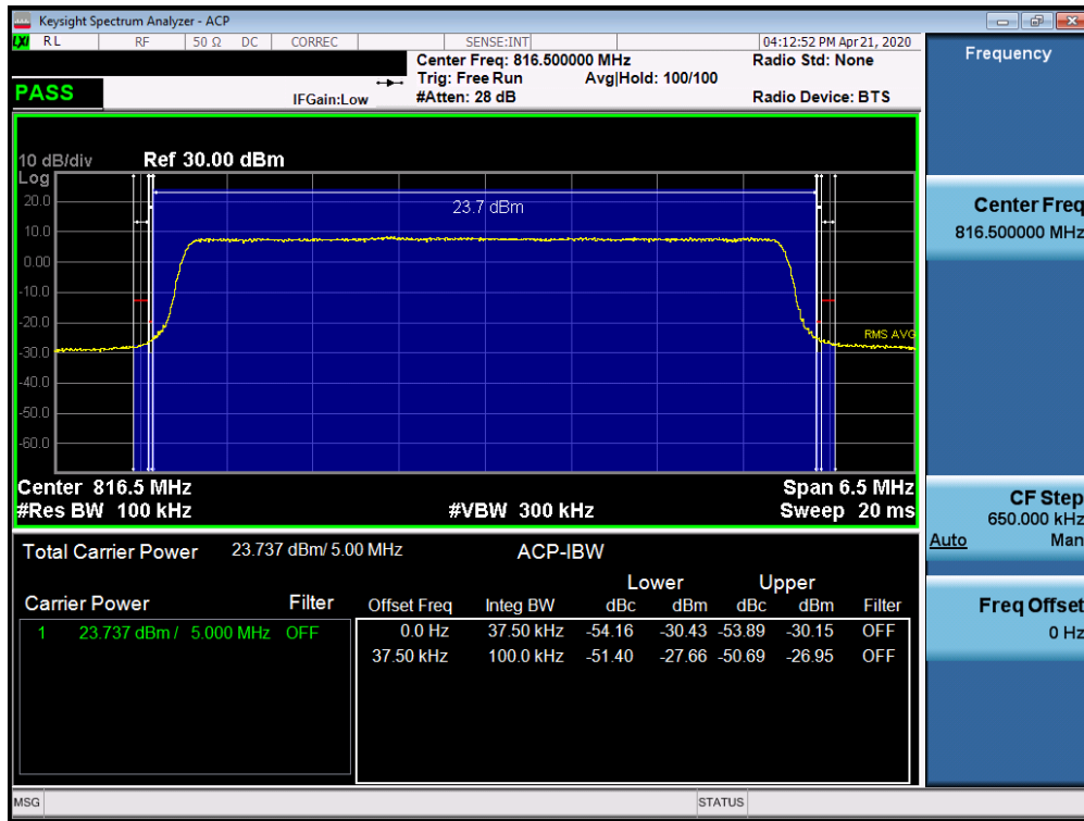
Plot 7-32. Channel Edge Plot (LTE Band 26 – 5MHz QPSK – Low Channel)
