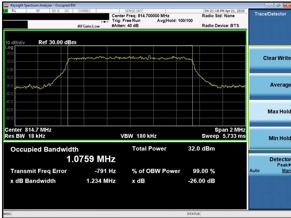
Plot 7-14. Occupied Bandwidth Plot (LTE Band 26 - 1.4MHz QPSK - Full RB Configuration)
