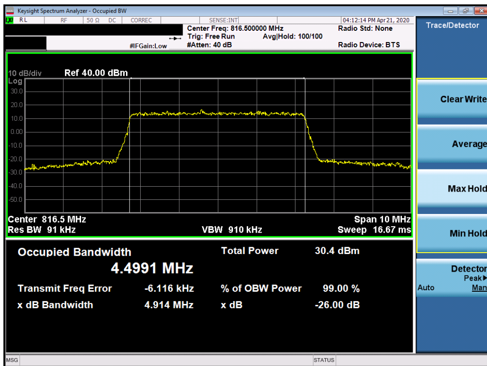
Plot 7-10. Occupied Bandwidth Plot (LTE Band 26 - 5MHz 64-QAM - Full RB Configuration)
