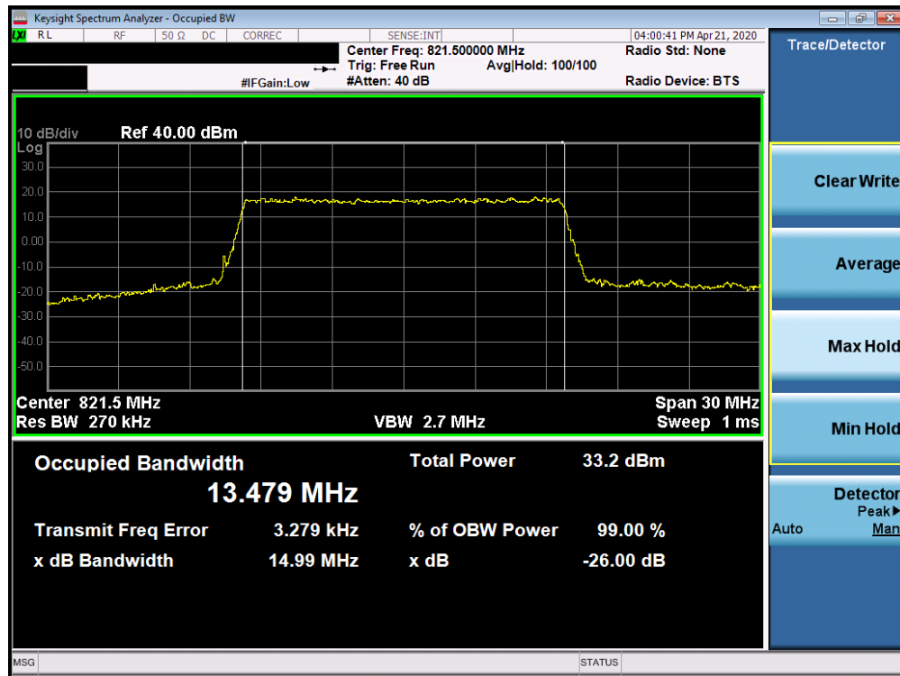
Plot 7-2. Occupied Bandwidth Plot (LTE Band 26 - 15MHz QPSK - Full RB Configuration)
