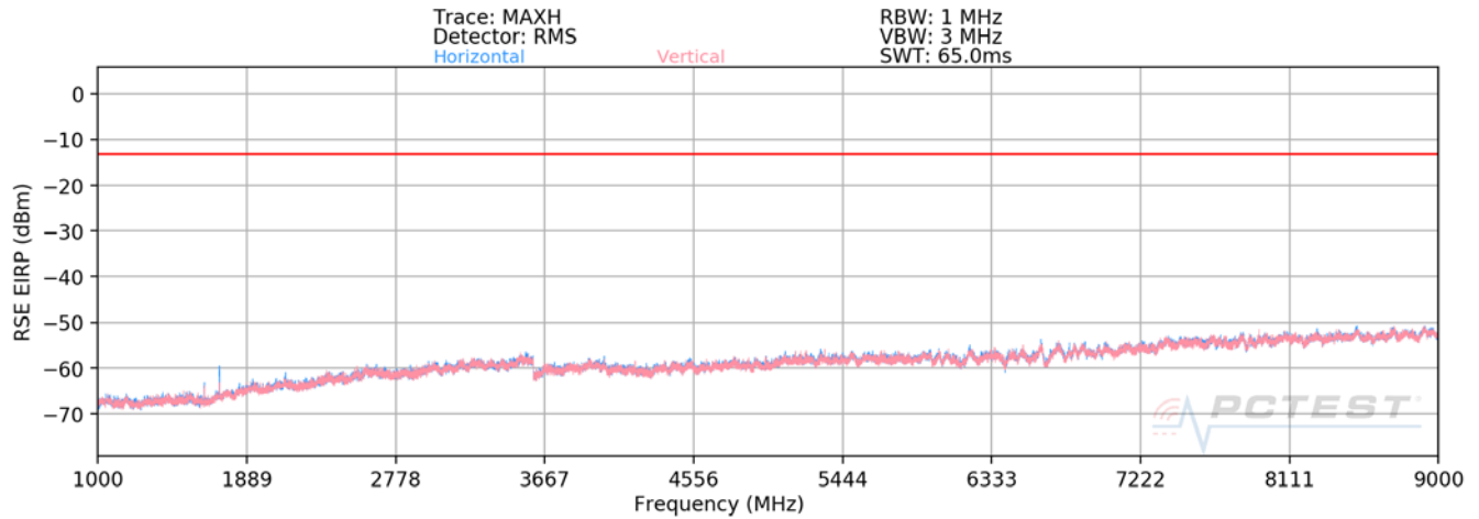
Plot 7-37. Radiated Spurious Plot (CDMA BC10)
