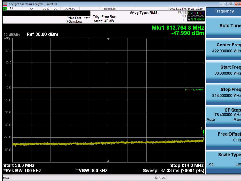
Plot 7-17. Conducted Spurious Plot (CDMA/EvDO, Ch. 476)
