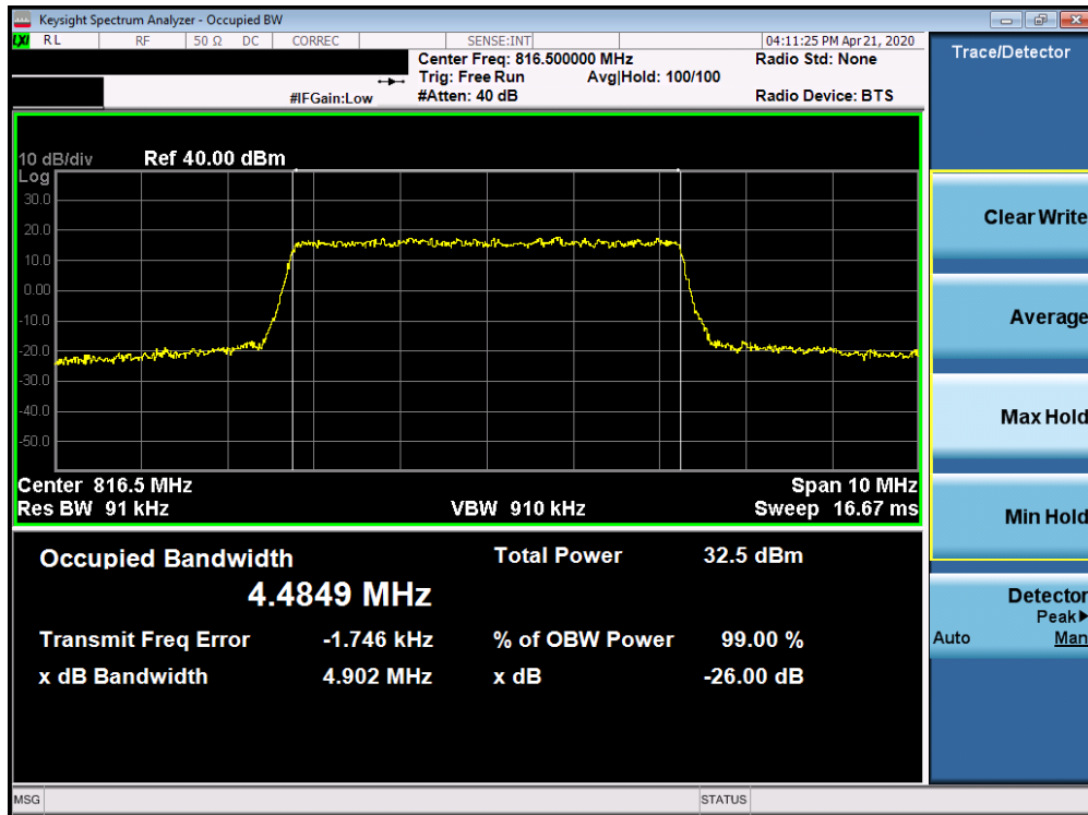
Plot 7-8. Occupied Bandwidth Plot (LTE Band 26 - 5MHz QPSK - Full RB Configuration)
