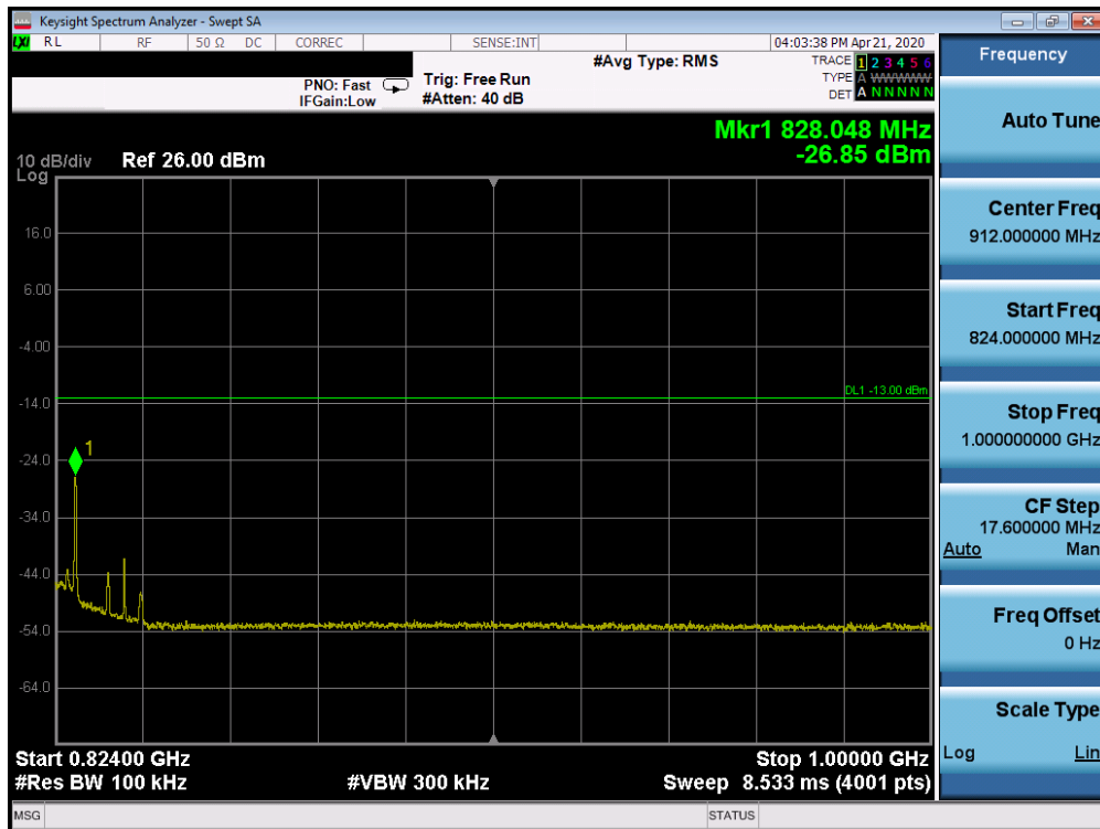
Plot 7-24. Conducted Spurious Plot (LTE Band 26 – 10MHz QPSK Size 1, RB Offset 0- Mid Channel)
