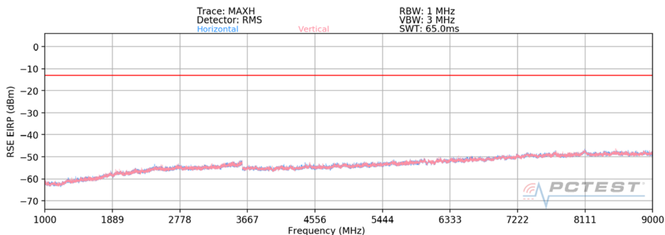
Plot 7-38. Radiated Spurious Plot (Band 26)
