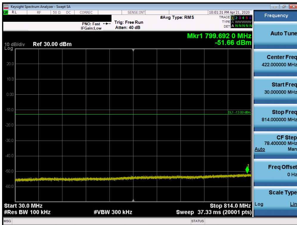
Plot 7-20. Conducted Spurious Plot (CDMA/EvDO, Ch. 684)
