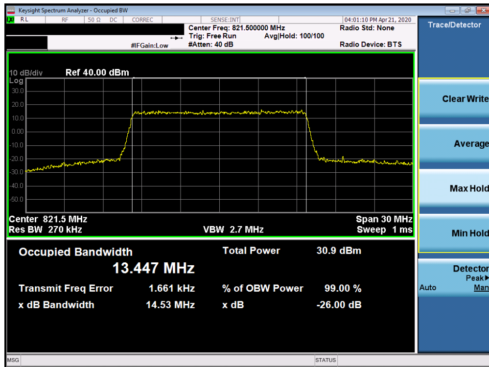
Plot 7-4. Occupied Bandwidth Plot (LTE Band 26 - 15MHz 64-QAM - Full RB Configuration)
