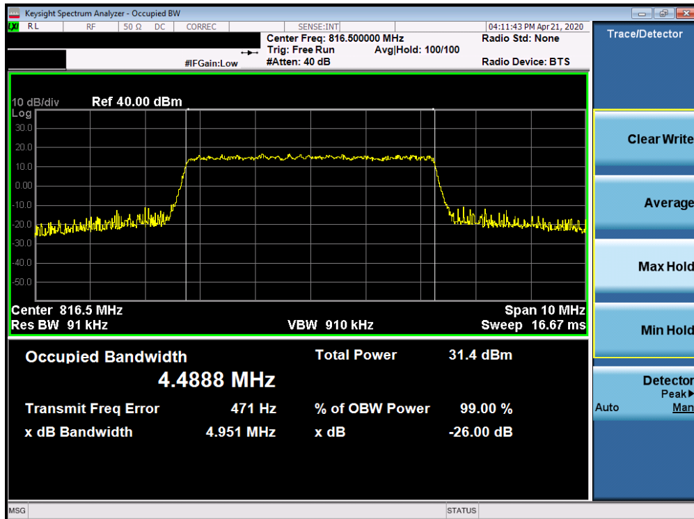
Plot 7-9. Occupied Bandwidth Plot (LTE Band 26 - 5MHz 16-QAM - Full RB Configuration)
