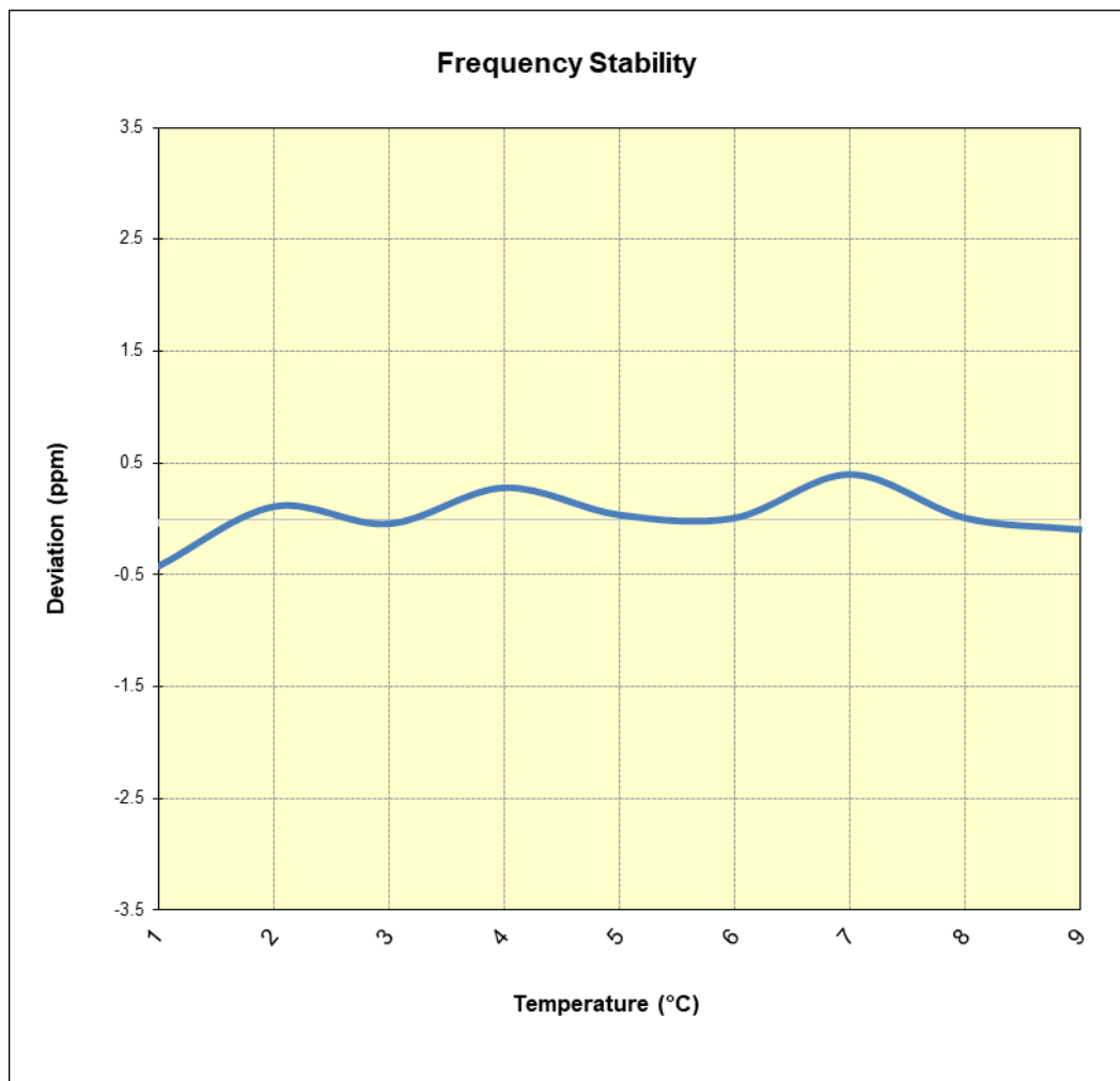
Figure 7-7. CDMA BC10 Frequency Stability Chart
