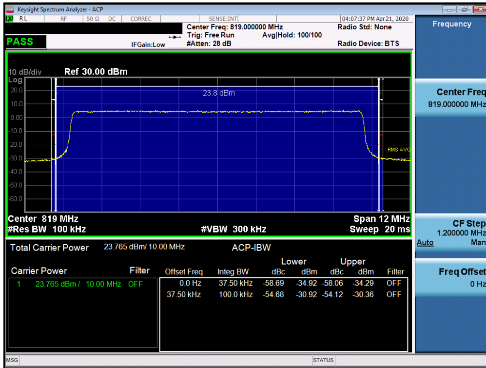
Plot 7-34. Channel Edge Plot (LTE Band 26 – 10MHz QPSK)
