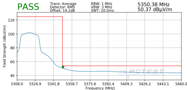
Plot 7-9. Radiated Upper Band Edge Plot (Average – UNII Band 2A)
