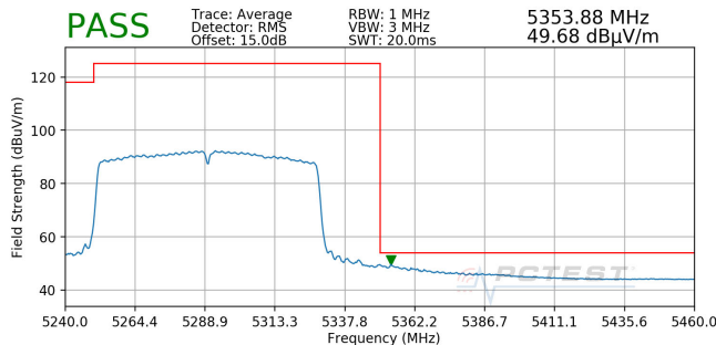
Plot 7-23. Radiated Upper Band Edge Plot (Average – UNII Band 2A)
