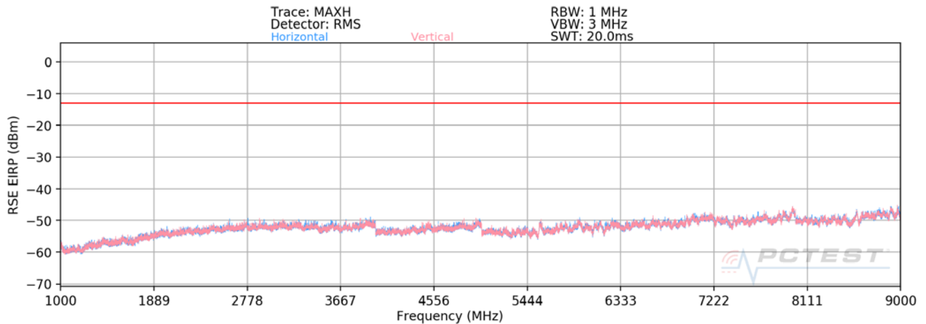
Plot 6-1. Radiated Spurious Plot above 1GHz (CDMA BC10)
