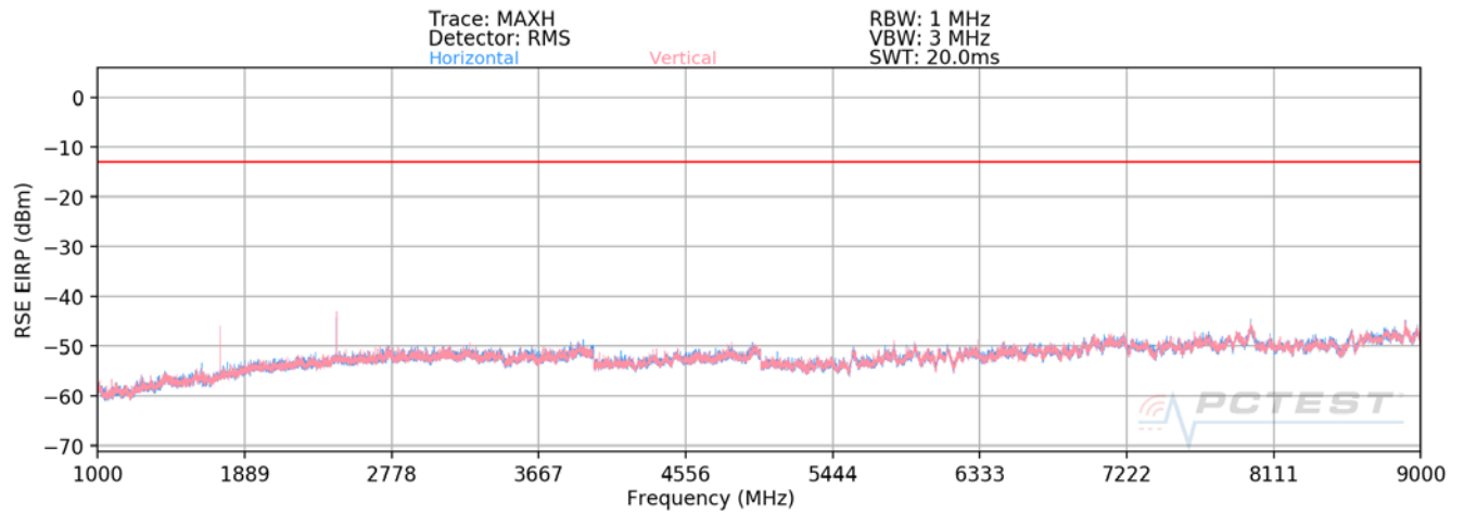
Plot 6-2. Radiated Spurious Plot above 1GHz (LTE B26)
