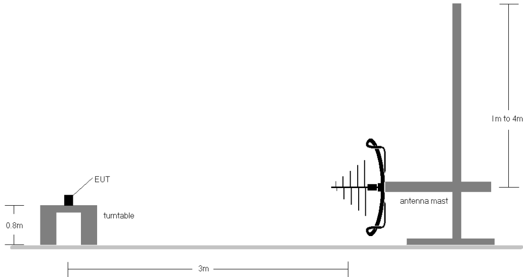
Figure 6-2. Test Instrument & Measurement Setup < 1GHz
