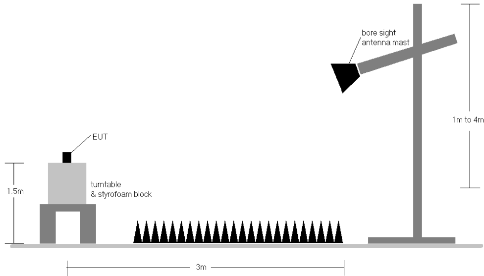
Figure 6-3. Test Instrument & Measurement Setup >1 GHz
