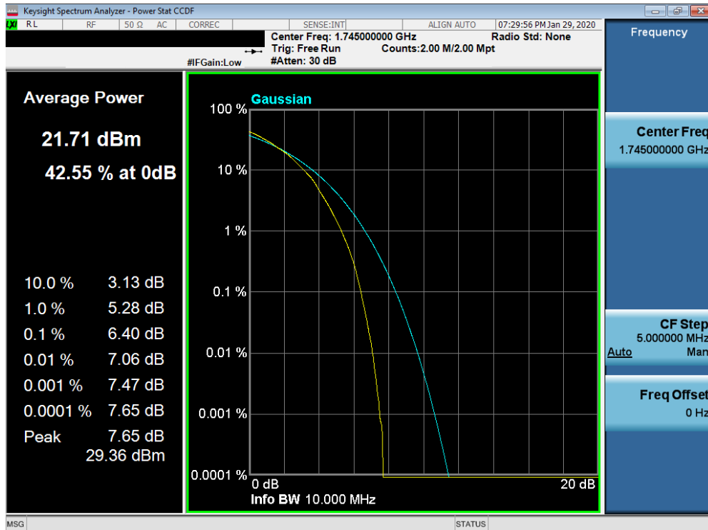
Plot 7-302. PAR Plot (Band 66/4 – 10.0MHz 64QAM - Full RB Configuration)
