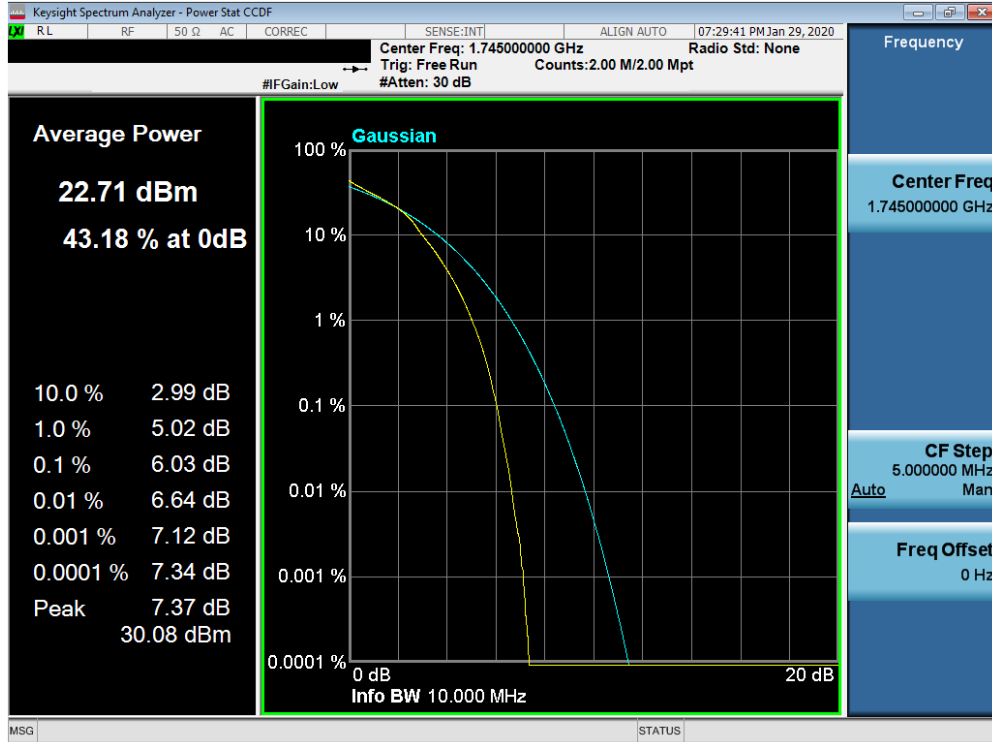
Plot 7-301. PAR Plot (Band 66/4 – 10.0MHz 16QAM - Full RB Configuration)
