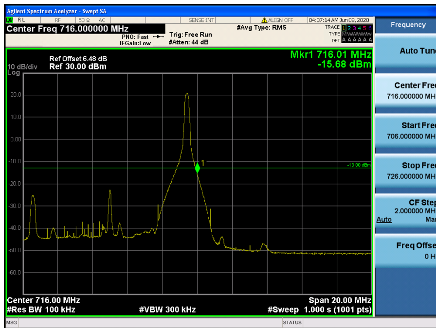
LTE Band 12, 17 / 10 MHz / 64QAM - RB Size/Offset (1/49)
