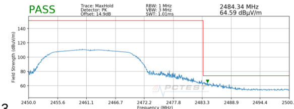
Plot 7-38. Radiated Restricted Upper Band Edge Measurement (Peak)
