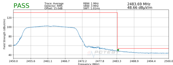
Plot 7-37. Radiated Restricted Upper Band Edge Measurement (Average)
