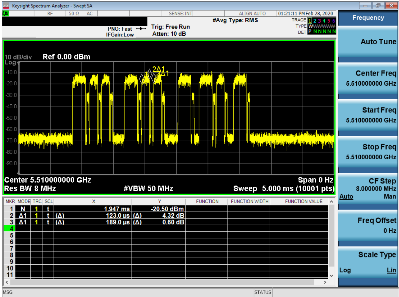
Figure 7-1. Band 2C Period
