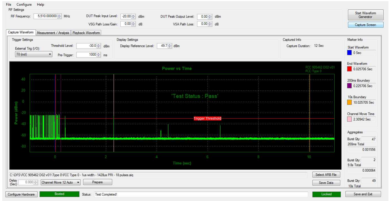
Figure 7-2. Band 2C Move Time and Aggregate Time
