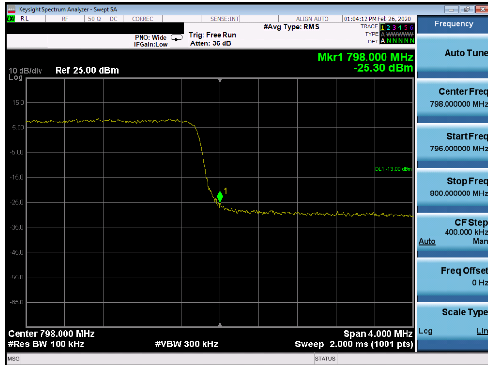
Plot 7-10. Upper Band Edge Plot (Band 14 - 5MHz QPSK - Full RB Configuration)
