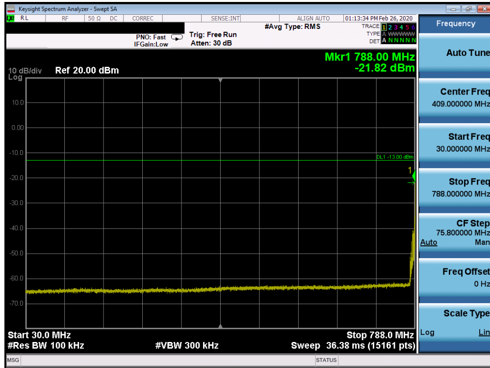
Plot 7-5. Conducted Spurious Plot (Band 14 - 10MHz QPSK - RB Size 1, RB Offset 0 - Mid Channel)
