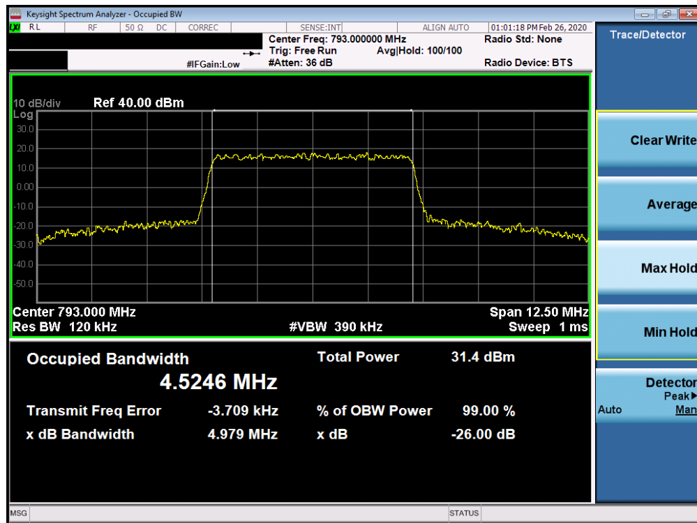
Plot 7-4. Occupied Bandwidth Plot (Band 14 - 5MHz 16-QAM - Full RB Configuration)
