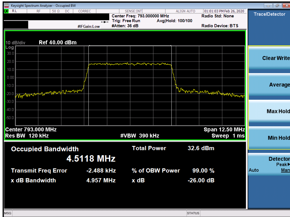
Plot 7-3. Occupied Bandwidth Plot (Band 14 - 5MHz QPSK - Full RB Configuration)
