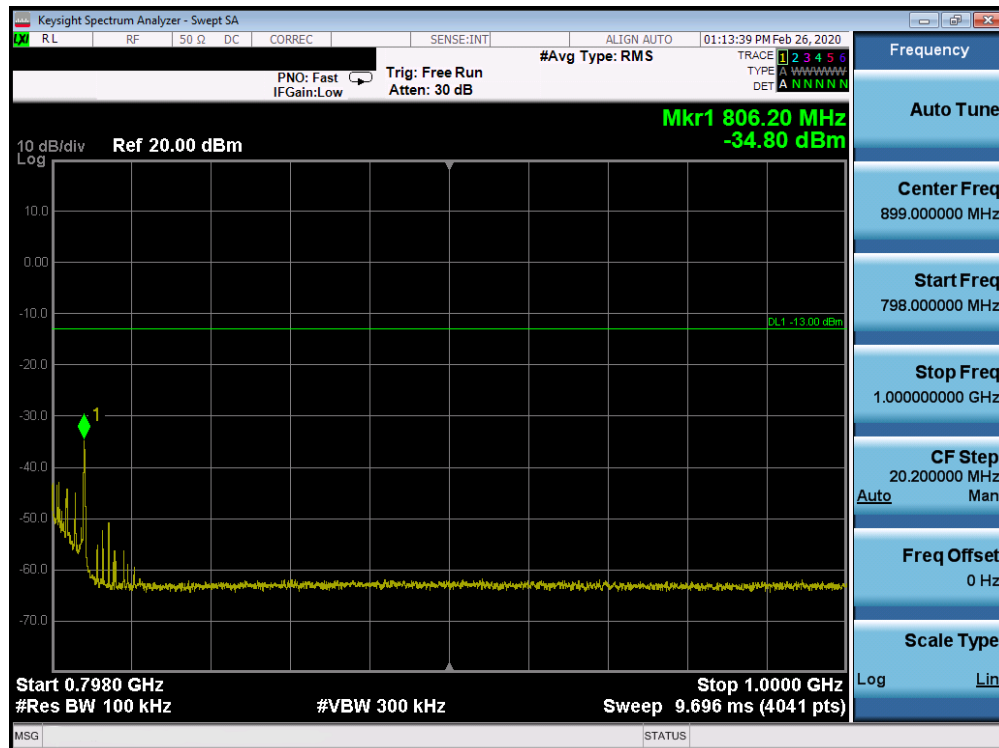
Plot 7-6. Conducted Spurious Plot (Band 14 - 10MHz QPSK - RB Size 1, RB Offset 0 - Mid Channel)
