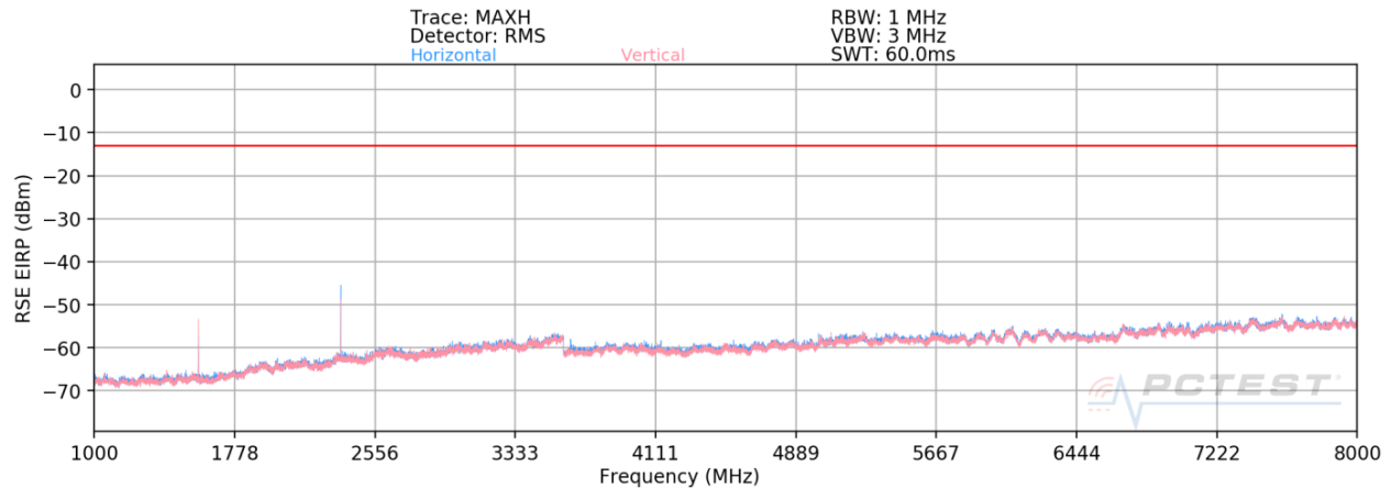
Plot 7-17. Radiated Spurious Plot (Band 14)
