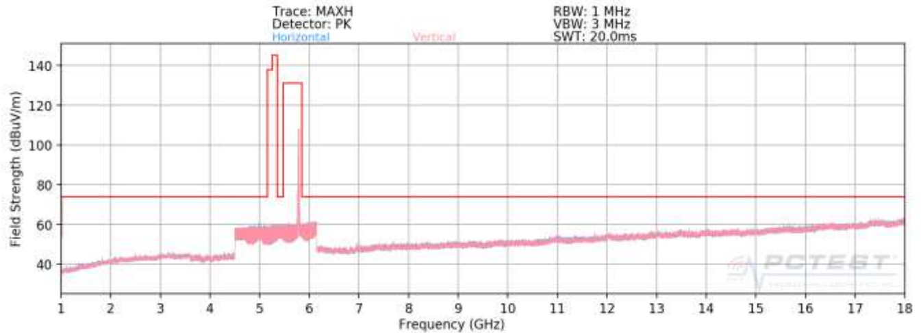
Plot 7-80. Radiated Spurious Plot above 1GHz (802.11a – U3 Ch. 157)
