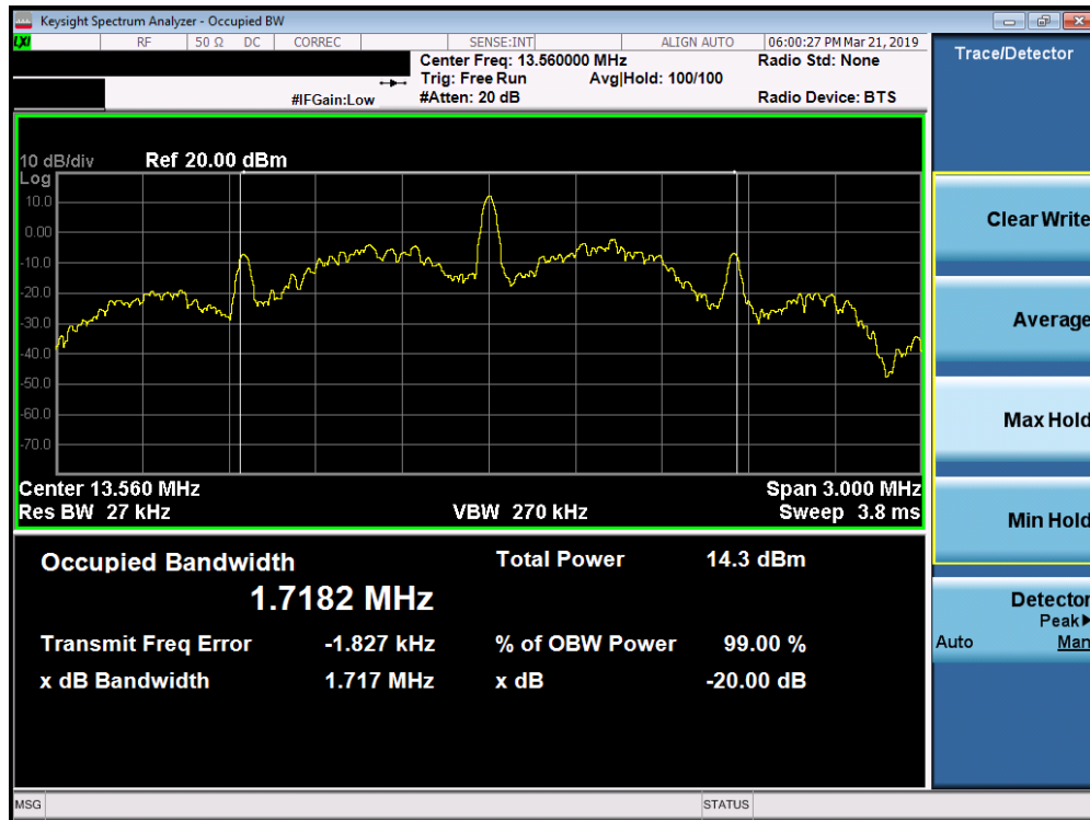
Figure 7-2. Bandwidth Plot
