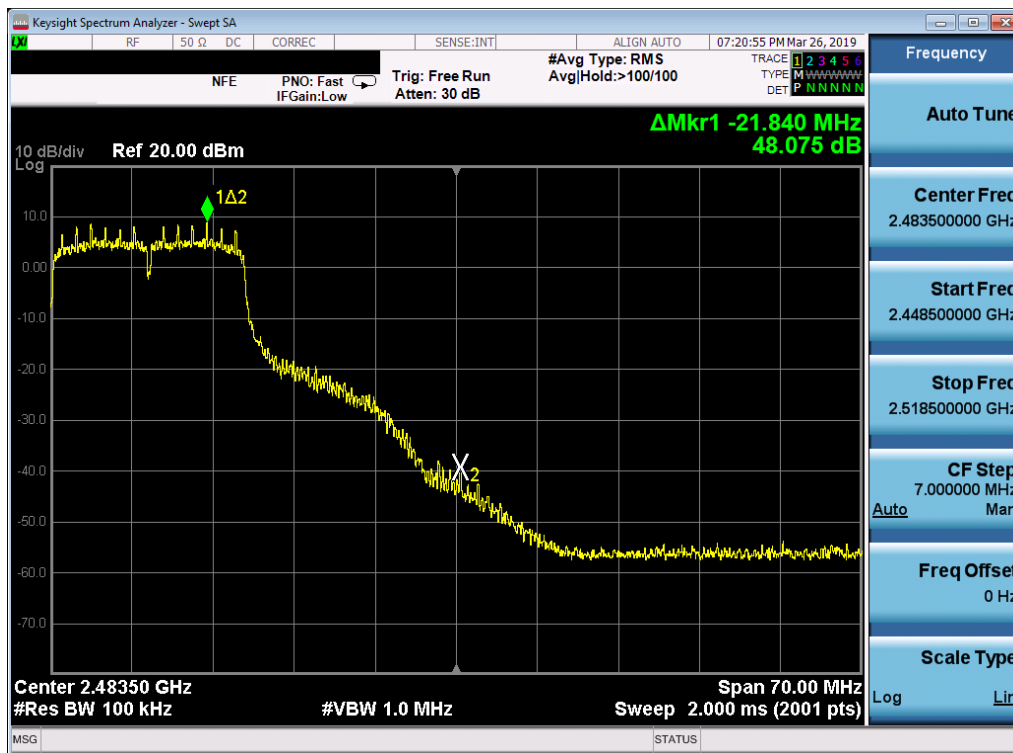
Plot 7-29. Band Edge Plot (802.11g - Ch. 10)
