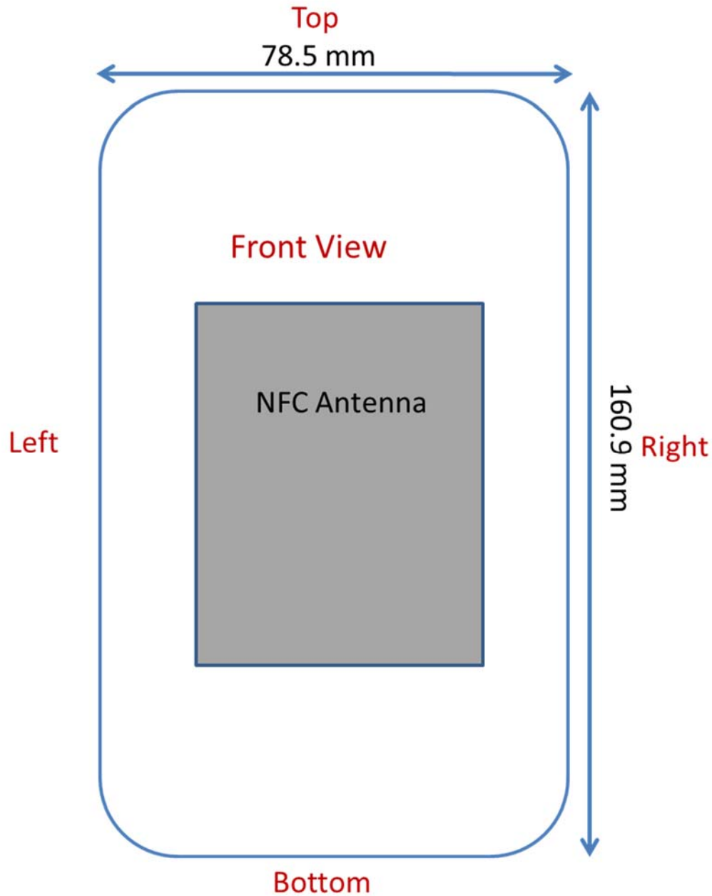
Figure F-2 NFC Antenna Locations
