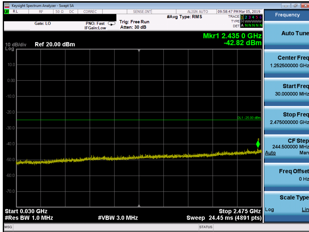
Plot 7-148. Conducted Spurious Plot (Band 41 - 15.0MHz QPSK - RB Size 1, RB Offset 0 - Low Channel)
