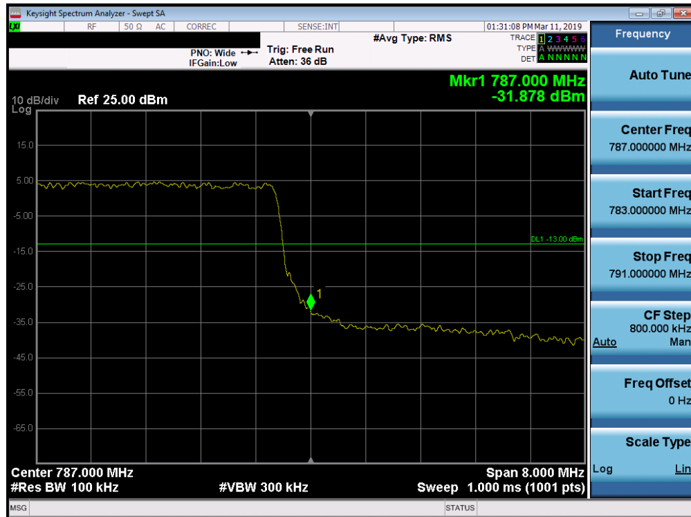
Plot 7-181. Upper Band Edge Plot (Band 13 - 10.0MHz QPSK - Full RB Configuration)
