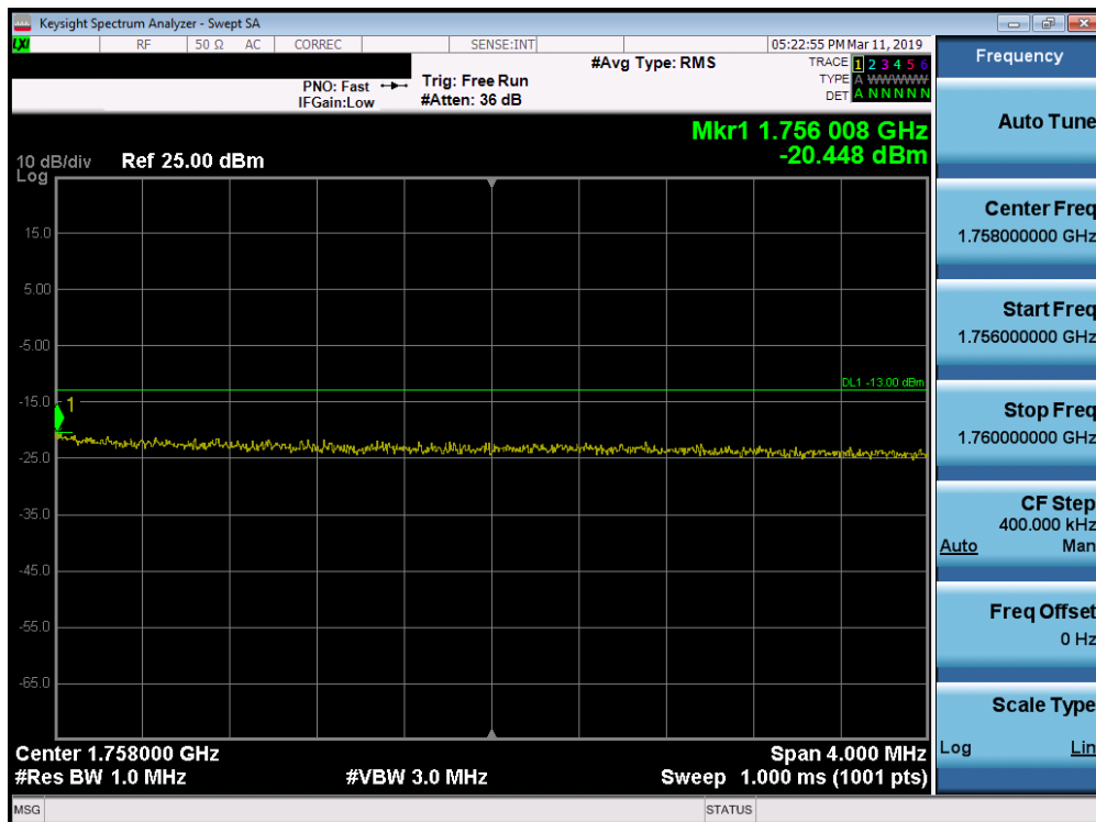
Plot 7-214. Upper Extended Band Edge Plot (Band 4 - 10.0MHz QPSK - Full RB Configuration)
