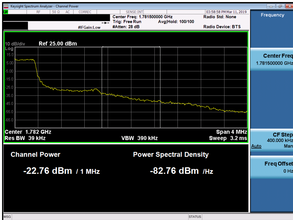
Plot 7-198. Upper Extended Band Edge Plot (Band 66 - 1.4MHz QPSK - Full RB Configuration)
