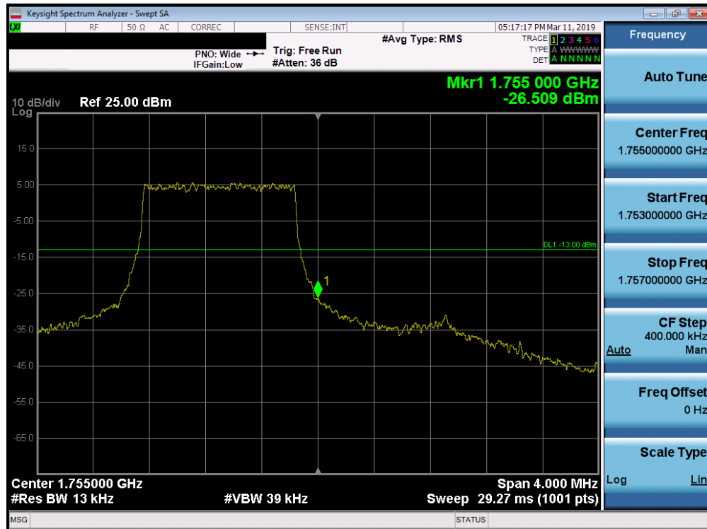
Plot 7-195. Upper Band Edge Plot (Band 4 - 1.4MHz QPSK - Full RB Configuration)
