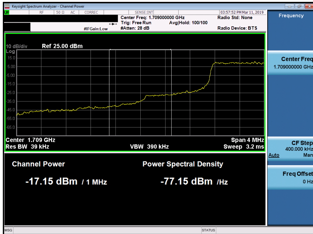
Plot 7-194. Lower Extended Band Edge Plot (Band 66/4 - 1.4MHz QPSK - Full RB Configuration)
