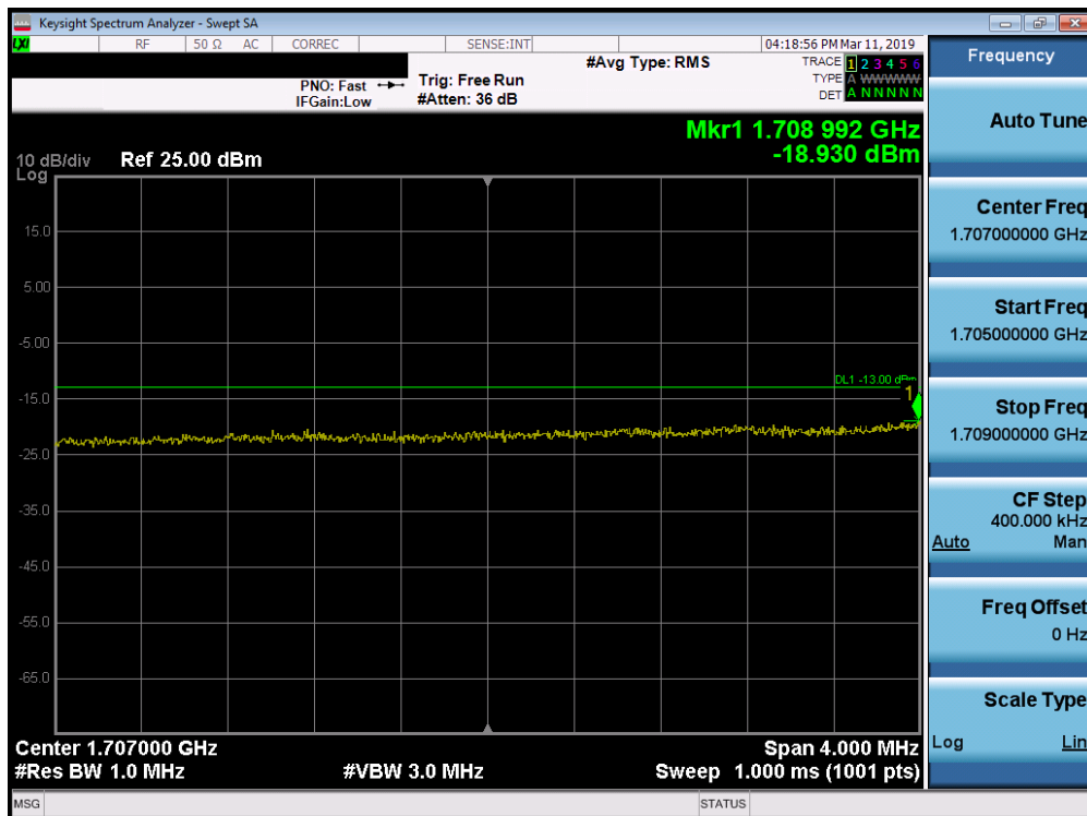
Plot 7-212. Lower Extended Band Edge Plot (Band 66/4 - 10.0MHz QPSK - Full RB Configuration)
