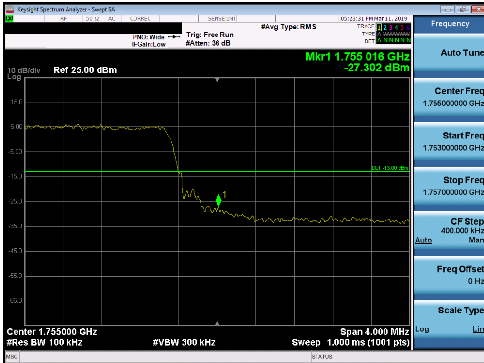
Plot 7-213. Upper Band Edge Plot (Band 4 - 10.0MHz QPSK - Full RB Configuration)
