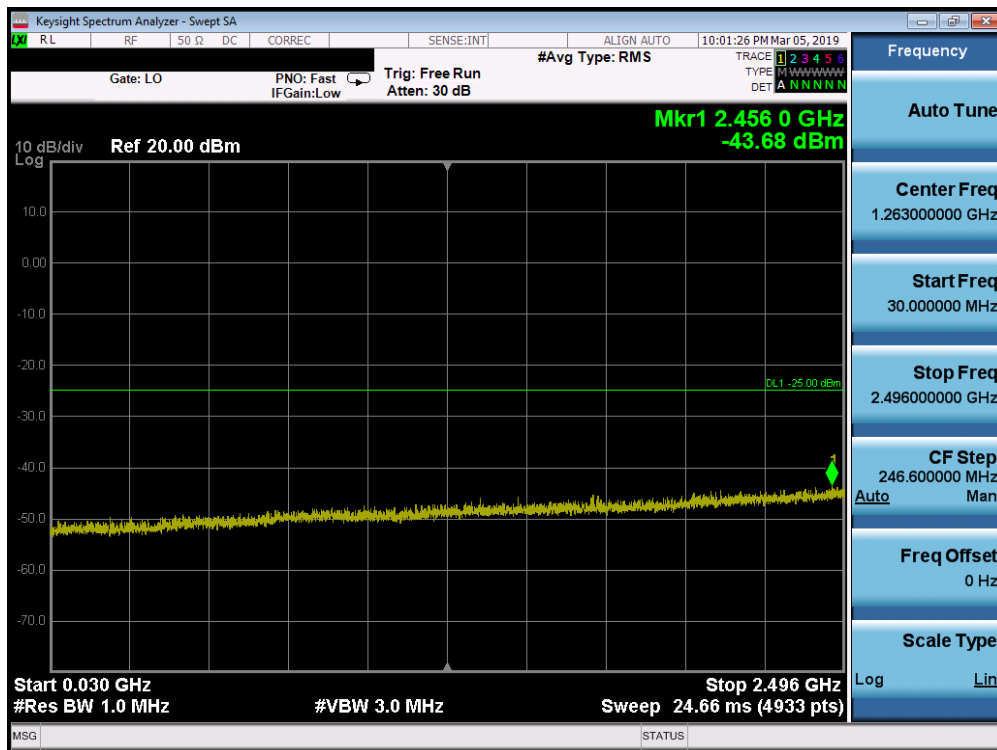
Plot 7-151. Conducted Spurious Plot (Band 41 - 15.0MHz QPSK - RB Size 1, RB Offset 0 - Mid Channel)
