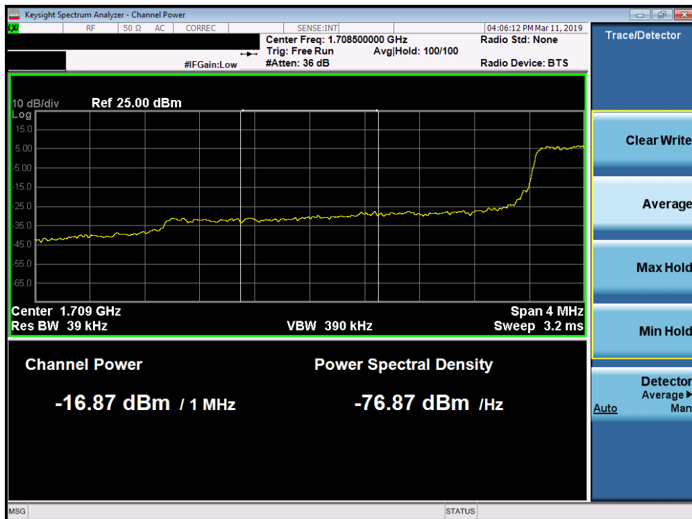
Plot 7-200. Lower Extended Band Edge Plot (Band 66/4 - 3.0MHz QPSK - Full RB Configuration)
