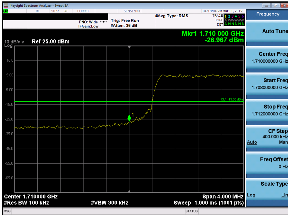
Plot 7-211. Lower Band Edge Plot (Band 66/4 - 10.0MHz QPSK - Full RB Configuration)
