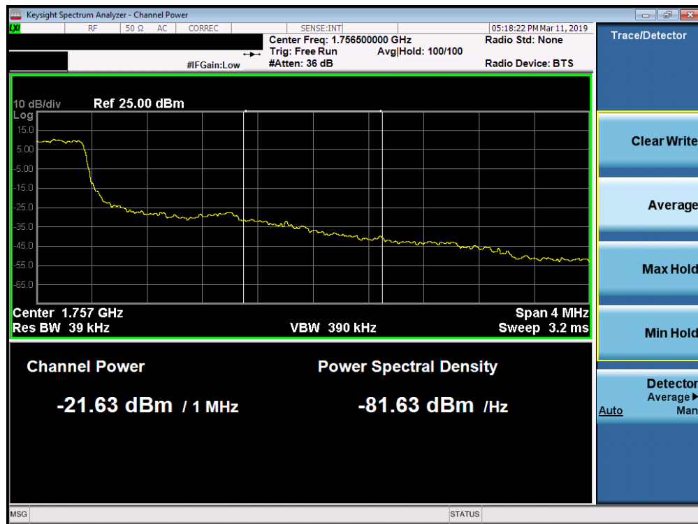
Plot 7-196. Upper Extended Band Edge Plot (Band 4 - 1.4MHz QPSK - Full RB Configuration)
