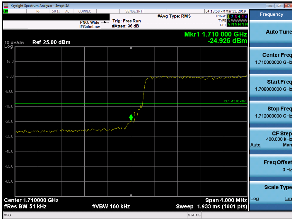
Plot 7-205. Lower Band Edge Plot (Band 66/4 - 5.0MHz QPSK - Full RB Configuration)
