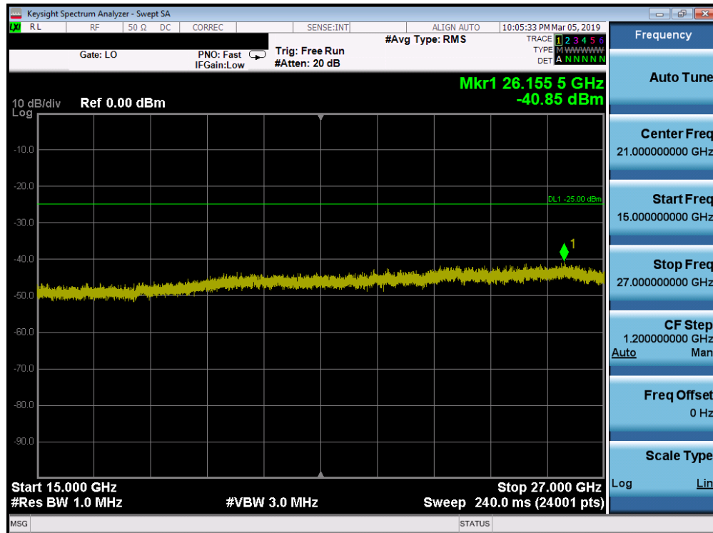
Plot 7-156. Conducted Spurious Plot (Band 41 - 15.0MHz QPSK - RB Size 1, RB Offset 0 - High Channel)
