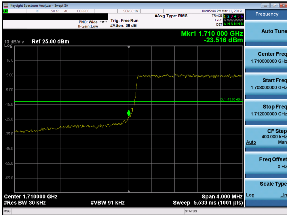
Plot 7-199. Lower Band Edge Plot (Band 66/4 - 3.0MHz QPSK - Full RB Configuration)
