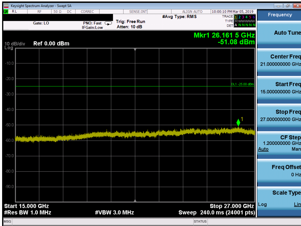
Plot 7-150. Conducted Spurious Plot (Band 41 - 15.0MHz QPSK - RB Size 1, RB Offset 0 - Low Channel)
