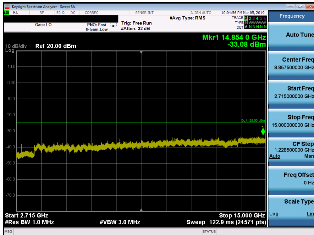
Plot 7-155. Conducted Spurious Plot (Band 41 - 15.0MHz QPSK - RB Size 1, RB Offset 0 - High Channel)
