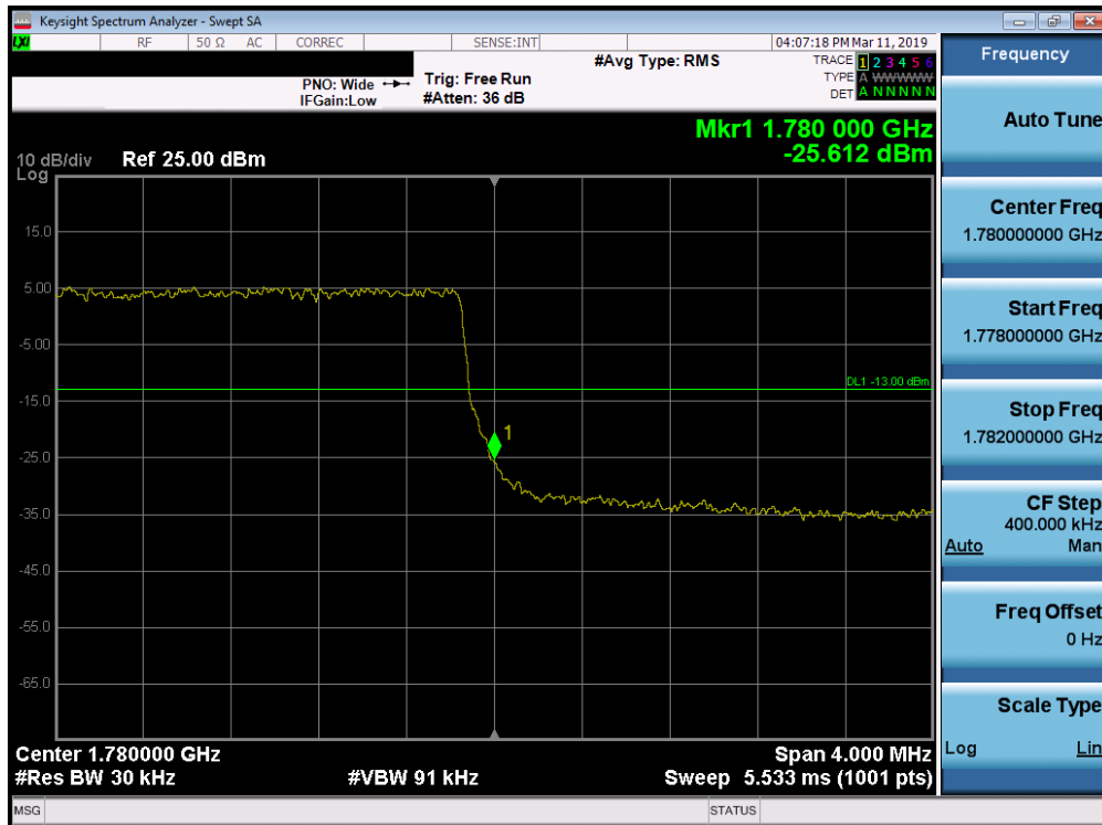
Plot 7-203. Upper Band Edge Plot (Band 66 - 3.0MHz QPSK - Full RB Configuration)
