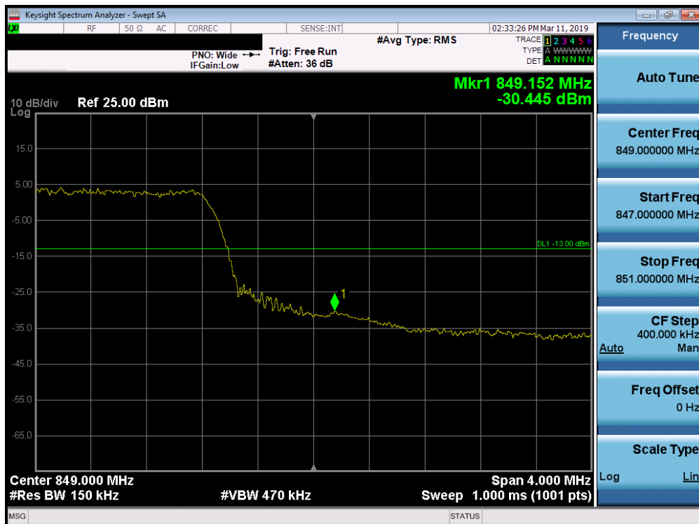
Plot 7-192. Upper Band Edge Plot (Band 26 - 15.0MHz QPSK - Full RB Configuration)
