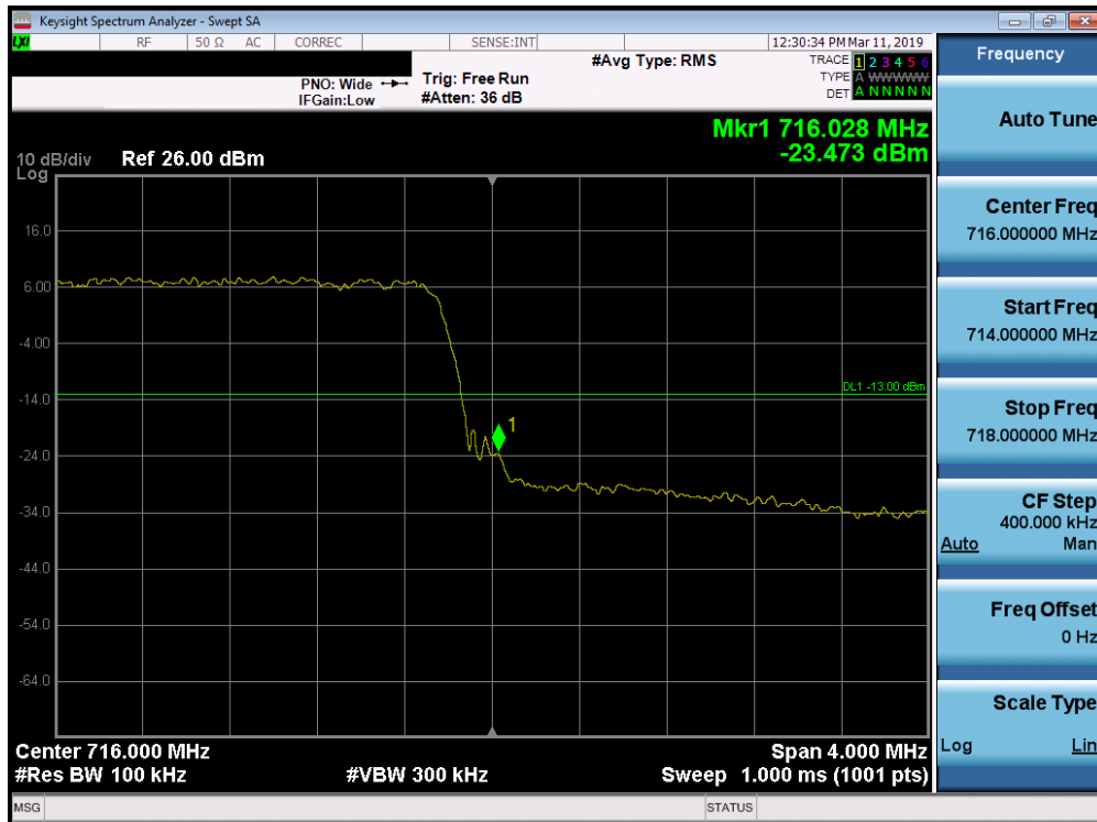
Plot 7-171. Upper Band Edge Plot (Band 12/17 - 5.0MHz QPSK - Full RB Configuration)
