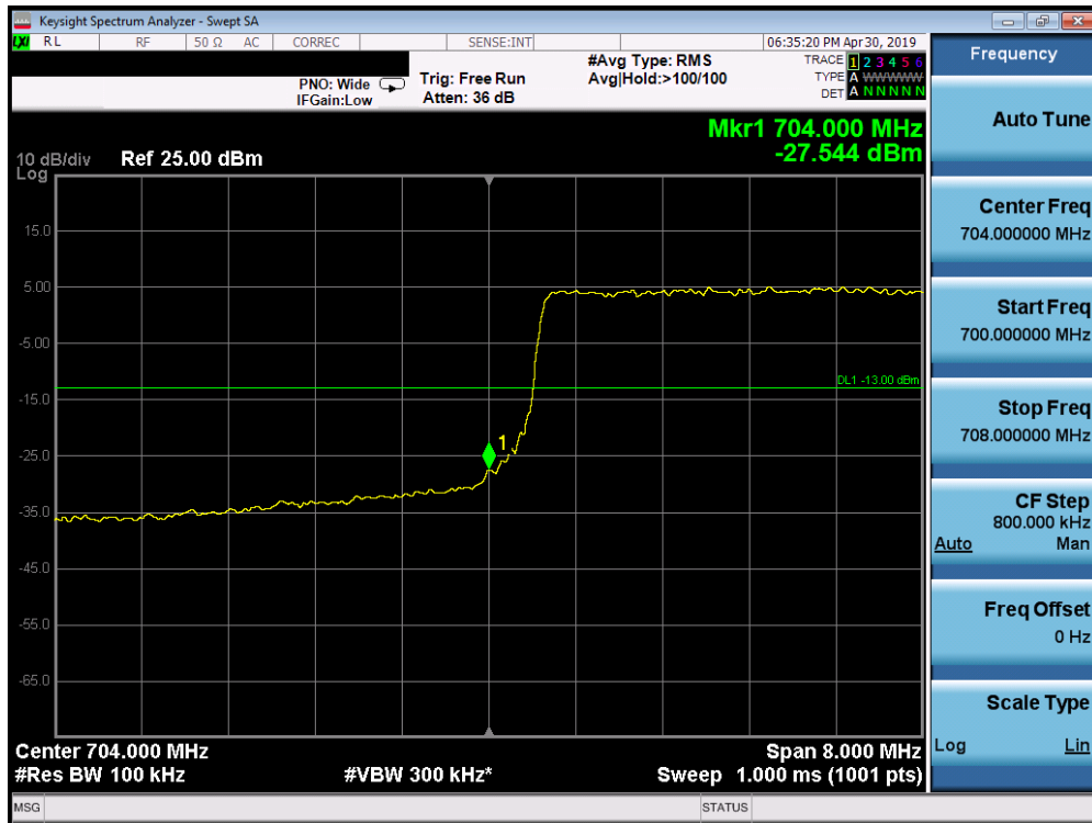
Plot 7-173. Lower Band Edge Plot (Band 17 - 10.0MHz QPSK - Full RB Configuration)
