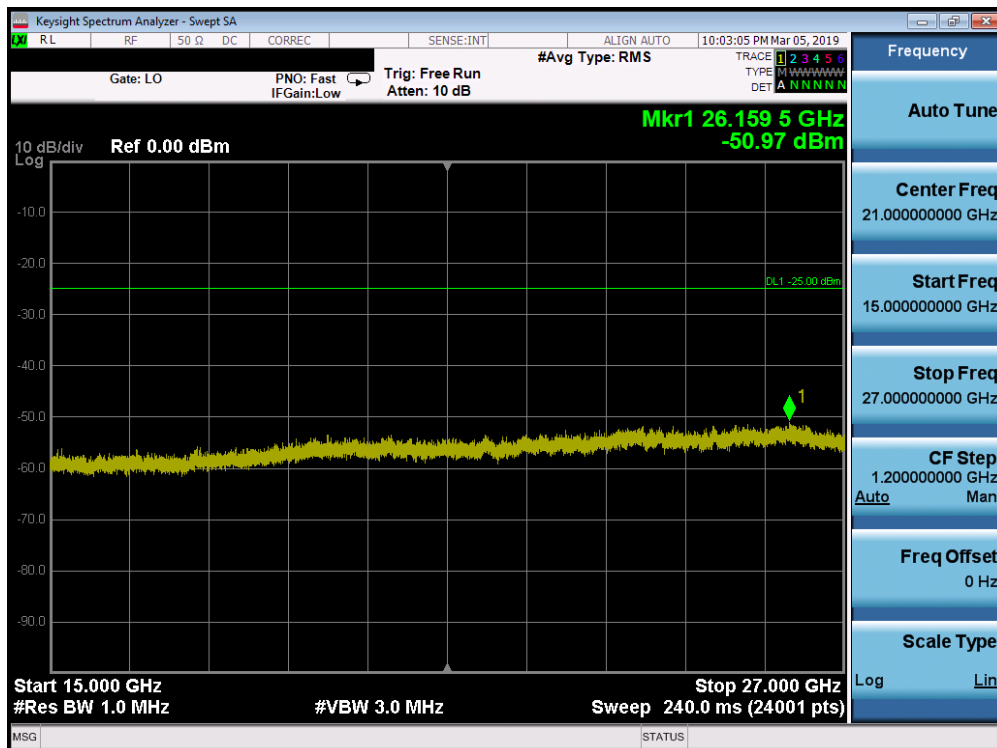
Plot 7-153. Conducted Spurious Plot (Band 41 - 15.0MHz QPSK - RB Size 1, RB Offset 0 - Mid Channel)
