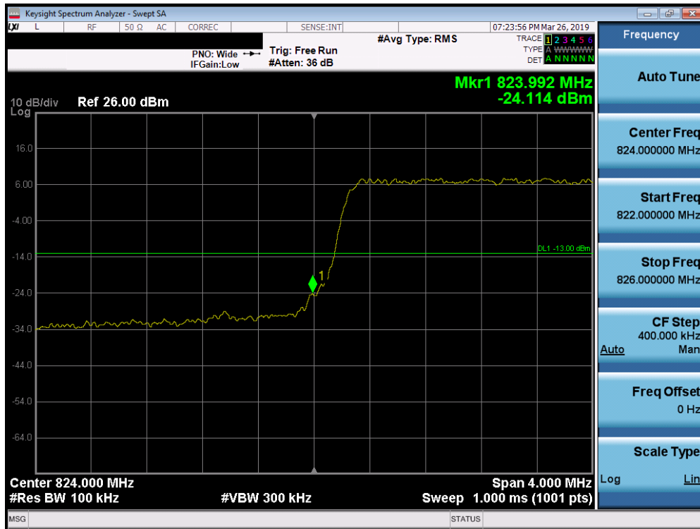
Plot 7-187. Lower Band Edge Plot (Band 26/5 - 5.0MHz QPSK - Full RB Configuration)
