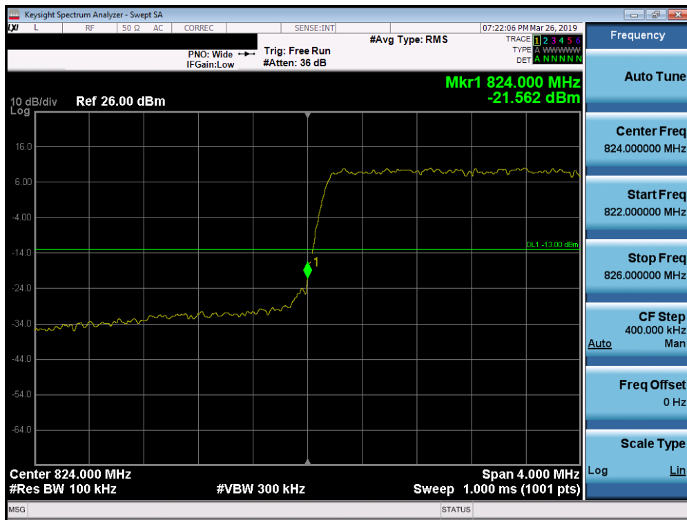
Plot 7-185. Lower Band Edge Plot (Band 26/5 - 3.0MHz QPSK - Full RB Configuration)
