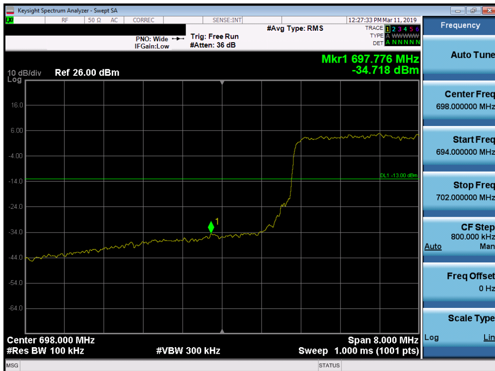
Plot 7-172. Lower Band Edge Plot (Band 12 - 10.0MHz QPSK - Full RB Configuration)
