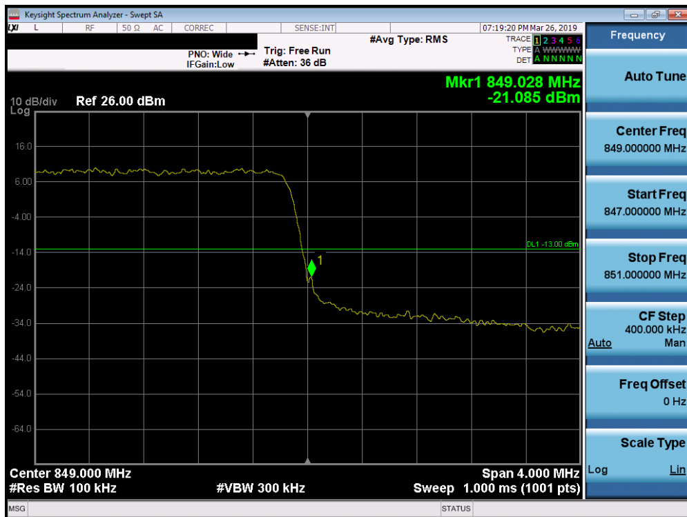
Plot 7-186. Upper Band Edge Plot (Band 26/5 - 3.0MHz QPSK - Full RB Configuration)
