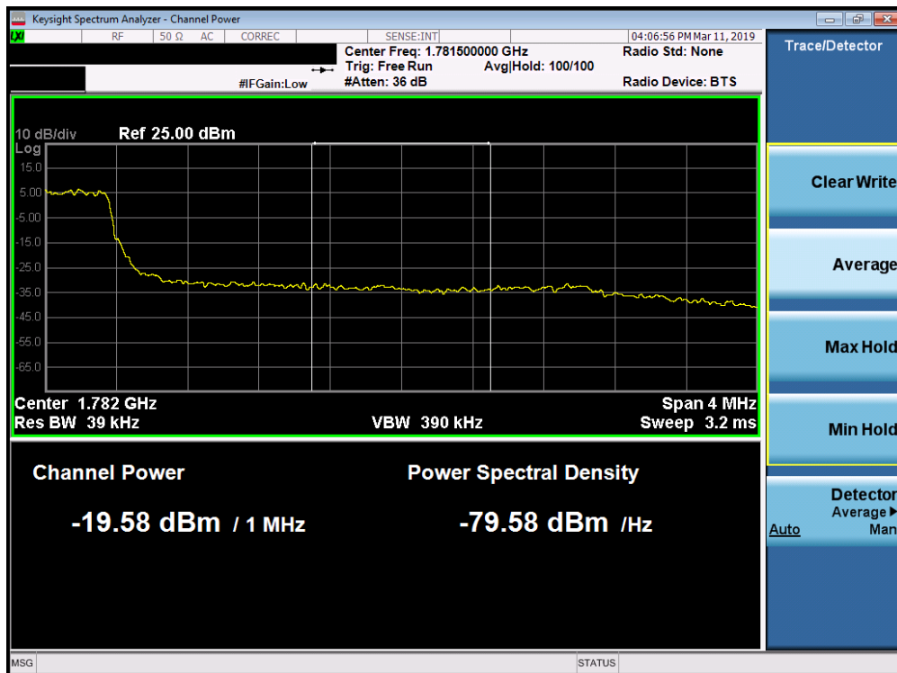
Plot 7-204. Upper Extended Band Edge Plot (Band 66 - 3.0MHz QPSK - Full RB Configuration)
