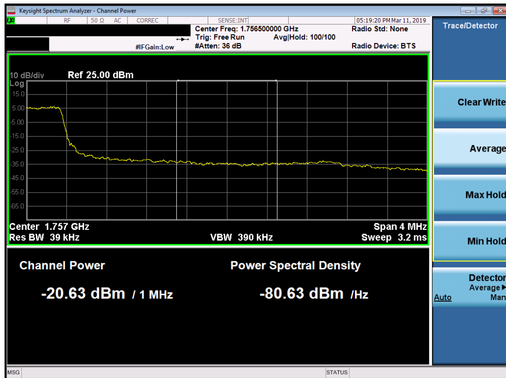
Plot 7-202. Upper Extended Band Edge Plot (Band 4 - 3.0MHz QPSK - Full RB Configuration)
