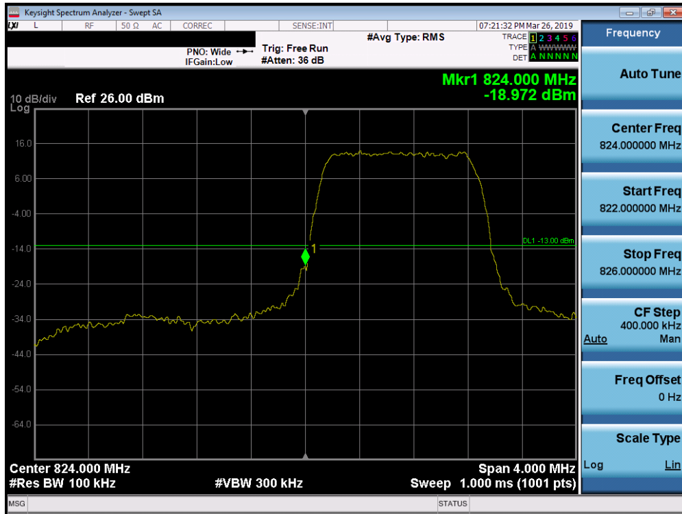
Plot 7-183. Lower Band Edge Plot (Band 26/5 - 1.4MHz QPSK - Full RB Configuration)
