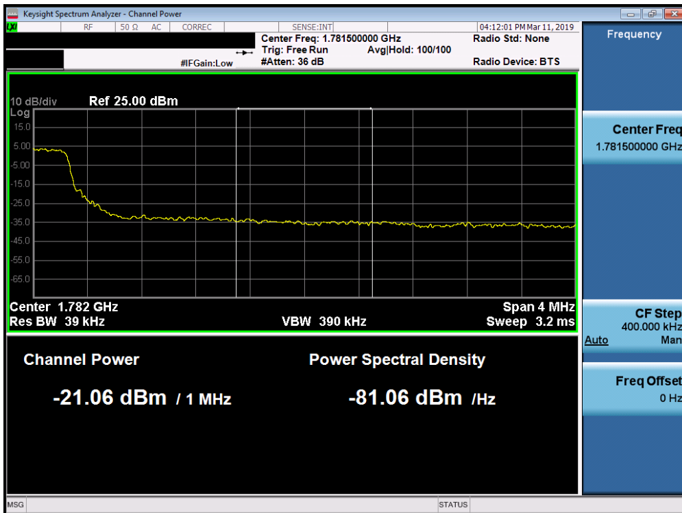
Plot 7-210. Upper Extended Band Edge Plot (Band 66 - 5.0MHz QPSK - Full RB Configuration)
