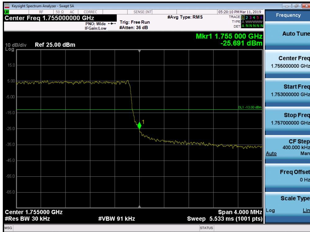
Plot 7-201. Upper Band Edge Plot (Band 4 - 3.0MHz QPSK - Full RB Configuration)
