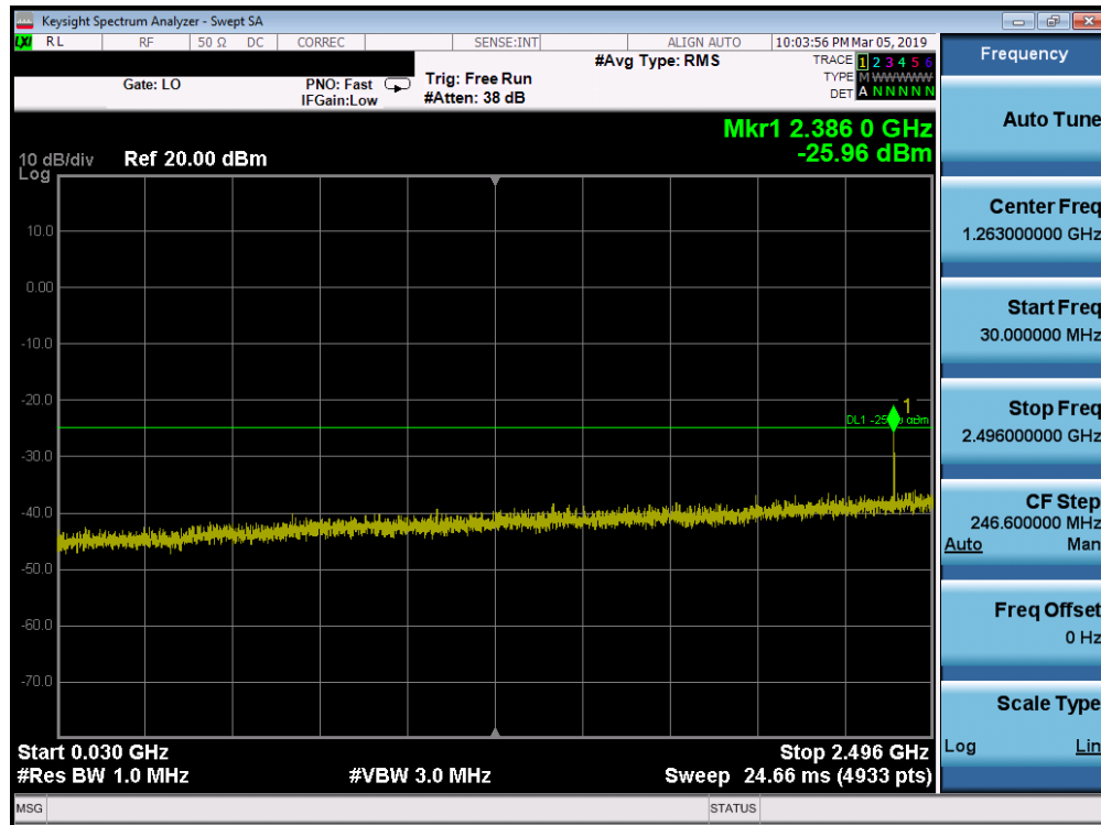
Plot 7-154. Conducted Spurious Plot (Band 41 - 15.0MHz QPSK - RB Size 1, RB Offset 0 - High Channel)
