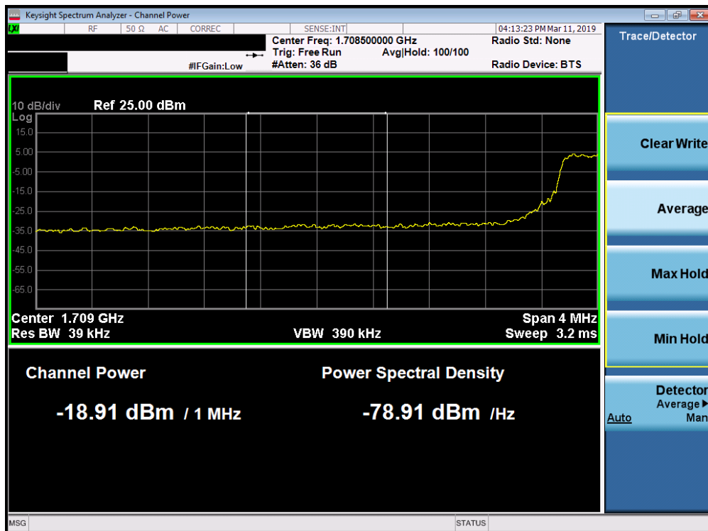
Plot 7-206. Lower Extended Band Edge Plot (Band 66/4 - 5.0MHz QPSK - Full RB Configuration)
