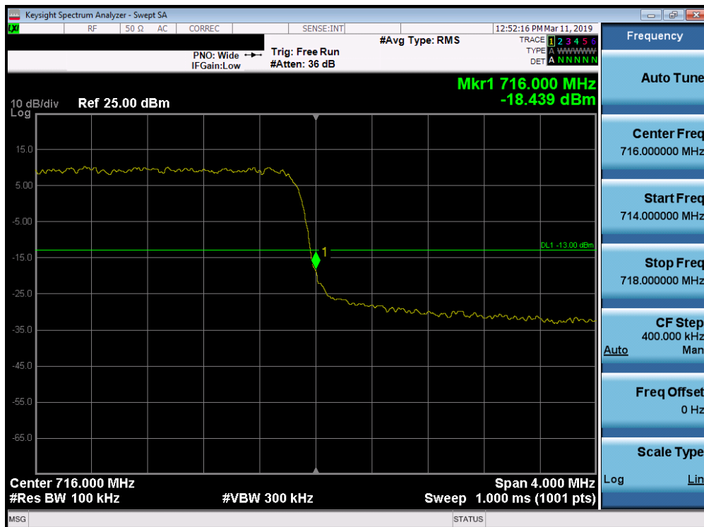
Plot 7-168. Upper Band Edge Plot (Band 12 - 3.0MHz QPSK - Full RB Configuration)
