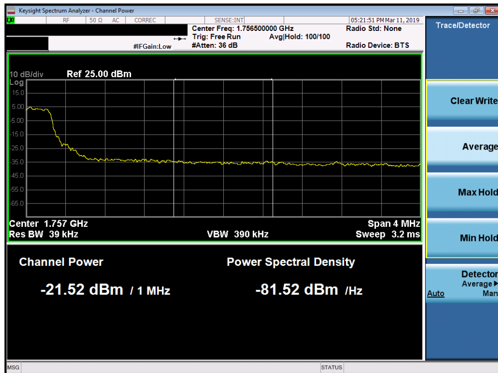
Plot 7-208. Upper Extended Band Edge Plot (Band 4 - 5.0MHz QPSK - Full RB Configuration)
