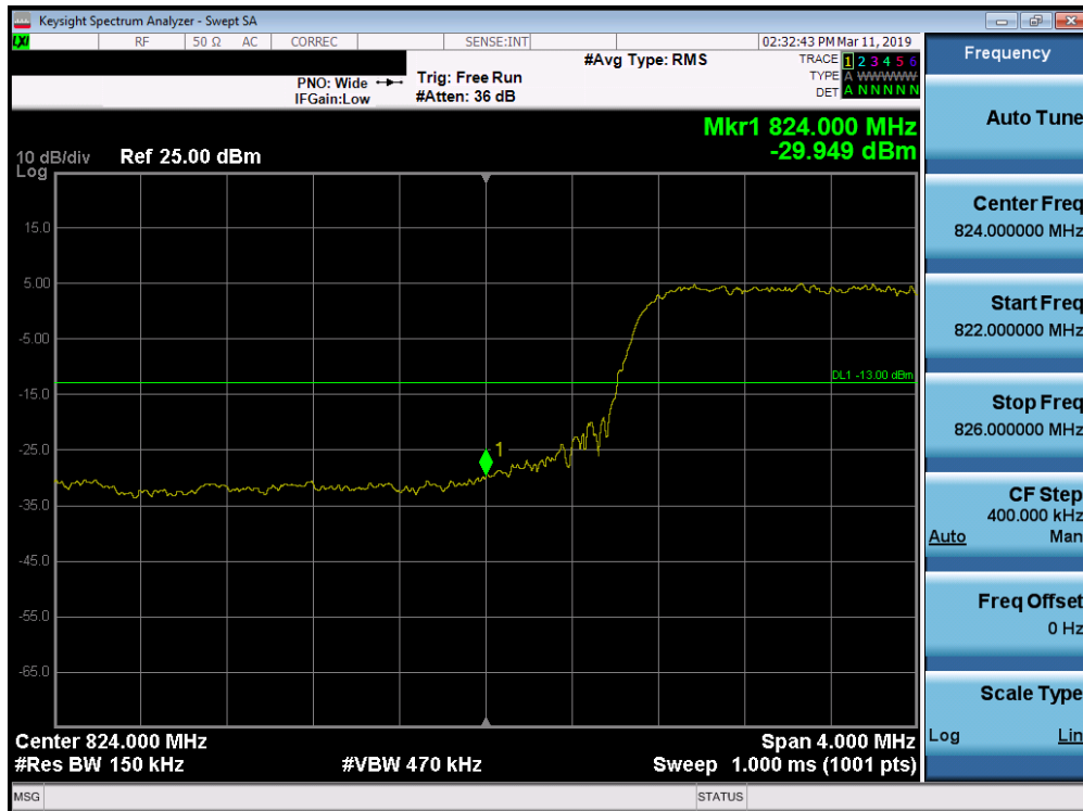
Plot 7-191. Lower Band Edge Plot (Band 26 - 15.0MHz QPSK - Full RB Configuration)
