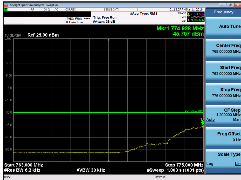
Plot 7-176. Lower Emission Mask Plot (Band 13 - 5.0MHz QPSK - Full RB Configuration)
