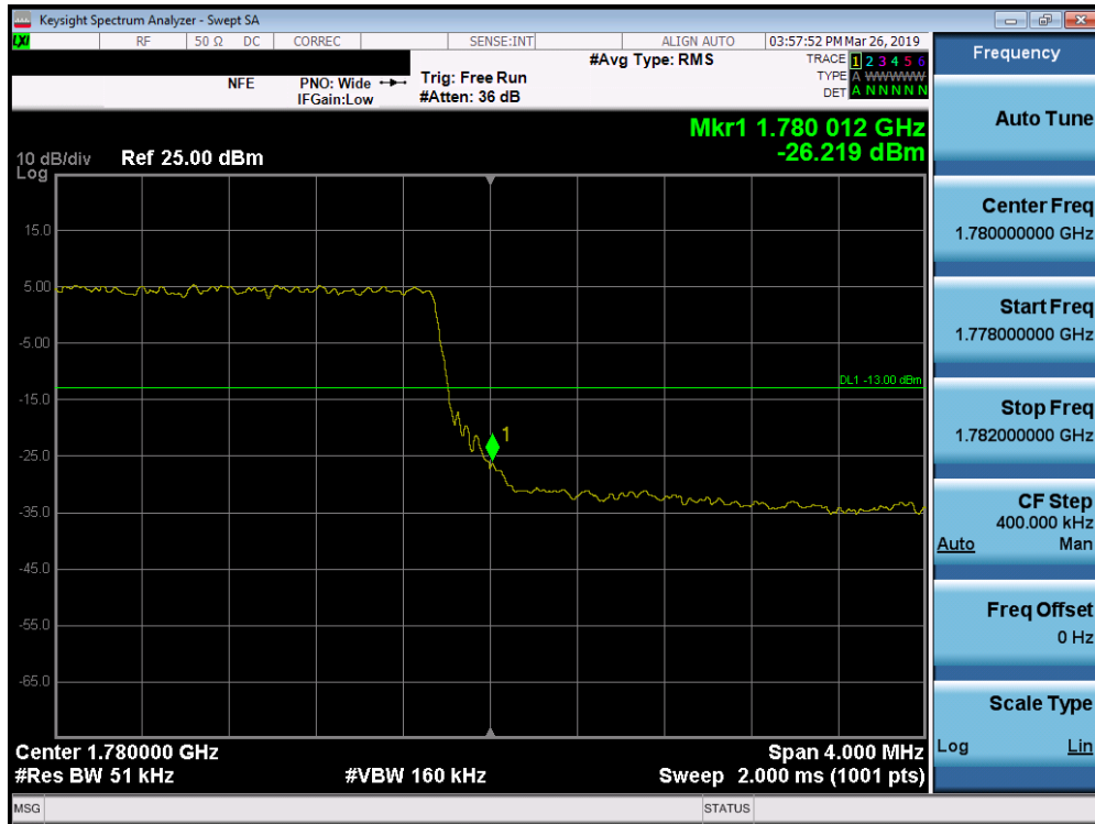
Plot 7-209. Upper Band Edge Plot (Band 66 - 5.0MHz QPSK - Full RB Configuration)
