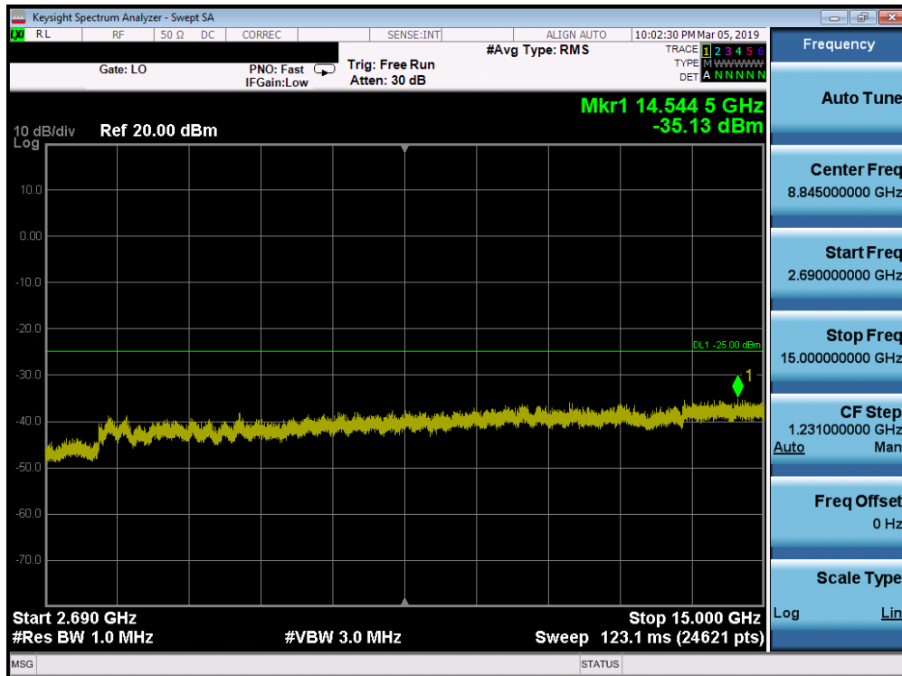
Plot 7-152. Conducted Spurious Plot (Band 41 - 15.0MHz QPSK - RB Size 1, RB Offset 0 - Mid Channel)
