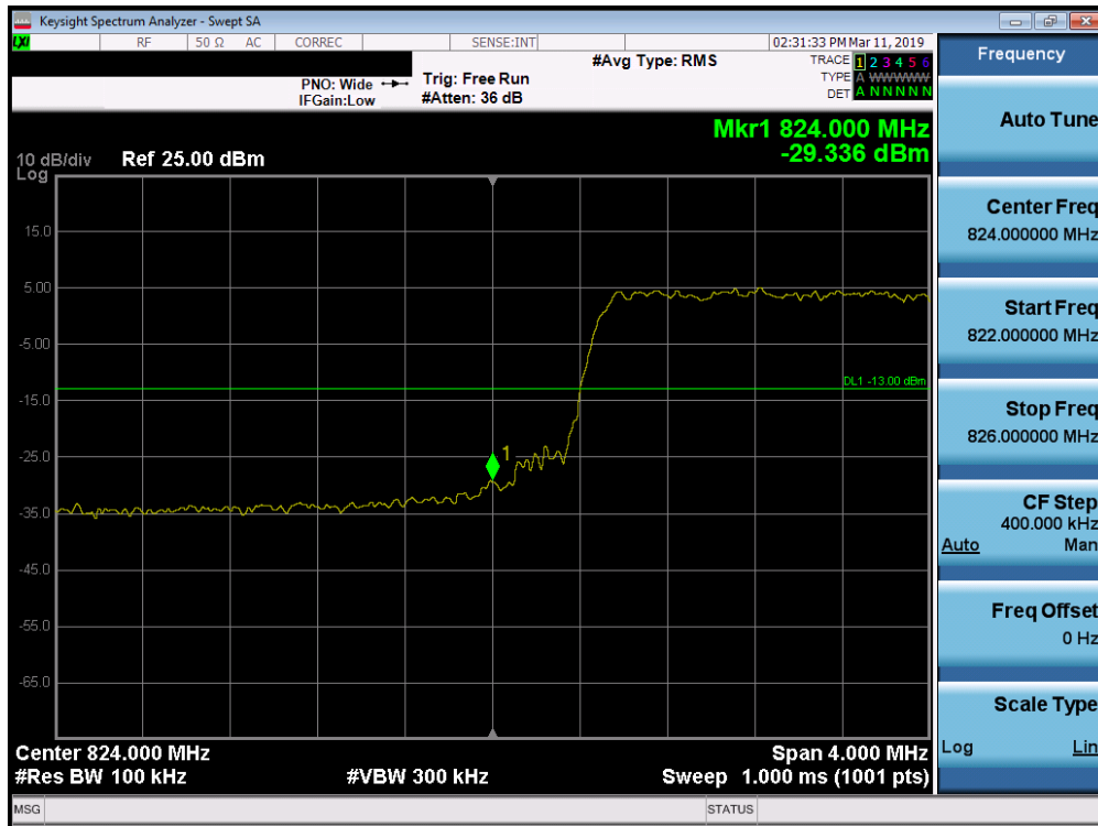
Plot 7-189. Lower Band Edge Plot (Band 26/5 - 10.0MHz QPSK - Full RB Configuration)
