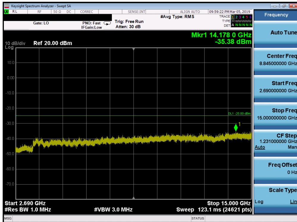
Plot 7-149. Conducted Spurious Plot (Band 41 - 15.0MHz QPSK - RB Size 1, RB Offset 0 - Low Channel)
