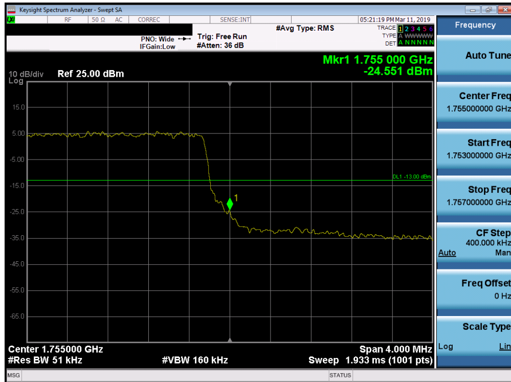
Plot 7-207. Upper Band Edge Plot (Band 4 - 5.0MHz QPSK - Full RB Configuration)
