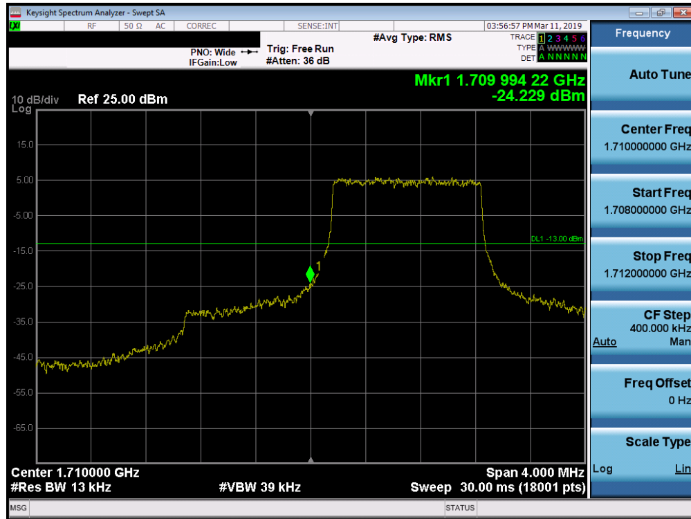
Plot 7-193. Lower Band Edge Plot (Band 66/4 - 1.4MHz QPSK - Full RB Configuration)
