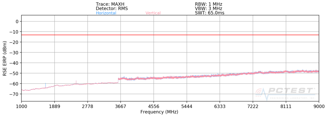
Plot 7-38. Radiated Spurious Plot above 1GHz (BC10 CDMA Mode)
