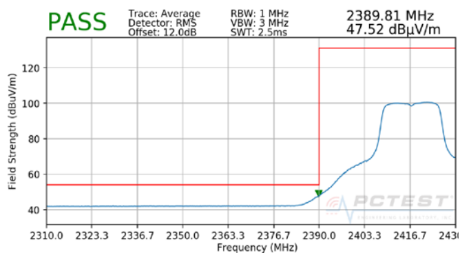
Plot 7-49. Radiated Restricted Lower Band Edge Measurement (Average)
