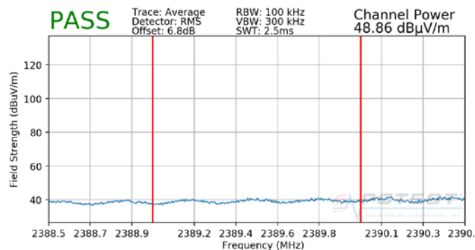
Plot 7-51. Radiated Restricted Lower Band Edge Measurement (Average)
