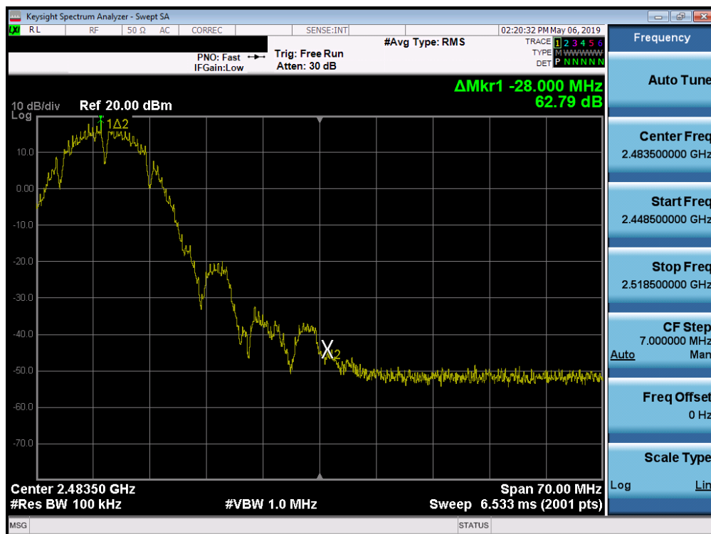
Plot 7-23. Band Edge Plot (802.11b – Ch. 10)
