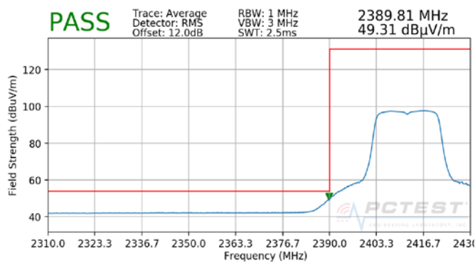
Plot 7-47. Radiated Restricted Lower Band Edge Measurement (Average)
