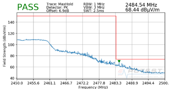
Plot 7-54. Radiated Restricted Upper Band Edge Measurement (Peak)
