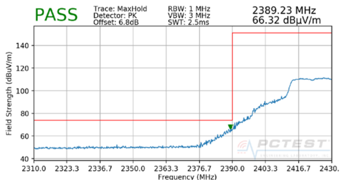
Plot 7-52. Radiated Restricted Lower Band Edge Measurement (Peak)
