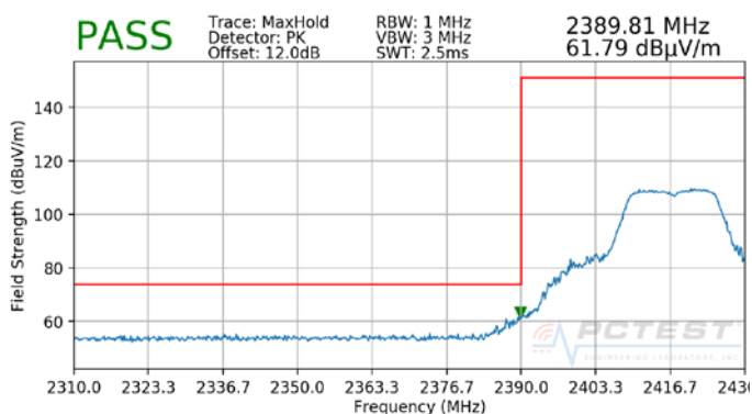
Plot 7-50. Radiated Restricted Lower Band Edge Measurement (Peak)
