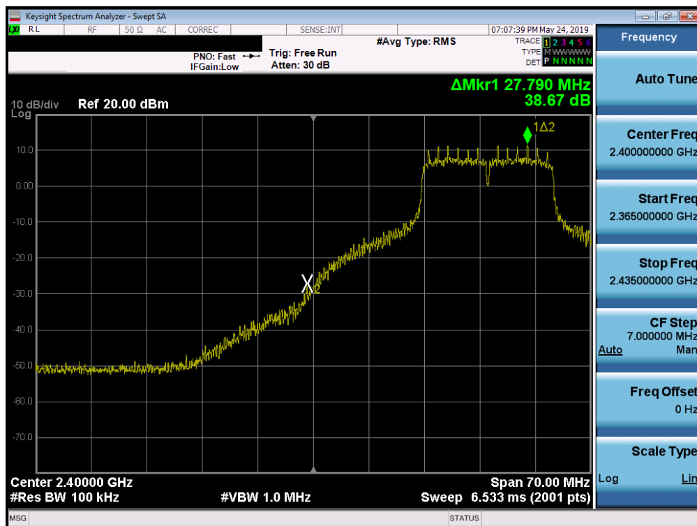
Plot 7-27. Band Edge Plot (802.11g– Ch. 3)
