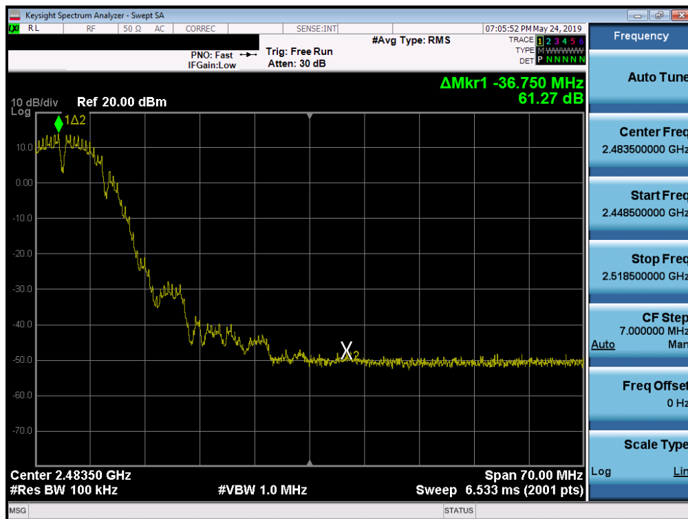
Plot 7-22. Band Edge Plot (802.11b – Ch. 9)
