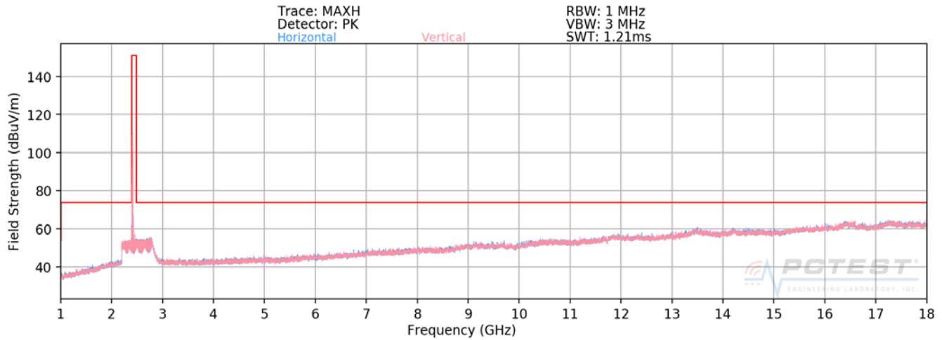
Plot 7-43. Radiated Spurious Plot above 1GHz (802.11b – Ch. 1)
