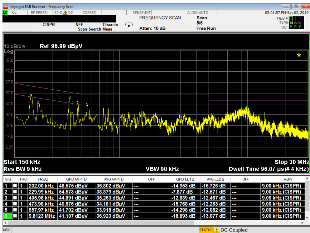
Plot 7-61. Line Conducted Plot with 802.11b (N)
