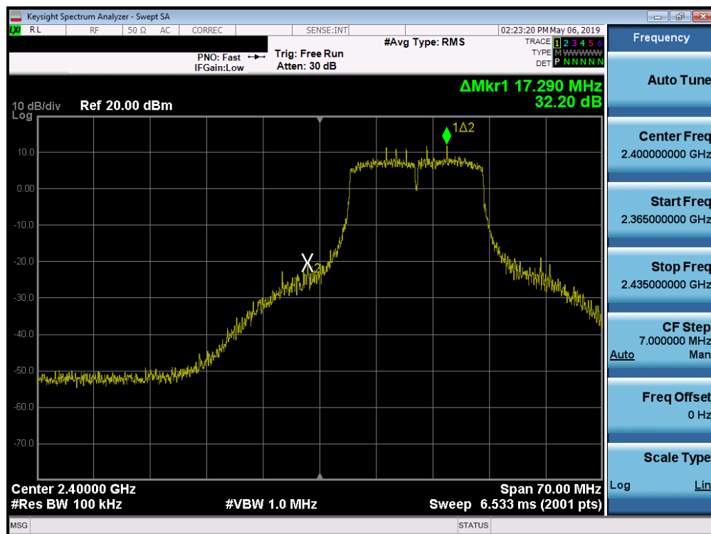
Plot 7-25. Band Edge Plot (802.11g– Ch. 1)
