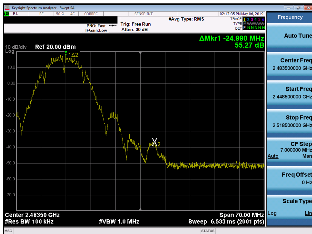
Plot 7-24. Band Edge Plot (802.11b – Ch. 11)
