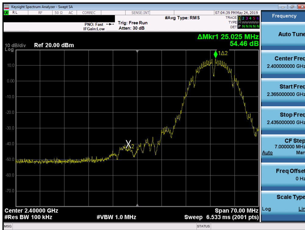
Plot 7-21. Band Edge Plot (802.11b – Ch. 3)
