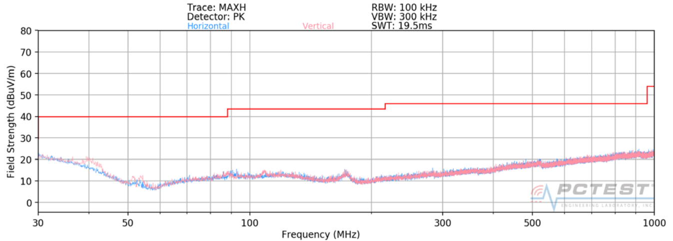
Plot 7-59. Radiated Spurious Plot below 1GHz
