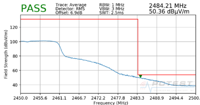
Plot 7-53. Radiated Restricted Upper Band Edge Measurement (Average)
