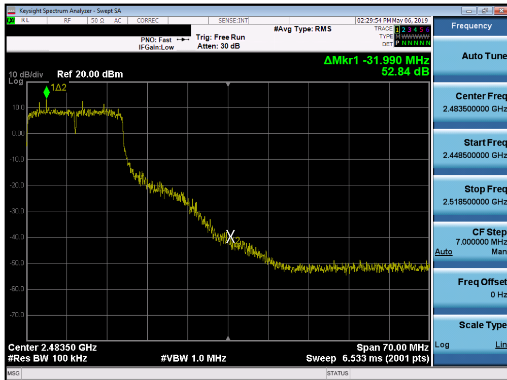
Plot 7-29. Band Edge Plot (802.11g - Ch. 10)
