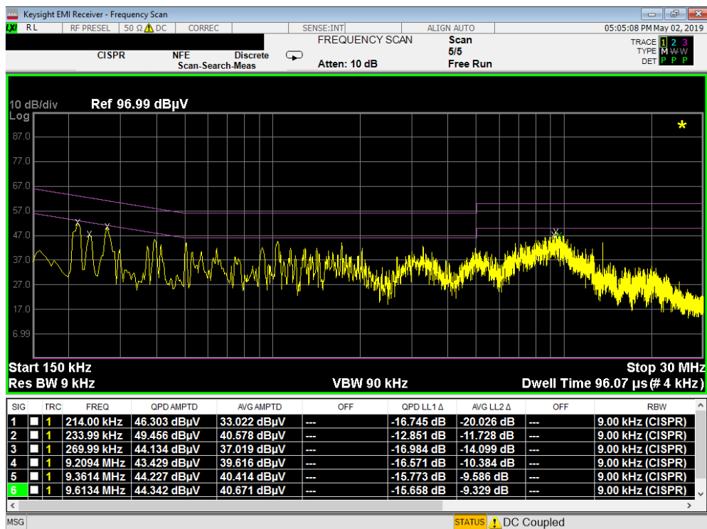
Plot 7-60. Line Conducted Plot with 802.11b (L1)
