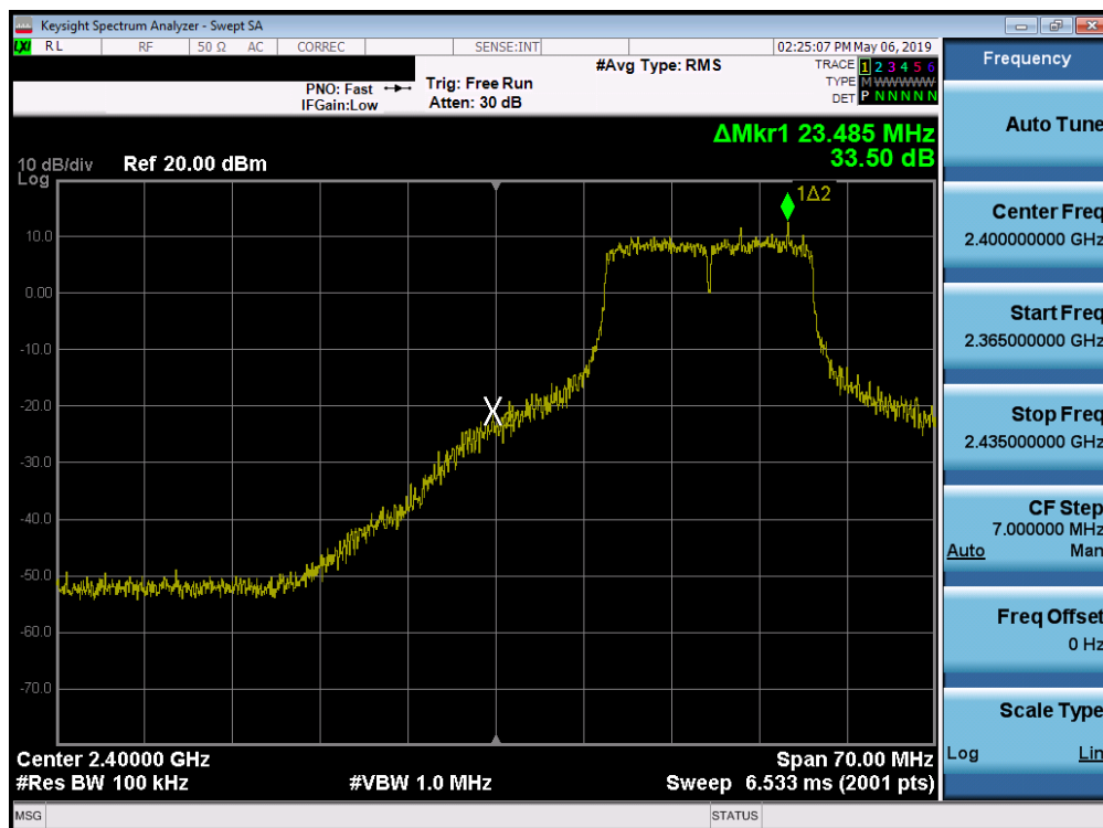
Plot 7-26. Band Edge Plot (802.11g– Ch. 2)
