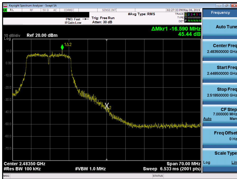
Plot 7-30. Band Edge Plot (802.11g - Ch. 11)
