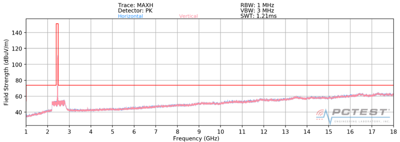
Plot 7-45. Radiated Spurious Plot above 1GHz (802.11b – Ch. 11)
