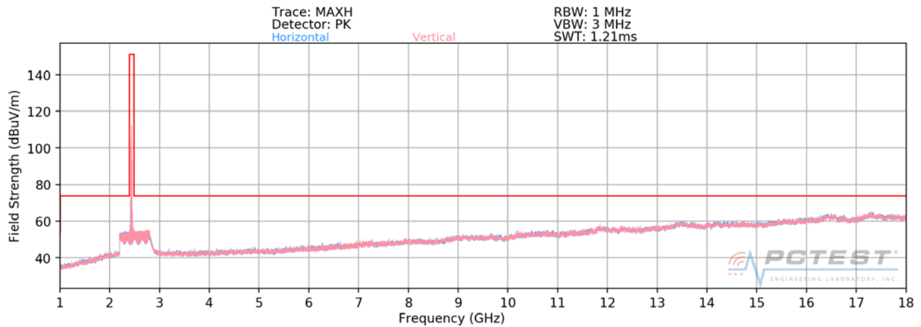
Plot 7-44. Radiated Spurious Plot above 1GHz (802.11b – Ch. 6)
