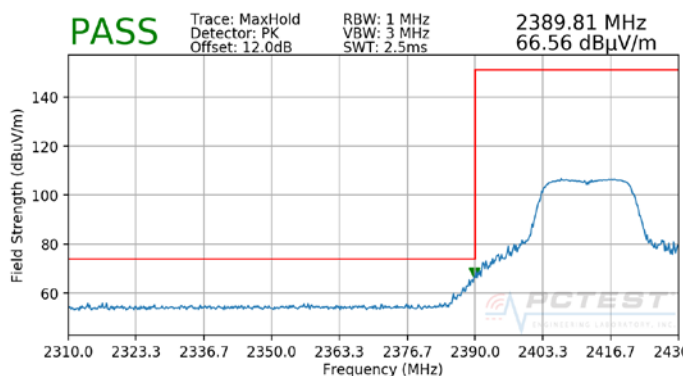
Plot 7-48. Radiated Restricted Lower Band Edge Measurement (Peak)
