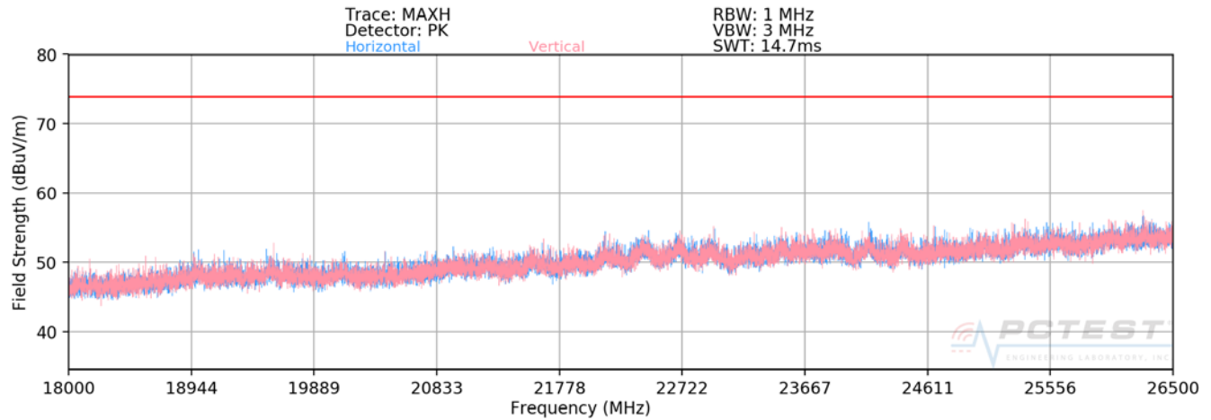
Plot 7-46. Radiated Spurious Plot above 18GHz
