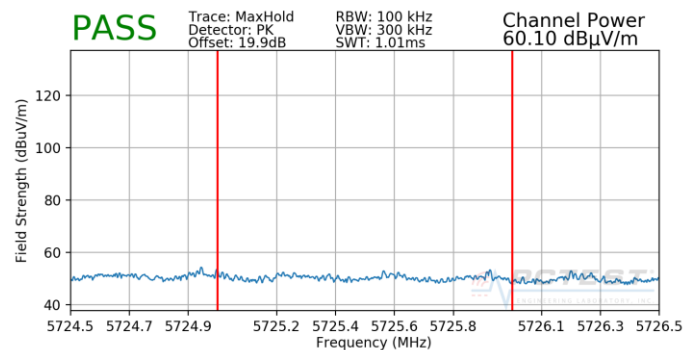
Plot 7-96. Radiated Upper Band Edge Plot (Peak – UNII Band 2C-Interior)
