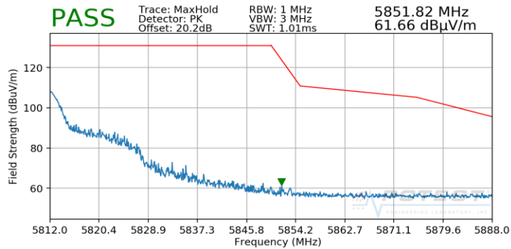
Plot 7-99. Radiated Upper Band Edge Plot (Peak – UNII Band 3)
