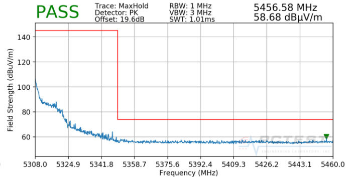
Plot 7-88. Radiated Upper Band Edge Plot (Peak – UNII Band 2A-Interior)
