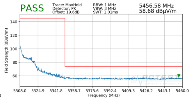
Plot 7-90. Radiated Upper Band Edge Plot (Peak – UNII Band 2A)
