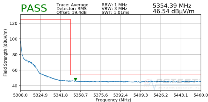
Plot 7-89. Radiated Upper Band Edge Plot (Average – UNII Band 2A)
