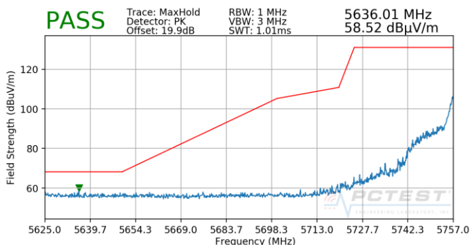
Plot 7-98. Radiated Lower Band Edge Plot (Peak – UNII Band 3-Interior)
