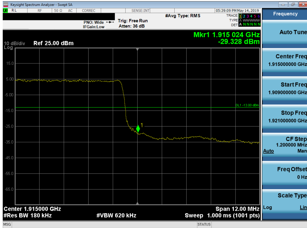
Plot 7-259. Upper Band Edge Plot (Band 25 - 15.0MHz QPSK - Full RB Configuration)
