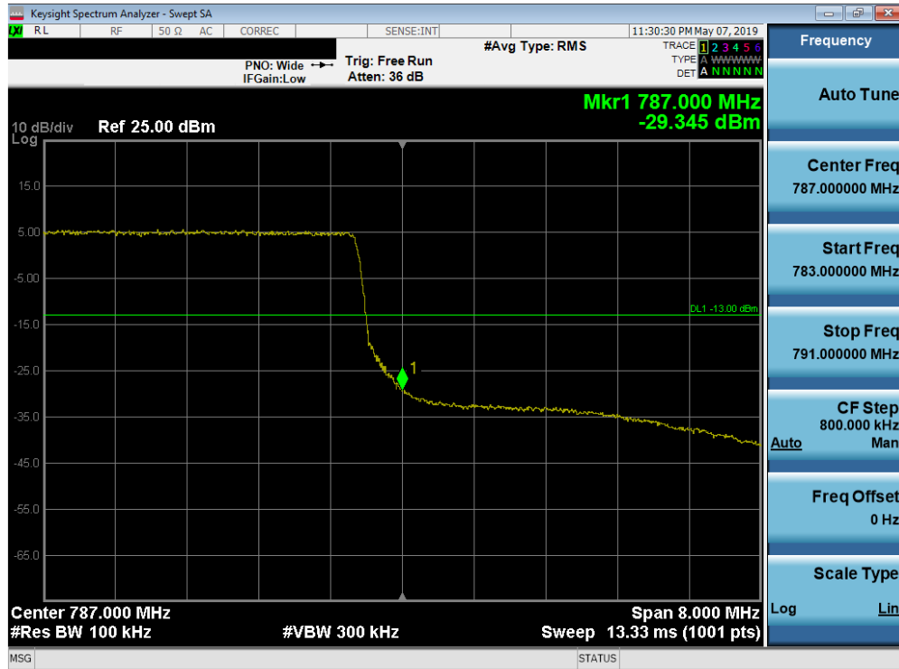
Plot 7-183. Upper Band Edge Plot (Band 13 - 10.0MHz QPSK - Full RB Configuration)
