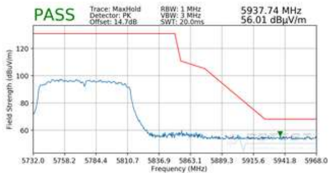
Plot 7-39. Radiated Upper Band Edge Plot (Peak – UNII Band 3)
