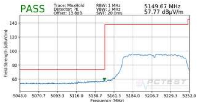
Plot 7-33. Radiated Lower Band Edge Plot (Peak – UNII Band 1)
