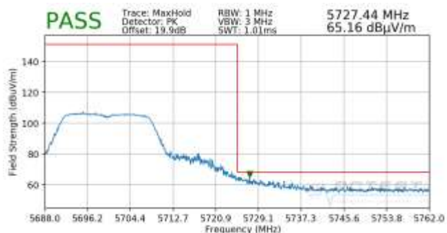
Plot 7-20. Radiated Upper Band Edge Plot (Peak – UNII Band 2C)
