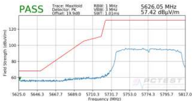
Plot 7-38. Radiated Lower Band Edge Plot (Peak – UNII Band 3)
