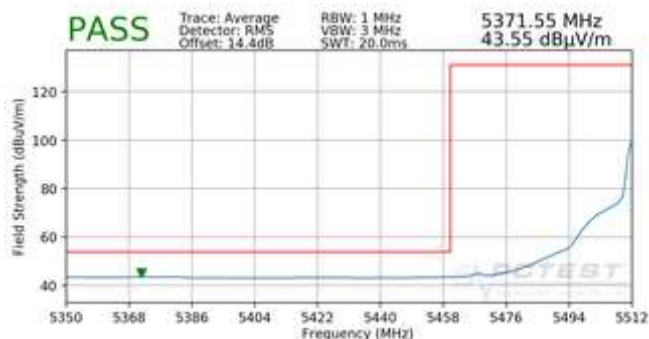
Plot 7-17. Radiated Lower Band Edge Plot (Average – UNII Band 2C)
