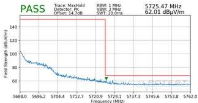
Plot 7-19. Radiated Upper Band Edge Plot (Peak – UNII Band 2C)
