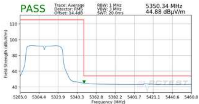
Plot 7-25. Radiated Upper Band Edge Plot (Average – UNII Band 2A)
