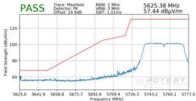
Plot 7-30. Radiated Lower Band Edge Plot (Peak – UNII Band 3)
