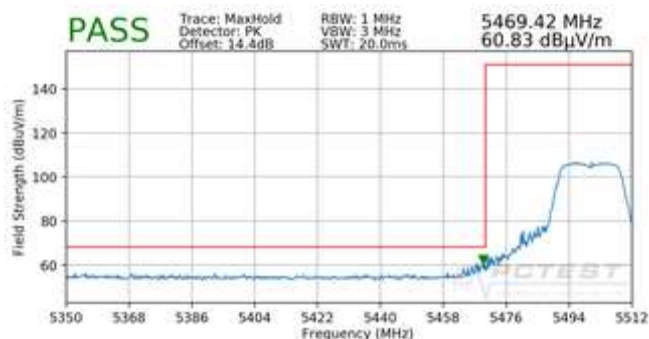
Plot 7-16. Radiated Lower Band Edge Plot (Peak – UNII Band 2C)
