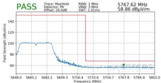
Plot 7-29. Radiated Upper Band Edge Plot (Peak – UNII Band 2C)
