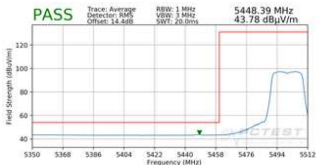
Plot 7-15. Radiated Lower Band Edge Plot (Average – UNII Band 2C)
