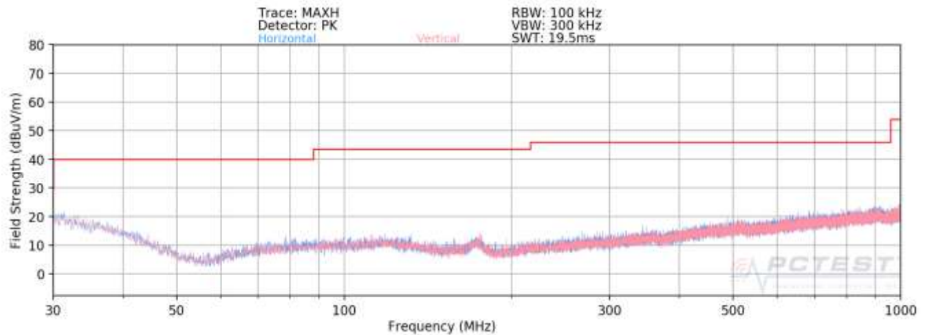
Plot 7-40. Radiated Spurious Plot below 1GHz (802.11a – U3 Ch. 157)
