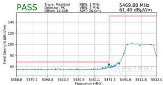
Plot 7-28. Radiated Lower Band Edge Plot (Peak – UNII Band 2C)
