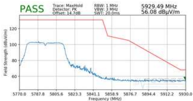
Plot 7-31. Radiated Upper Band Edge Plot (Peak – UNII Band 3)
