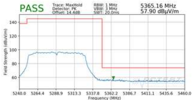
Plot 7-35. Radiated Upper Band Edge Plot (Peak – UNII Band 2A)
