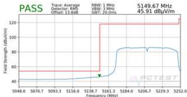
Plot 7-32. Radiated Lower Band Edge Plot (Average – UNII Band 1)
