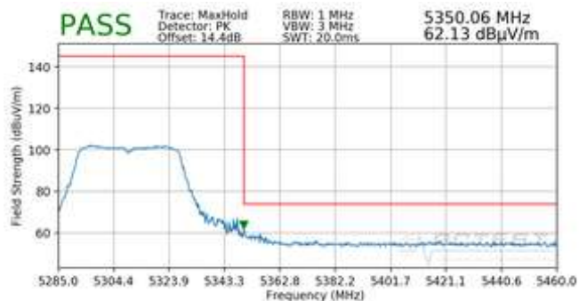
Plot 7-26. Radiated Upper Band Edge Plot (Peak – UNII Band 2A)
