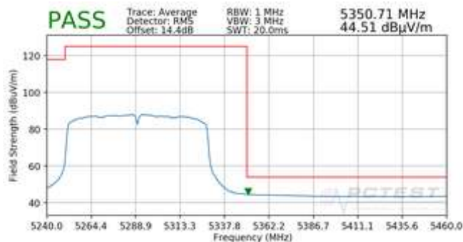
Plot 7-34. Radiated Upper Band Edge Plot (Average – UNII Band 2A)
