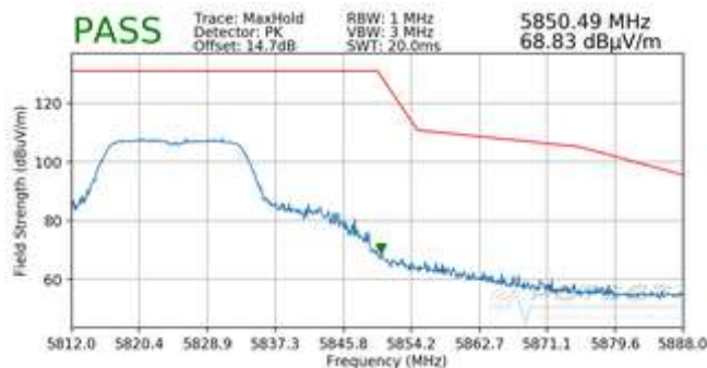
Plot 7-22. Radiated Upper Band Edge Plot (Peak – UNII Band 3)
