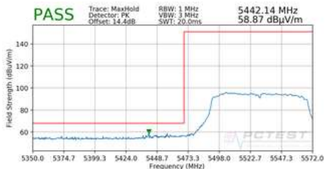
Plot 7-37. Radiated Lower Band Edge Plot (Peak – UNII Band 2C)
