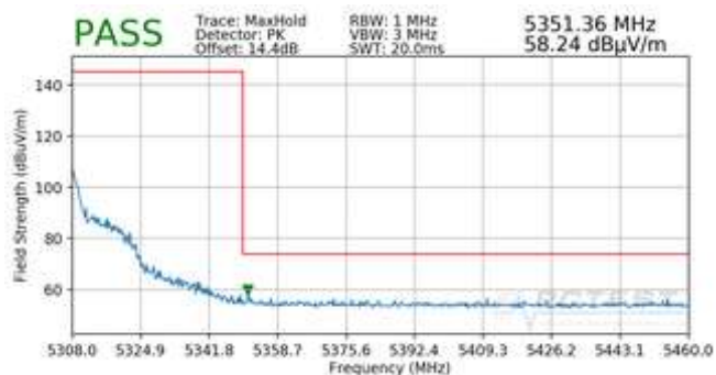
Plot 7-12. Radiated Upper Band Edge Plot (Peak – UNII Band 2A)
