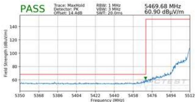
Plot 7-18. Radiated Lower Band Edge Plot (Peak – UNII Band 2C)
