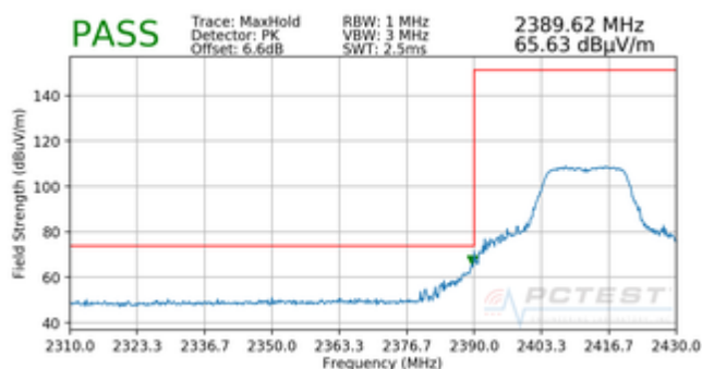
Plot 7-6. Radiated Restricted Lower Band Edge Measurement (Peak)
