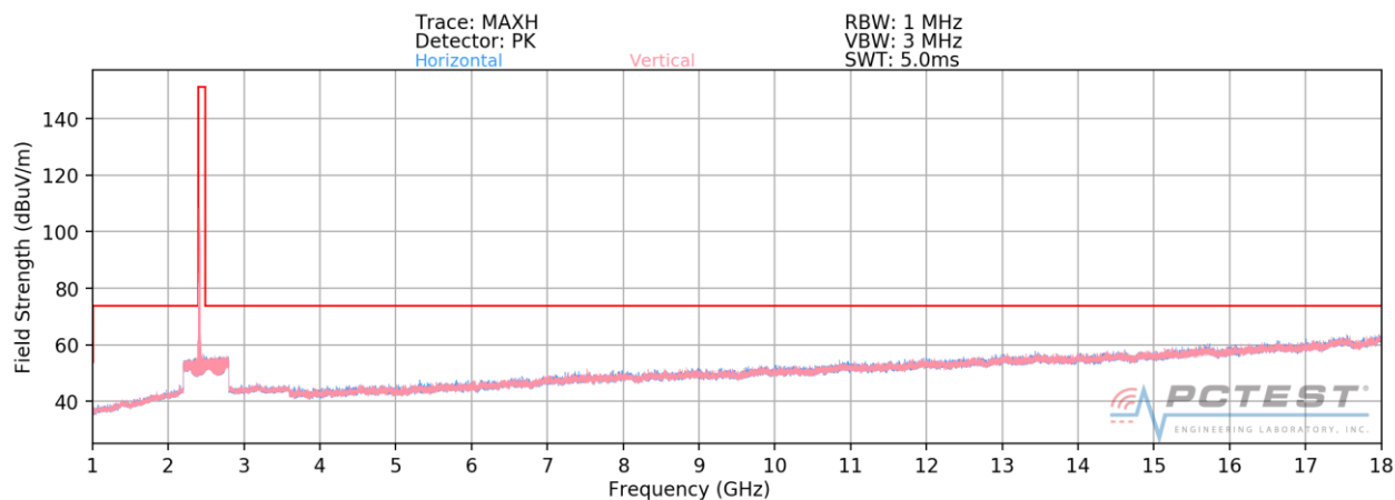
Plot 7-1. Radiated Spurious Plot above 1GHz (802.11b – Ch. 1)
