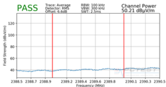
Plot 7-5. Radiated Restricted Lower Band Edge Measurement (Average)
