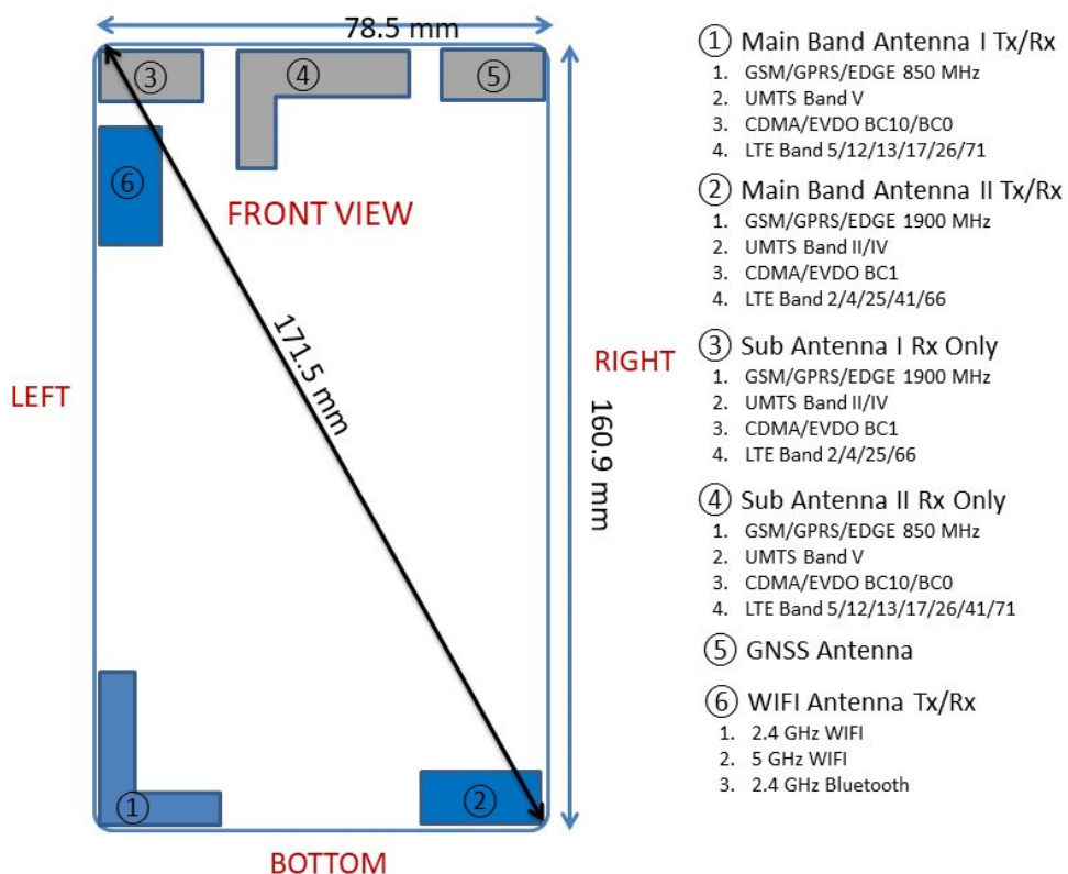
Figure F-1 DUT Antenna Locations
