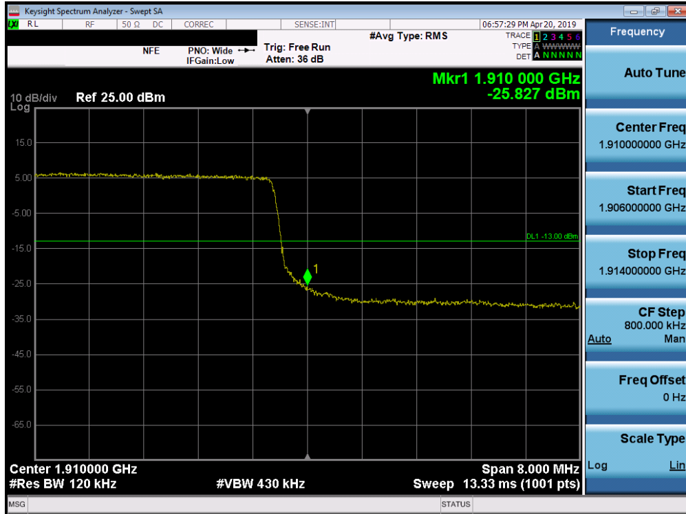
Plot 7-247. Upper Band Edge Plot (Band 2 – 10.0MHz QPSK - Full RB Configuration)
