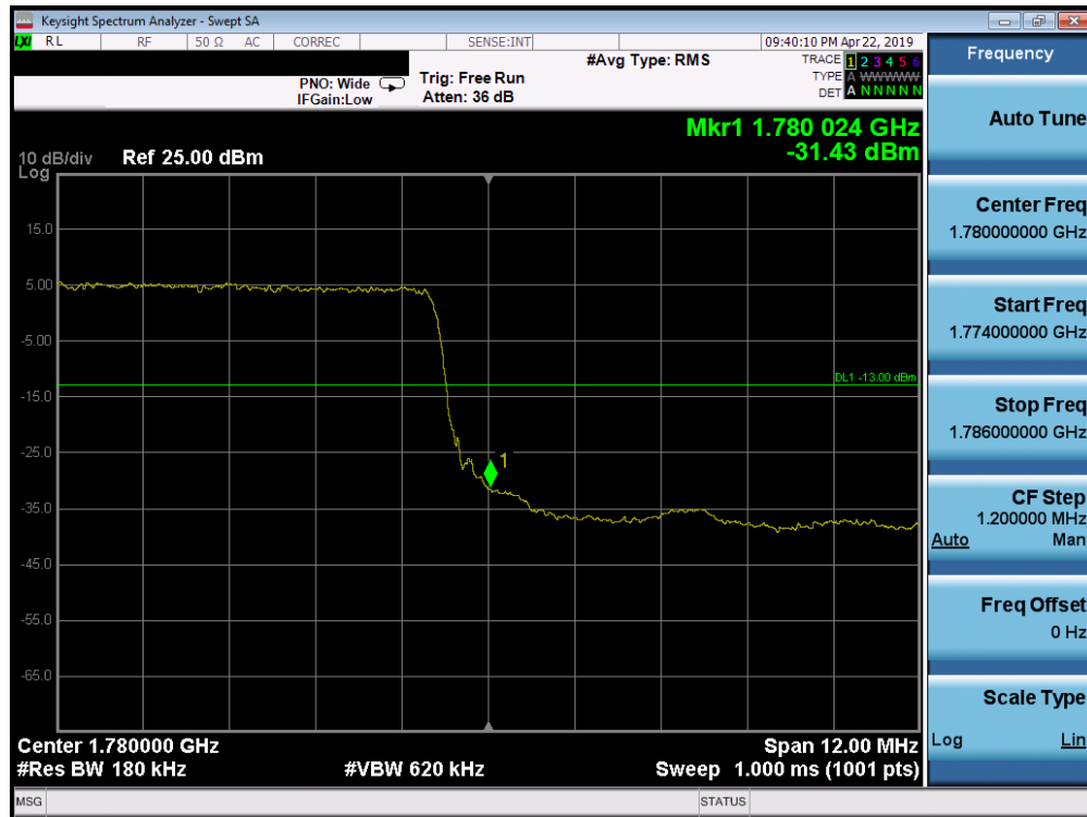
Plot 7-219. Upper Band Edge Plot (Band 66 - 15.0MHz QPSK - Full RB Configuration)
