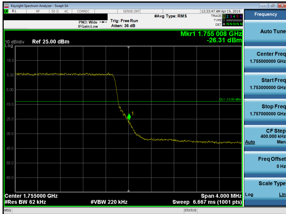
Plot 7-205. Upper Band Edge Plot (Band 4 – 5.0MHz QPSK - Full RB Configuration)
