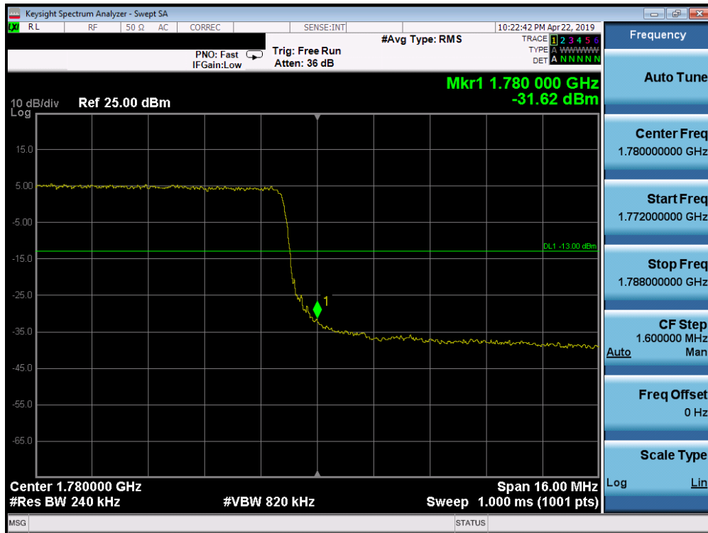
Plot 7-225. Upper Band Edge Plot (Band 66 - 20.0MHz QPSK - Full RB Configuration)
