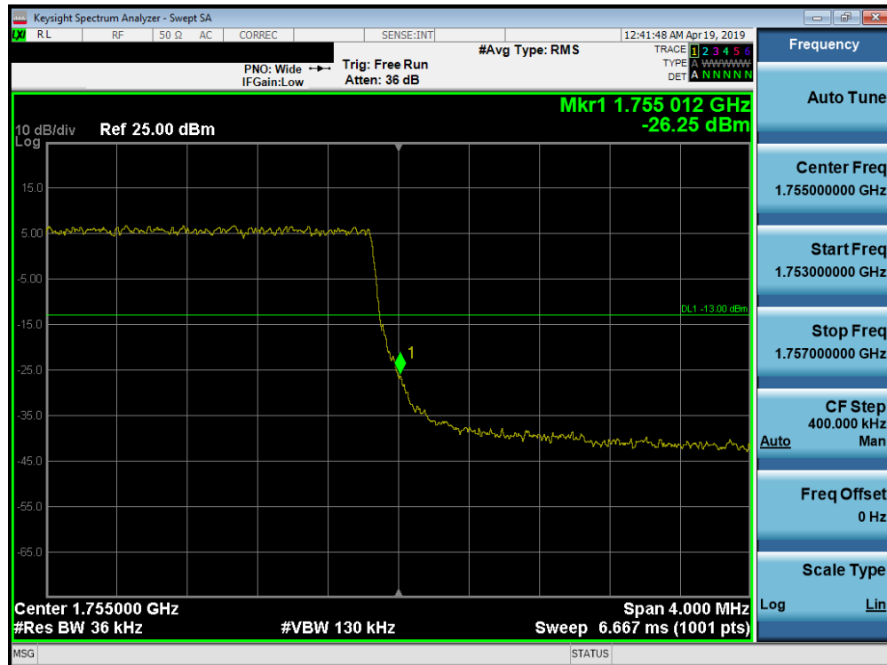
Plot 7-199. Upper Band Edge Plot (Band 4 – 3.0MHz QPSK - Full RB Configuration)
