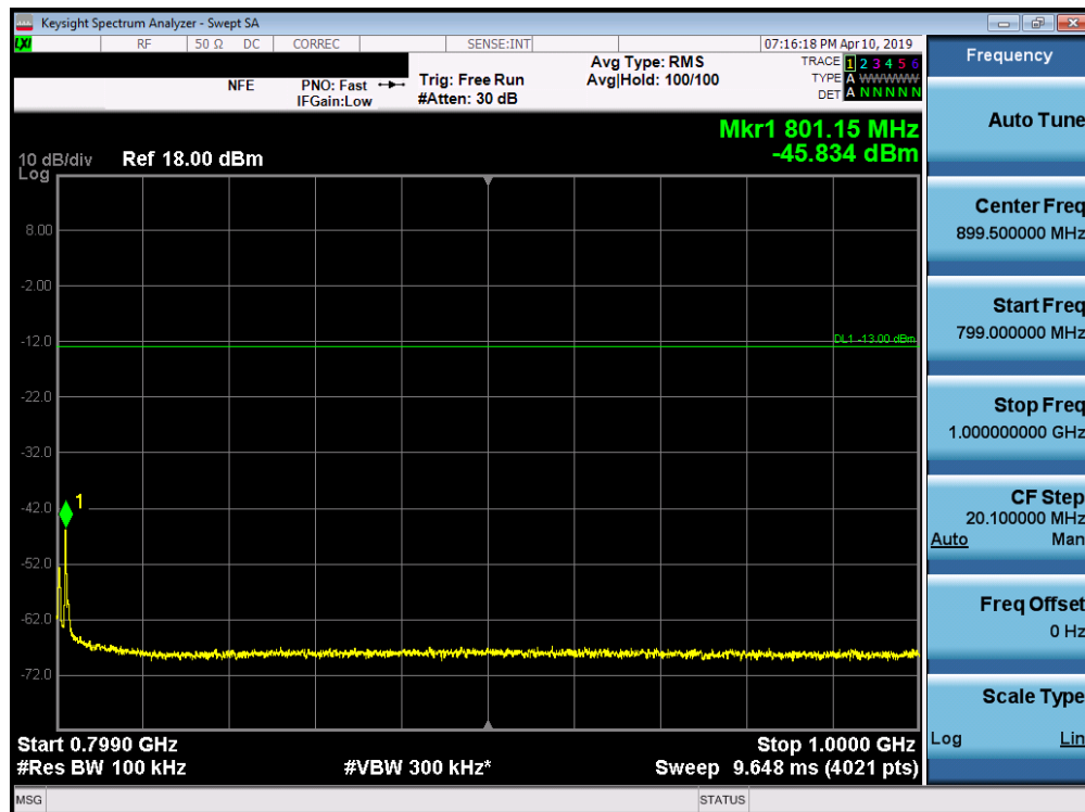
Plot 7-12. Conducted Spurious Plot (LTE Band 14, 5MHz QPSK – RB Size 1, RB Offset 0 – High Channel)
