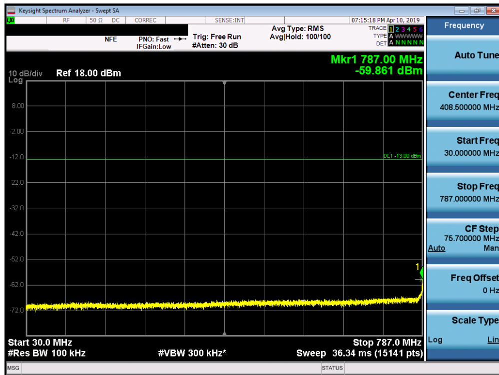
Plot 7-11. Conducted Spurious Plot (LTE Band 14, 5MHz QPSK – RB Size 1, RB Offset 0 – High Channel)
