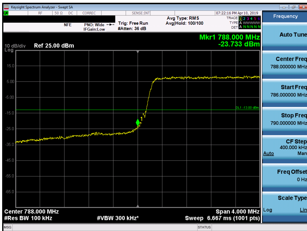
Plot 7-14. Lower Band Edge Plot (LTE Band 14, 5MHz QPSK – RB Size 25)
