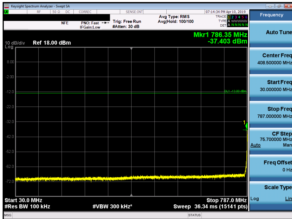
Plot 7-5. Conducted Spurious Plot (LTE Band 14, 5MHz QPSK – RB Size 1, RB Offset 0 – Low Channel)
