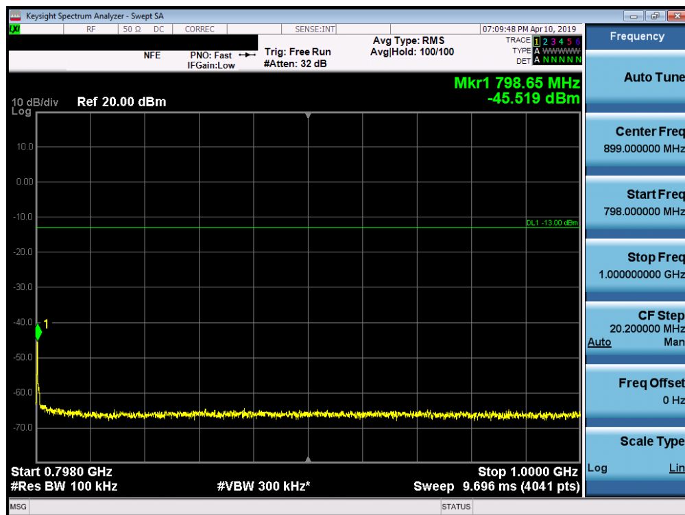
Plot 7-9. Conducted Spurious Plot (LTE Band 14, 5MHz QPSK – RB Size 1, RB Offset 0 – Mid Channel)
