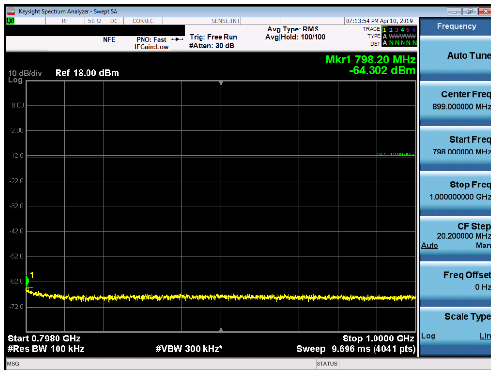
Plot 7-6. Conducted Spurious Plot (LTE Band 14, 5MHz QPSK – RB Size 1, RB Offset 0 – Low Channel)
