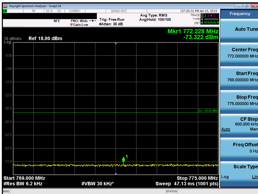
Plot 7-15. Lower Emission Mask Plot (LTE Band 14, 5MHz QPSK – RB Size 25)
