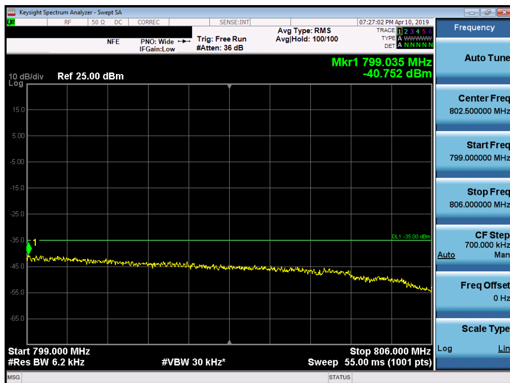
Plot 7-21. Upper Emission Mask Plot (LTE Band 14, 10MHz QPSK - RB Size 50)
