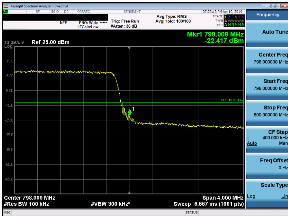
Plot 7-16. Upper Band Edge Plot (LTE Band 14, 5MHz QPSK – RB Size 25)
