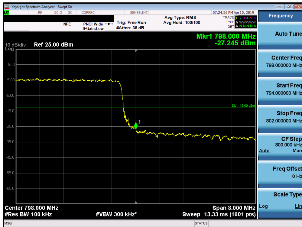
Plot 7-20. Upper Band Edge Plot (LTE Band 14, 10MHz QPSK - RB Size 50)
