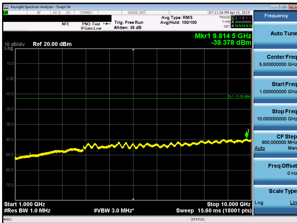
Plot 7-7. Conducted Spurious Plot (LTE Band 14, 5MHz QPSK – RB Size 1, RB Offset 0 – Low Channel)
