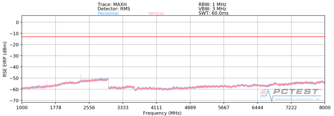
Plot 7-23. Radiated Spurious Plot above 1GHz (LTE Band 14 – Mid Channel)
