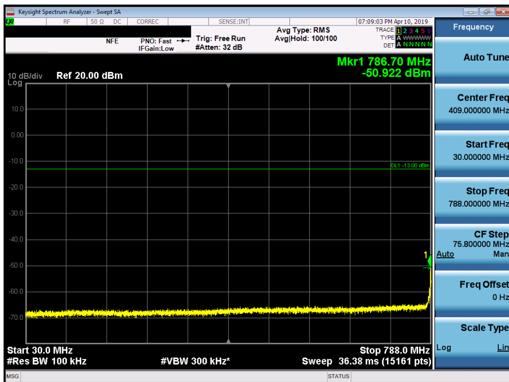
Plot 7-8. Conducted Spurious Plot (LTE Band 14, 5MHz QPSK – RB Size 1, RB Offset 0 – Mid Channel)
