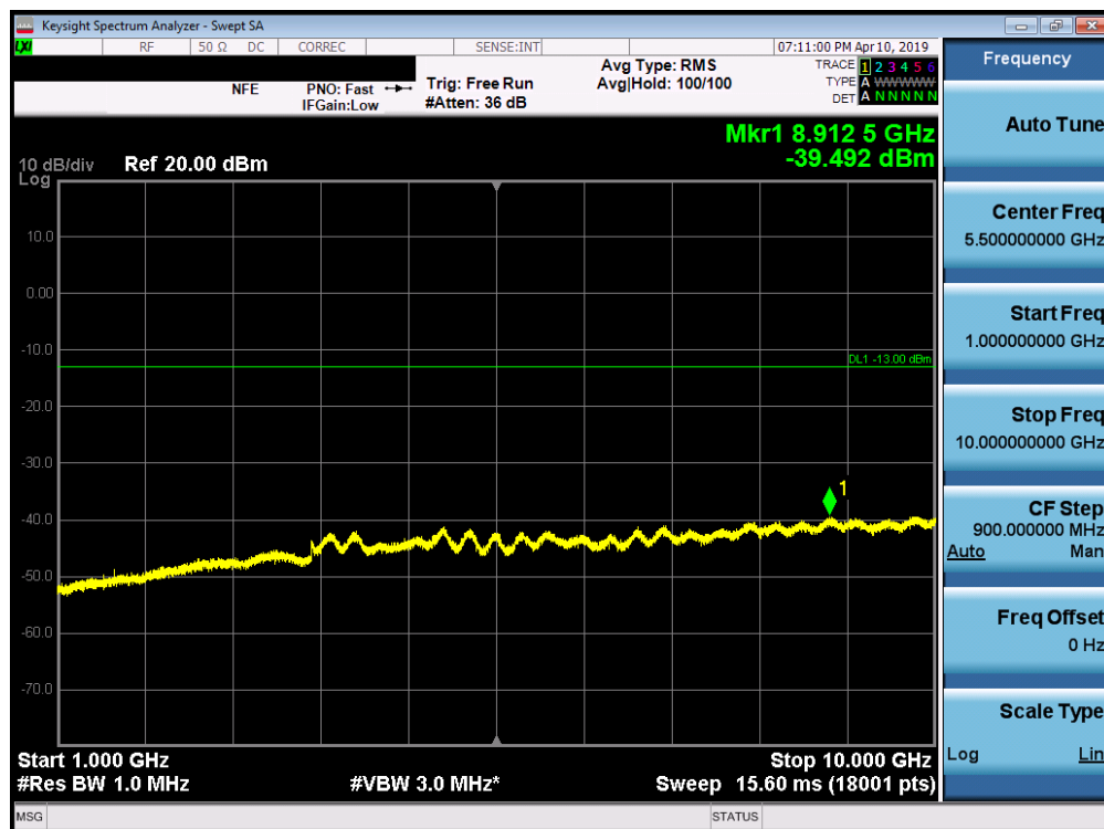
Plot 7-10. Conducted Spurious Plot (LTE Band 14, 5MHz QPSK – RB Size 1, RB Offset 0 – Mid Channel)
