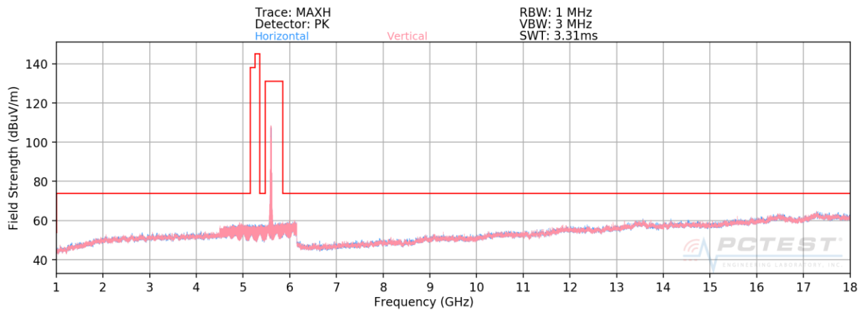
Plot 7-79. Radiated Spurious Plot above 1GHz (802.11a – U2C Ch. 120)
