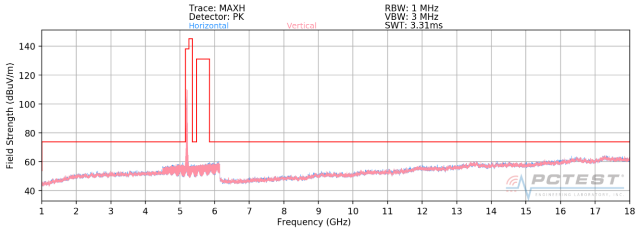
Plot 7-77. Radiated Spurious Plot above 1GHz (802.11a – U1 Ch. 40)
