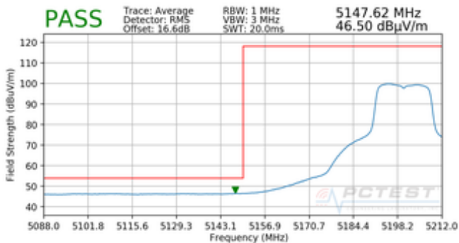
Plot 7-85. Radiated Lower Band Edge Plot (Average – UNII Band 1)
