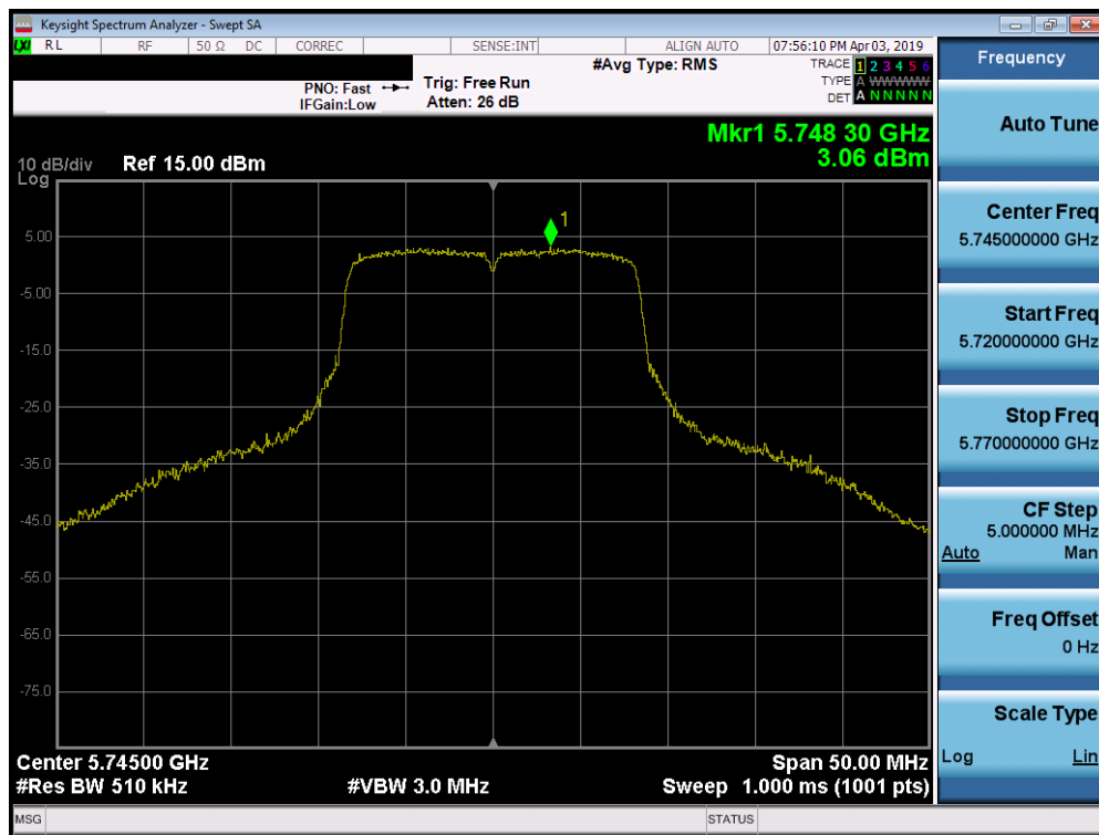
Plot 7-68. Power Spectral Density Plot (802.11a (UNII Band 3) – Ch. 149)
