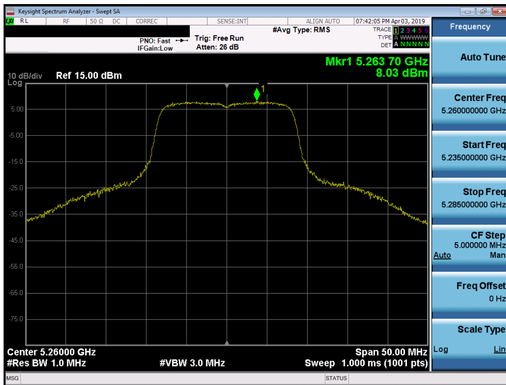
Plot 7-48. Power Spectral Density Plot (802.11a (UNII Band 2A) – Ch. 52)
