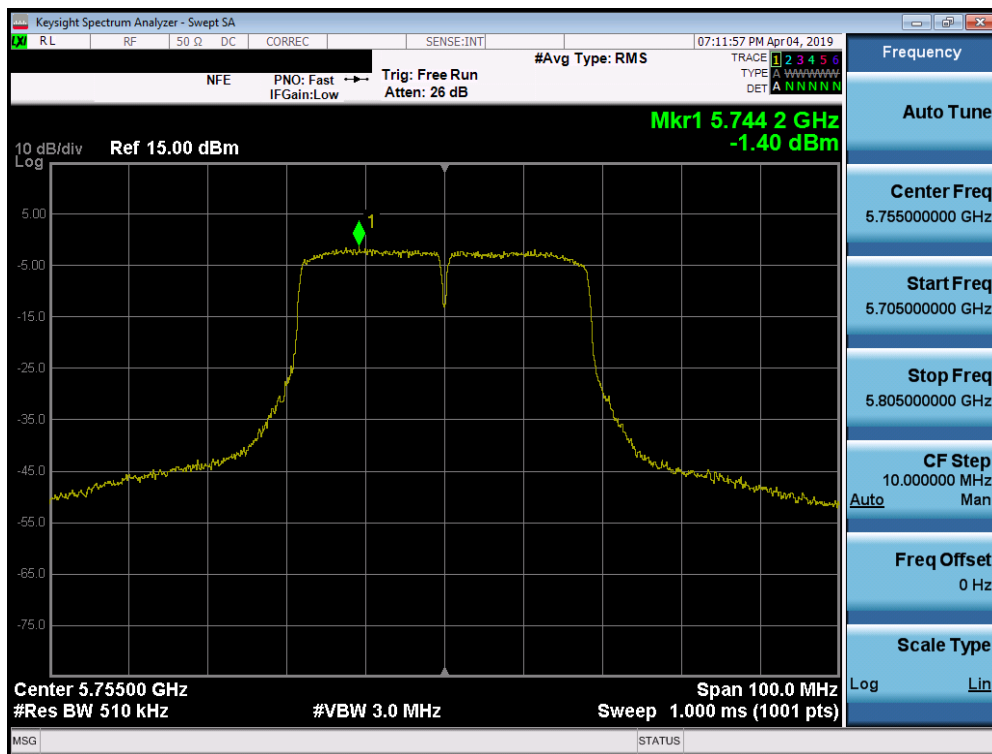
Plot 7-74. Power Spectral Density Plot (40MHz BW 802.11n (UNII Band 3) – Ch. 151)
