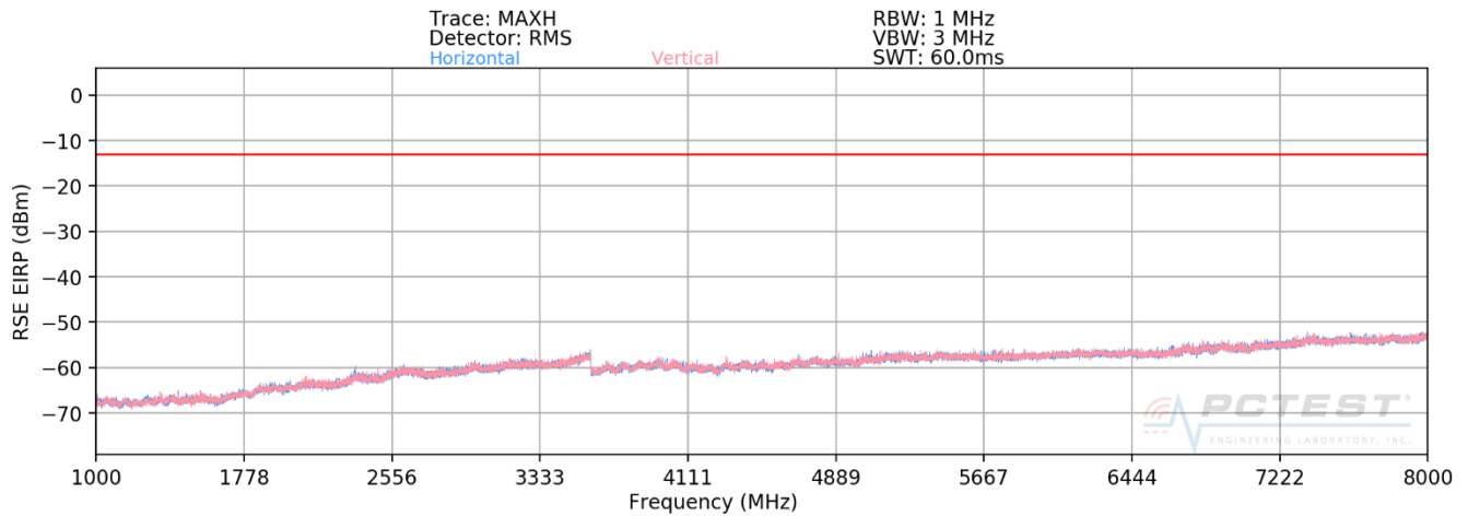
Plot 7-17. Radiated Spurious Plot above 1GHz (LTE Band 14)
