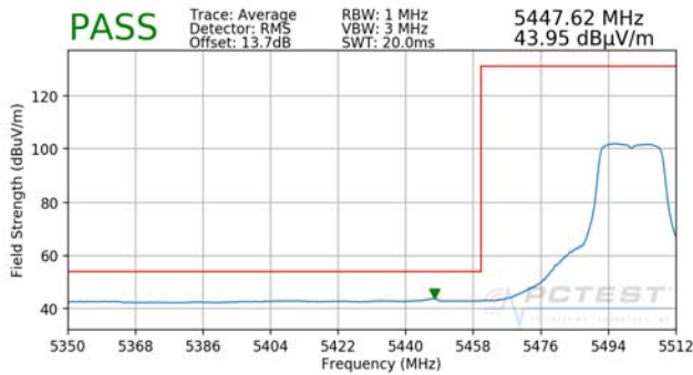
Plot 7-87. Radiated Lower Band Edge Plot (Average – UNII Band 2C)
