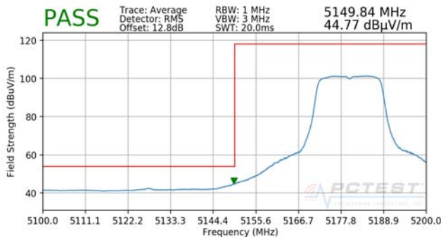
Plot 7-83. Radiated Lower Band Edge Plot (Average – UNII Band 1)
