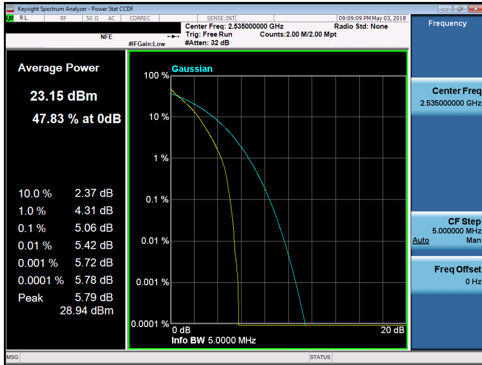
Plot 7-260. PAR Plot (Band 7 – 5.0MHz QPSK - Full RB Configuration)
