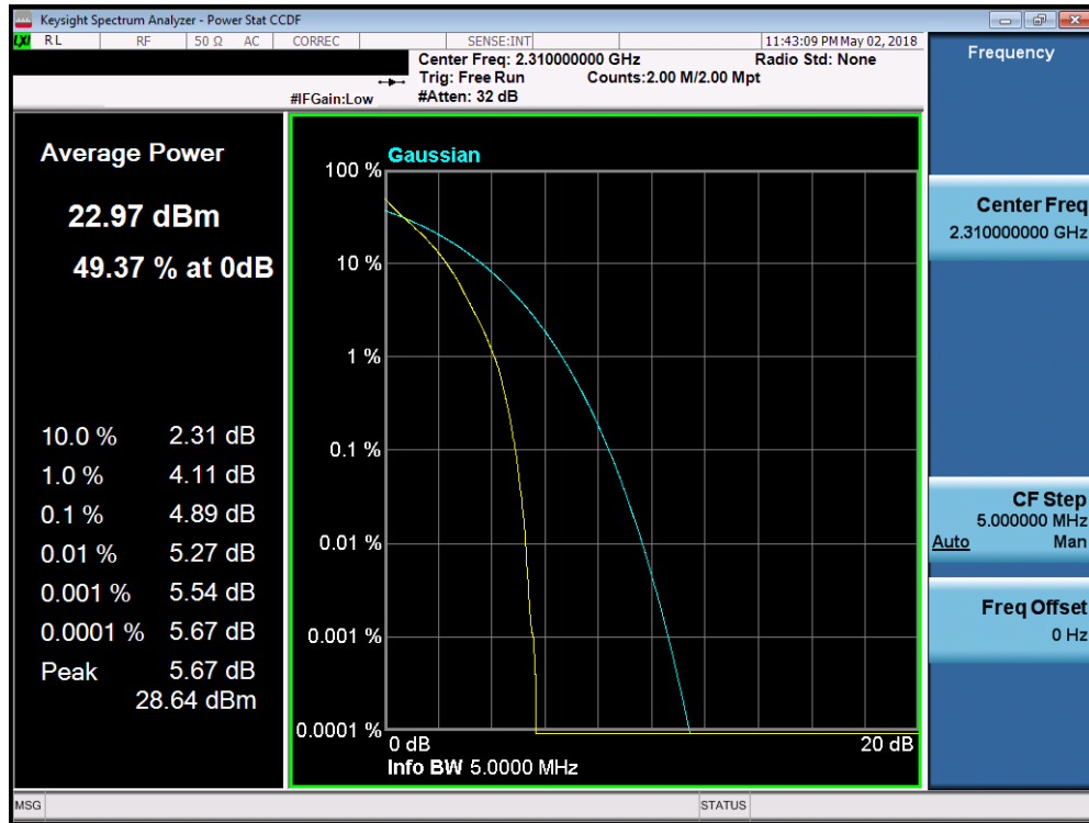
Plot 7-256. PAR Plot (Band 30 – 5.0MHz QPSK - Full RB Configuration)
