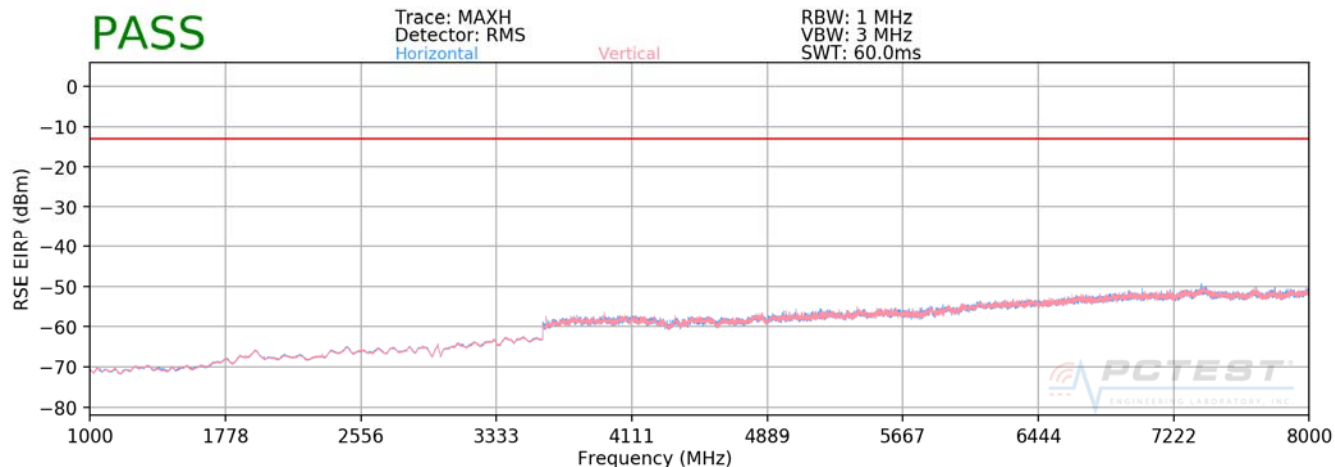
Plot 7-269. Radiated Spurious Plot above 1GHz (Band 13)
