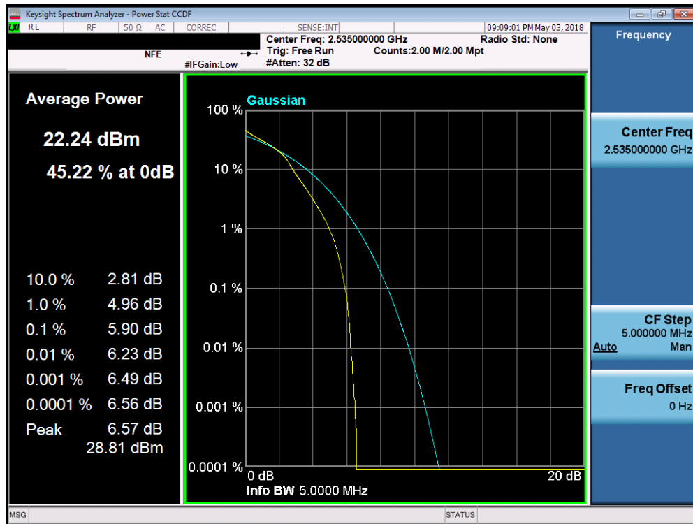
Plot 7-261. PAR Plot (Band 7 – 5.0MHz 16-QAM - Full RB Configuration)
