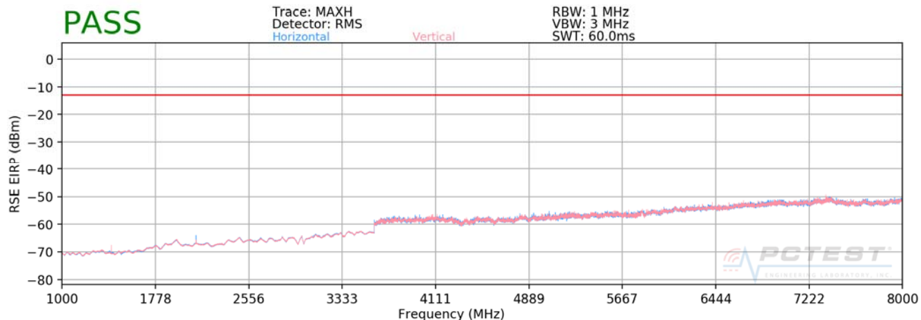
Plot 7-268. Radiated Spurious Plot above 1GHz (Band 12/17)
