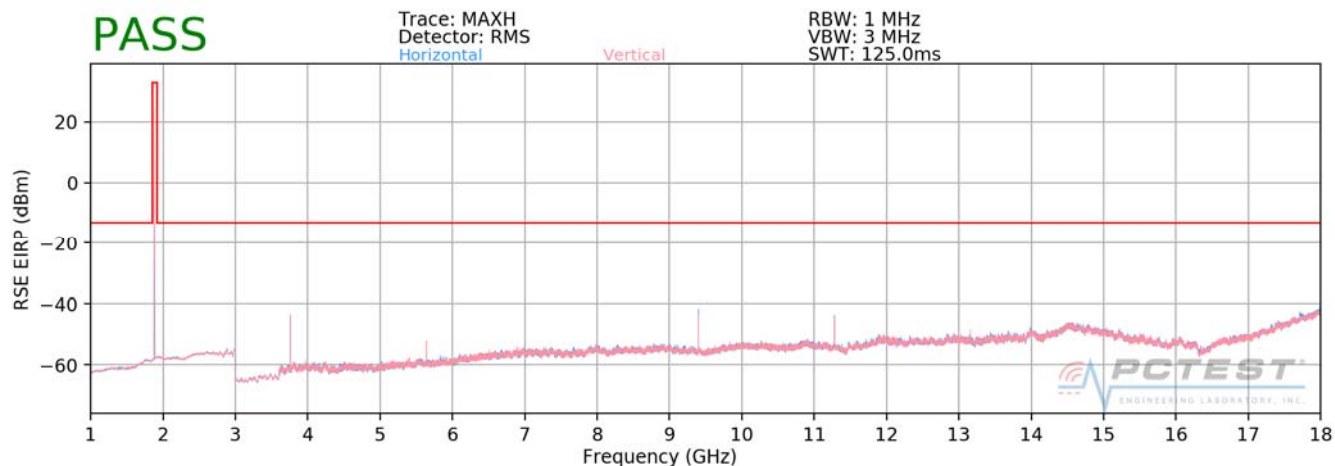
Plot 7-79. Radiated Spurious Plot 1GHz – 18GHz (PCS GPRS Mode)
