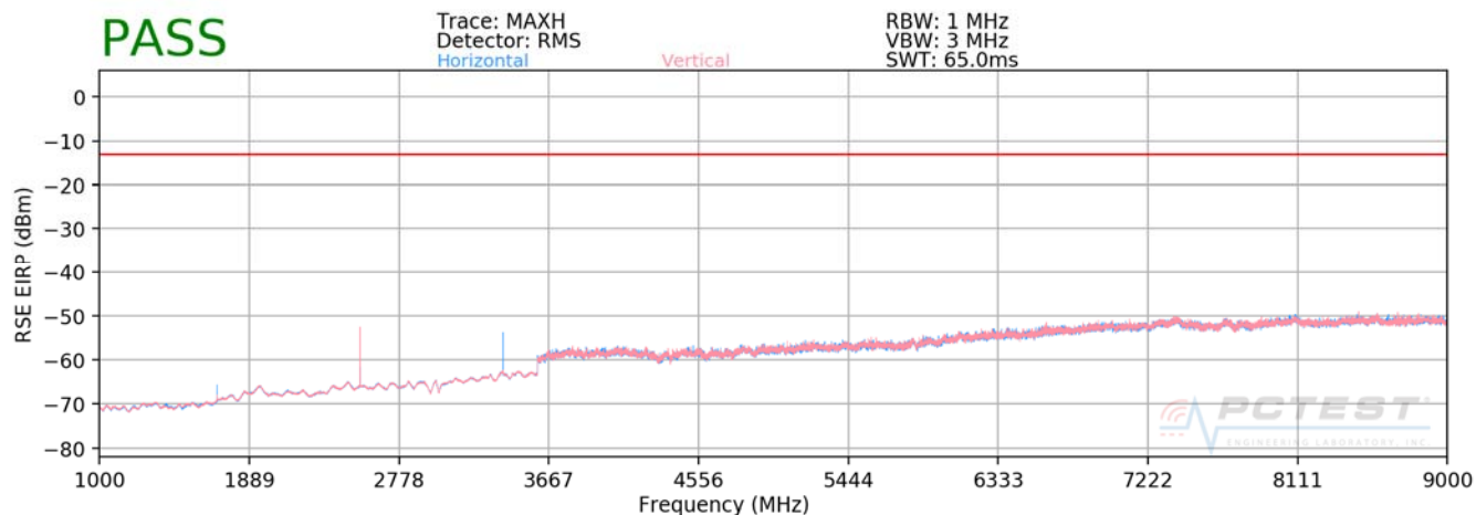
Plot 7-76. Radiated Spurious Plot 1GHz – 9GHz (Cellular GPRS Mode)
