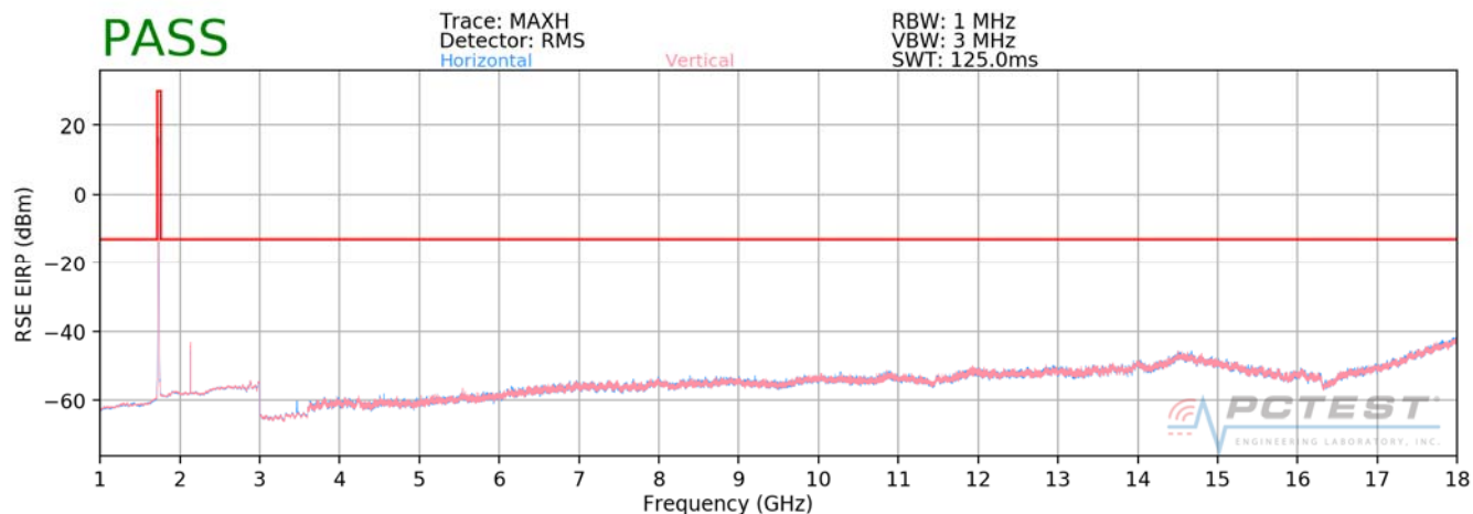
Plot 7-78. Radiated Spurious Plot 1GHz – 18GHz (AWS WCDMA Mode)
