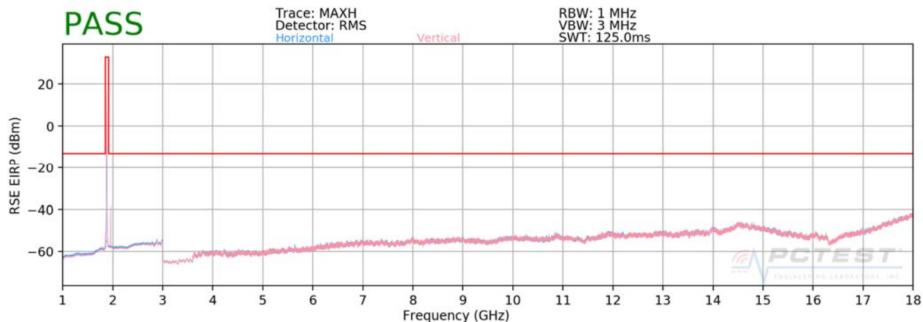
Plot 7-80. Radiated Spurious Plot 1GHz – 18GHz (PCS WCDMA Mode)
