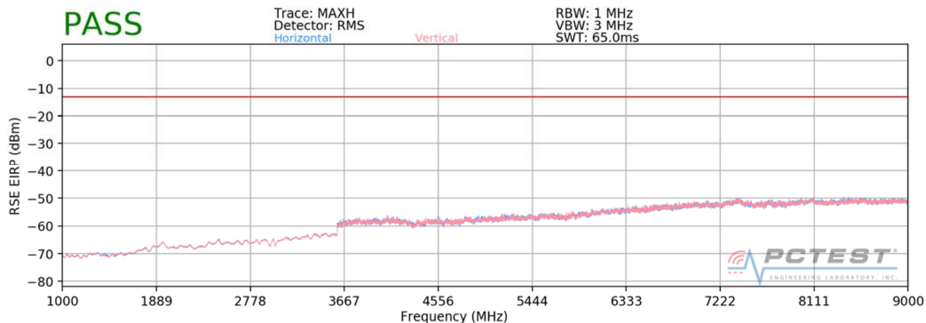
Plot 7-77. Radiated Spurious Plot 1GHz – 9GHz (Cellular WCDMA Mode)
