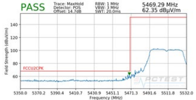
Plot 7-97. Radiated Lower Band Edge Plot (Peak – UNII Band 2C)
