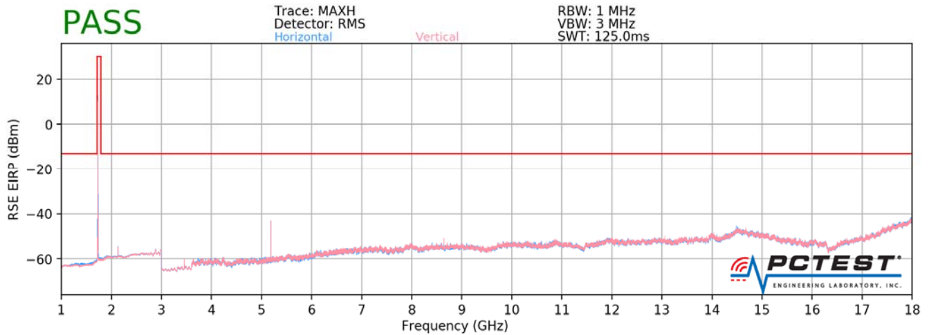
Plot 7-263. Radiated Spurious Plot above 1GHz (Band 66)
