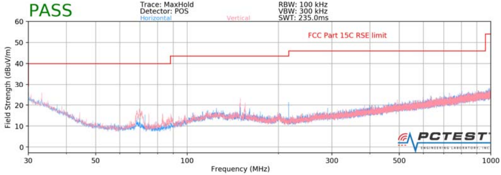
Plot 7-48. Radiated Spurious Plot below 1GHz
