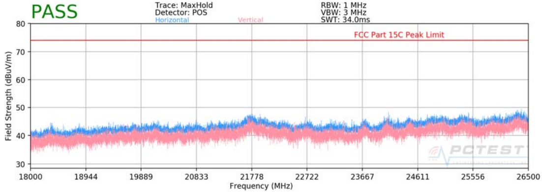
Plot 7-45. Radiated Spurious Plot above 18GHz
