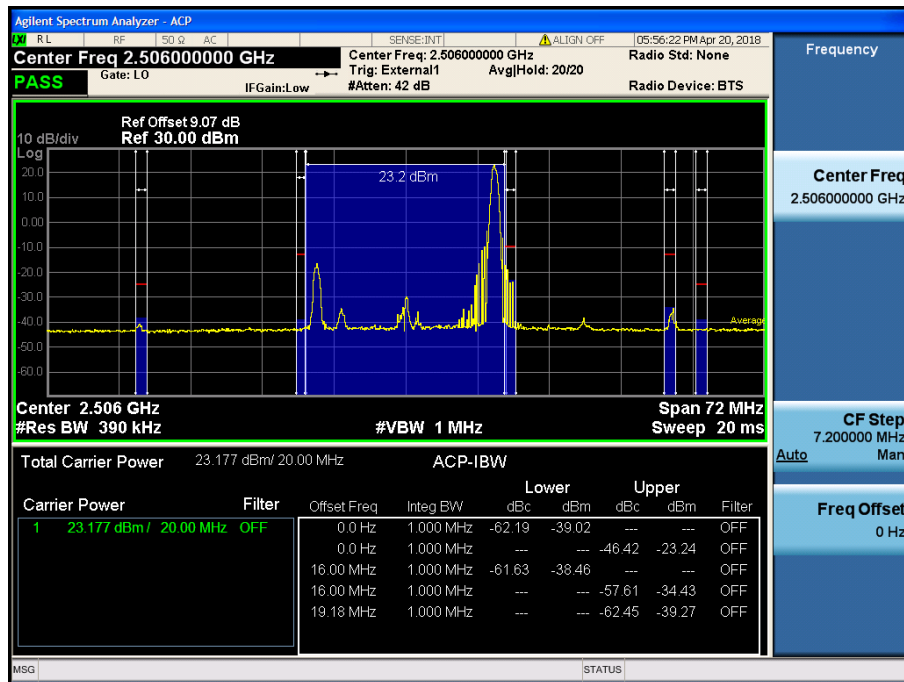
LTE Band 41 / 20MHz / QPSK - RB Size/Offset (1/99)
