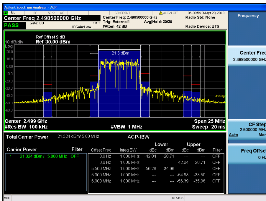
LTE Band 41 / 5MHz / 16QAM Offset/Size (25/0)
