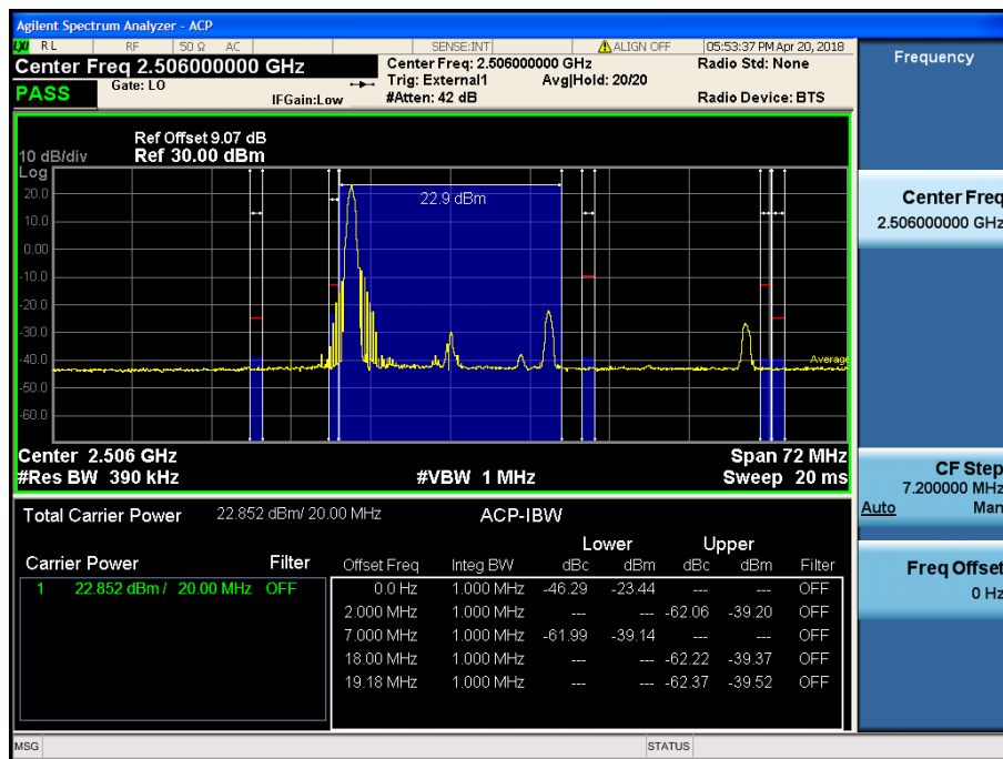
LTE Band 41 / 20MHz / QPSK - RB Size/Offset (50/50)
