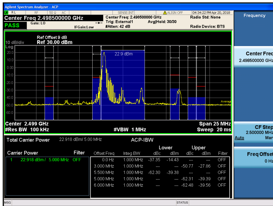
LTE Band 41 / 5MHz / QPSK Offset/Size (1/0)
