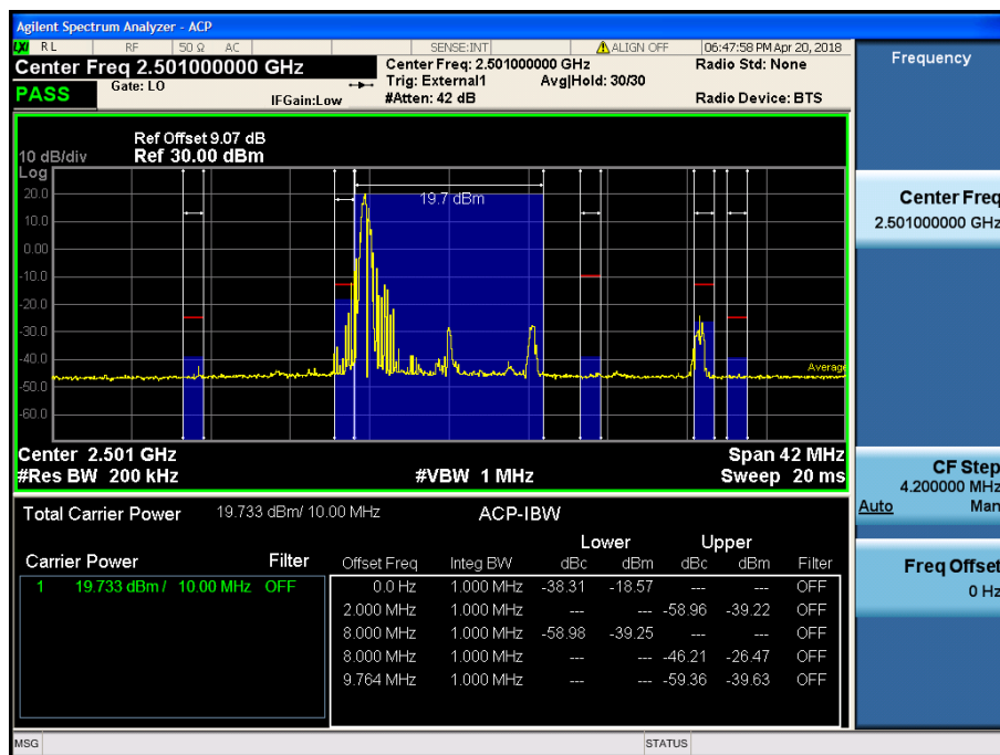
LTE Band 41 / 10MHz / 16QAM - RB Size/Offset (1/0)
