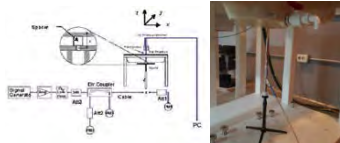
Figure 11.1 Dipole Verification Test Setup Diagram & Photo
